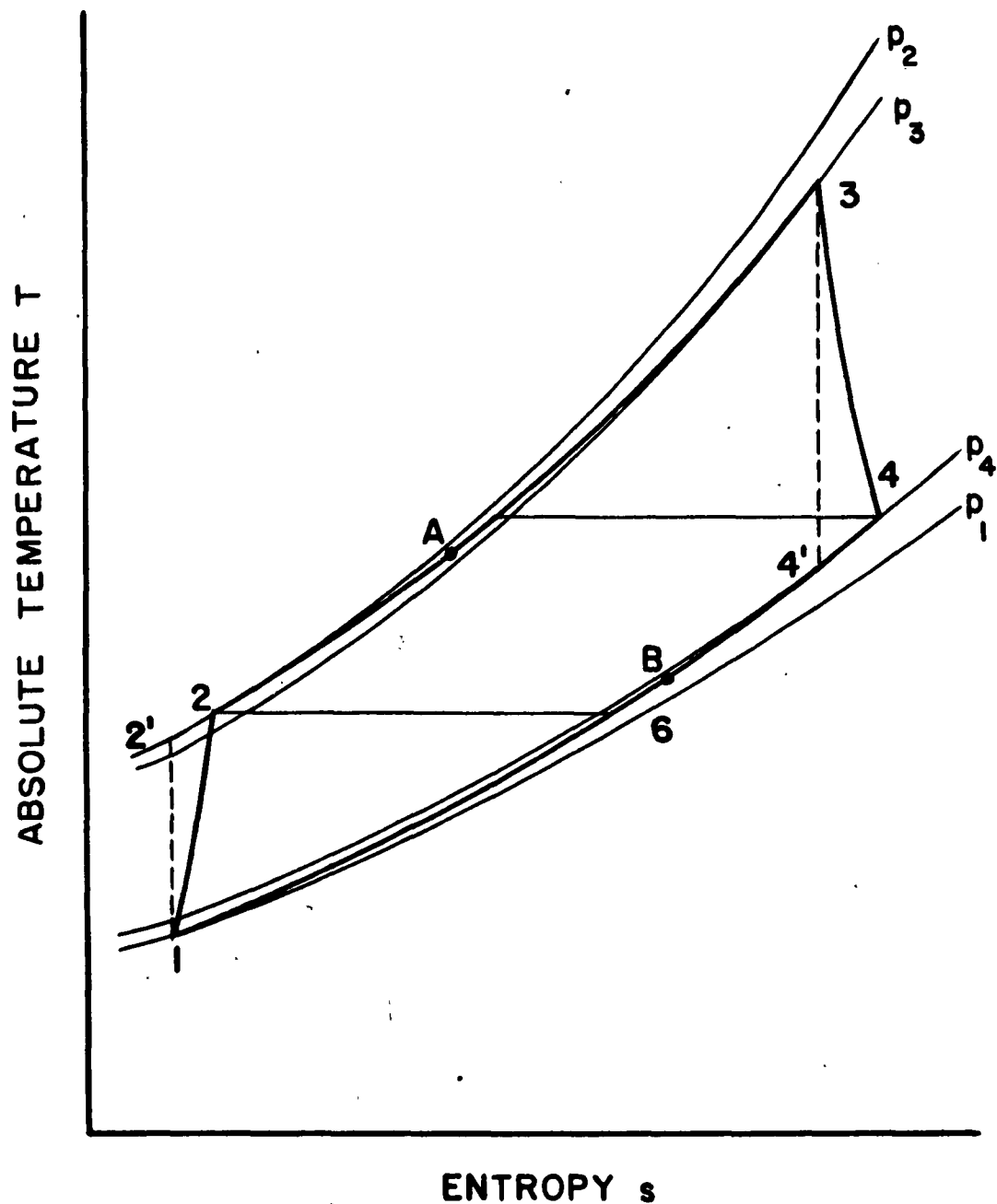
FIG. 4-1 TEMPERATURE-ENTROPY PLANE FOR A REAL REGENERATIVE GAS-TURBINE CYCLE
