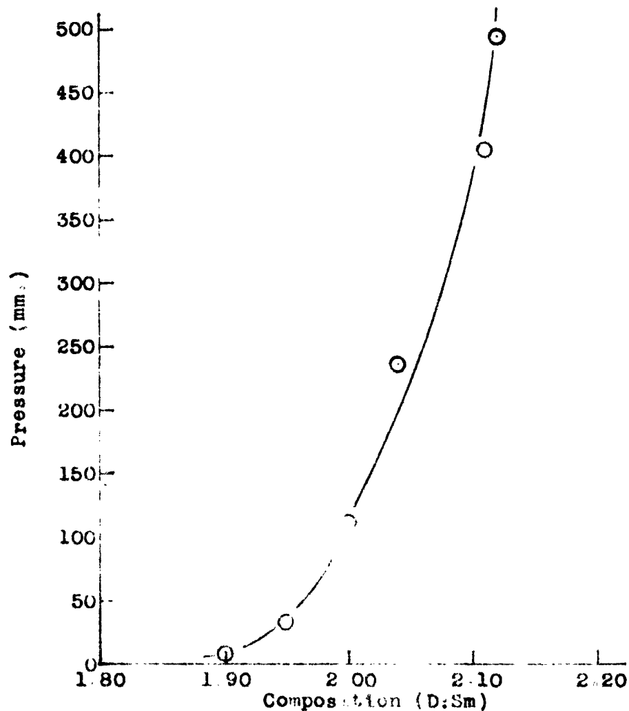
Figure 26. Dissociation pressure data for the samarium-deuterium system at 600° C.
