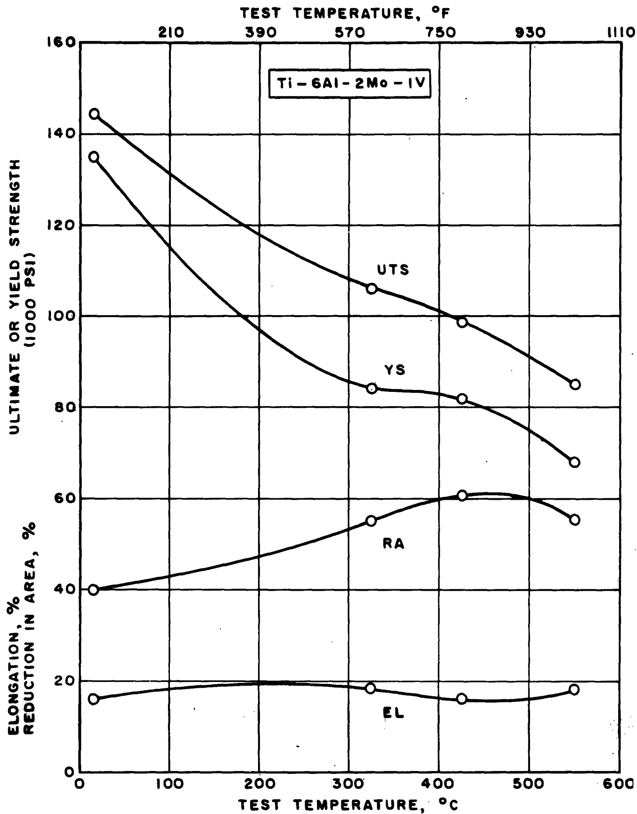
FIG. 8 - TENSILE PROPERTIES OF Ti-6%Al-2%Mo-1%V ALLOY
