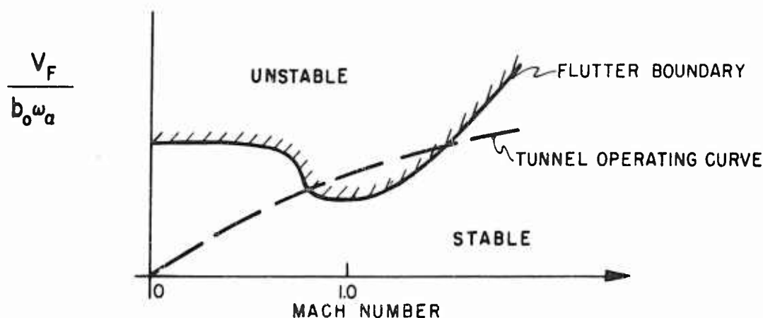
Fig. 21. Hypothetical flutter boundary.
