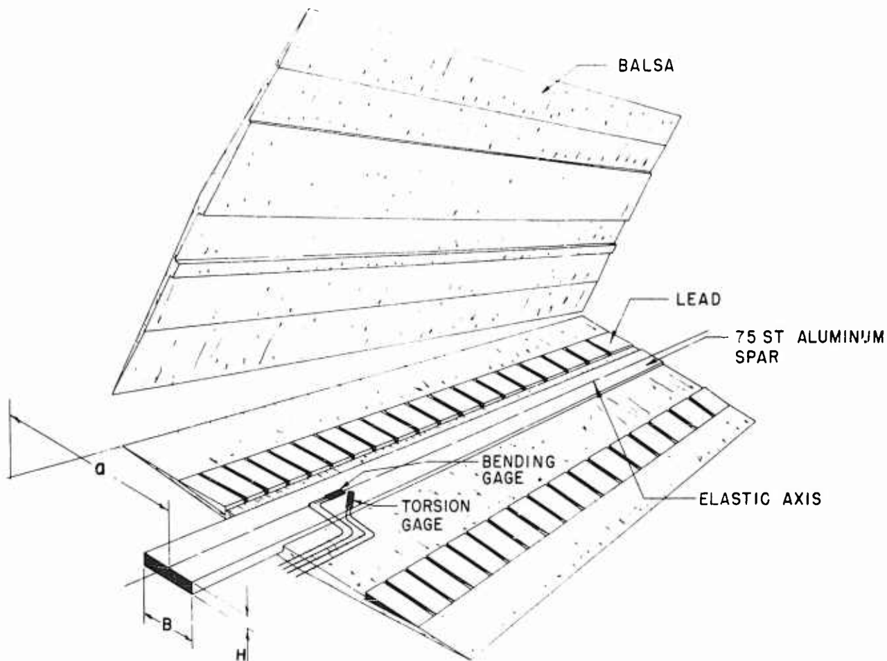
Fig. 2. Exploded view of straight wing.
