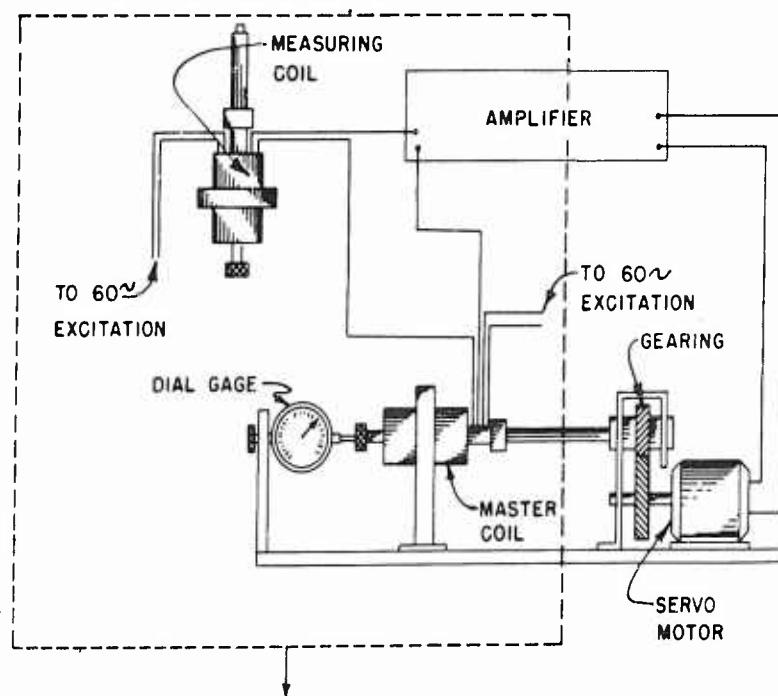
Fig. 9. Setup for static test using Schaevitz coils.
