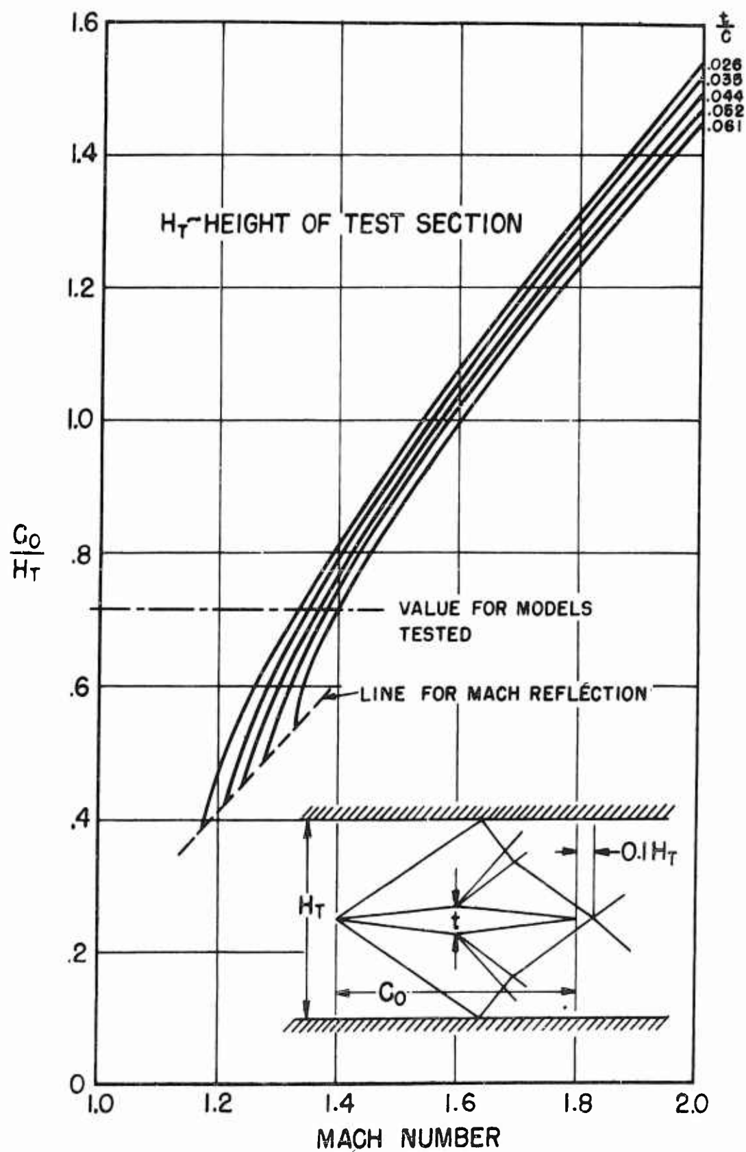
Fig. 20. Allowable root chord as determined by the two-dimensional shock wave pattern.
