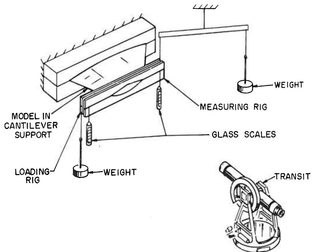
Fig. 6. Schematic diagram of optical system for EI, GJ and elastic axis position measurement.
