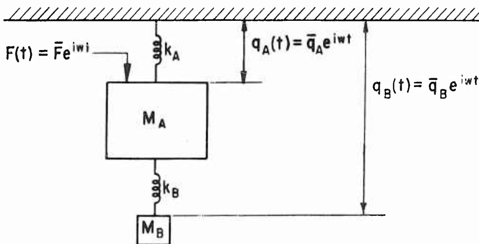
Fig. 12. Two-degree-of-freedom spring-mass system.
