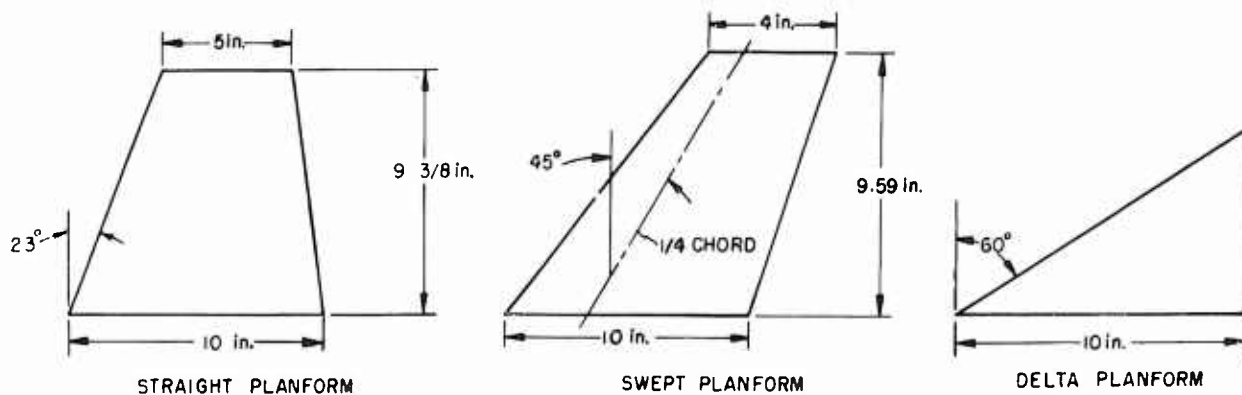
Fig. 1. Basic wing planforms.
