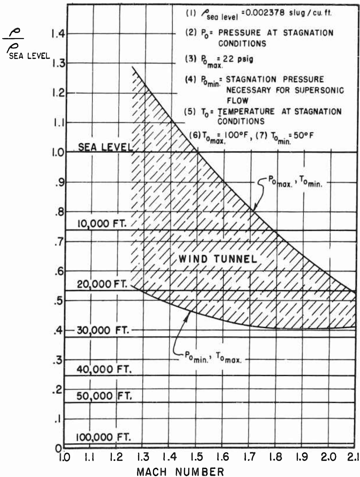
Fig. 22. Density versus Mach number for extreme ranges of atmospheric and wind tunnel conditions.
