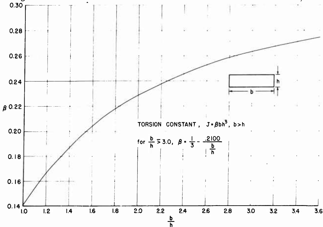
Fig. 5. Values of \beta for torsion constant of solid rectangular cross section.
