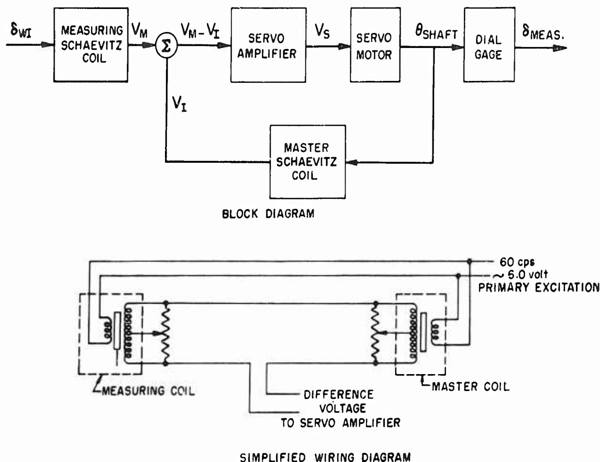
Fig. 10. Block and wiring diagram for null-balance Schaevitz coil system. position of the core of the indicating coil is recorded by a sensitive dial gage, and so the position of the core of the measuring coil can be recorded remotely by a sensitive dial gage. More than one measuring coil can be attached to the wing at a time, and a simple switching arrangement allows all the measuring coils to be compared one after another with the master coil. A large number of deflections on a wing can then be quickly read. Figure 11 is a photograph of a wing with a number of Schaevitz coils attached for the measurement of flexibility influence coefficients.
