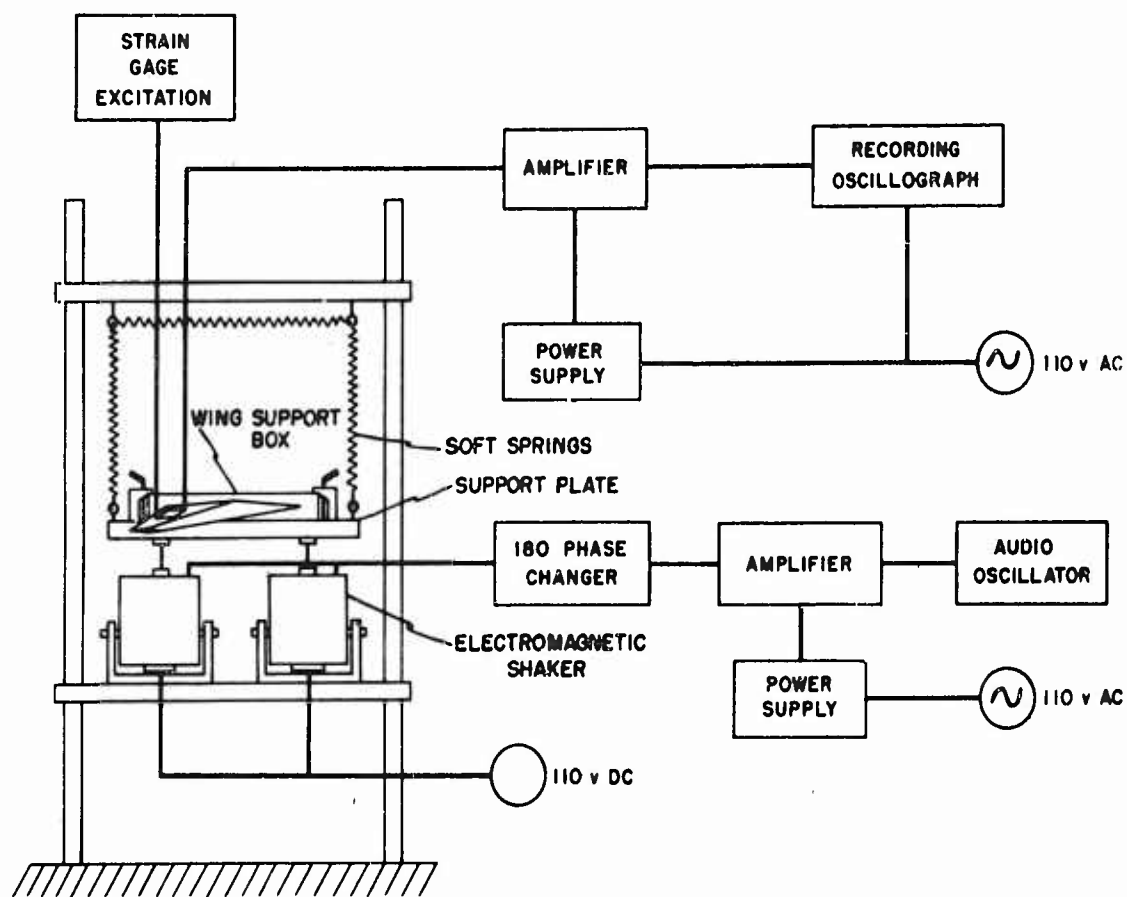
Fig. 13. Setup for vibration test using electromagnetic shaker.
