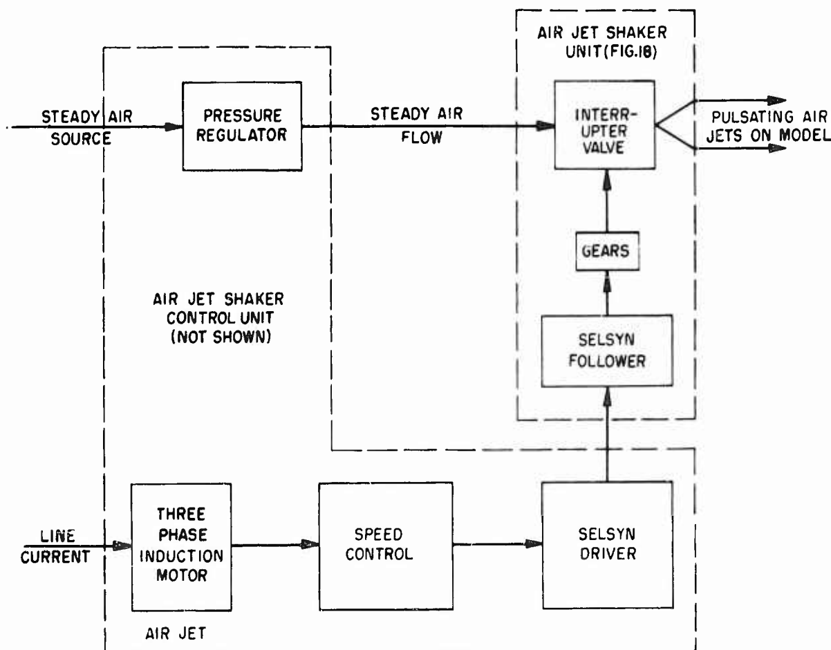
Fig. 19. Block diagram for air jet shakers.
