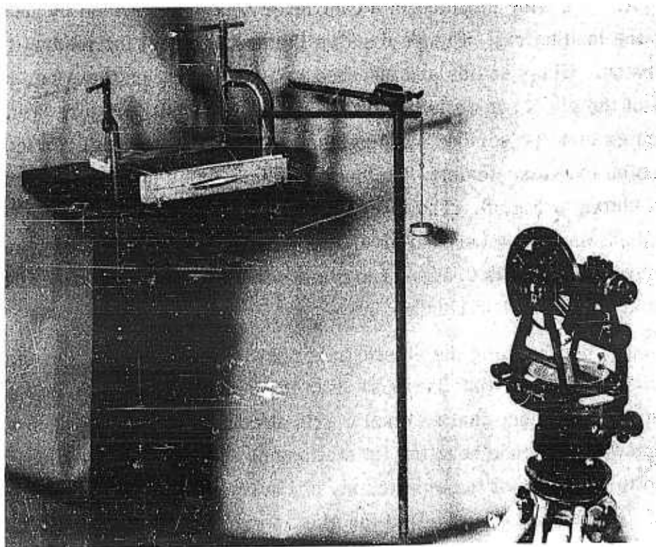
Fig. 7. Glass scale and transit measurement rig.
