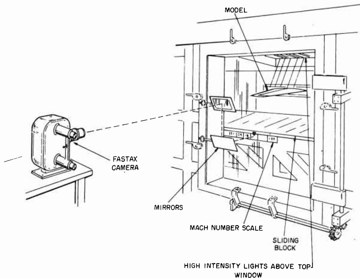
Fig. 24. Arrangement of camera for high speed photography.
