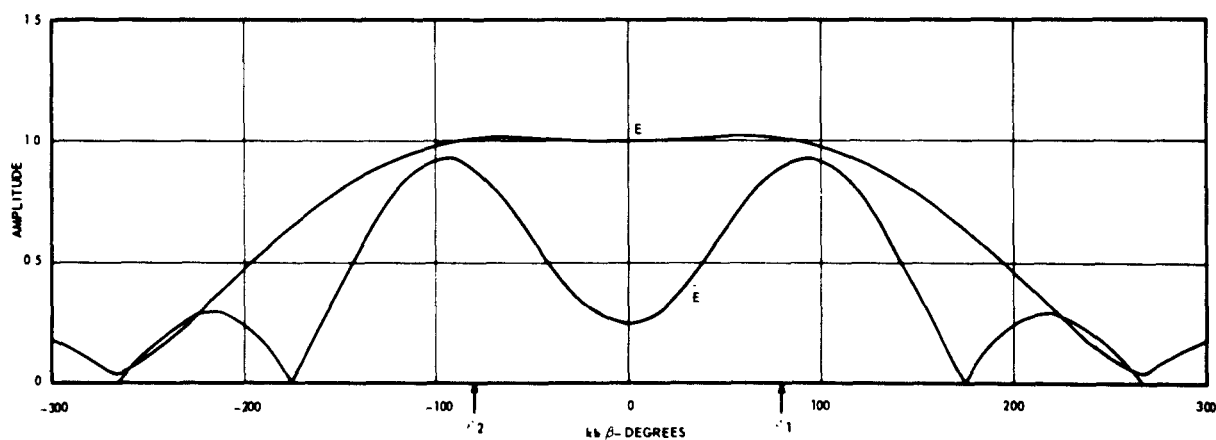
Figure 9. E and \tilde{E} for 160^\circ Separation of Two Incoherent Signals.
