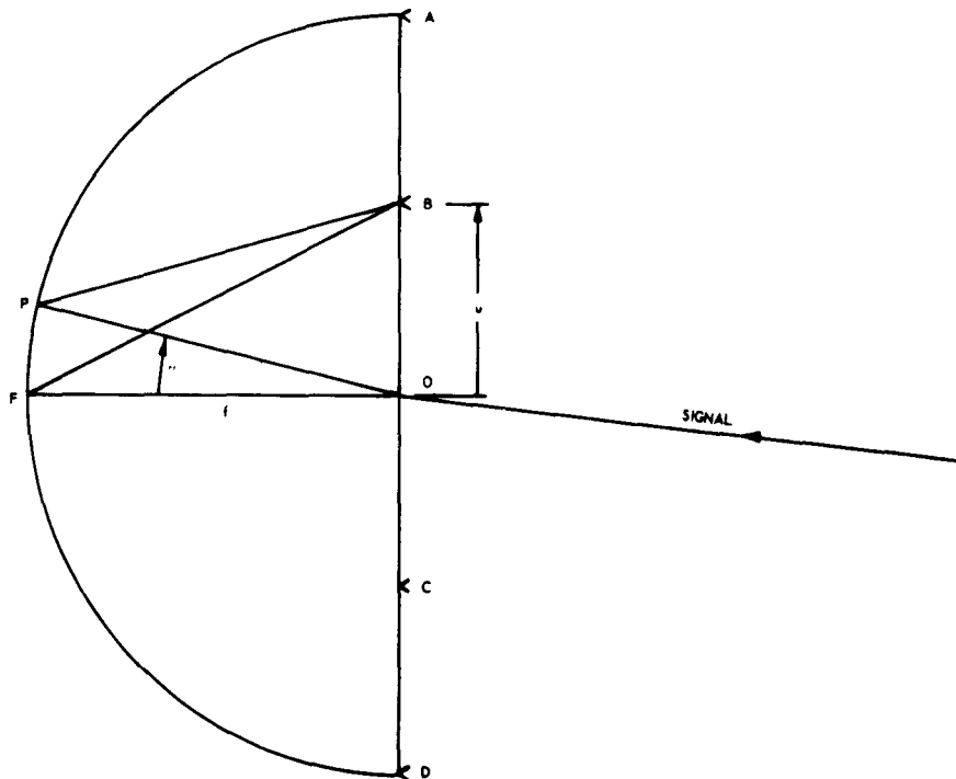
Figure 3. Four Horn Aperture Geometry.
