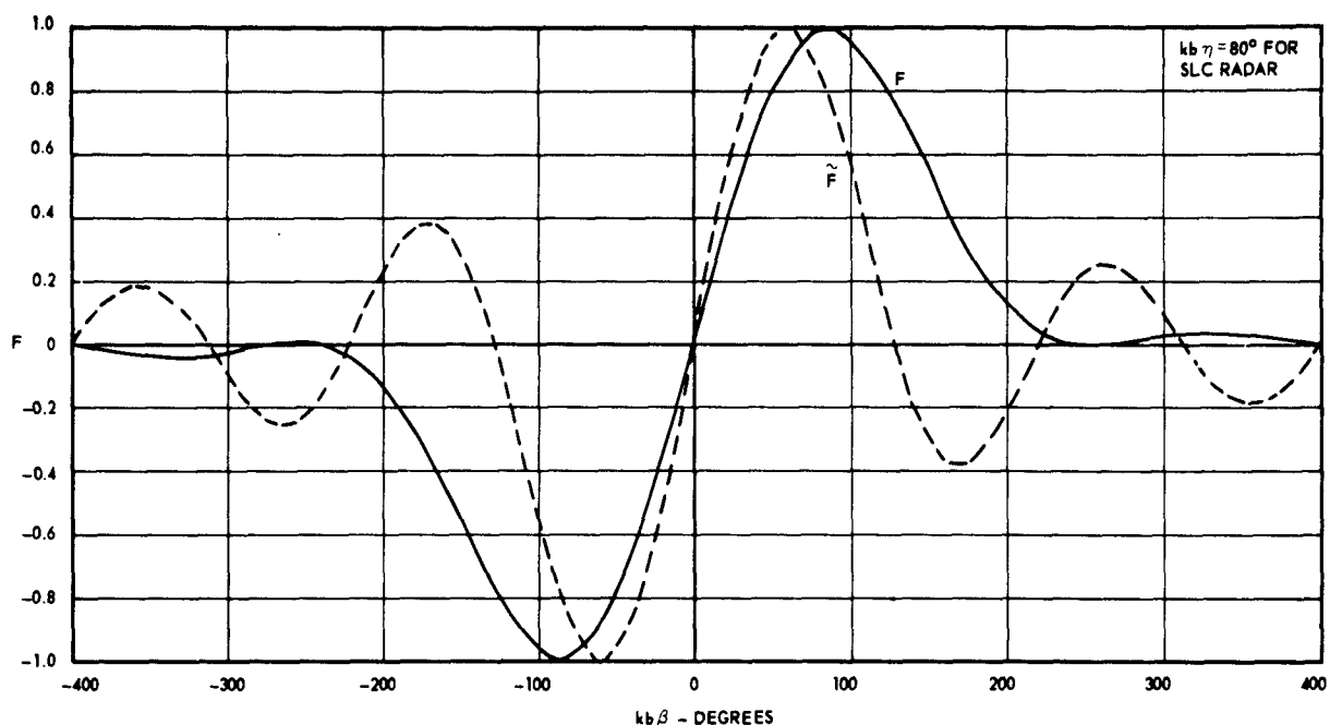
Figure 2. Normalized Error Signals for SLC Radar (F) and for Dot Product Scheme ( \tilde{F} ).
