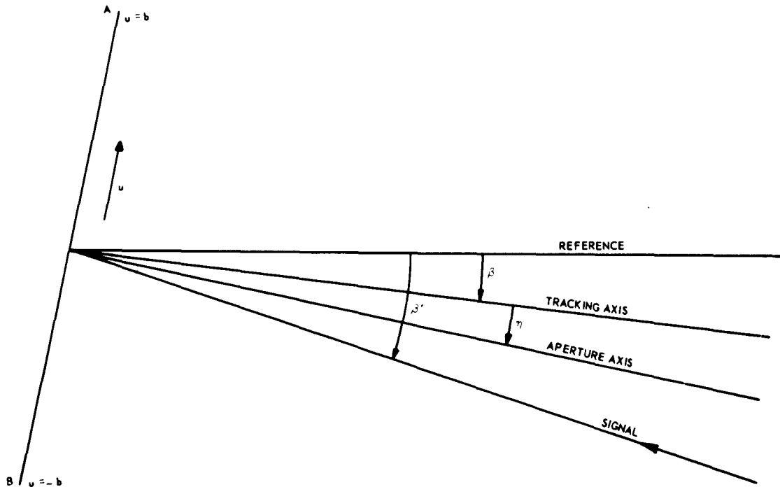
Figure 1. Antenna Geometry
