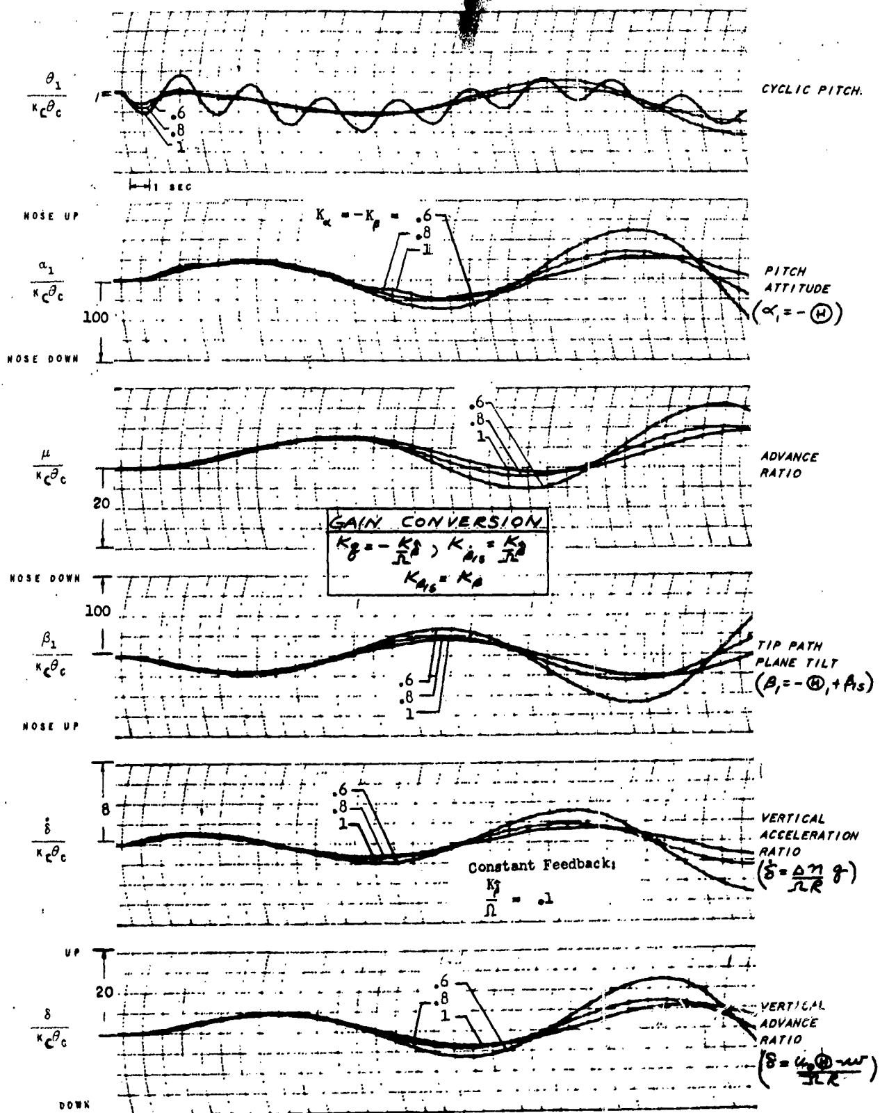
FIG. 62. AERODYNAMIC SERVO CONTROL FLAP ; \mu_0 = .2
