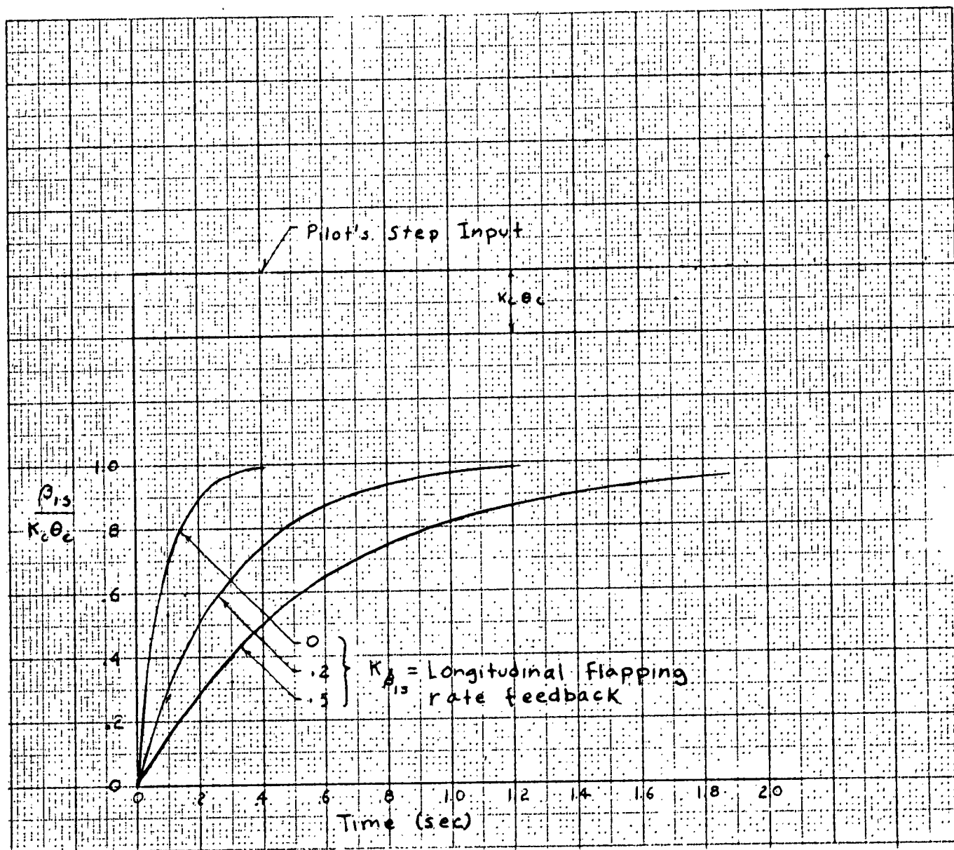
FIG. 45. VARIATION OF BLADE RESPONSE WITH FLAPPING RATE FEEDBACK (FUSELAGE FIXED)
