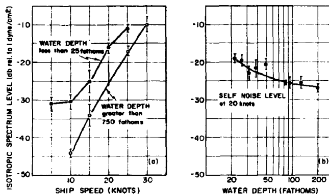
Figure 10 - Effect of water depth on self-noise in surface ships. Figure 10a shows the variation with speed for two water depths. Figure 10b shows the decrease in observed level in going from shallow to deep water. Data for QHB transducer in USS WRIGHT (CVL 49) on beam bearings (045, 090, 135, 225, 270, and 315), assumed directivity index 27 db, frequency 25 kc. (Ref. 34)
