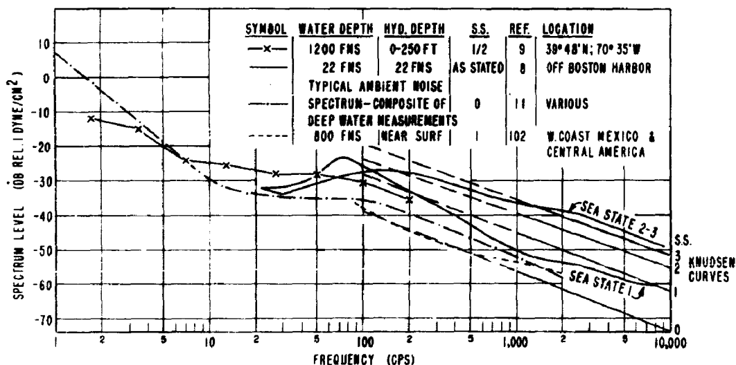
Figure 2 - Deep-water ambient-noise levels measured from surface vessels
