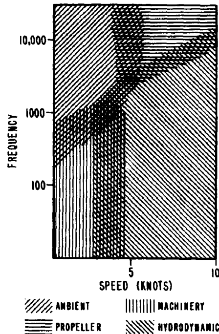
Figure 15 - Diagram showing the importance of the various sources of submarine self-noise at different frequencies and speeds for a forward topside hydrophone at periscope depth
