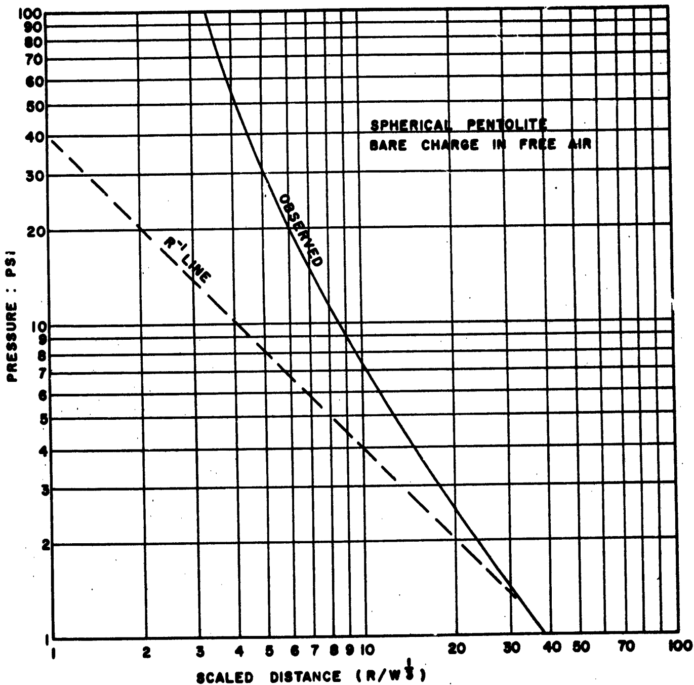
FIGURE 1: PEAK PRESSURE AS A FUNCTION OF SCALED DISTANCE. (BRL DATA)
