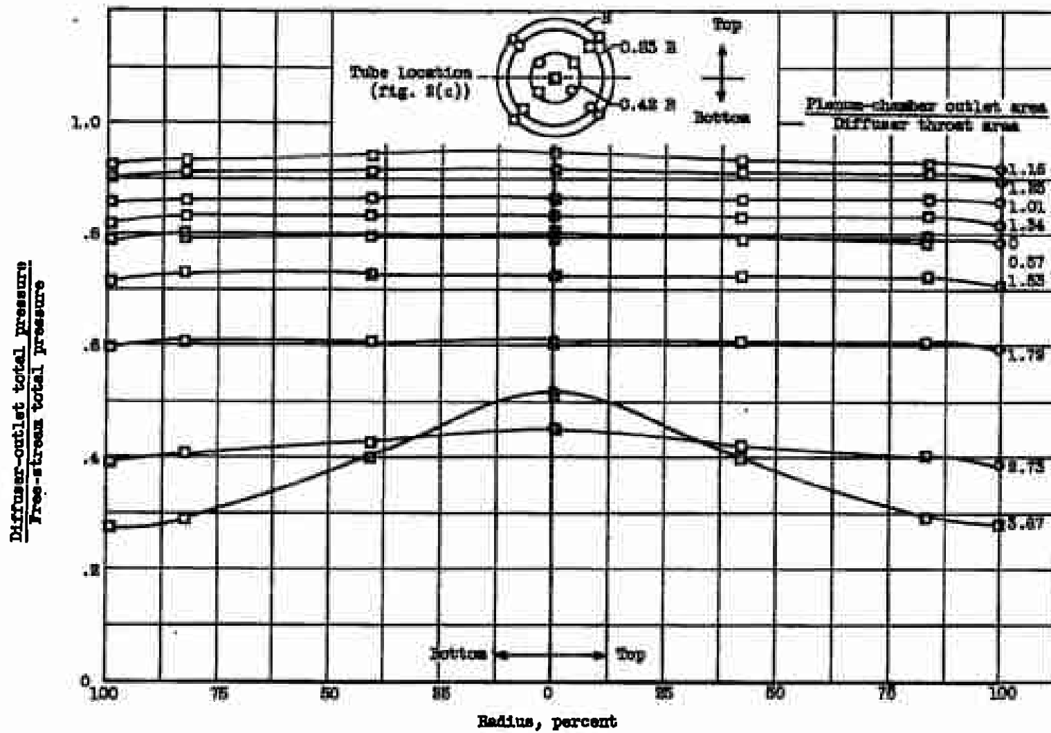
Figure 8. - Total-pressure distribution across diffuser outlet. Free-stream Mach number, 1.85.
