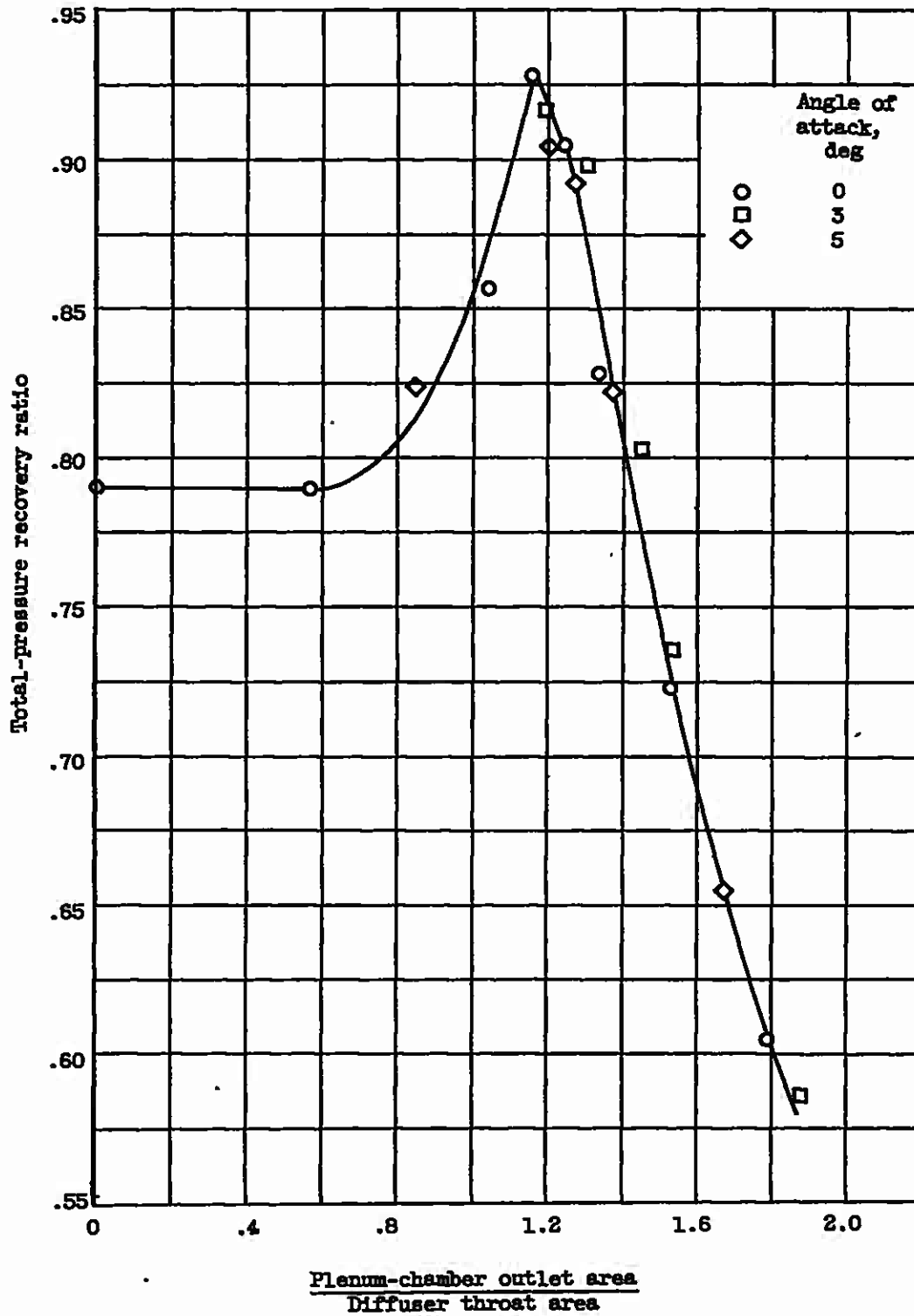
Figure 3. - Total-pressure recovery of perforated supersonic diffuser. Free-stream Mach number, 1.85.
