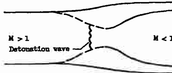
Stable location of detonation wave
