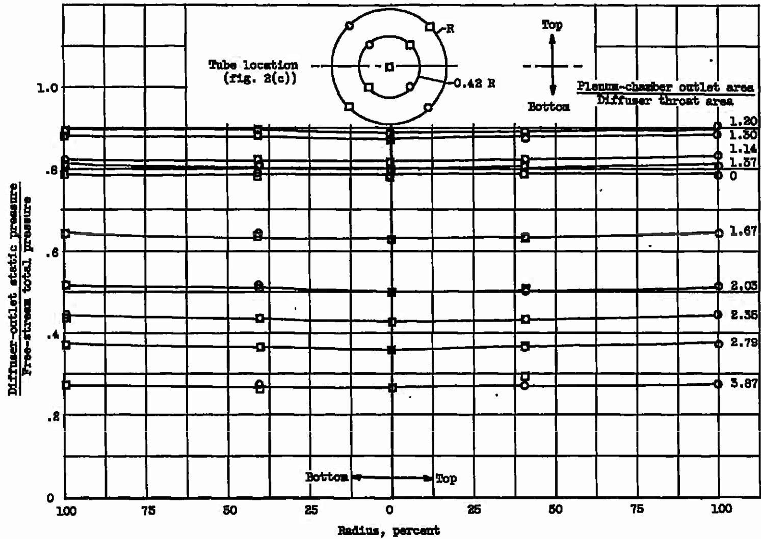
Figure 5. - Concluded. Static-pressure distribution across diffuser outlet. Free-stream Mach number, 1.85.
