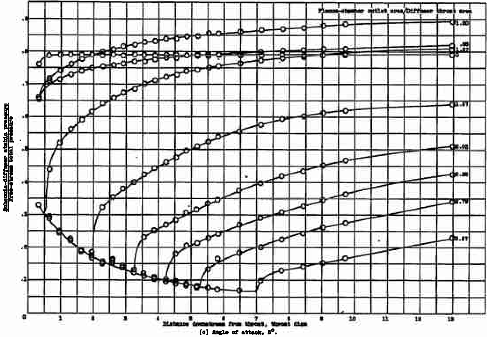
Figure 4. - Concluded. Static-pressure distribution along subsonic diffuser. Free-stream Mach number, 1.05.
