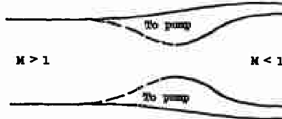
Second throat of supersonic wind tunnel
