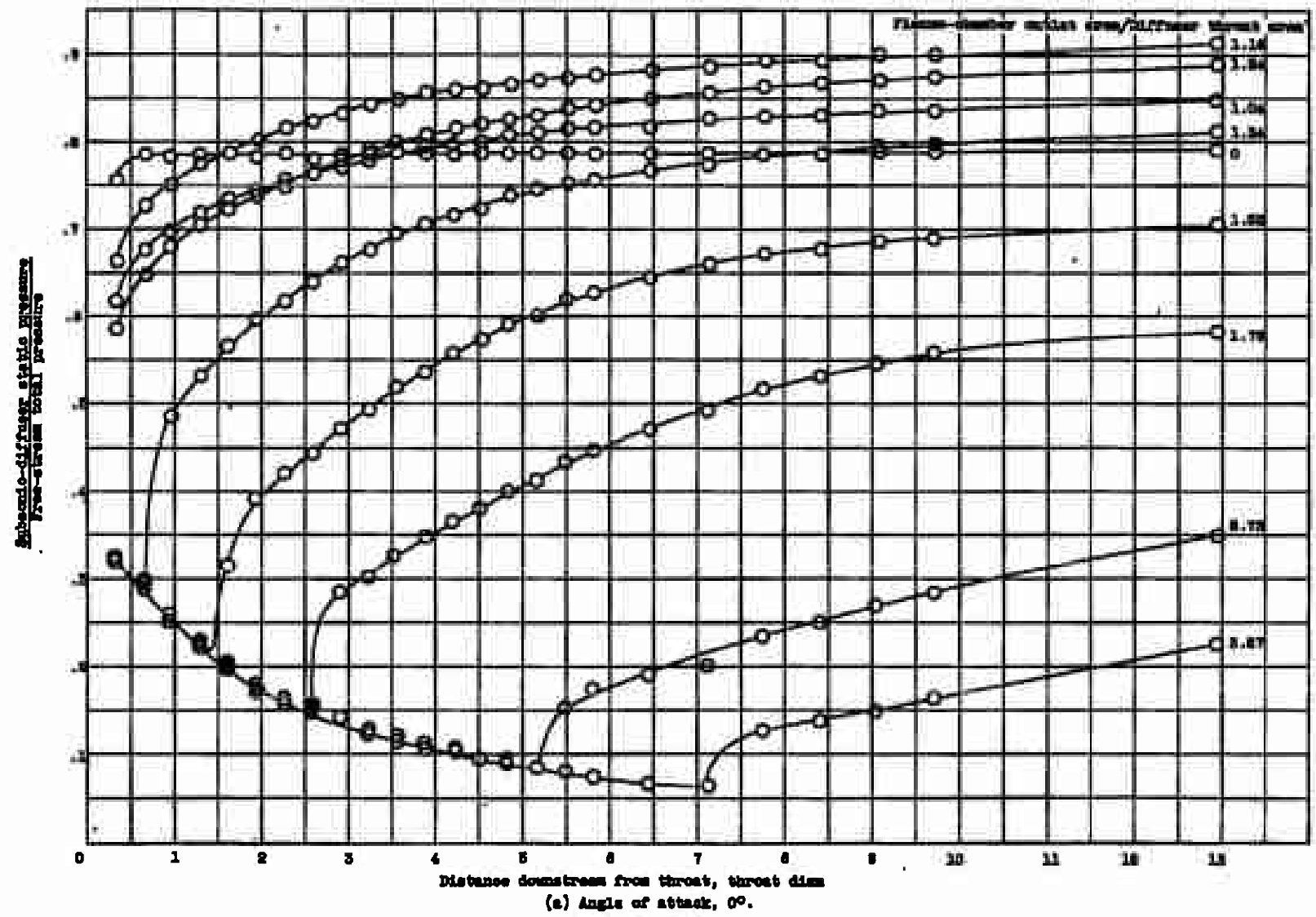
Figure 4. - Static-pressure distribution along subsonic diffuser. Free-stream Mach number, 1.00.
