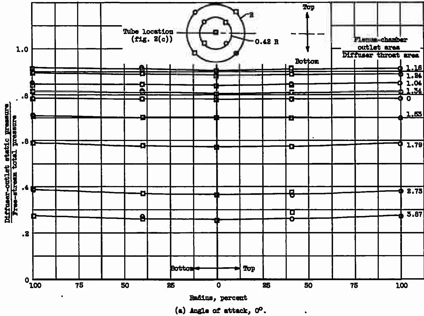
Figure 5. - Static-pressure distribution across diffuser outlet. Free-stream Mach number, 1.85.
