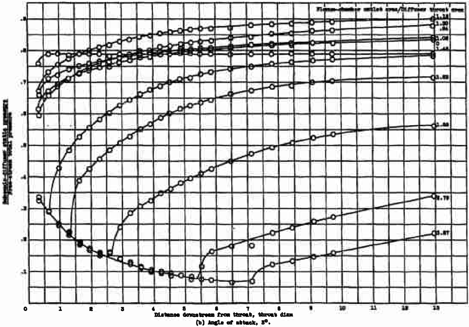
Figure 4. - Continued. Static-pressure distribution along subsonic diffuser. Free-stream Mach number, 1.05.
