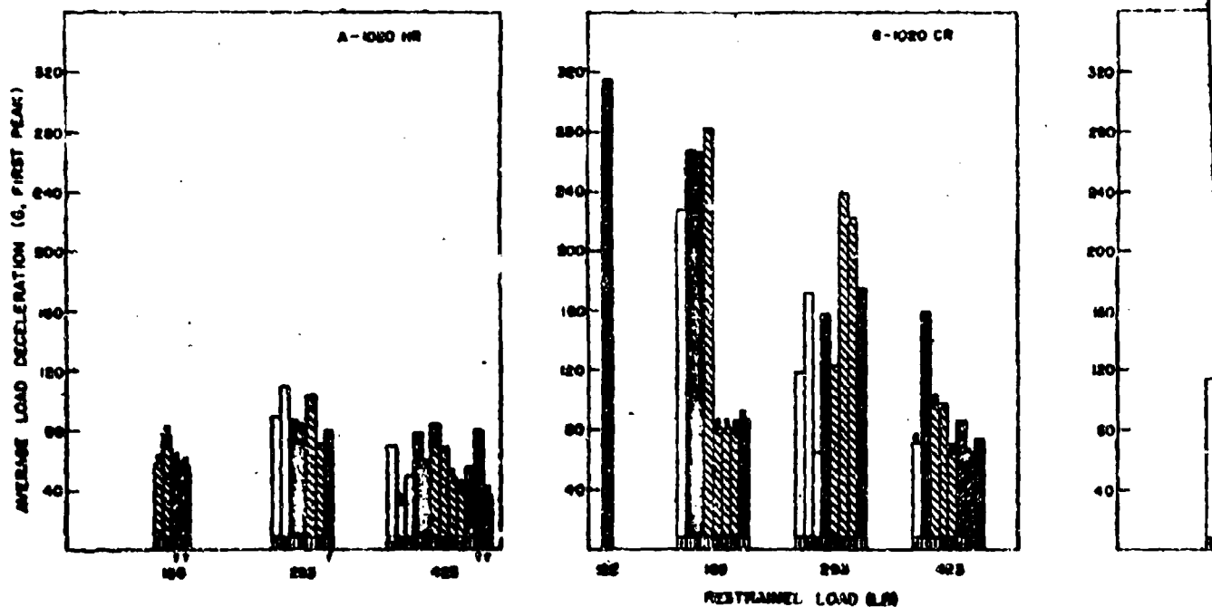
Fig. 12 - Average load deceleration (first peak) vs restraint load. This quantity is derived from the negative slope of the load vs displacement curve and hence is probably a better measure of the bolt performance than the values given by the accelerometer. The values given
