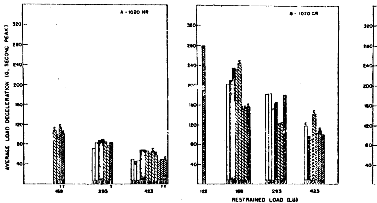
Fig. 14- Average load deceleration (second peak) vs restrained load. It may be noted that decelerations during this period are lower than those during the first peak. The values shown are averages for all blows.
