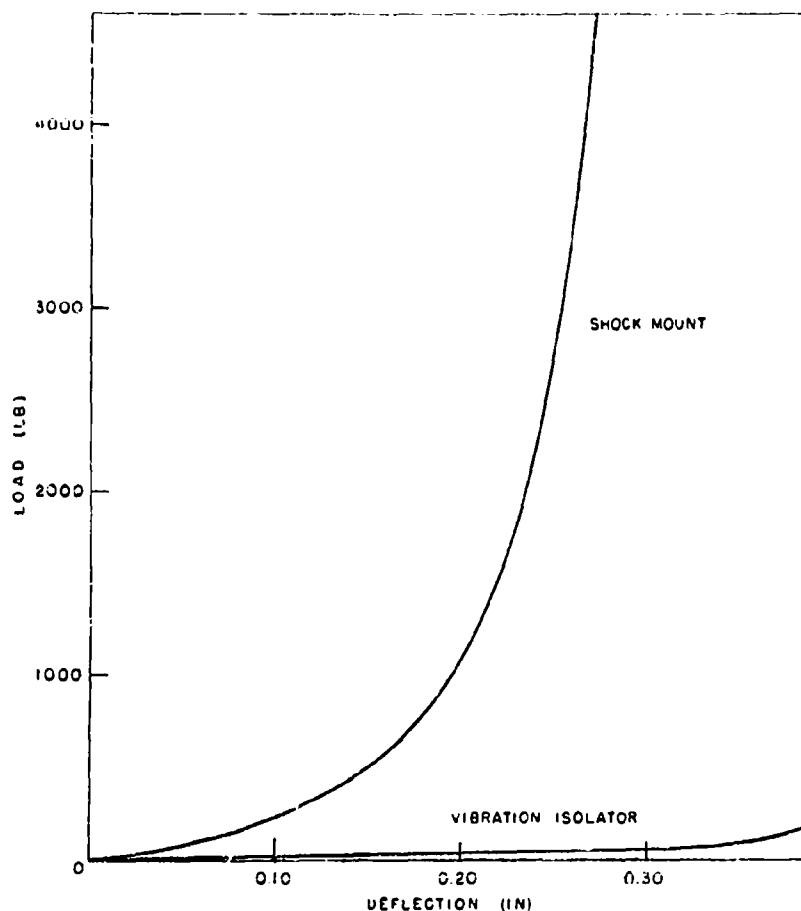
Fig. 1 - Load-deflection curves for a typical shock mount and a typical vibration isolator, both of which have a nominal load rating of approximately 20 lb. The shock mount is resonant at 25 cps and the isolator at 8 cps.
