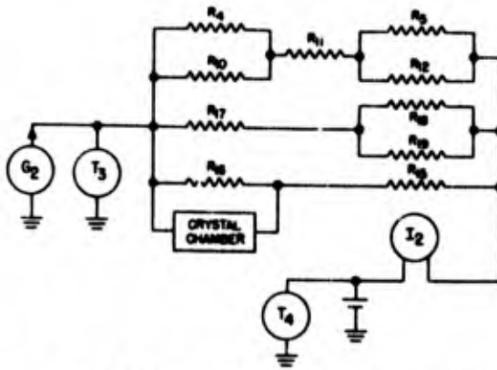
Figure 4-14. Thermal D-C path of heater power
