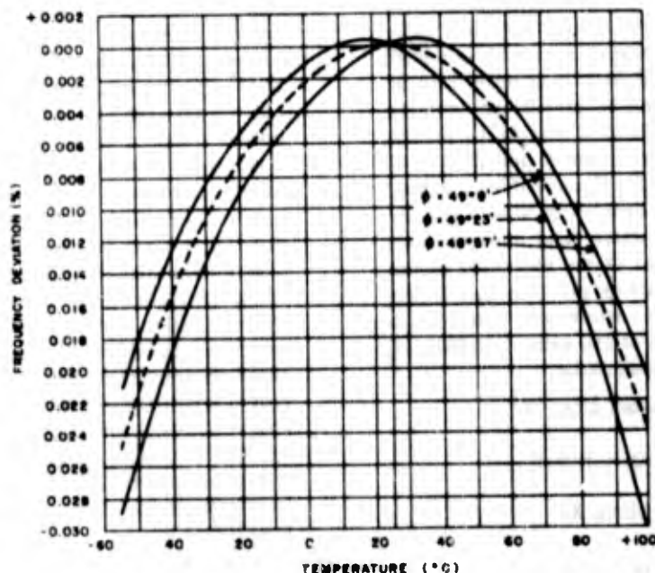
Figure 1-50. Temperature-frequency characteristics of element B
