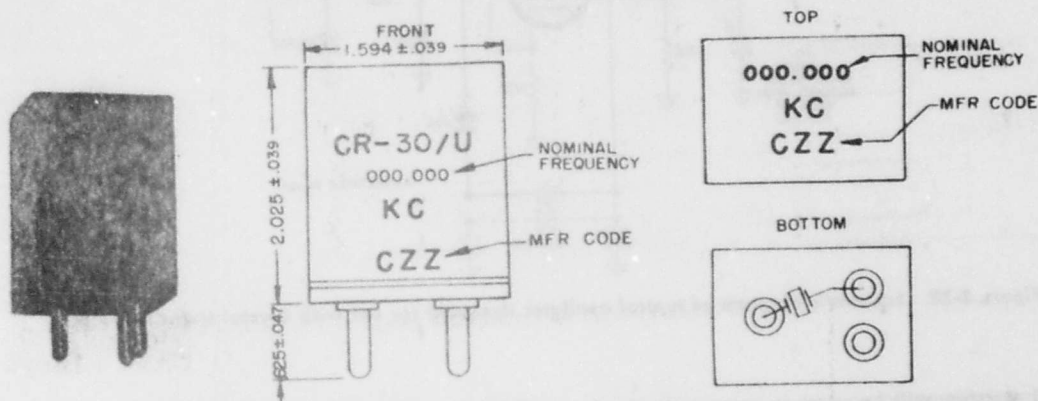
Figure 2-23. Crystal Unit CR-30/U
