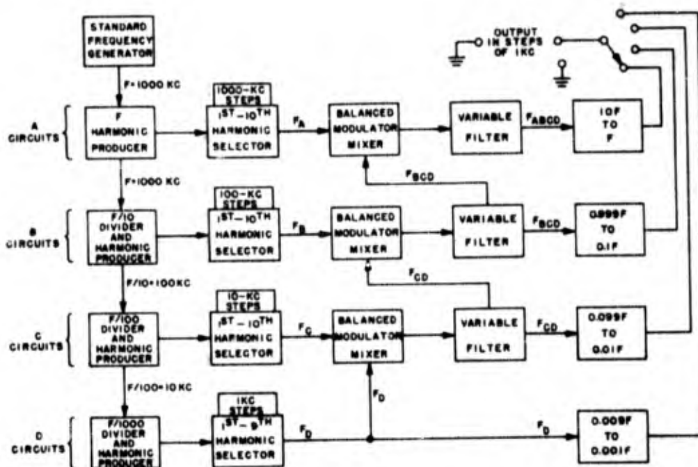
Figure 1-188. Block diagram of a Plessey synthesizer designed to cover the 0—10-mc spectrum in 1-kc steps
