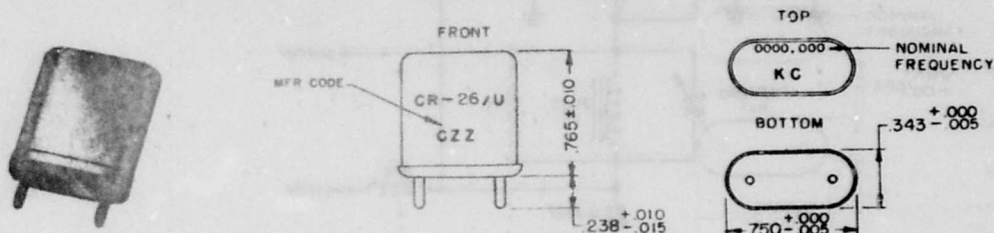
Figure 2-15. Crystal Unit CR-26/U
