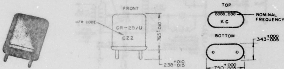
Figure 2-13. Crystal Unit CR-25/U
