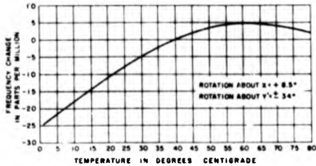
Figure 1-35. Frequency-temperature characteristics of element M*
