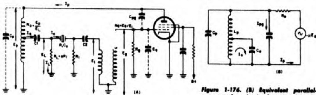
Figure 1-176. (A) Basic circuit of transformer-coupled oscillator
