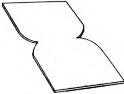
Figure 1-76. Dielectric sheet cut to fill air gap of nodal-clamped mounting
