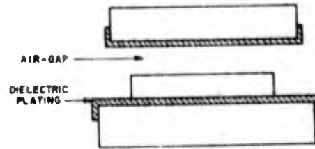
Figure 1-77. Cross-sectional view of gravity-air-gap mounting with electrode surfaces protected by coating of high-dielectric material
