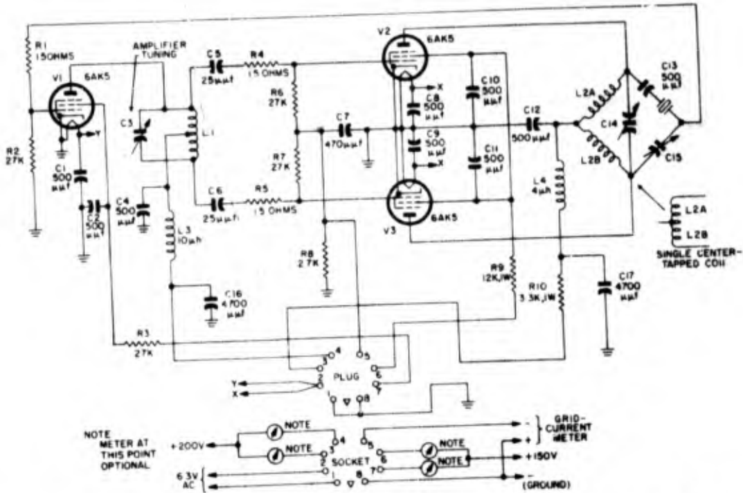
Figure 1-171. A multitube capacitance-bridge oscillator which is practical for operation in the 50-200-mc range. Resistors not otherwise specified are rated at 1/2 w
