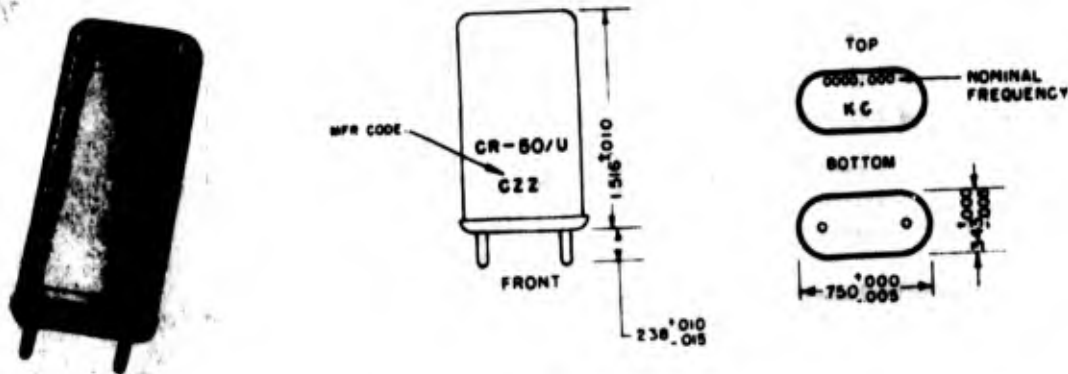
Figure 2-57. Crystal Unit CR-50/U
