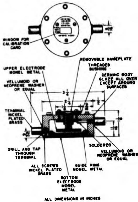
Figure 3-18. Crystal Holder FT-164
