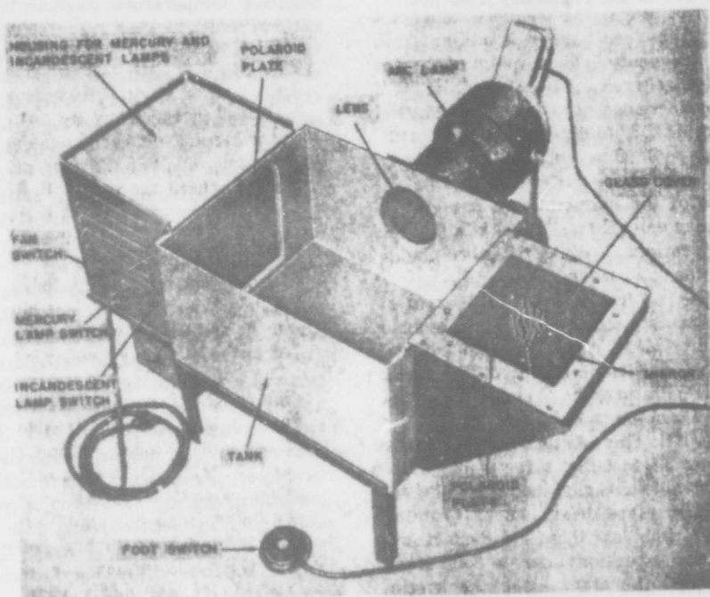
Figure 1-57. Polariscope-inspectoscope. Used for examining raw quartz
