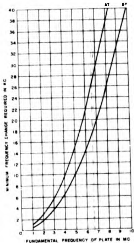
Figure 1-89. Minimum change in frequency that AT and BT plates must undergo due to etching, if the etching is to be sufficient to remove all surface cracks and fissures remaining from the final lapping stage. Note that, as the crystal becomes thinner, a given change in the thickness dimension means a greater change in the frequency. The frequency change for a BT cut is less than that for an AT cut of the same initial frequency, since the larger frequency constant of the BT cut permits a thicker plate
