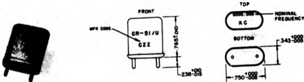
Figure 2-59. Crystal Unit CR-51/U
