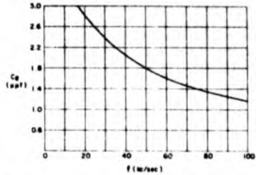
Figure 1-94. C_0 versus frequency for typical wire-mounted N elements
