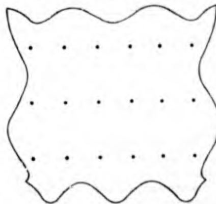
Figure 1-13. Face-shear mode for m = 6 , n = 3 . Dots indicate nodes *
