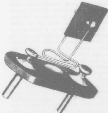
Figure 1-85. Solder-cone wire mounting of face-shear element
