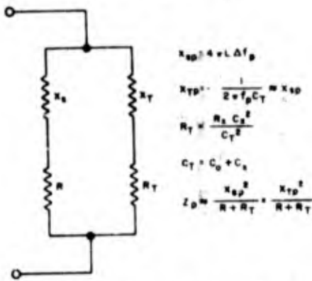
Figure 1-102. Equivalent parallel-resonant tank circuit, in which the motional impedance of the crystal unit is the inductive arm of the tank, and the total shunt impedance is the capacitive arm
