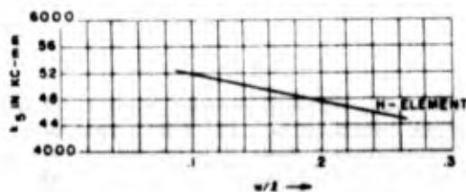
Figure 1-27. Frequency constant versus w/l ratio for element H
