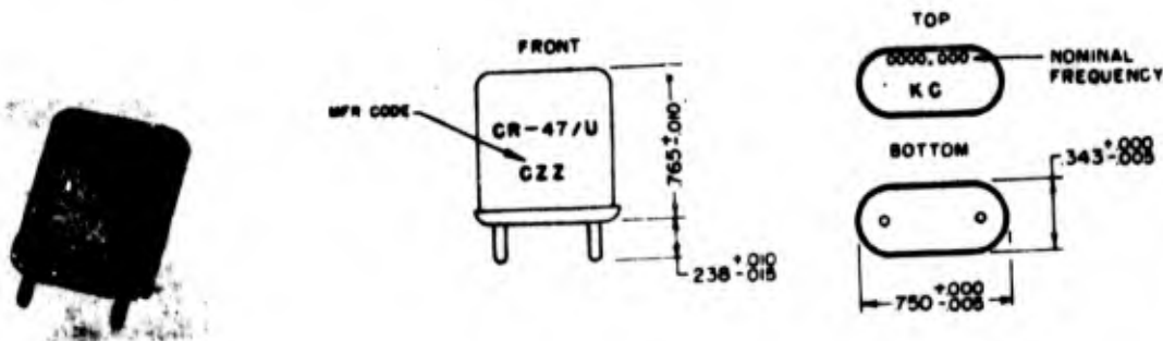
Figure 2-51. Crystal Unit CR-47/U
