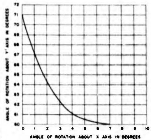
Figure 1-37. Angles of rotation for N element with w/l ratio of 0.05 which will provide zero temperature coefficient at 25°C*
