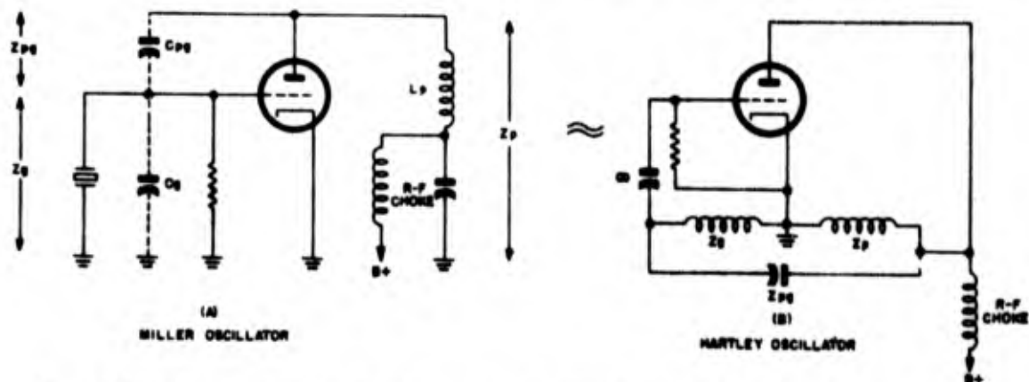
Figure 1-140. Diagrams illustrating the equivalence between the Miller circuit and the Hartley circuit
