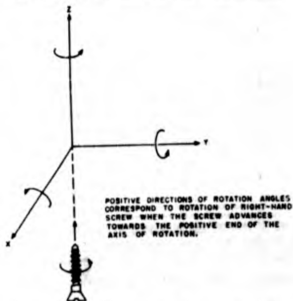
Figure 1-14. Positive directions of angles of rotation according to conventions of right-handed coordinate system
