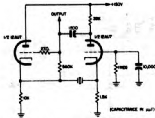
Figure 2-4. Schematic diagram of typical oscillator designed for use with Crystal Unit CR-16/U
