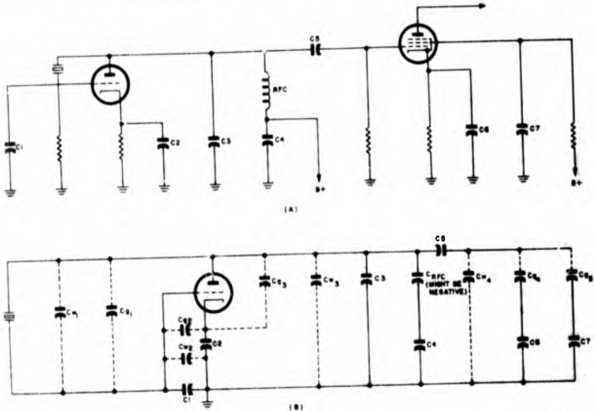
Figure 1-124. (A) Conventional Pierce oscillator and buffer-amplifier circuit. (B) Static capacitances of circuit (A). C_p = interelectrode capacitances. C_w = distributed capacitances of wires
