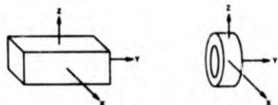
Figure 1-48. Y-cut block and doughnut-shaped crystals which can provide zero temperature coefficients for certain combination modes
