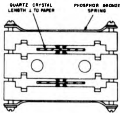
Figure 1-83. Knife-edge clamp support for two crystal plates. Each crystal has two pairs of plated electrodes, and is so mounted that each pressure blade makes electrical contact with a different electrode. This arrangement effectively provides four crystal elements for use in a balanced filter circuit*
