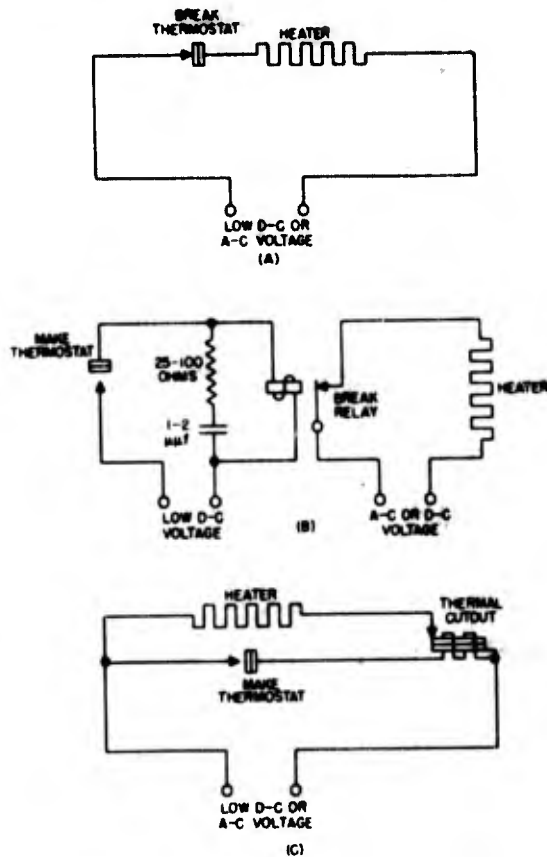
Figure 4-6. Bimetallic thermostat circuits
