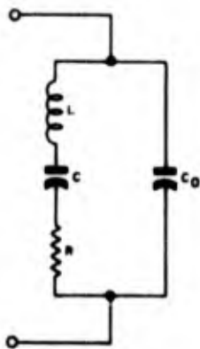
Figure 1-91. Simplified equivalent circuit of crystal unit
