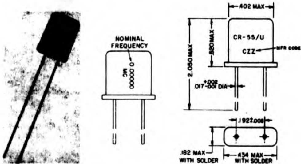
Figure 2-67. Crystal Unit CR-55/U
