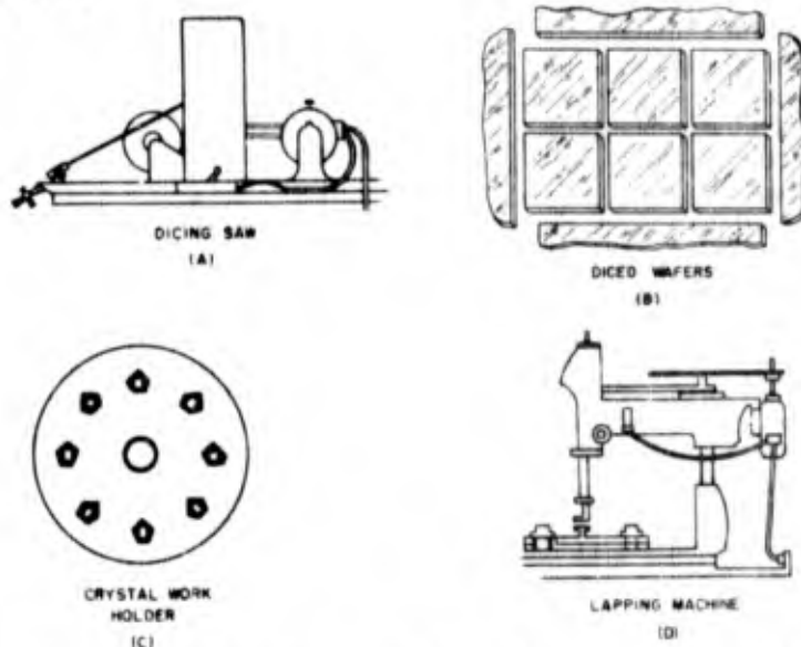
Figure 1-67. (A) Dicing saw. (B) Diced wafer. (C) Nest of lapping machine. (D) Lapping machine
