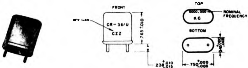
Figure 2-31. Crystal Unit CR-36/U
