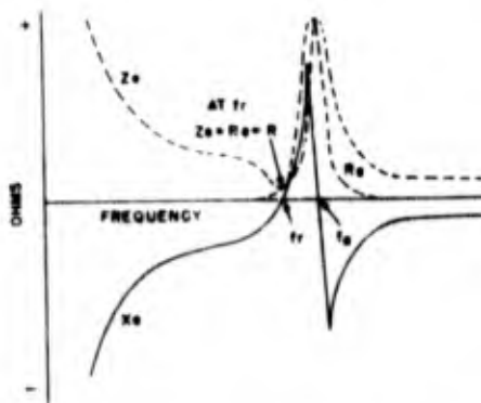
Figure 1-100. Impedance characteristics versus frequency of crystal unit. Neither the frequency nor the impedances are drawn to scale
