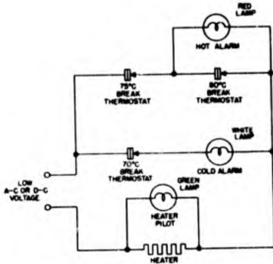
Figure 4-10. Thermostat monitoring and alarm circuit
