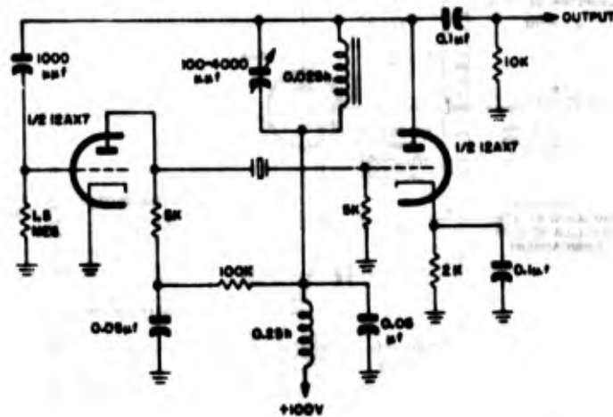
Figure 2-58. Schematic diagram of typical oscillator designed for use with Crystal Unit CR-50/U
