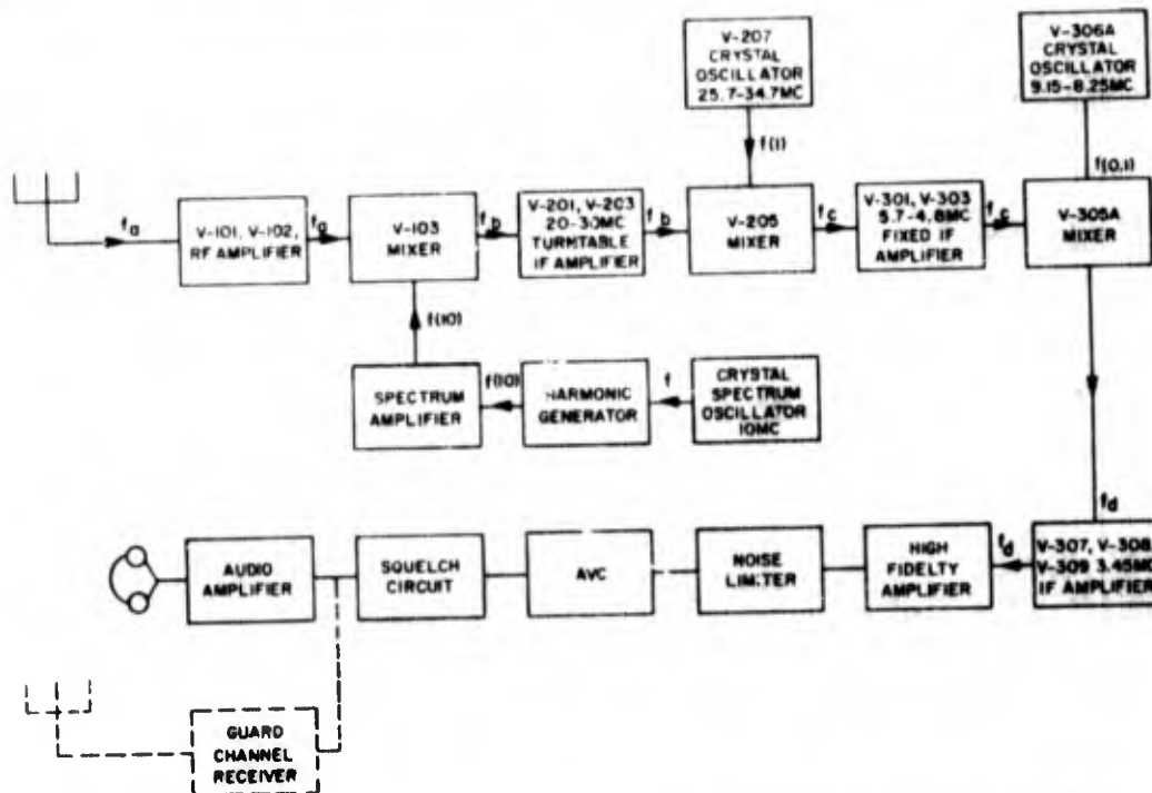
Figure 1-210. Block diagram of main receiver network of Receiver-Transmitter RT-178/ARC-27
