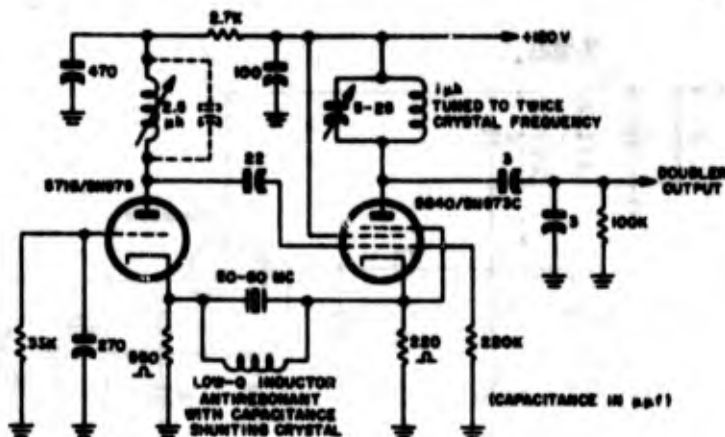
Figure 2-34. Schematic diagram of typical oscillator designed for use with Crystal Unit CR-32/U
