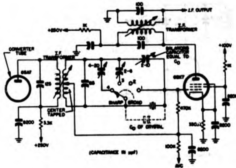
Figure 2-48. Schematic diagram of typical oscillator designed for use with Crystal Unit CR-45/U
