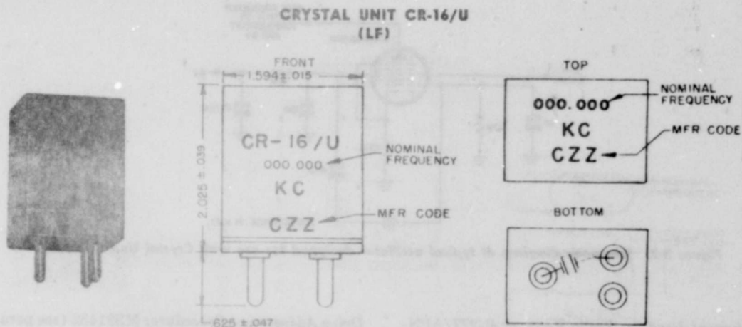
Figure 2-3. Crystal Unit CR-16/U
