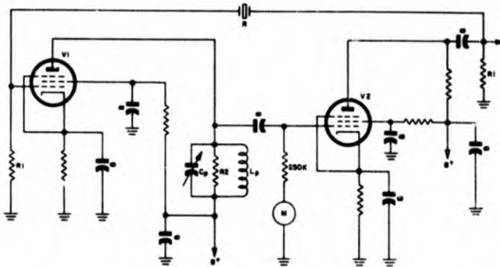
Figure 1-183. Grounded-cathode two-stage feed-back oscillator
