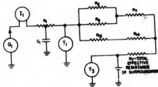
Figure 4-13. Thermal D-C path of crystal power
