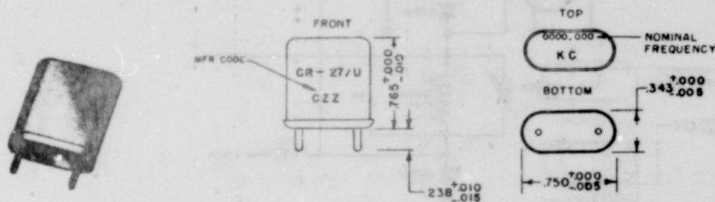
Figure 2-17. Crystal Unit CR-27/U
