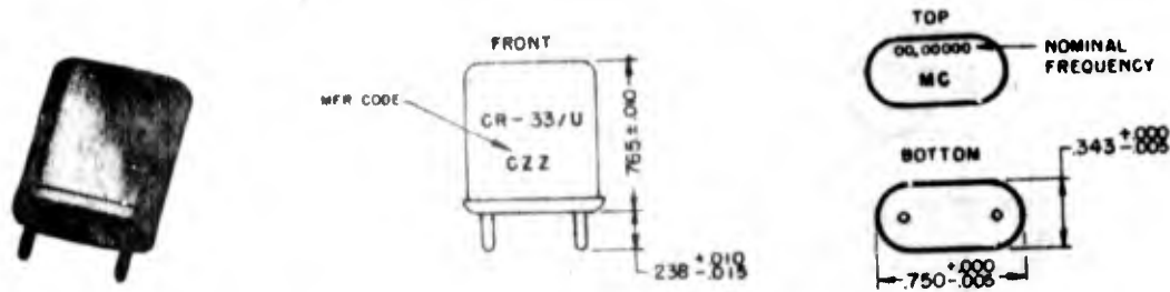
Figure 2-27. Crystal Unit CR-33/U
