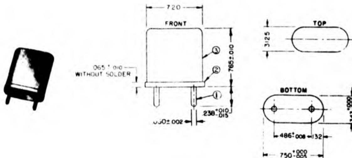
Figure 3-2. Crystal Holder HC-6/U
