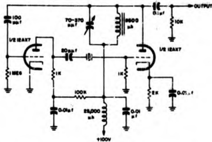
Figure 2-34. Schematic diagram of typical oscillator designed for use with Crystal Unit CR-37/U
