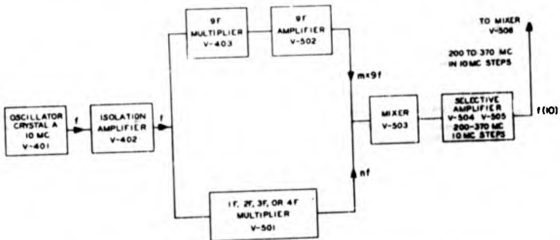
Figure 1-212. Block diagram of spectrum generator system in Radio Set AN/ARC-27
