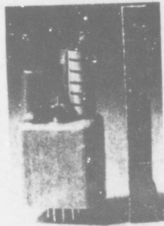
Figure 1-242. Miniature plug-in (standard octal base) Pierce oscillator (0.8 to 16 mc) developed at Armour Research Foundation by H. E. Gruen et al., as an initial basic packaged oscillator unit to be standardized for military use.
