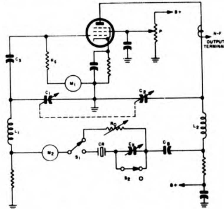
Figure 1-106. Simplified schematic diagram of CI meter
