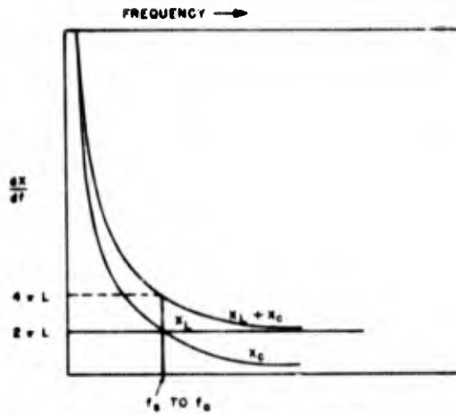
Figure 1-110. Rates of change of reactance of equivalent series-arm parameters, L and C , with frequency
