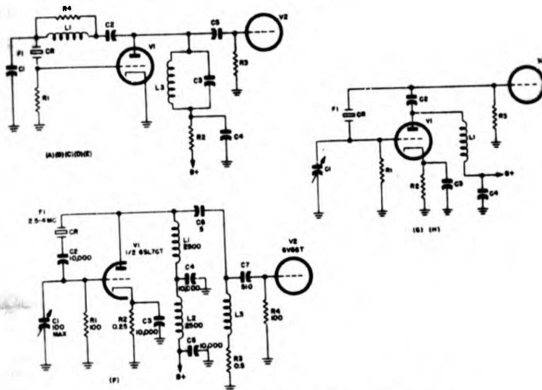
Figure 1-135. Modifications of Pierce oscillator using triodes
