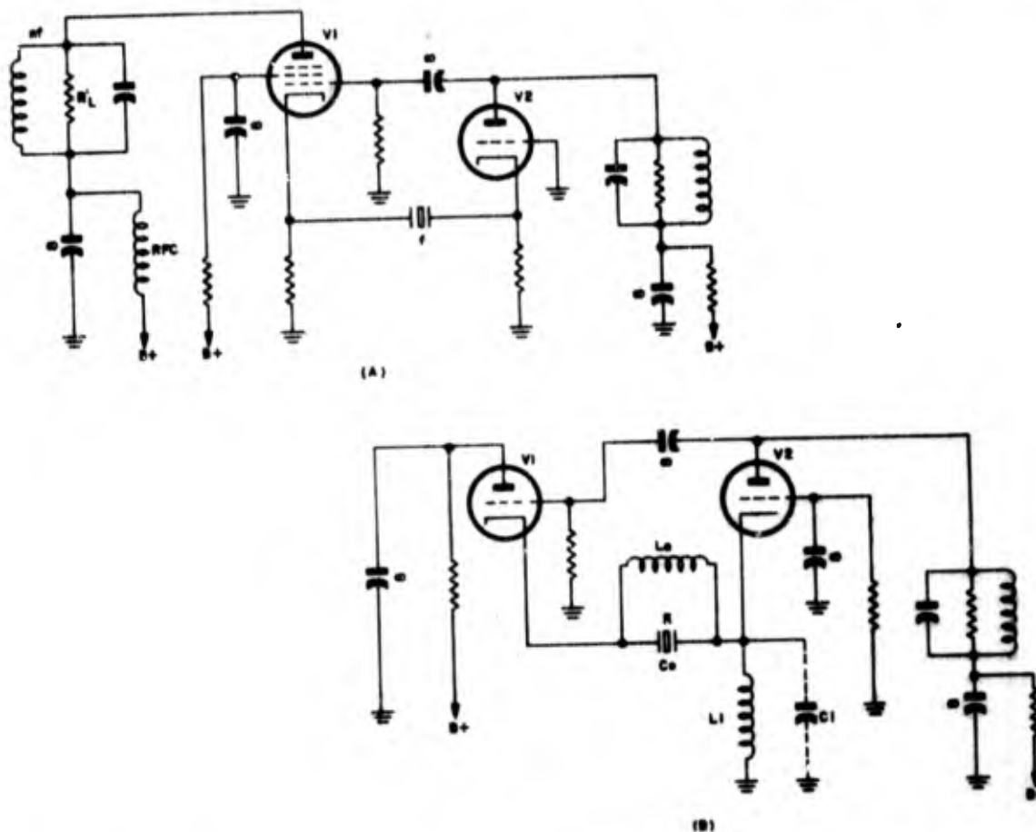
Figure 1-174. (A) Electron-coupled Butler circuit. (B) Butler circuit having common cathode ground return WADC TR 56-156 252
