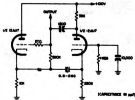
Figure 2-20. Schematic diagram of typical oscillator designed for use with Crystal Unit CR-28/U
