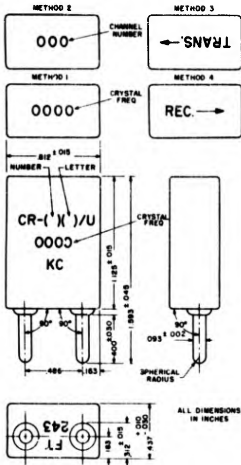
Figure 3-21. Crystal Holder FT-243. The markings indicated are applicable for Crystal Units CR-5B/U, CR-6B/U, CR-7B/U, CR-10B/U, and CR-12A/U. Method 1 is used where the operating frequencies of the using equipment are in terms of frequencies only; or where a single crystal is used to control both a transmitter and a receiver and the channel is expressed in terms of frequency. Method 2 is used where the operating frequencies of the using equipment are designated in terms of channel numbers and frequencies; or where a single crystal is used to control both a transmitter and a receiver and the operating frequency is expressed as a channel number as well as a frequency. Methods 3 and 4 are used respectively where two separate crystal units are employed in a single equipment, each performing a different function, such as one being used for transmitting and the other for receiving. Method 4 is used where the crystal unit is used to control the local oscillator of a receiver. On the back of the receiver crystal holder is marked "RECEIVE ON 0000 KC," where 0000 is the receiver frequency, which is always to be 455 kc below the crystal frequency. For an exploded view of the FT-243 holder, as a part of Crystal Unit CR-8B/U, see figure 1-70.
