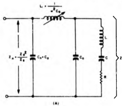
Figure 1-182. Impedance-inverting oscillator circuits. (A) Basic impedance-inverting network
