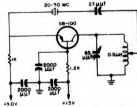
Figure 1-227. High-frequency transistor oscillator
