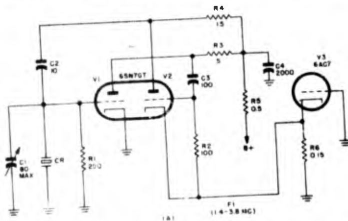
Figure 1-155. Two-stage parallel-resonant oscillators of the multivibrator type.
