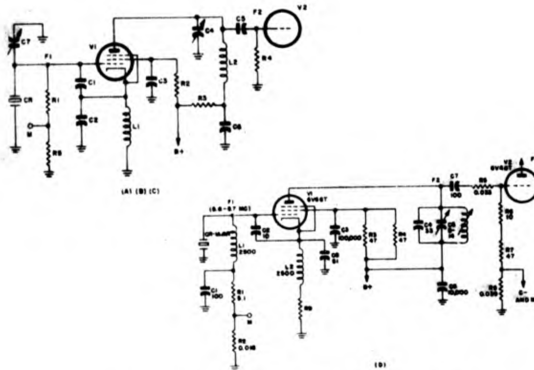
Figure 1-137. Electron-coupled Pierce oscillator modifications. All circuits except circuit (A) provide frequency multiplication
