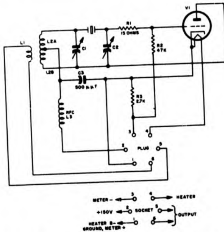
Figure 1-168. A plug-in capacitance-bridge oscillator which is practical for 50-150-mc frequency range
