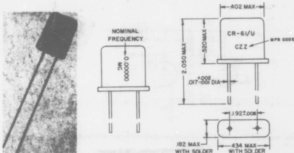
Figure 2-79. Crystal Unit CR-61/U
