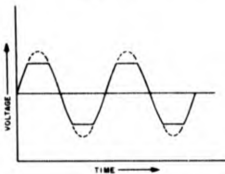
Figure 1-241. Voltage waveform after clipping of both peaks by diode rectifiers
