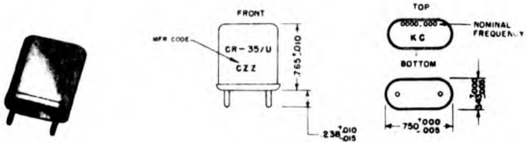
Figure 2-29. Crystal Unit CR-35/U
