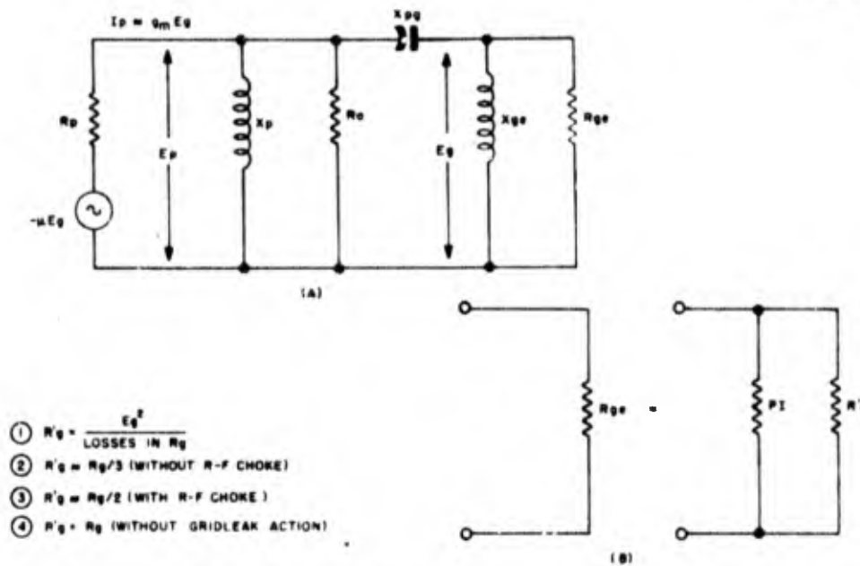
Figure 1-141. Equivalent circuit of Miller oscillator. R_p is assumed to be large compared with the total load impedance. R_o is an equivalent resistance accounting for the output losses. R_{gg} is an equivalent resistance accounting for the crystal and grid losses; it is approximately equal to the resistance of the parallel circuit shown in (B). PI is the performance index of the crystal unit; R'_g is the equivalent grid resistance; and R_g is the actual gridleak resistance
