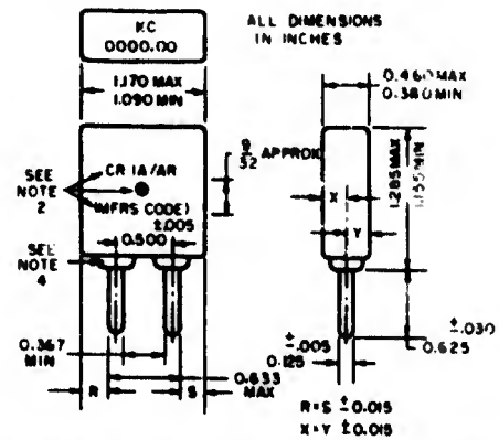
Figure 3-23. Crystal Holder for Crystal Unit CR-1A/AR
