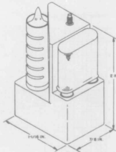
Figure 1-249. Miniature plug-in (standard octal base) cathode-coupled Butler oscillator (10 to 75 mc) developed at Armour Research Foundation by H. E. Gruen et al., as an initial basic packaged oscillator unit to be standardized for military use
