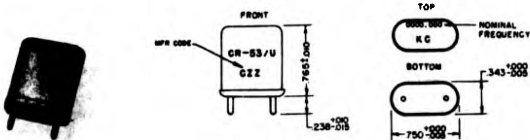
Figure 2-63. Crystal Unit CR-53/U
