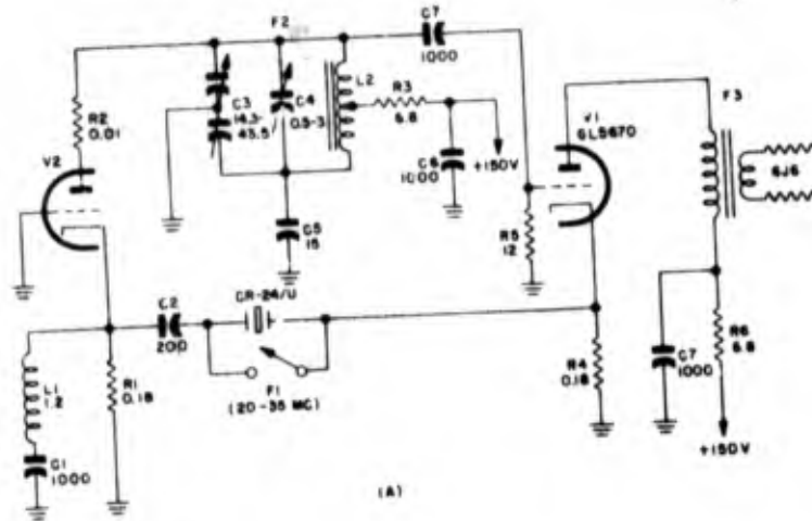
Figure 1-175. Modifications of Butler oscillator. Dotted lines in circuit (G) indicate stray capacitances
