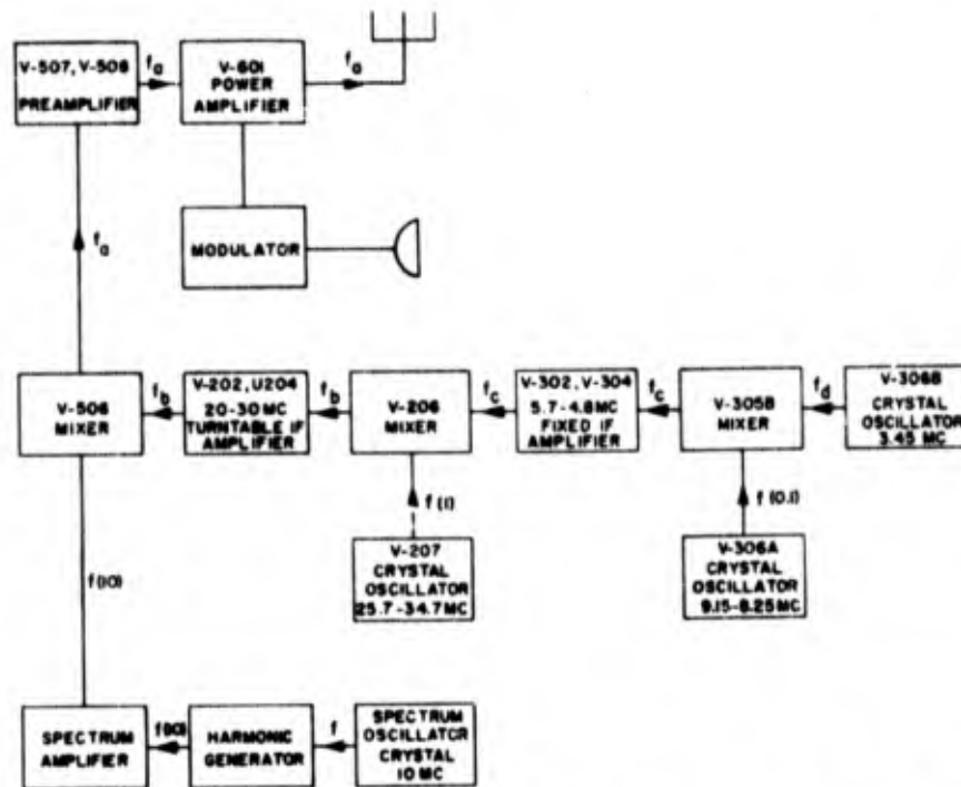
Figure 1-211. Block diagram of transmitter network of Receiver-Transmitter RT-178/ARC-27
