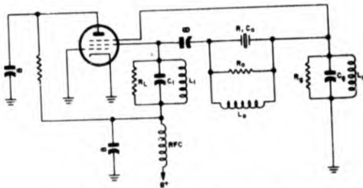
Figure 1-181. Transitron crystal oscillator
