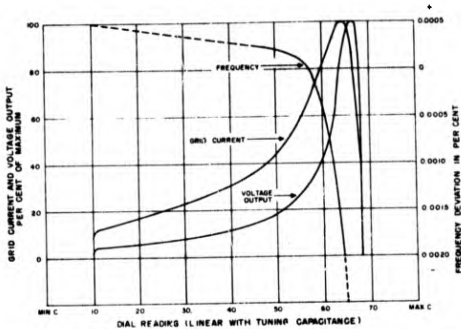
Figure 1-166. Typical performance curves of capacitance-bridge oscillator, showing effects of change in bridge tuning capacitance on voltage output, activity (d-c grid current), and frequency
