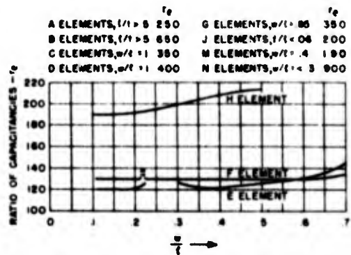
Figure 1-95. Approximate values of the ratio of capacitances, r = \frac{C_0}{C} , for various plated crystal elements
