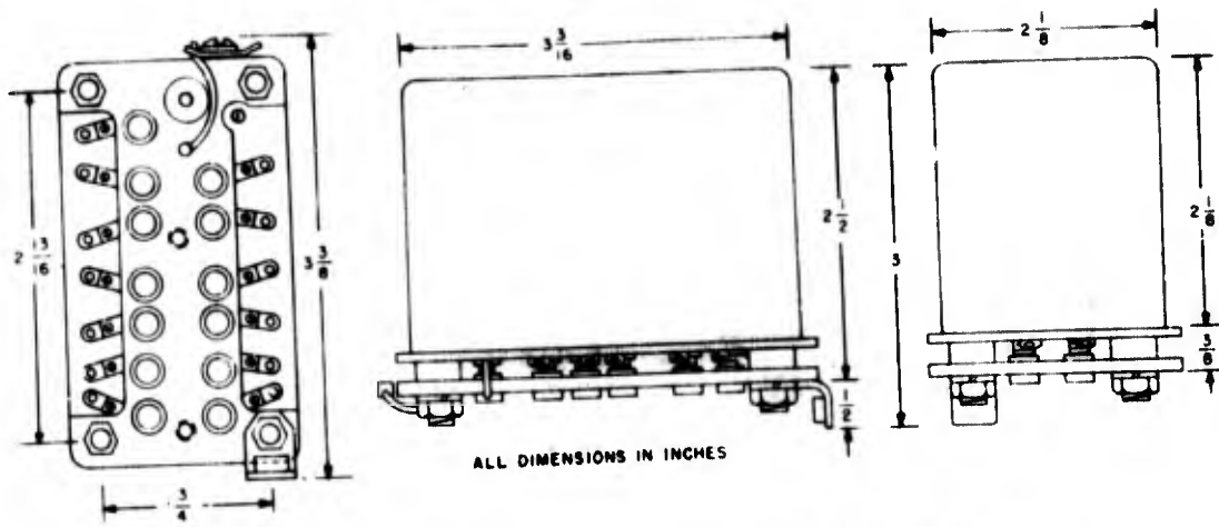
Figure 4-23. Dimensions of Bendix Radio Crystal Oven N205651
