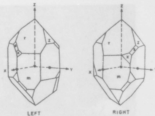
Figure 1-4. Left and right quartz crystals
