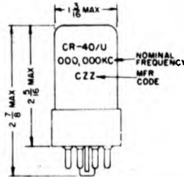
Figure 2-39. Crystal Unit CR-40/U
