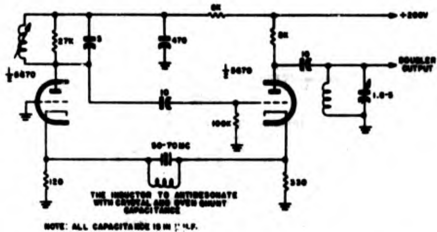
Figure 2-76. Schematic diagram of typical oscillator designed for use with Crystal Unit CR-39/U
