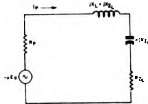
Figure 1-123. Coil inserted in plate circuit of Pierce oscillator to prevent phase of I_p from being influenced by changes in R_p .
