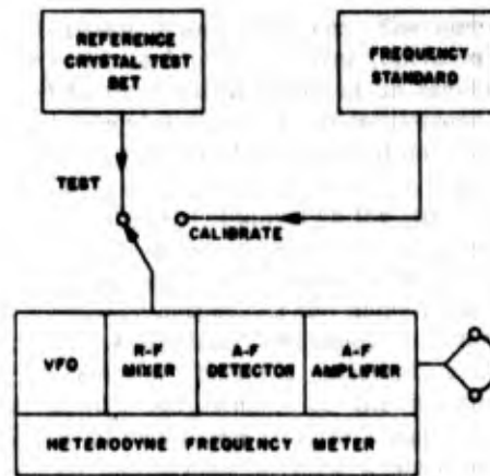
Figure 2-88. System for measuring crystal frequencies accurately with heterodyne frequency meter
