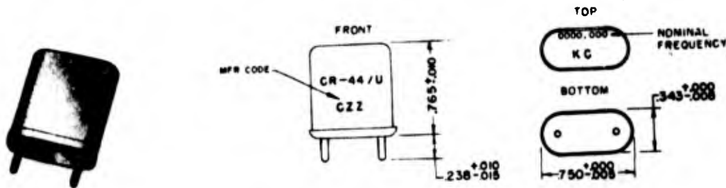
Figure 2-45. Crystal Unit CR-44/U
