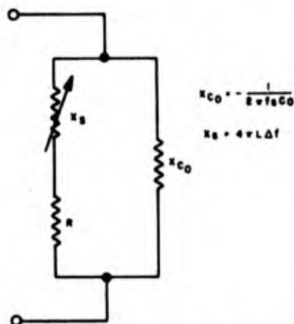
Figure 1-97. Impedance diagram of equivalent circuit of crystal unit
