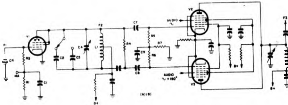
Figure 1-153 Miscellaneous Miller-oscillator modifications
