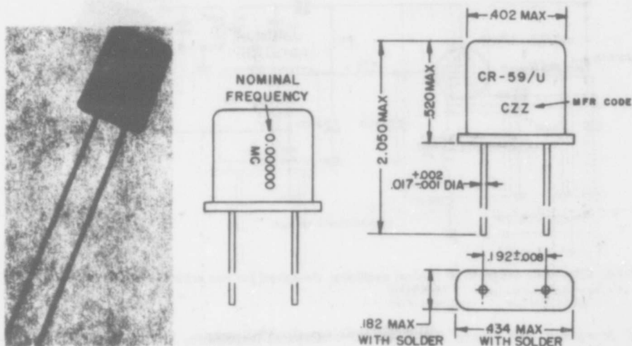
Figure 2-75. Crystal Unit CR-59/U
