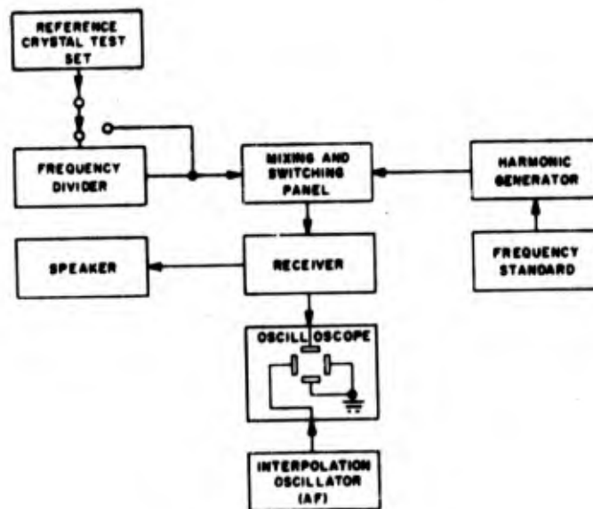
Figure 2-92. System recommended for Government inspection measurements of crystal frequencies at room temperature. The measurements are made visually with the oscilloscope and interpolation oscillator. The speaker is used principally as an aid in determining whether the crystal frequency under test is greater or less than the standard harmonic
