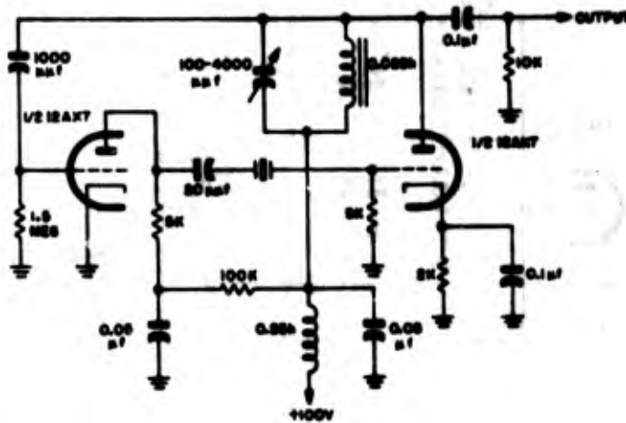
Figure 2-36. Schematic diagram of typical oscillator designed for use with Crystal Unit CR-38/U
