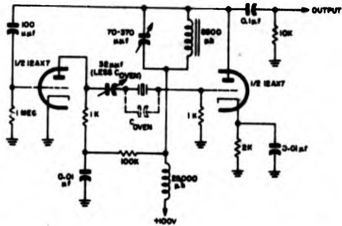
Figure 2-42. Schematic diagram of typical oscillator designed for use with Crystal Unit CR-42/U
