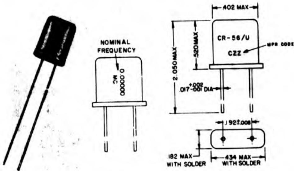
Figure 2-69. Crystal Unit CR-56/U
