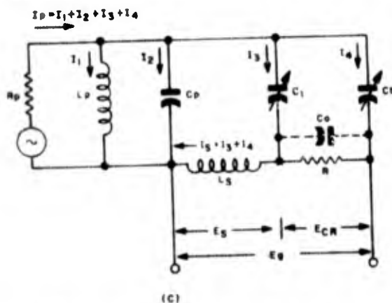
Figure 1-165. (C) Simplified equivalent circuit
