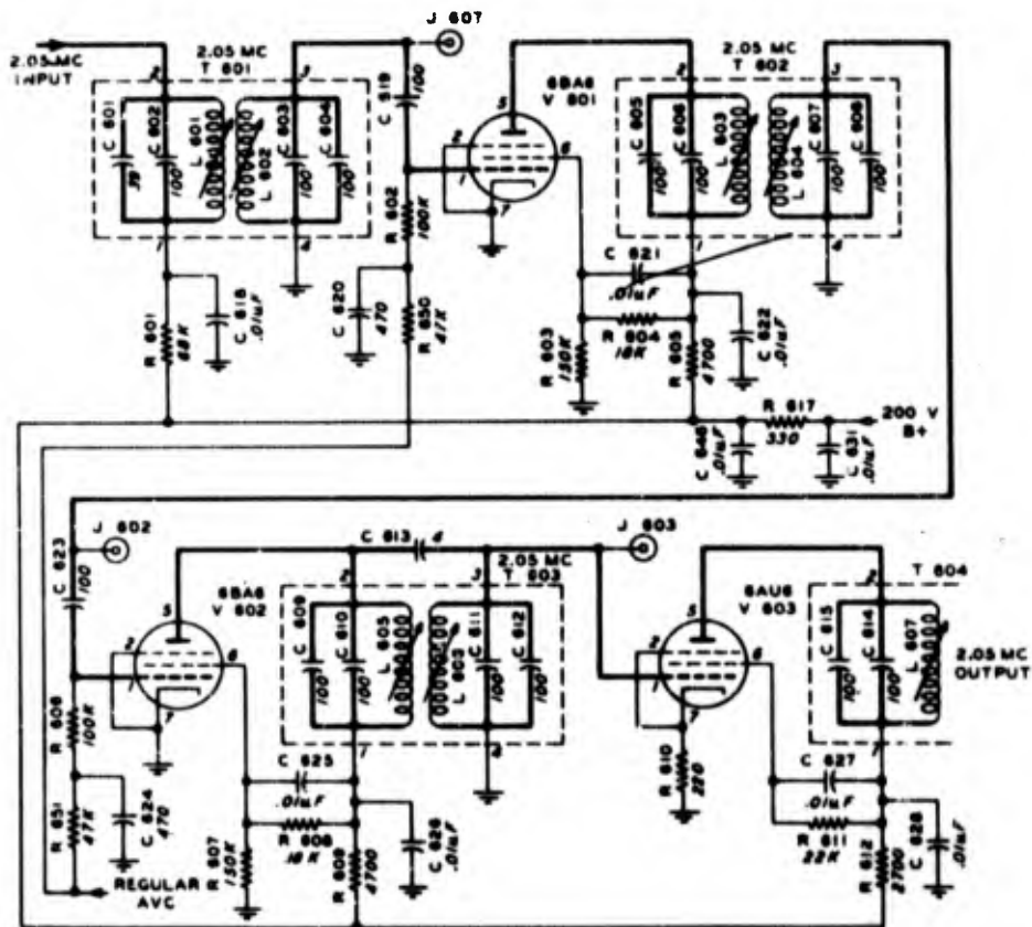
Figure 1-209. Third i-f amplifier in Radio Receiver R-270/GR. Schematic diagram
