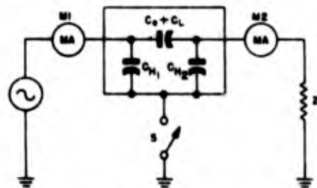
Figure 1-93. Circuit diagram indicating the effect that grounding a metal holder may have on shunt capacitance
