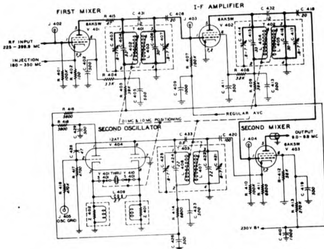
Figure 1-207. First i-f amplifier unit in Radio Receiver R-27B/GR. Schematic diagram
