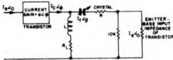
Figure 1-225. Simplified equivalent circuit of junction transistor crystal-feedback oscillator, showing tuned tank in collector circuit for obtaining desired current amplification and loop phase shift for feedback to emitter input. For stable oscillations to be maintained
