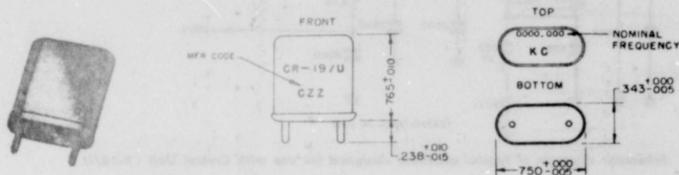
Figure 2-7. Crystal Unit CR-19/U
