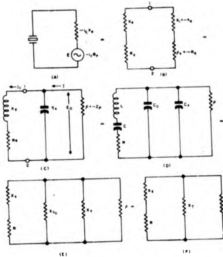
Figure 1-108. Generalized crystal oscillator circuit
