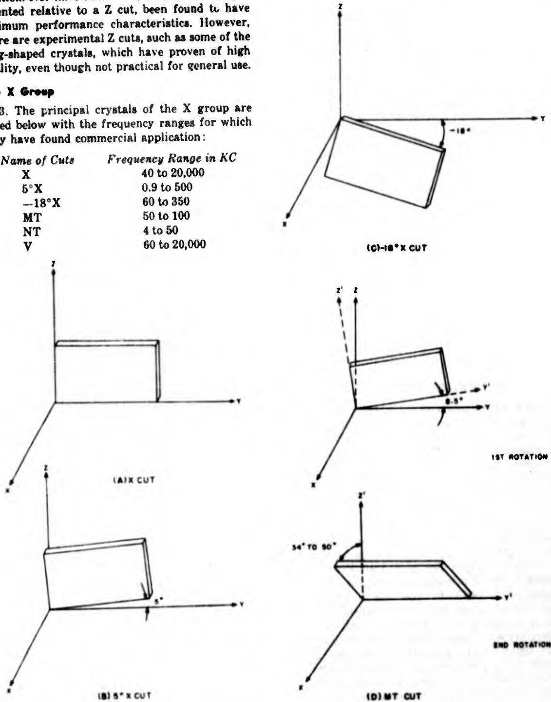
Figure 1-19. The X group. (The second rotations of the MT, NT, and V cuts are shown only for the positive angles) *
