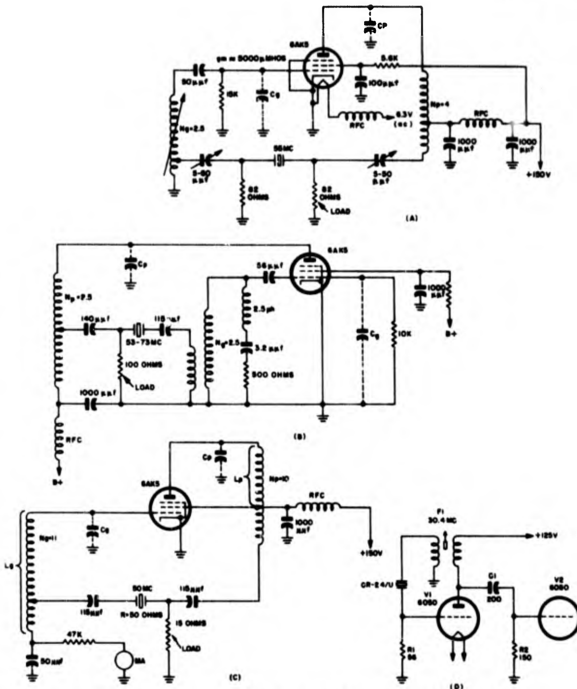
Figure 1-177. Modifications of transformer-coupled oscillator for: (A) High stability. (B) Untuned broad band. (C) Large output. (D) Slug-tuned, narrow band
