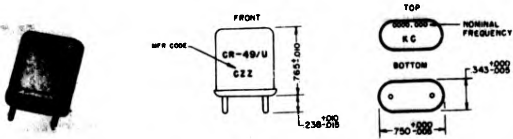
Figure 2-55. Crystal Unit CR-49/U
