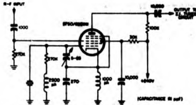
Figure 2-54. Schematic diagram of typical oscillator designed for use with Crystal Unit CB-49/U
