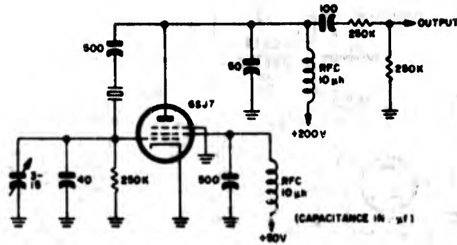
Figure 2-46. Schematic diagram of typical exciter designed for use with Crystal Unit CR-44/U
