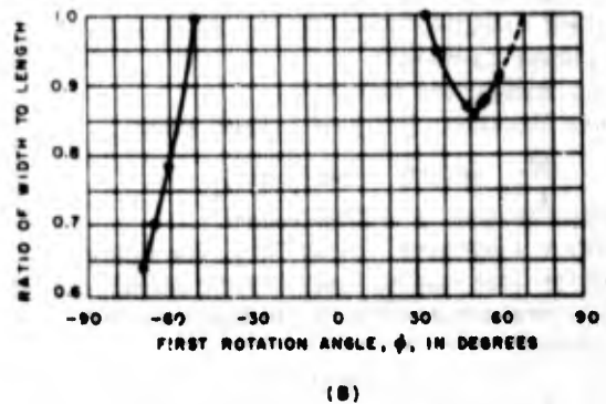
Figure 1-56. (A) Diagram illustrating the equivalence between a face-shear mode and the length- and width-extensional modes of a rectangular plate which has been cut diagonally with respect to the face-shear element. (B) w/l ratio vs rotation angle, \phi , of element G providing zero temperature coefficient *
