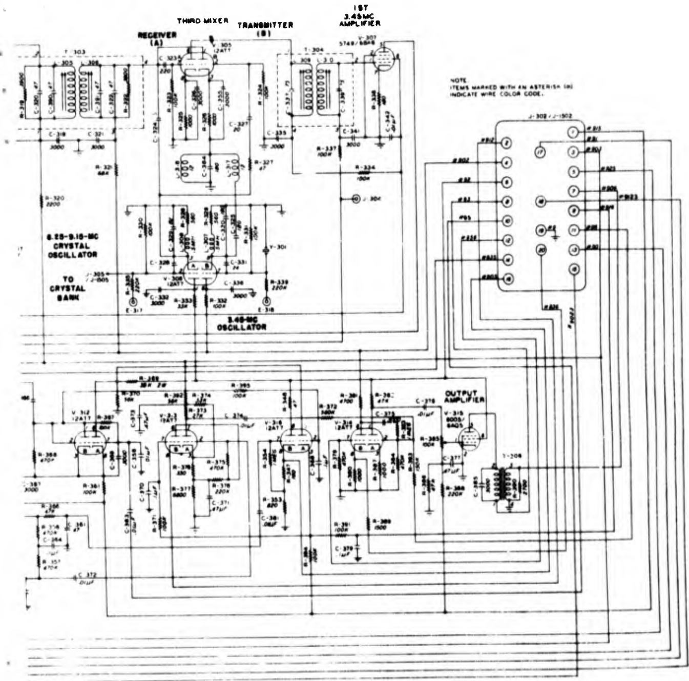
Figure 1-217. Fixed-i-f amplifier subassembly, Receiver-Transmitter RT-178/ARC-27. See figure 1-210 for function of receiver circuits V301, V303, V305A, V306A, and V307. (V308 and V309, the 2nd and 3rd 3.45-mc amplifiers, which are similar in design to the V307 stage, are not shown. Also omitted are the vacuum-tube heater circuits.) See figure 1-211 for function of transmitter circuits V302, V304, V305B, V306A, and V306B
