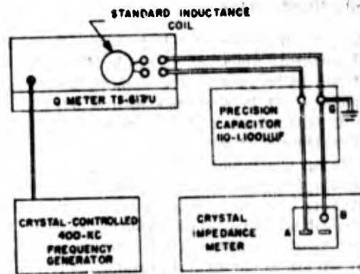
Figure 2-95. Constant parallel-capacitance method for calibration of load capacitance dial
