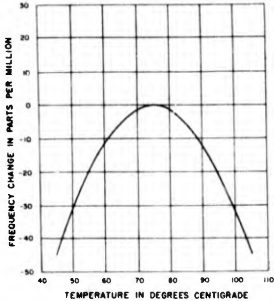
Figure 1-54. Temperature-frequency characteristics of FT-cut plate vibrating in combination mode *
