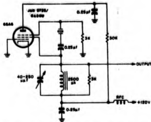
Figure 2-14. Schematic diagram of typical oscillator designed for use with Crystal Unit CR-25/U
