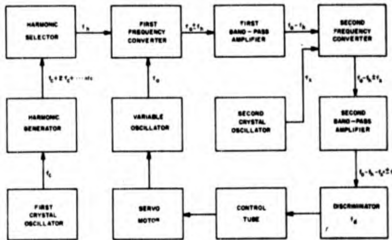
Figure 1-191. Block diagram of frequency-synthesizer circuit
