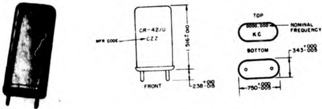
Figure 2-41. Crystal Unit CR-42/U
