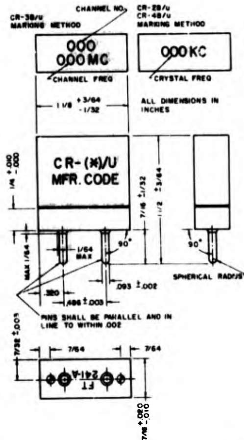
Figure 3-20. Crystal Holder FT-241-A. The markings indicated are applicable for Crystal Units CR-2B/U, CR-3B/U and CR-4B/U
