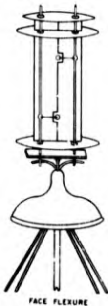
Figure 1-86. Cage assembly for solder-cone wire mounting of low-frequency length-width flexure crystal *
