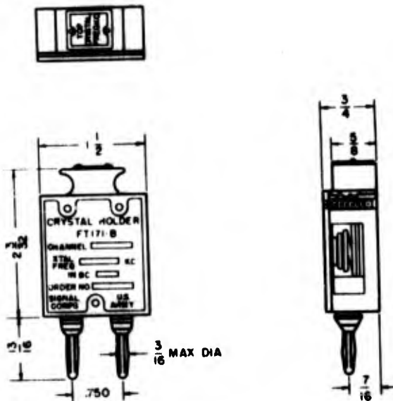
Figure 3-19. Crystal Holder FT-171-B
