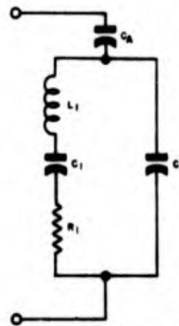
Figure 1-92. Simplified equivalent circuit of air-gap crystal unit
