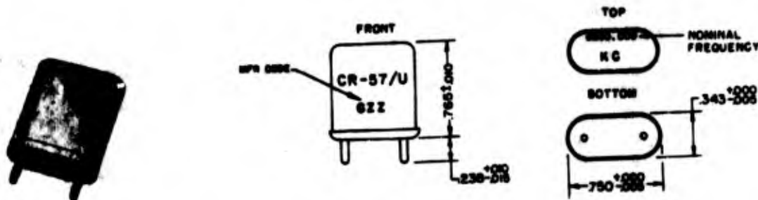
Figure 2-71. Crystal Unit CR-57/U
