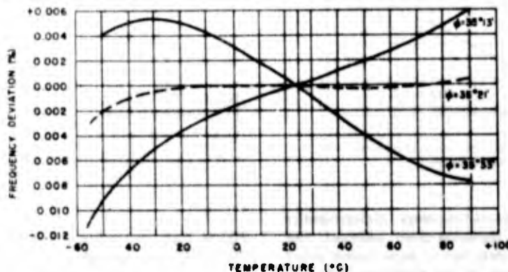
Figure 1-49. Temperature-frequency characteristics of element A
