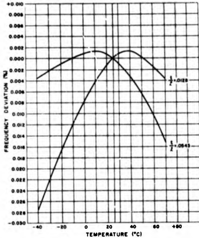
Figure 1-31. Percentage frequency deviation for J elements. The smaller t/l ratio is representative of a 1.2-kc element, and the larger t/l ratio is representative of a 10-kc element
