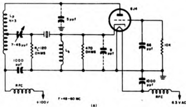
Figure 1-179. Modifications of grounded-grid oscillator. (A) Narrow-band circuit
