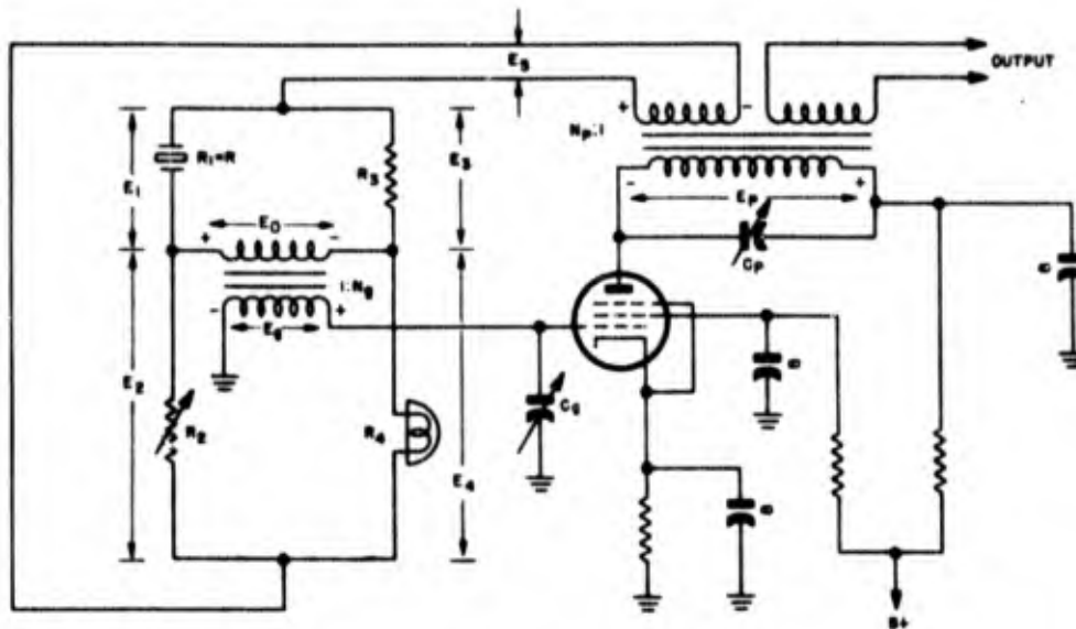
Figure 1-160. Basic circuit of Meacham bridge-stabilized oscillator
