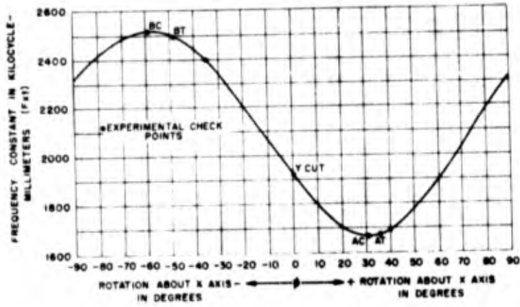
Figure 1-43. Frequency constant versus angle of rotation about X axis for thickness-shear elements of Y group. (Values shown for Y, BT, and BC cuts are smaller than the average) *
