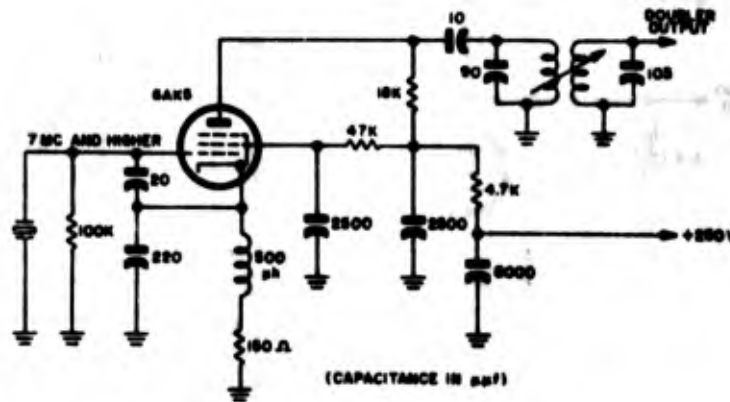
Figure 2-74. Schematic diagram of typical ocmeter designed for use with Crystal Unit CR-58/U
