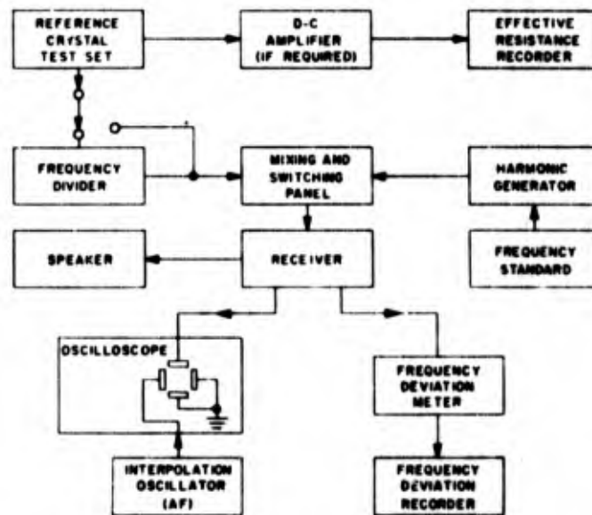
Figure 2-93. System recommended for Government inspection measurements of crystal frequencies over the operating temperature range. The instantaneous frequency-measuring system is the same as that shown in Figure 2-80 for room temperature measurements. Added are the frequency-deviation recorder circuit and the effective-resistance recorder circuit
