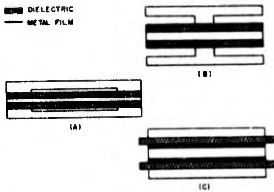
Figure 1-78. (A) Air-gap mounting using dielectric sheets having conducting films on each major surface. (B) Air-gap mounting using dielectric sheets having a conducting film on major surface in contact with electrode. (C) Dielectric sandwich in which leaves of metal foil are inserted between dielectric and crystal
