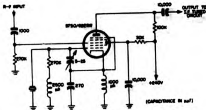
Figure 2-54. Schematic diagram of typical oscillator designed for use with Crystal Unit CR-48/U
