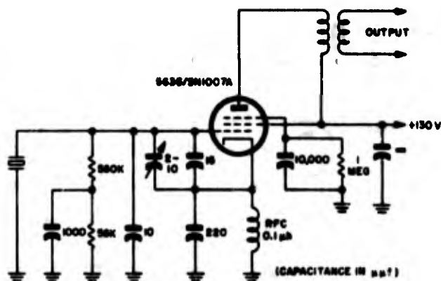
Figure 2-32. Schematic diagram of typical oscillator designed for use with Crystal Unit CR-36/U
