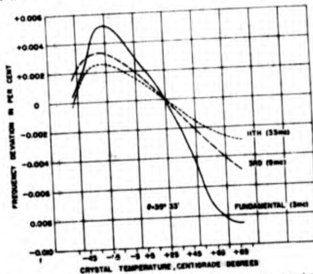
Figure 1-112. Typical variations in frequency-temperature characteristics of A element when operated at different harmonics
