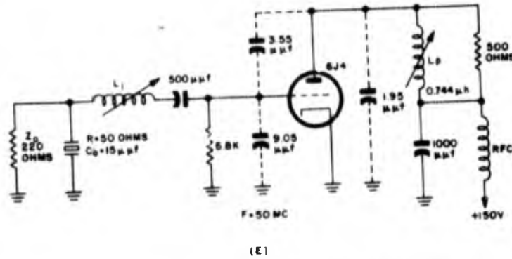
Figure 1-182. Impedance-inverting oscillator circuits. (E) Impedance-inverting Miller oscillator
