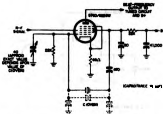
Figure 2-22. Schematic diagram of typical oscillator designed for use with Crystal Unit CR-29/U
