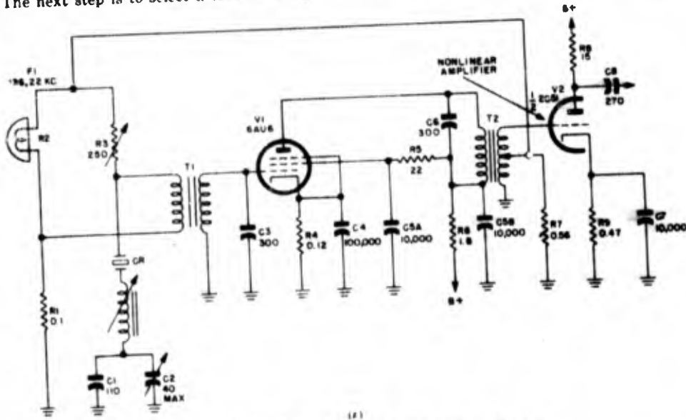
Figure 1-163. Meacham bridge-stabilized oscillators
