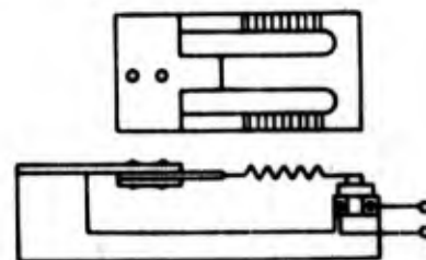
Figure 4-5. E-shaped, bimetallic, snap thermostat
