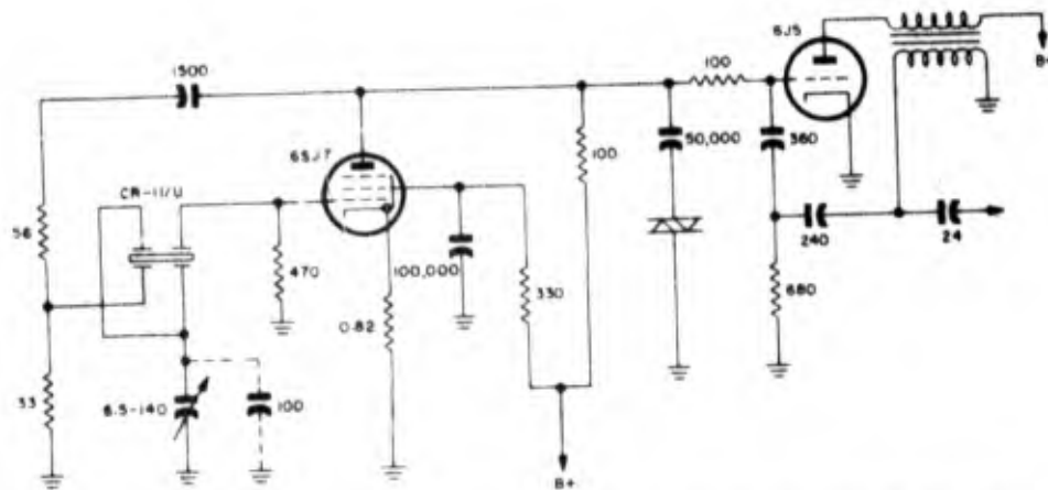
Figure 1-158. Duplex-electrode crystal circuit in Test Set TS-251/UP for synchronizing blocking oscillator at 1818.18 cps. Resistance is given in kilohms, capacitance in micromicrofarads
