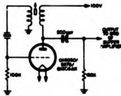
Figure 2-80. Schematic diagram of typical oscillator designed for use with Crystal Unit CR-61/U
