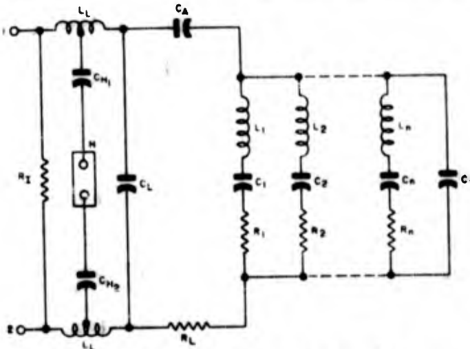
Figure 1-90. Equivalent circuit of crystal unit
