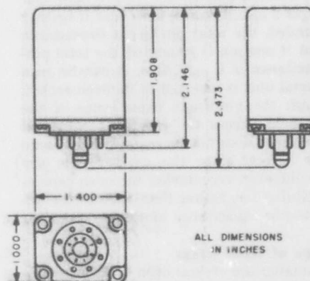
Figure 4-20. Dimensions of Crystal Oven HD-54/U
