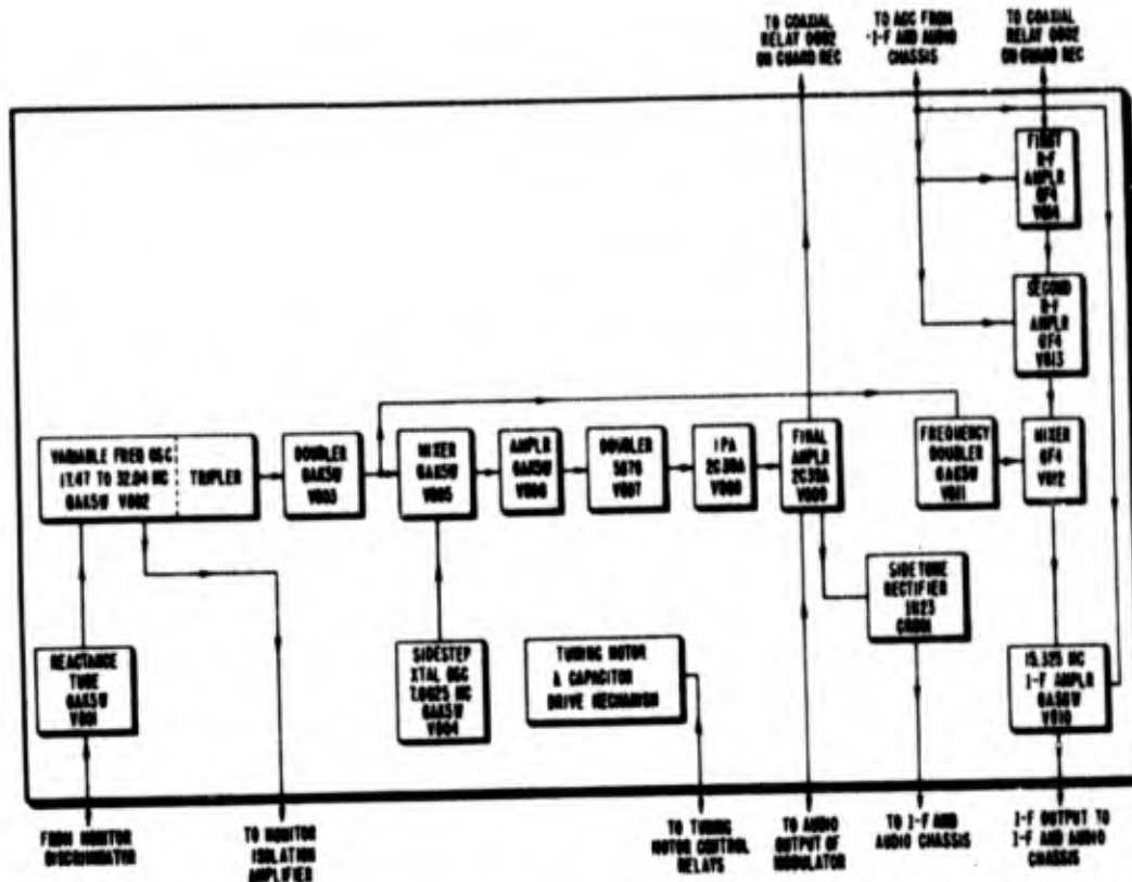
Figure 1-198. R-f head. Block diagram of main channel transmitter and receiver r-f circuits in Radio Set AN/ARC-33
