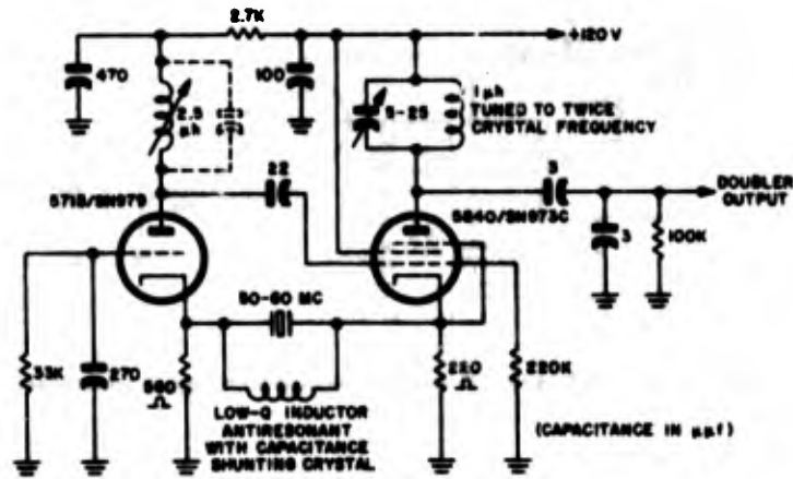
Figure 2-70. Schematic diagram of typical oscillator designed for use with Crystal Unit CR-56/U
