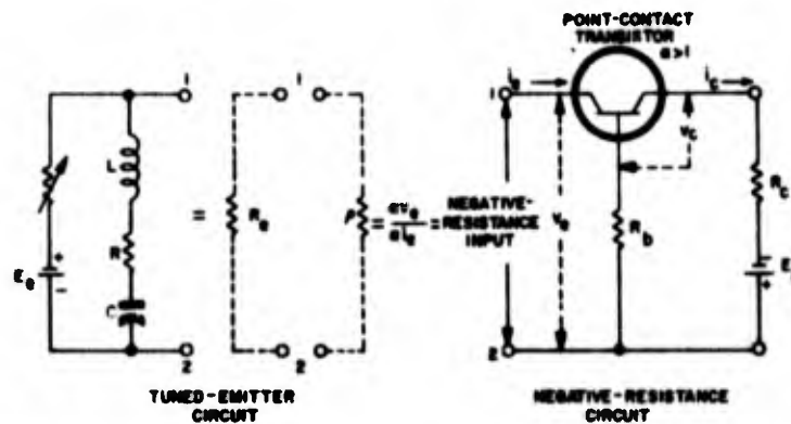
Figure 1-228. Tuned-emitter negative-resistance circuit. Essential features are that alpha be greater than unity, the insertion of an external resistance, R_b , in the common-base circuit to increase the collector-to-emitter energy feedback; and for oscillations to build up, the effective positive resistance, R_e , of the tuned-emitter circuit must be less, numerically, than the negative resistance, at the emitter input
