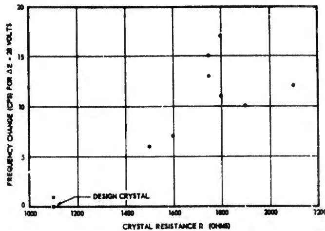
Figure 1-239. Frequency deviation of circuit shown in figure 1-238 for a given change in supply voltage at various values of crystal resistance
