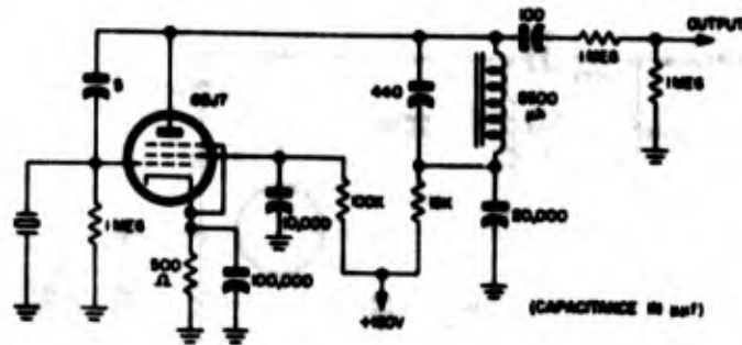
Figure 2-44. Schematic diagram of typical oscillator designed for use with Crystal Unit CR-43/U
