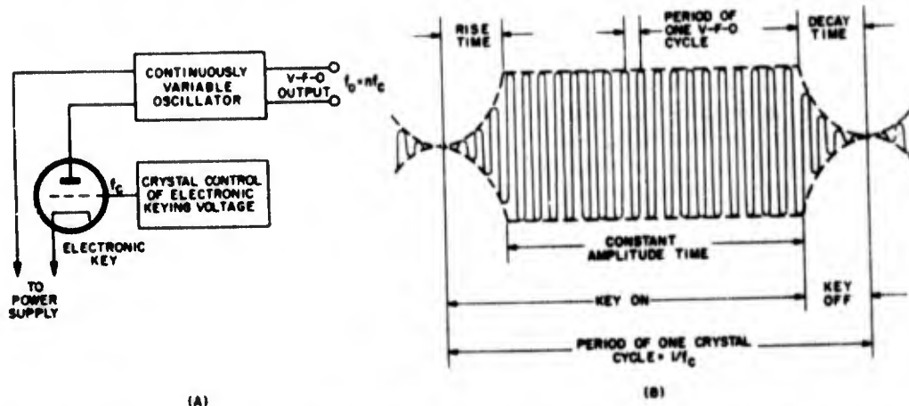
Figure 1-219. Simplified block diagram (A) and output waveform (B) of crystal-phase-controlled harmonic multiplier
