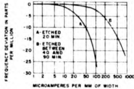
Figure 1-117. Frequency deviation versus crystal current density for two GT-cut crystals which were subjected to different periods of etching*
