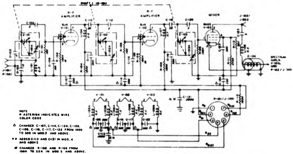
Figure 1-213. Main receiver r-f amplifier subassembly, Receiver-Transmitter RT-178/ARC-27. Includes receiver circuits V101, V102, and V103 (r-f amplifier and 1st mixer stages). See figure 1-210 for relation of the above stages to the rest of the receiver frequency-control system
