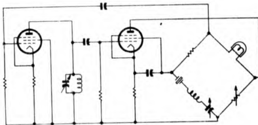
Figure 1-164. Two-stage Meacham bridge-stabilized oscillator
