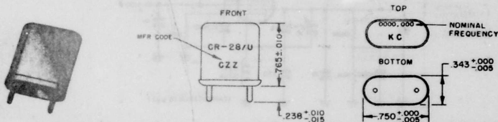
Figure 2-19. Crystal Unit CR-28/U
