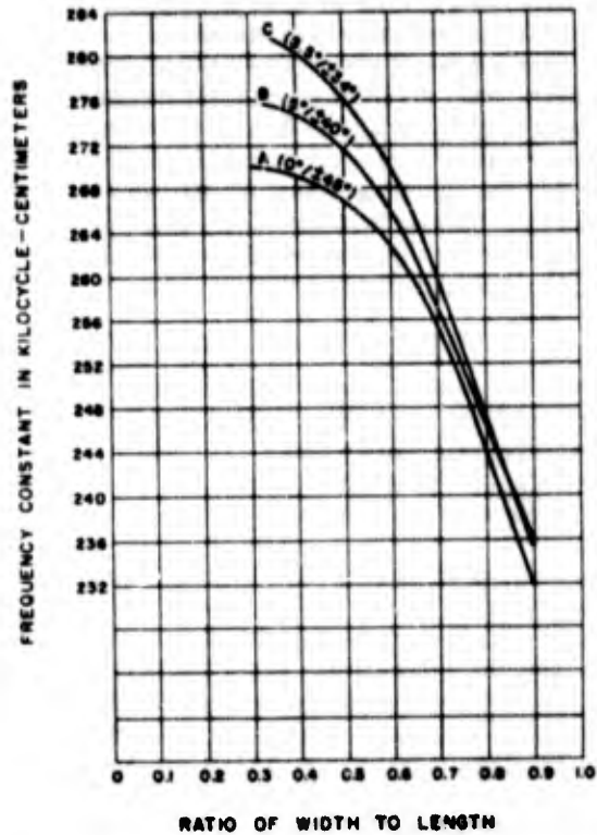
Figure 1-33. Frequency constant versus w/l ratio for M elements having low temperature coefficients. C is the curve of the most commonly used MT orientation*
