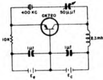
Figure 1-224. Junction transistor crystal-feedback oscillator
