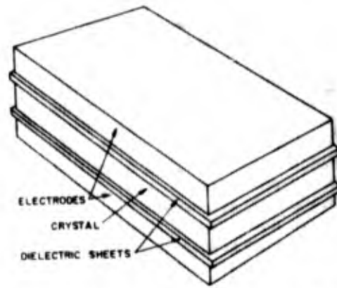
Figure 1-73. Pressure type of dielectric sandwich for mounting crystals
