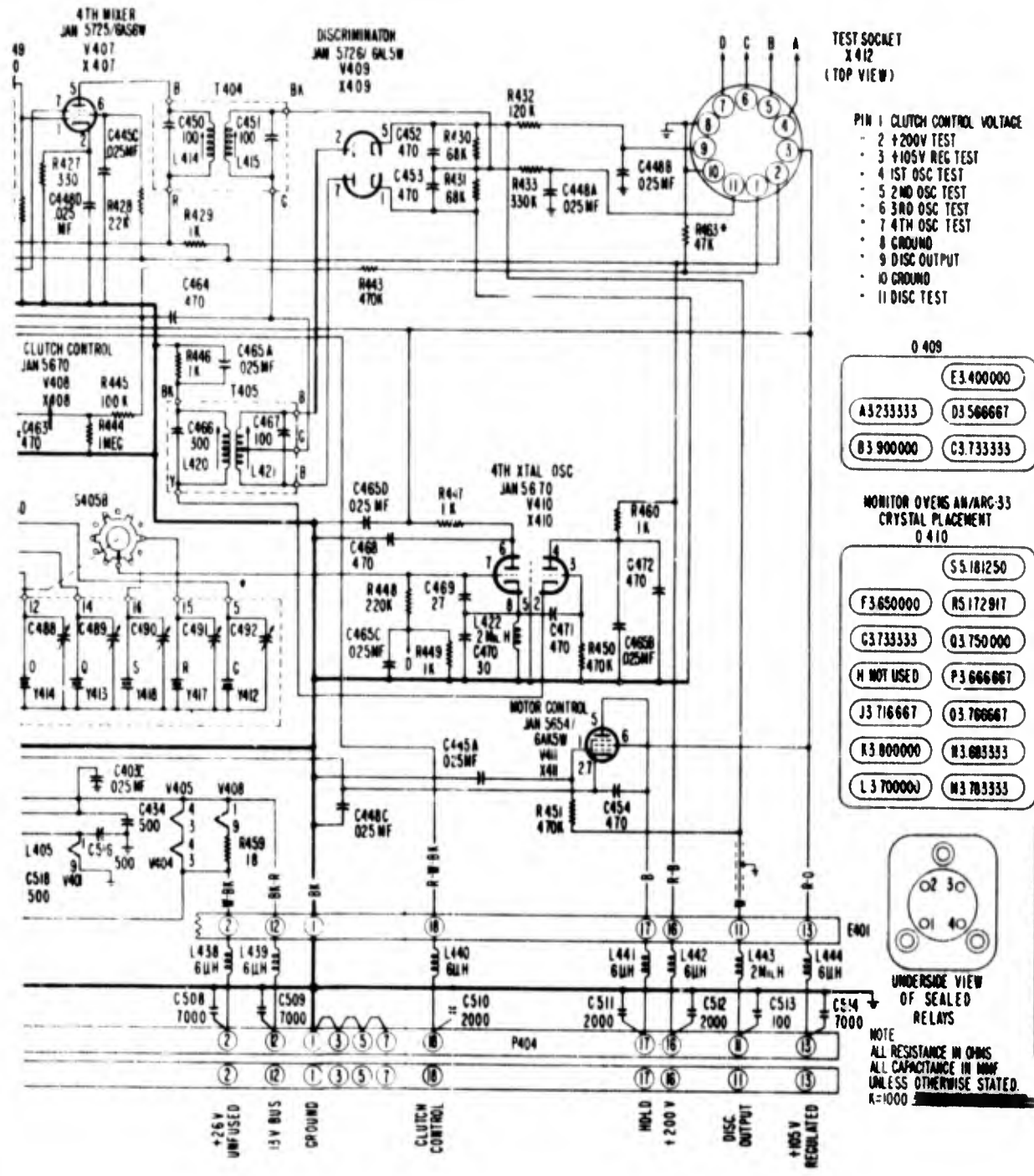
Figure 1-196. Monitor chassis. Schematic diagram of a-f-c system in Radio Set AN/ARC-33
