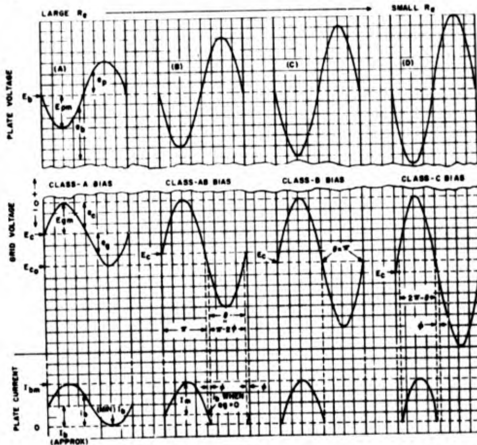
Figure 1-132. Change of state of Pierce oscillator with a C_p/C_s ratio of one, under no-load conditions when E_c is held constant and the effective resistance of the crystal changes
