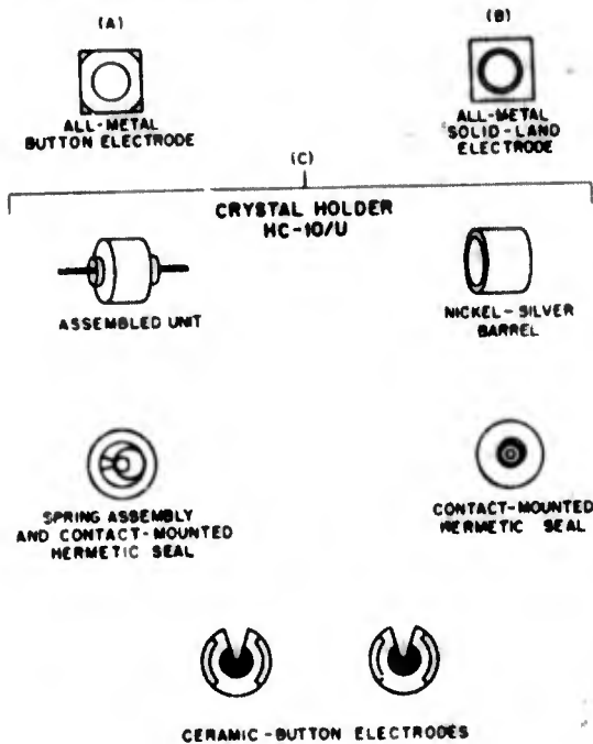
Figure 1-79. Button electrodes and methods of mounting
