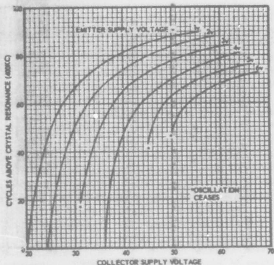
Figure 1-235. Deviation of frequency with the collector supply voltage for various values of emitter supply voltage. Test oscillator circuit is the same as that shown in figure 1-224
