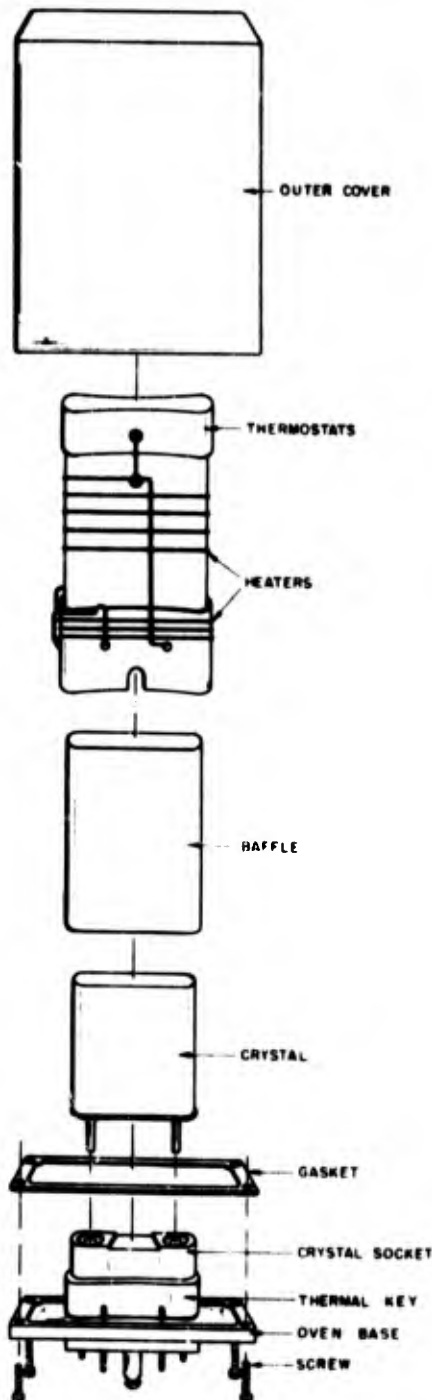
Figure 4-2. Small crystal oven equivalent to Military Type HD-54/U
