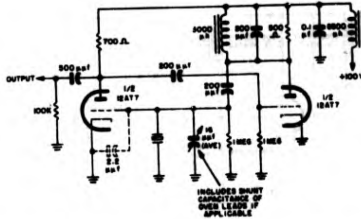
Figure 2-50. Schematic diagram of typical oscillator designed for use with Crystal Unit CR-45/U
