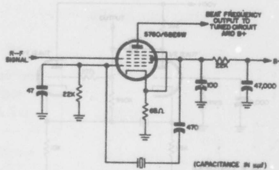
Figure 2-2. Schematic diagram of typical oscillator designed for use with Crystal Unit CR-15/U
