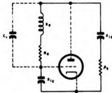
(B) PLATE-TO-GRID CRYSTAL CONNECTION
