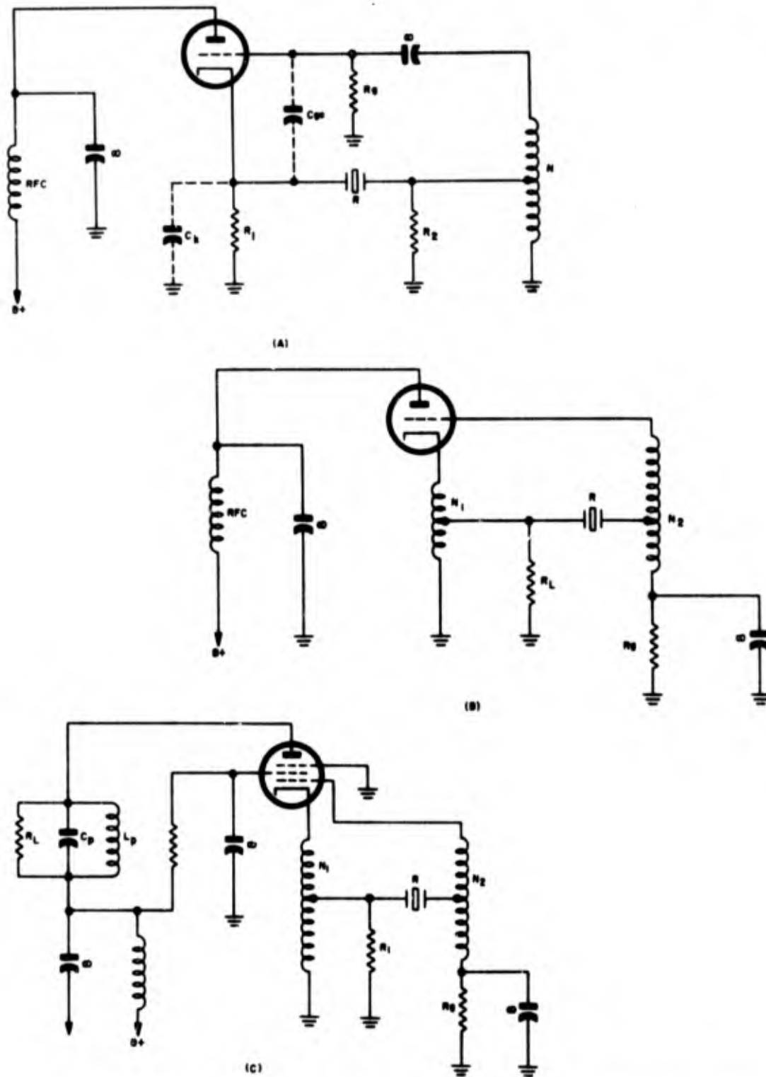
Figure 1-100. Grounded-plate oscillators. (A) Basic circuit. (B) Circuit for increased power output. (C) Electron-coupled circuit
