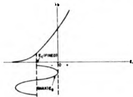
Figure 1-127. Point on E_c, I_p curve at which stable oscillations can be achieved with fixed bias. For minimum grid losses, the peak of the maximum excitation voltage must not exceed the fixed E_c .
