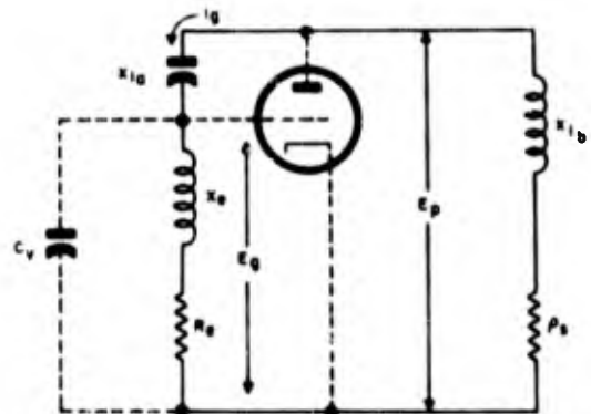
(A) GRID-TO-CATHODE CRYSTAL CONNECTION
