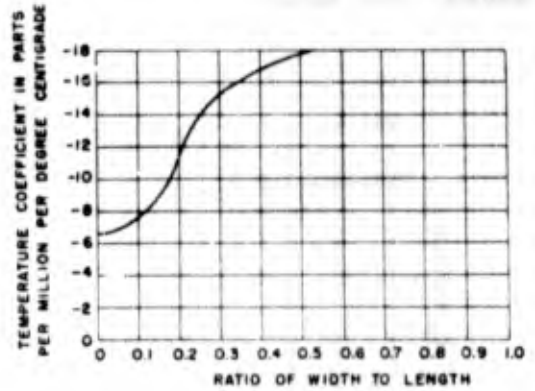
Figure 1-28. Temperature coefficient versus w/l ratio for element H*
