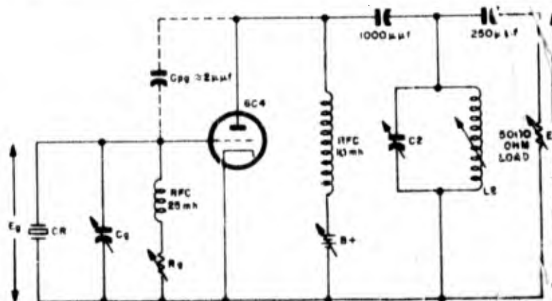
Figure 1-143. Experimental Miller oscillator whose characteristic curves are plotted in figures 1-144 to 1-148
