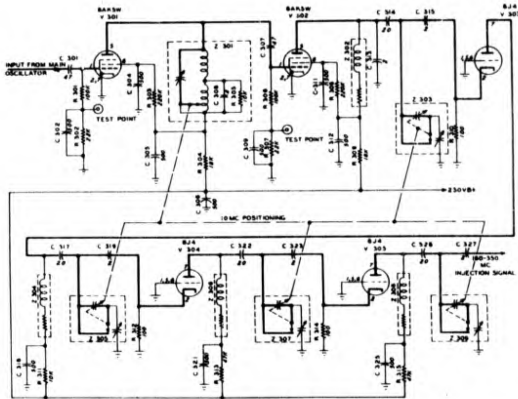
Figure 1-206. Multiplier-amplifier unit of 1st injection system in Radio Receiver R-278/GR. Schematic diagram
