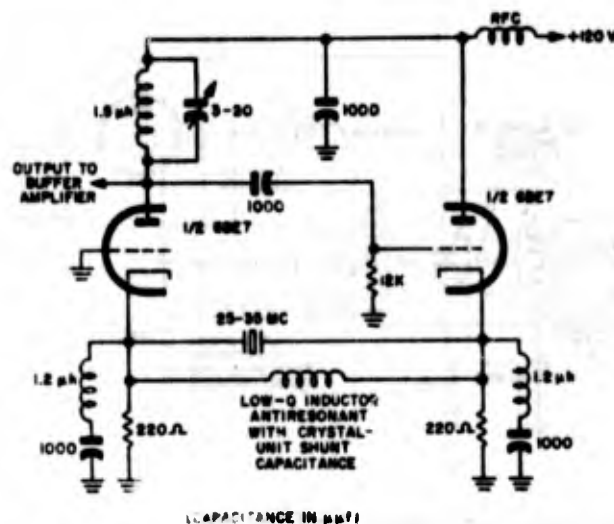
Figure 2-10. Schematic diagram of typical oscillator designed for use with Crystal Unit CR-23/U
