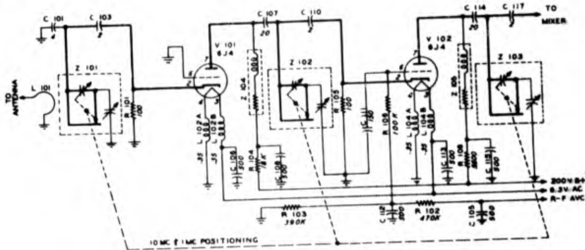
Figure 1-203. Radio-frequency amplifier unit of Radio Receiver R-278/GR. Schematic diagram
