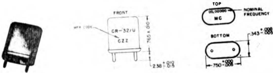
Figure 2-25. Crystal Unit CR-32/U
