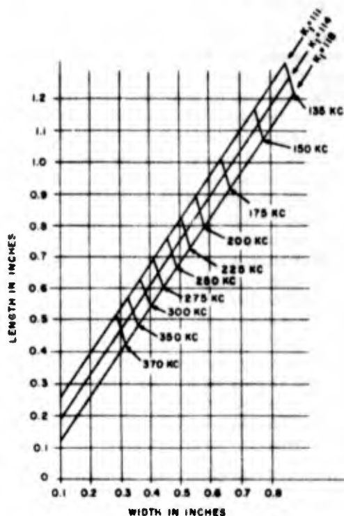
Figure 1-22. Frequency characteristics of X-cut crystal vibrating in width-extensional mode, where the width is parallel to the Y axis. w/l ratios not included between the two outer curves will have interfering modes. K_1 is in kc-inches
