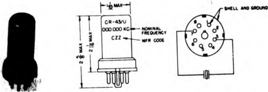
Figure 2-43. Crystal Unit CR-43/U
