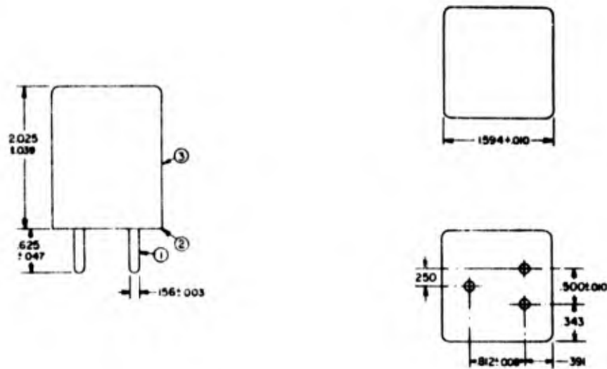
Figure 3-10. Crystal Holder HC-21/U
