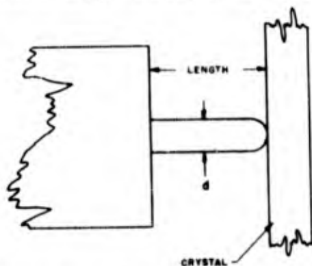
Figure 1-81. Cantilever clamp for providing a resonant-pin support for the crystal *
