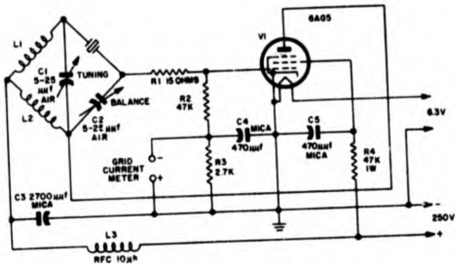
Figure 1-167. A single-tube capacitance-bridge oscillator which is practical for operation in the 50-90-mc frequency range. Resistors not otherwise specified are 1/2 w. L-1 and L-2 are a single center-tapped coil of suitable inductance
