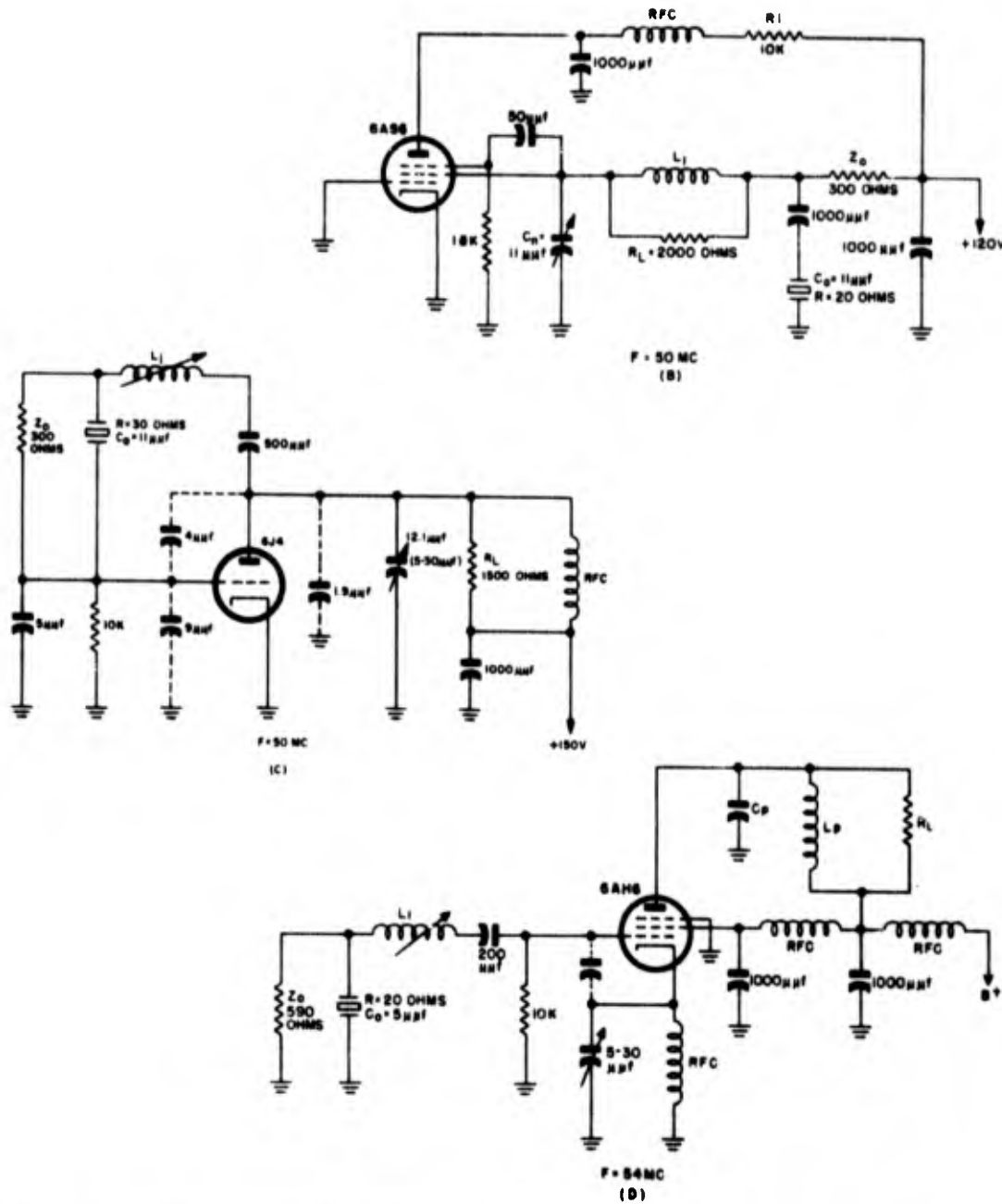
Figure 1-182. Impedance-inverting oscillator circuits. (B) Impedance-inverting transitron oscillator. (C) Impedance-inverting Pierce oscillator. (D) Impedance-inverting electron-coupled Pierce oscillator
