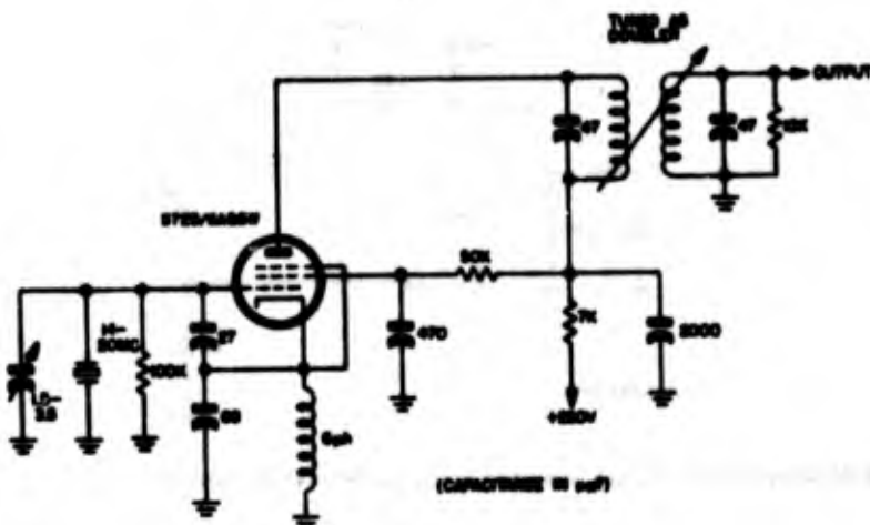
Figure 2-28. Schematic diagram of typical oscillator designed for use with Crystal Unit CR-33/U
