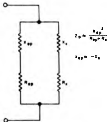
Figure 1-101. Equivalent parallel-resonant circuit of crystal unit ( X_{sp} , R_{sp} ) shunted by load ( X_p , R_p ). Normally f < f_p < f_a , so that X_{sp} is inductive and X_p is capacitive
