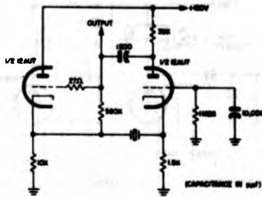
Figure 2-24. Schematic diagram of typical oscillator designed for use with Crystal Unit CR-30/U
