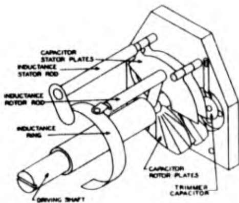
Figure 1-204. Construction of r-f tuner employed in Radio Receiver R-278/GR
