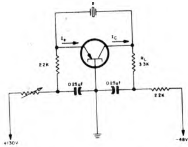
Figure 1-222. Basic circuit for crystal-controlled transistor oscillator
