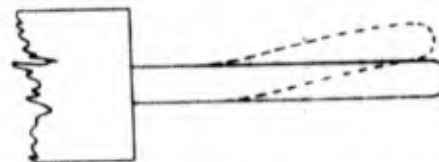
Figure 1-82. Resonant motion of cantilever pin when its length is equal to one-quarter wave-length of clamp-free flexural vibration. Note that the effective free end of the pin is that end supporting the crystal (not shown) *
