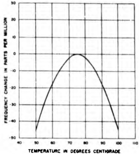
Figure 1-53. Temperature-frequency characteristics of ET-cut plate vibrating in combination mode *
