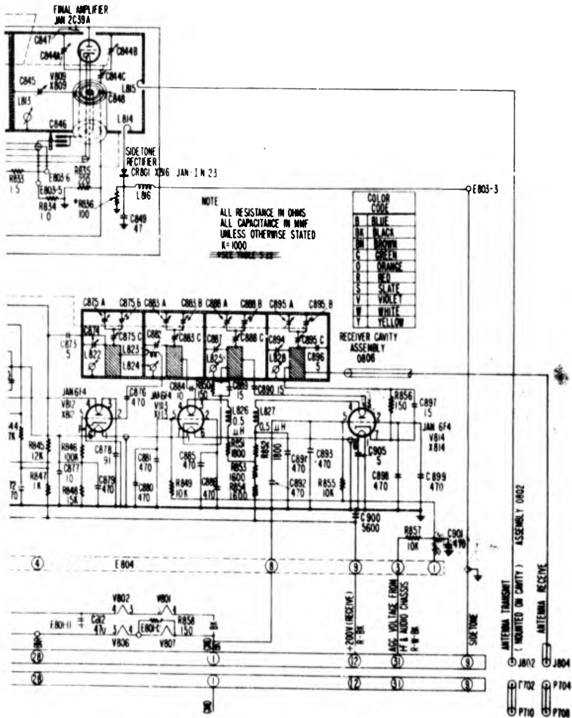
Figure 1-199. R-f head. Schematic diagram of main channel transmitter and receiver r-f circuits in Radio Set AN/ARC-33
