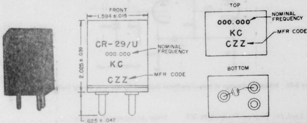
Figure 2-21. Crystal Unit CR-29/U
