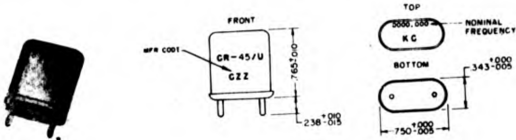
Figure 2-47. Crystal Unit CR-45/U
