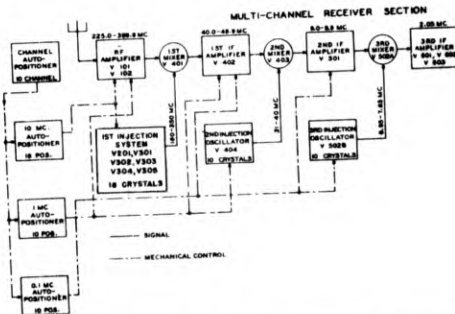
Figure 1-202. Block diagram and frequency chart of Collins frequency-control system as employed in Radio Receiver R-278/GR
