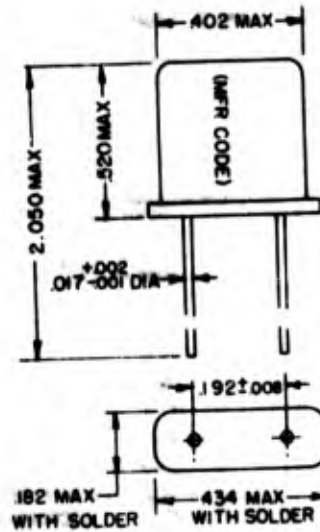
Figure 3-9. Crystal Holder HC-18/U
