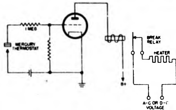
Figure 4-8. Heater control circuit using mercury thermostat
