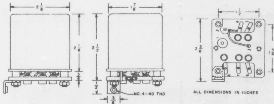
Figure 4-21. Dimensions of Bendix Radio Crystal Oven L205628
