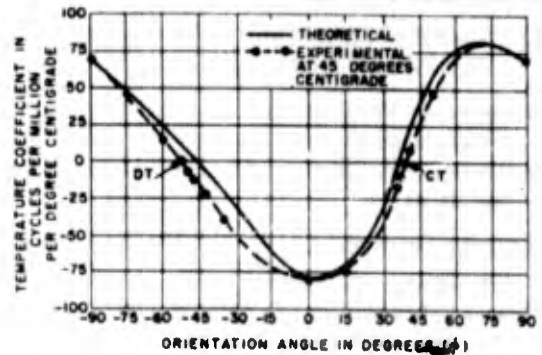
Figure 1-46. Temperature coefficient versus angle of rotation about X axis for face-shear elements of the Y group
