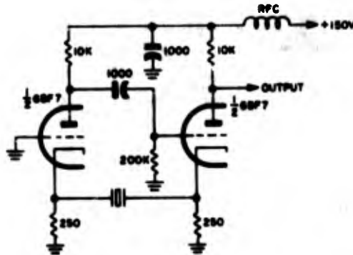
Figure 2-78. Schematic diagram of typical oscillator designed for use with Crystal Unit CR-60/U
