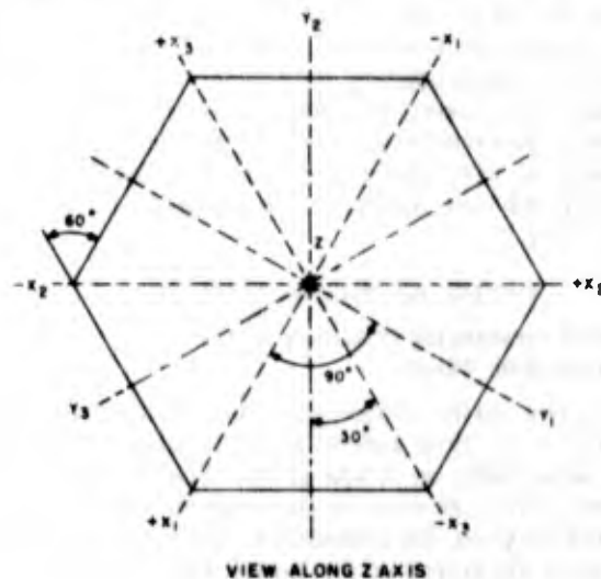
Figure 1-6. XY plane of quartz showing three sets of rectangular axes: X_1, Y_1, Z_1 , X_2, Y_2, Z_2 , X_3, Y_3, Z_3 (Z axis is perpendicular to plane of paper)
