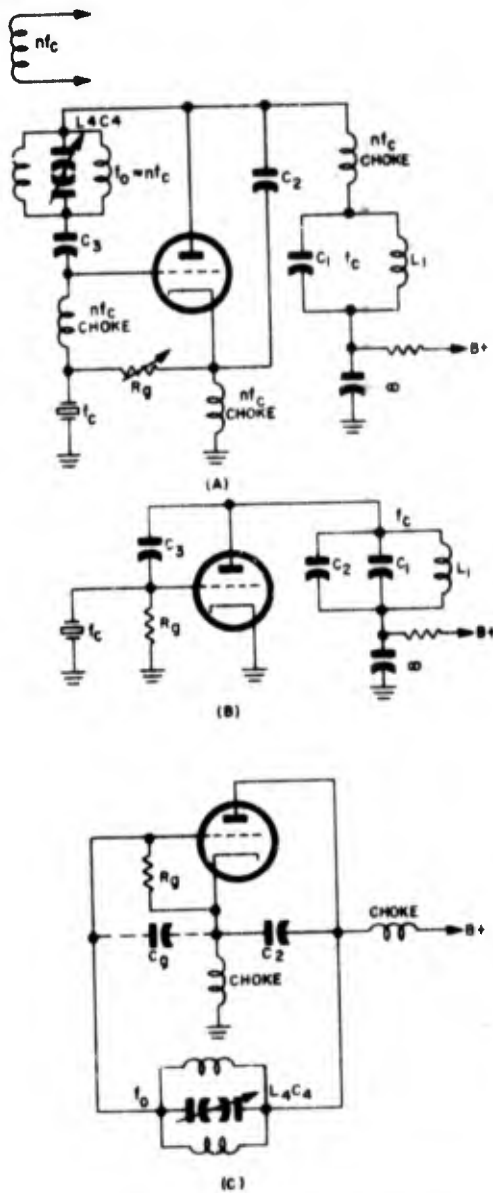
Figure 1-220. (A) Schematic diagram of Hahnel spectrum generator in which two oscillator circuits are combined in one stage; (B) Simplified schematic diagram of the crystal oscillator circuit of the spectrum generator; (C) Simplified schematic diagram of the v-f-o circuit of the spectrum generator
