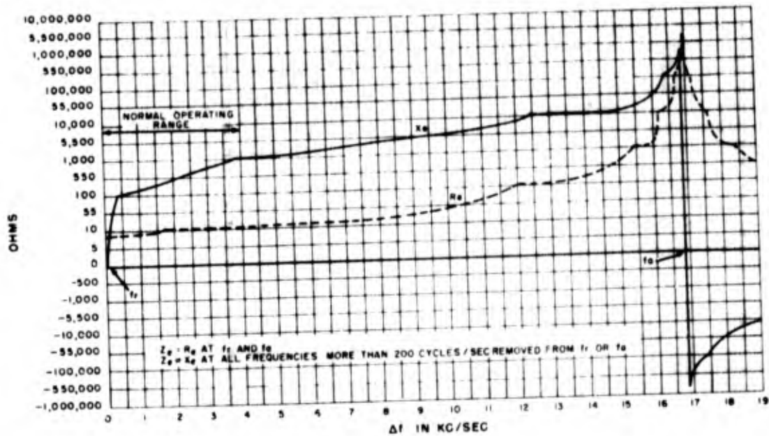
Figure 1-104. Typical characteristic curves for X_s and R_s of 10-mc crystal unit. (Shunt resistance, R_1 , across crystal is assumed to be negligible)
