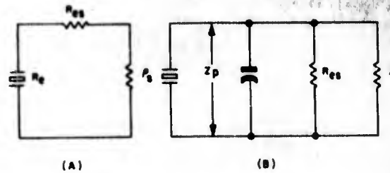
Figure 1-258. Equivalent circuit during build-up period of generalized negative-resistance crystal oscillator. (A) Series-mode circuit (B) Parallel-mode circuit
