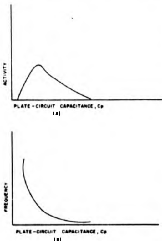
Figure 1-125. Variation of activity and frequency in Pierce oscillator as plate-circuit capacitance is increased
