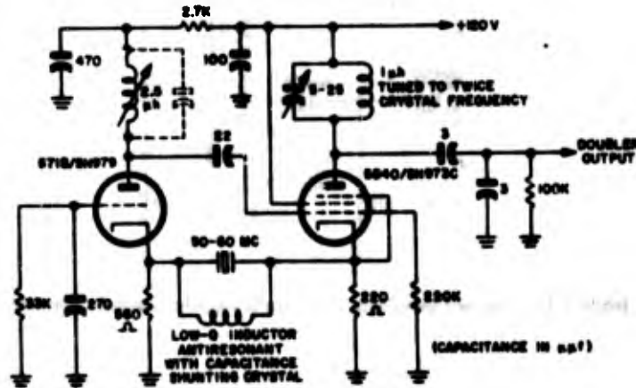
Figure 2-66. Schematic diagram of typical oscillator designed for use with Crystal Unit CR-54/U
