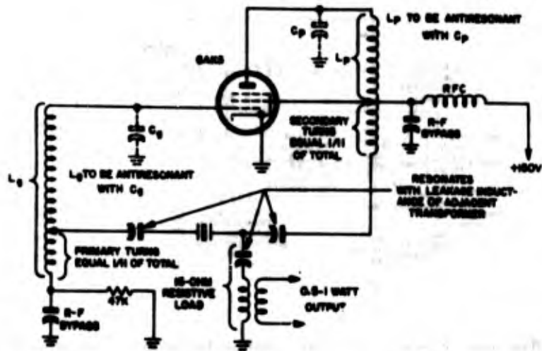
Figure 2-40. Schematic diagram of typical oscillator designed for use with Crystal Unit CR-51/U
