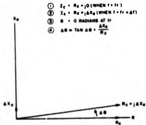
Figure 1-111. Phaser diagram, showing change in reactance, \Delta X_s , of series-mode crystal required to produce a small change in phase, \Delta\theta , where the resistance of the crystal circuit is equal to R_s .
