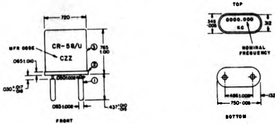
Figure 2-73. Crystal Unit CR-58/U
