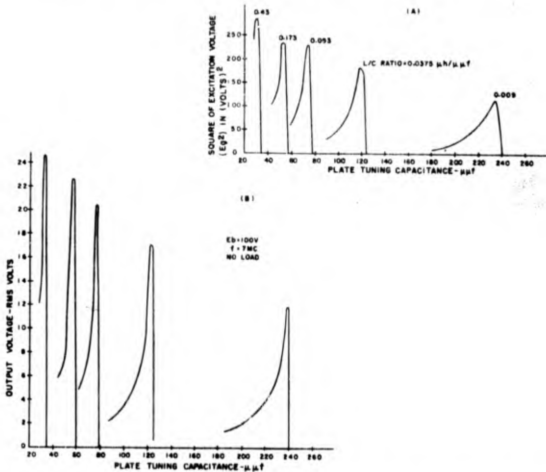
Figure 1-147. (A) Square of excitation voltage and (B) rms value of output voltage of experimental Miller oscillator versus plate tuning capacitance for various L/C ratios of plate tank. Same crystal unit as was used for curves in figure 1-144
