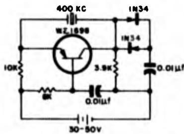
Figure 1-240. Modification of the crystal-feedback oscillator of figure 1-238 to provide greater frequency stability by providing greater amplitude stability with diode clipping
