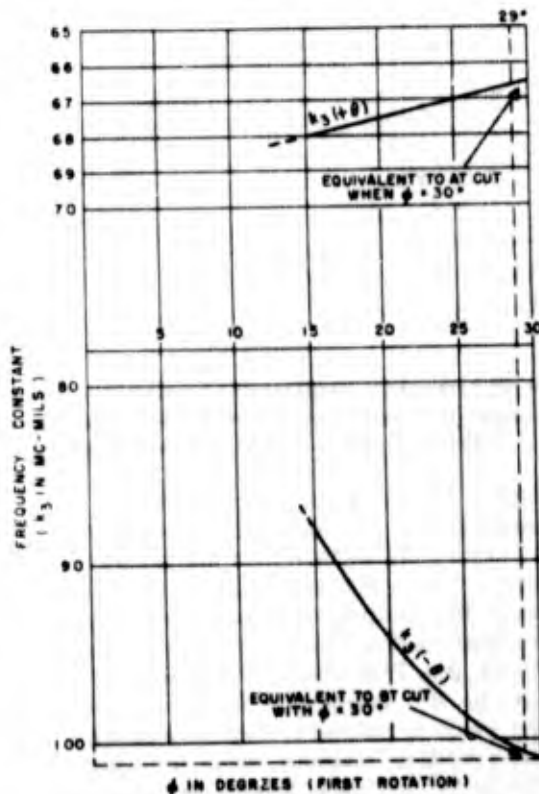
Figure 1-39. Frequency constant versus \phi (angle of rotation about Z axis) for the thickness-shear mode of V-cut crystals when \theta , the second angle of rotation, is so chosen that a zero temperature coefficient is obtained. The upper and lower curves are for positive and negative values of \theta , respectively
