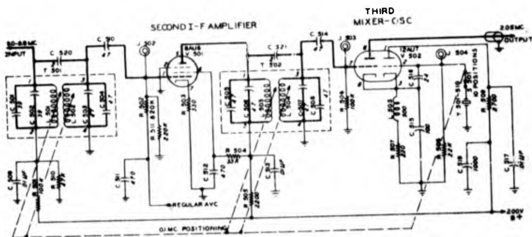
Figure 1-208. Second i-f amplifier unit in Radio Receiver R-27B/GR. Schematic diagram
