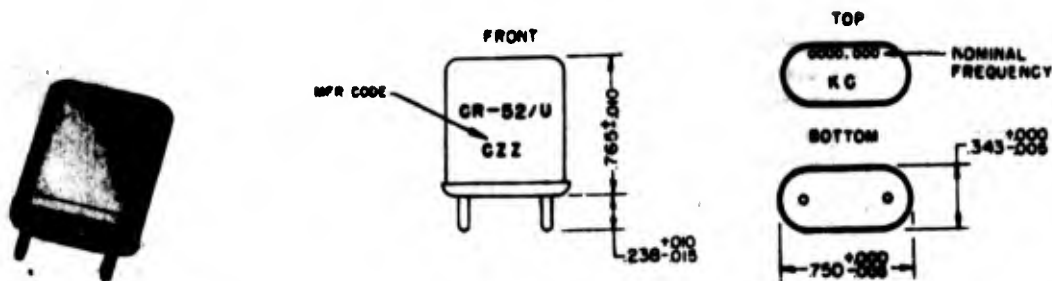
Figure 2-61. Crystal Unit CR-52/U
