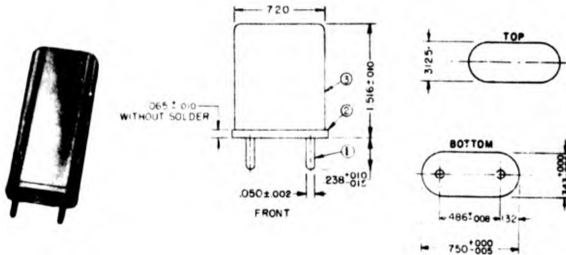
Figure 3-4. Crystal Holder HC-13/U
