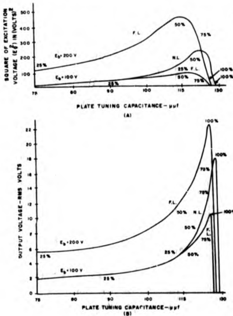
Figure 1-144. (A) Square of excitation voltage and (B) rms value of output voltage versus plate tuning capacitance of experimental Miller oscillator. Frequency = 7 mc; gridleak resistance = 1 megohm; and PI of CR-18/U crystal unit (with load capacitance of 32 \mu\mu f ) = 49 kilohms. F.L. = full load conditions (5,000 ohms series plate tank) and N.L. = no load conditions. Percentage points refer to percentages of maximum output voltage obtainable under given load and d-c plate voltage conditions
