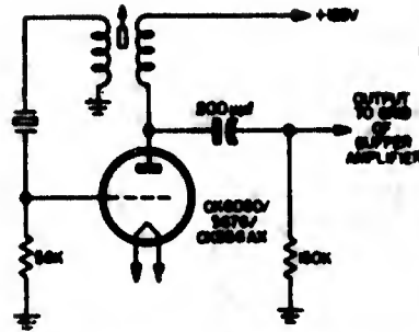
Figure 2-48. Schematic diagram of typical oscillator designed for use with Crystal Unit CR-55/U
