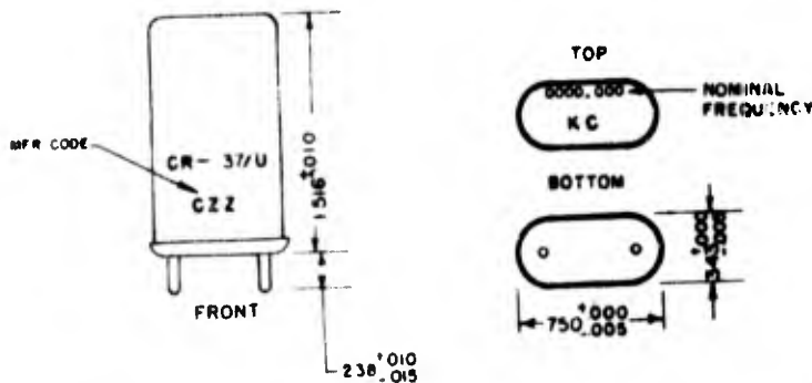
Figure 2-33. Crystal Unit CR-37/U
