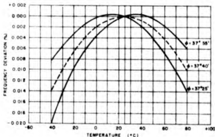
Figure 1-51. Temperature-frequency characteristics of element C
