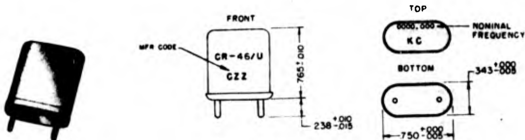
Figure 2-49. Crystal Unit CR-46/U
