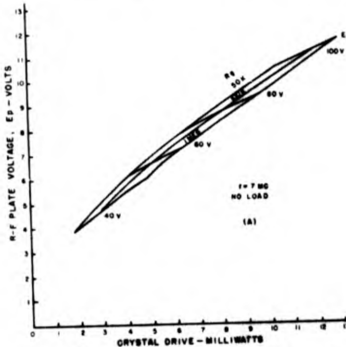
Figure 1-130. Output curves of tuned Pierce oscillator for different values of grid resistance when reactance of tuned plate circuit is adjusted for output voltages equal to 50 percent of the maximum attainable. A 7-mc CR-18/U crystal unit was used, having a P_i of 49,000 ohms when operating into its rated load capacitance of 32 \mu\mu\text{f} .
