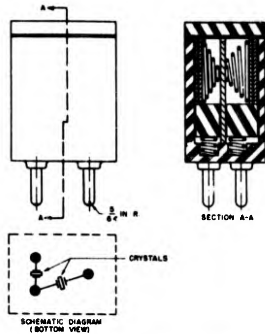
Figure 3-22. Crystal Holder FT-249
