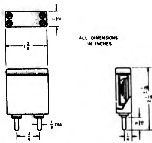
Figure 3-25. Crystal Holder HC-2/U and HC-3/U, except that the latter has pins of 5/32-in. diameter
