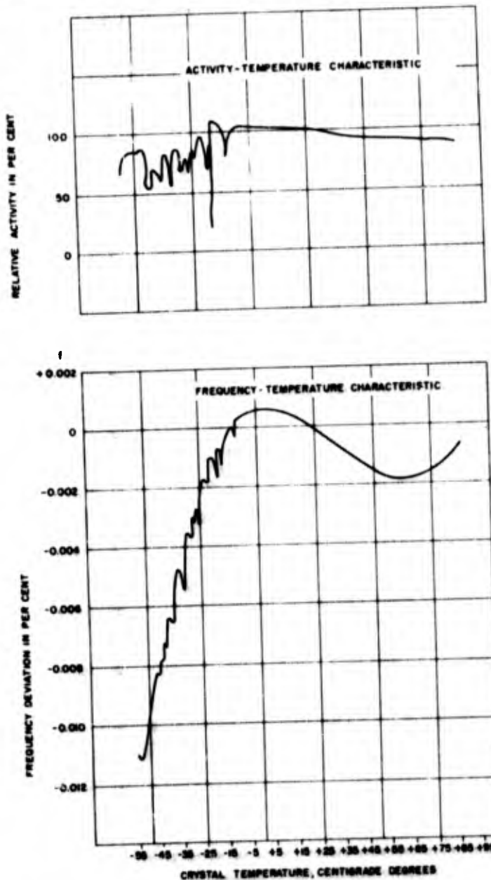
Figure 1-114. Activity-temperature and frequency-temperature characteristics of harmonic-mode A element, showing effects of unwanted modes
