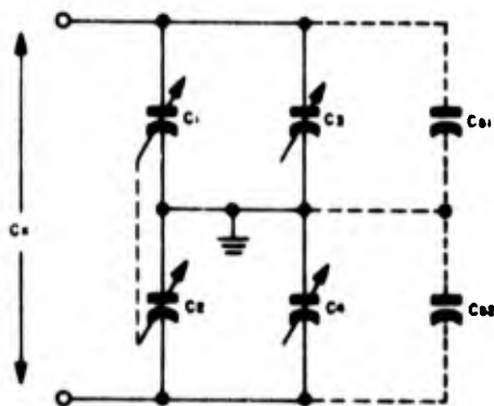
Figure 1-134. Ganged capacitances to enable adjustment of C_1/C_2 ratio of Pierce circuit without changing total load capacitance
