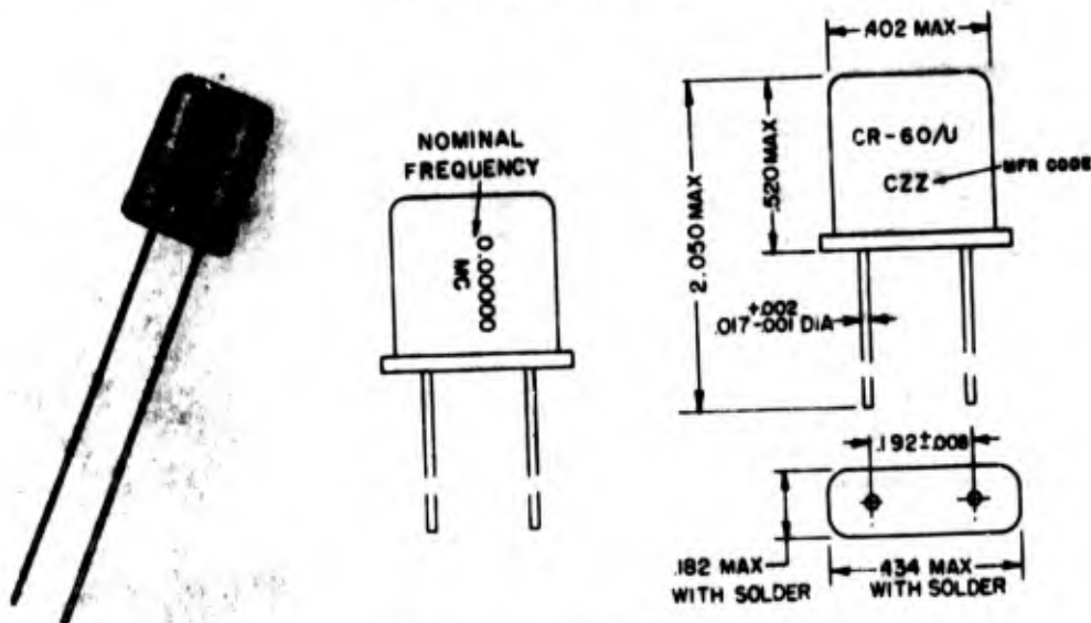
Figure 2-77. Crystal Unit CR-60/U
