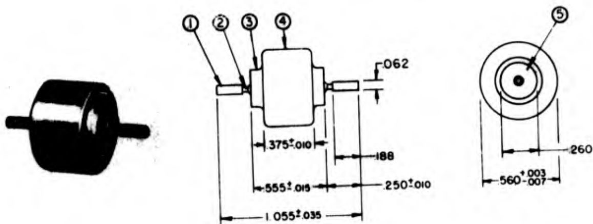
Figure 3-3. Crystal Holder HC-10/U
