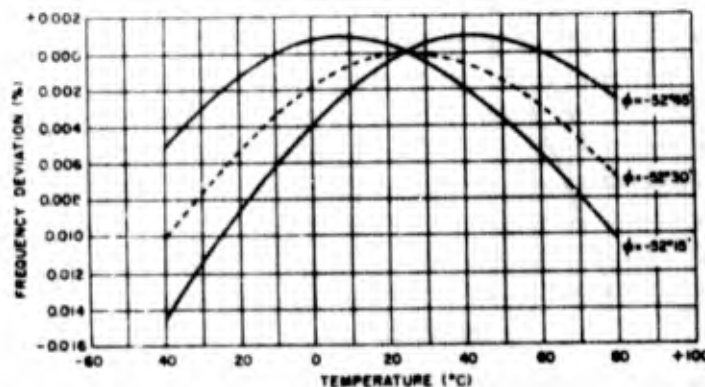
Figure 1-52. Temperature-frequency characteristics of element D
