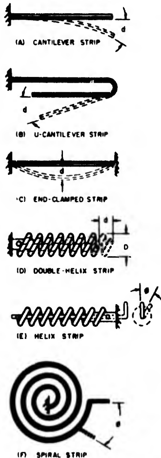
Figure 4-4. Basic types of bimetallic strips
