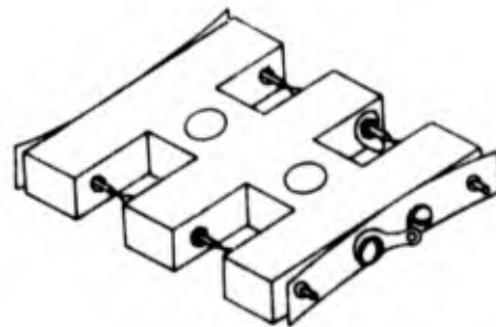
Figure 1-80. Pressure-pin mounting, with provisions for supporting four plated filter crystals *
