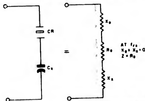
Figure 1-105. Equivalent circuit of crystal unit connected in series with capacitor
