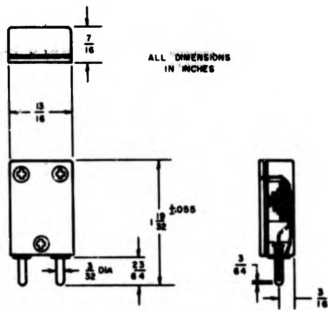
Figure 3-26. Crystal Holder HC-4/U
