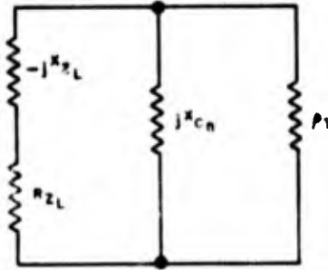
Figure 1-122. Generalized Pierce oscillator. X_{Z_L} and X_{C_n} represent the positive magnitudes of the equivalent reactances of the lead and the dynamic effects of the tube, respectively. R_p is the same as the R_p in figure 1-121
