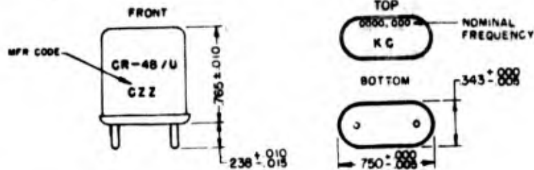
Figure 2-53. Crystal Unit CR-48/U
