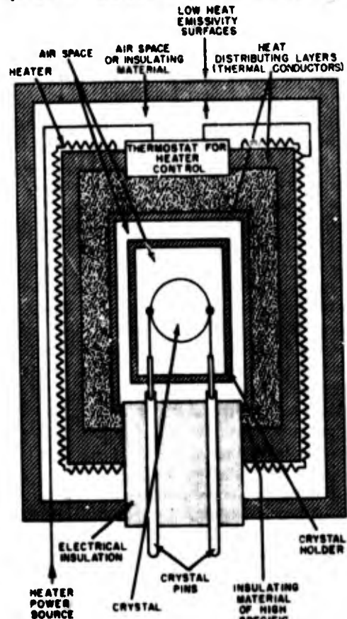
Figure 4-1. General construction features of typical crystal oven
