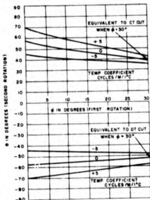
Figure 1-41. Relations of \theta to \phi , for face-shear mode of Y cut, which provide temperature coefficients of 0, +5, and -5 parts, per million per degree centigrade
