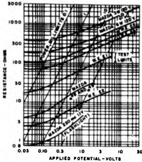
Figure 1-162. Resistance of typical tungsten lamps versus applied voltage and power dissipation when the ambient temperature is 300° Kelvin scale (approximately 27° C)
