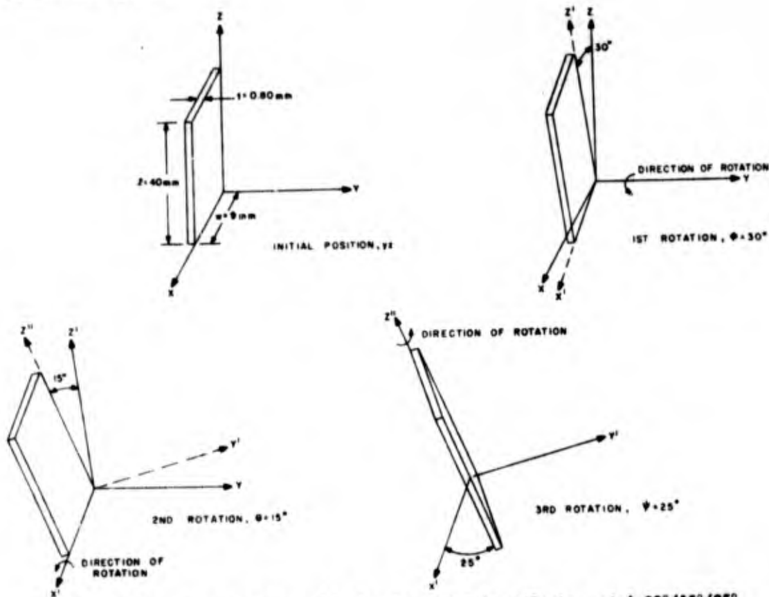
Figure 1-17 Orientation of crystal having the rotational specifications yztl: 30°/15°/25°
