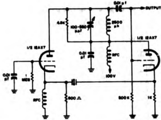
Figure 2-38. Schematic diagram of typical oscillator designed for use with Crystal Unit CR-39/U
