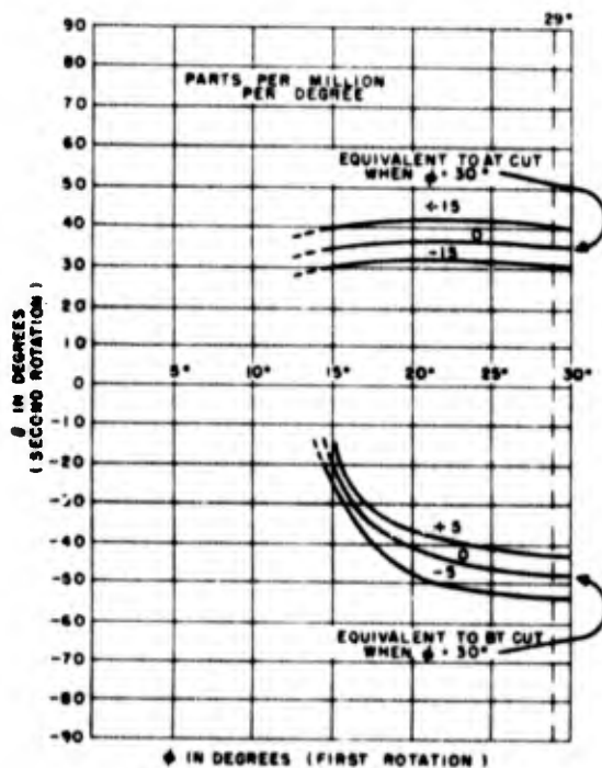
Figure 1-40. Relations of \theta to \phi , for thickness-shear mode of V cut, which provide the temperature coefficients indicated for each curve
