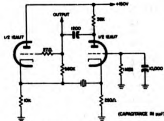
Figure 2-8. Schematic diagram of typical oscillator designed for use with Crystal Unit CR-19/U
