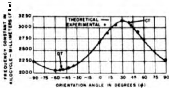
Figure 1-45. Frequency constant versus angle of rotation about X axis for face-shear elements of Y group
