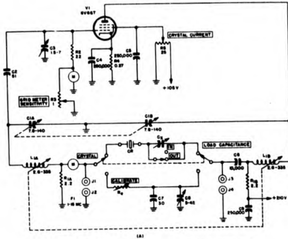
Figure 1-185. Colpitts circuits modified for series-mode crystal control
