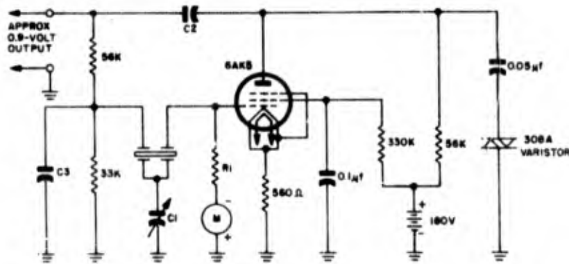
Figure 1-157. Practical crystal-oscillator design employing very-low-frequency crystal unit with two sets of electrodes
