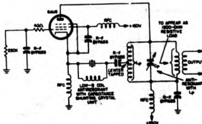
Figure 2-42. Schematic diagram of typical oscillator designed for use with Crystal Unit CR-52/U
