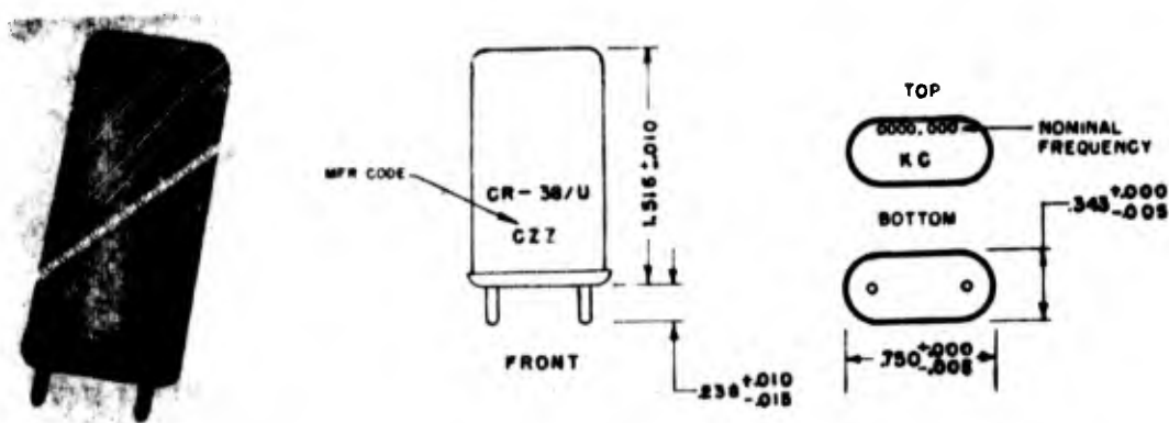
Figure 2-35. Crystal Unit CR-38/U
