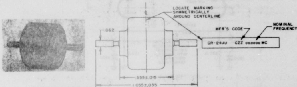
Figure 2-11. Crystal Unit CR-24/U
