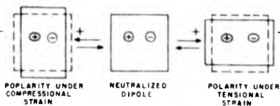
Figure 1-7. Effective polarities resulting from sudden displacements of the centers of charge of a neutralized dipole. (If after displacement, the crystal were maintained indefinitely in the strained position, the effective polarity would eventually be neutralized by an accumulation of ions at the poles. A sudden return from such a state would thus result in an effective polarization in the unstrained position)
