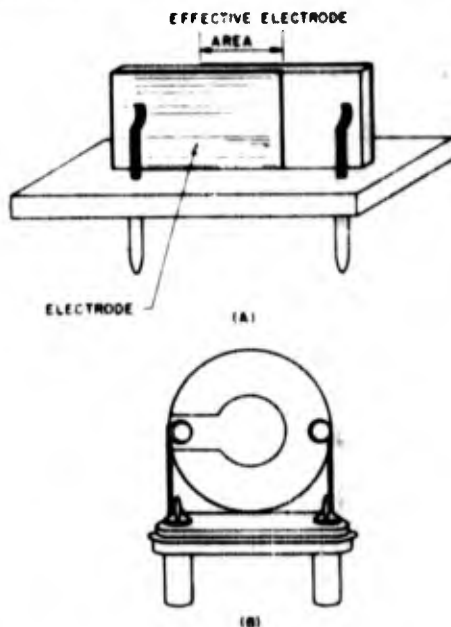
Figure 1-88. Edge-clamped systems of mounting. (A) Mounting for low-frequency crystals. (B) Cemented-lead mounting for high-frequency crystals
