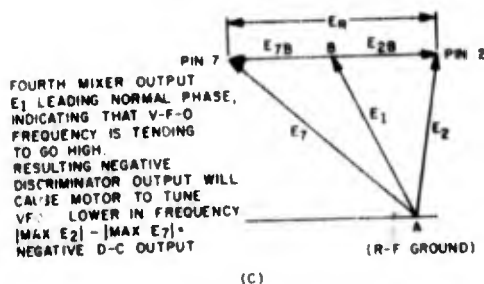
Figure 1-197. Discriminator operation as a function of the phase difference between the input voltages
