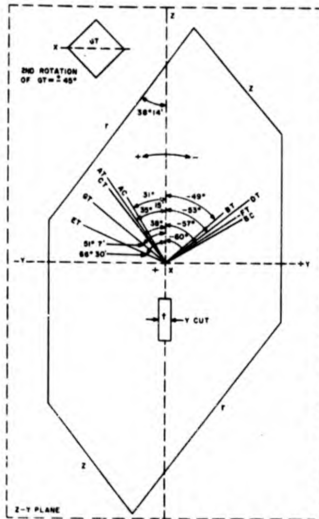
Figure 1-42. Rotation angles of Y cut about X axis which provide the principal members of the Y group. The GT cut is the only member having a second rotation ( \pm 45^\circ about the Y' axis). The +X sign indicates that the positive end of the X axis points toward the observer
