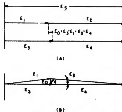
Figure 1-161. Phasor diagrams of bridge voltages in Meacham oscillator. Angles \phi and \theta (greatly magnified) represent small shifts in phase when crystal unit is operating slightly off series resonance
