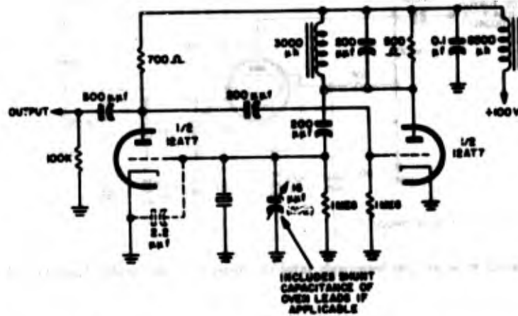
Figure 2-52. Schematic diagram of typical oscillator designed for use with Crystal Unit CR-47/U
