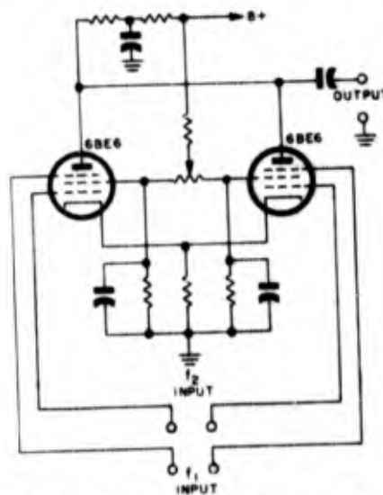
Figure 1-218. Balanced modulator circuit, which is useful as a mixer stage when maximum attenuation of the input frequencies in the output is desired
