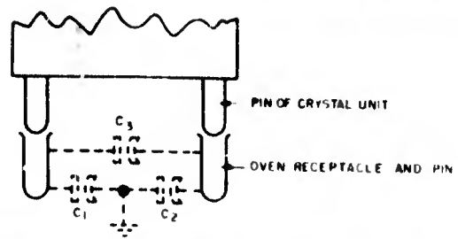
Figure 4-18. Pin-to-pin electrostatic capacitance of crystal oven
