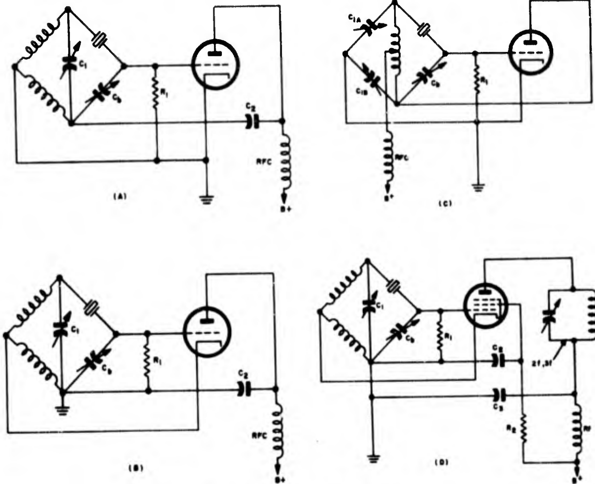
Figure 1-172. Miscellaneous capacitance-bridge oscillators
