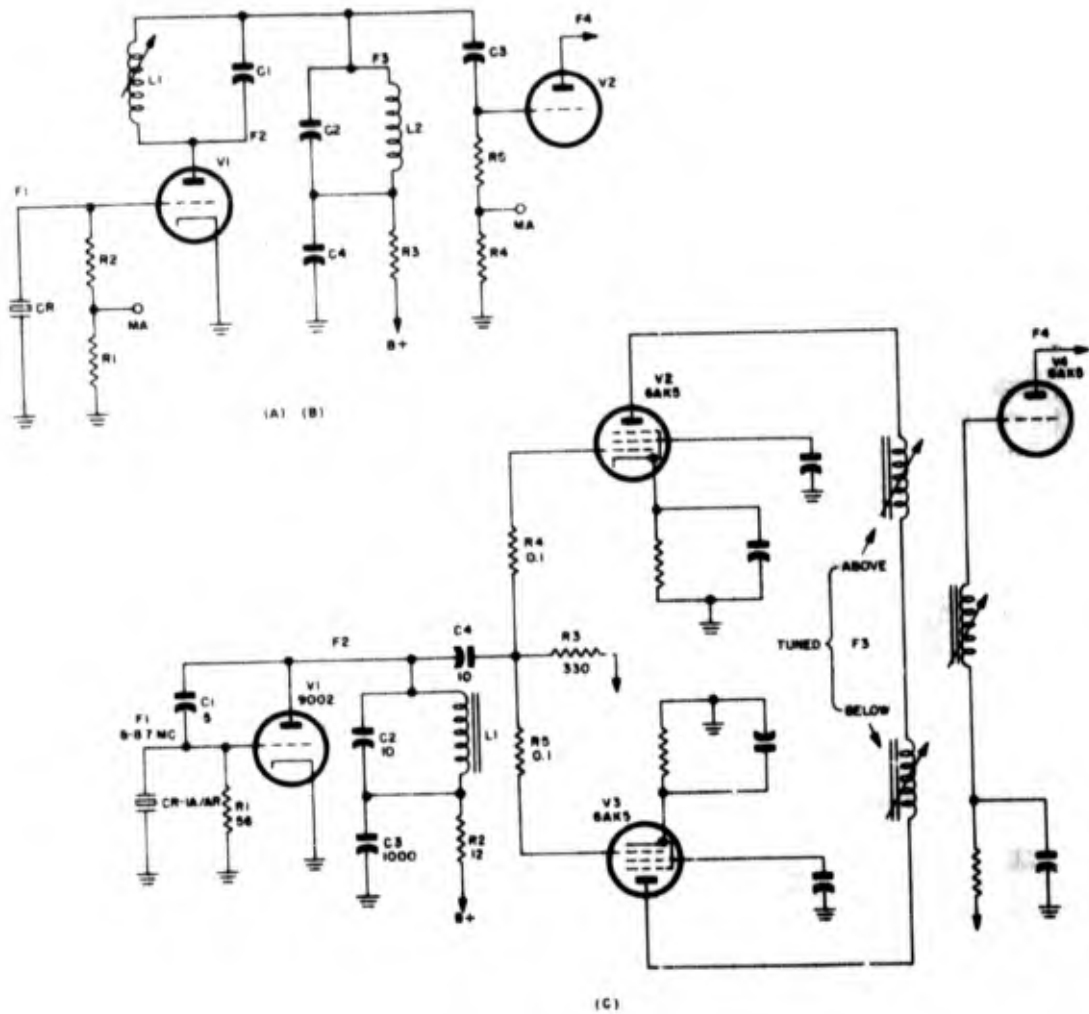
Figure 1-150. Modified Miller oscillators using triodes
