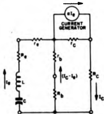
Figure 1-231. Equivalent a-c circuit of tuned-emitter negative-resistance oscillator. For crystal control, L , C , and R , can be interpreted as being the series-arm parameters of a crystal unit
