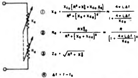
Figure 1-98. Equivalent circuit of crystal unit when represented as an effective reactance in series with an effective resistance. The ganged arrows indicate that X_e and R_e will vary together with changes in the frequency, as indicated by the approximate formulas given as functions of \Delta f . ( X_{c0} is negative.)
