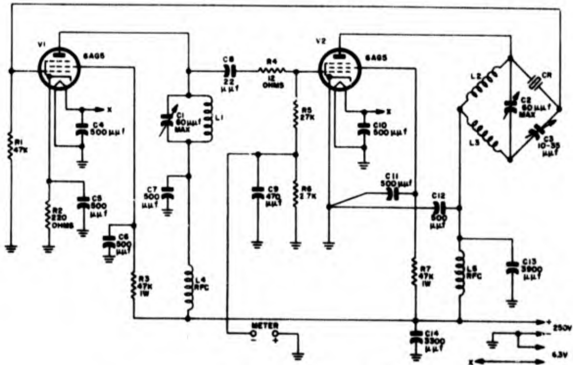
Figure 1-170. A two-tube capacitance-bridge oscillator which is practical for operation in the 50-100-mc frequency range
