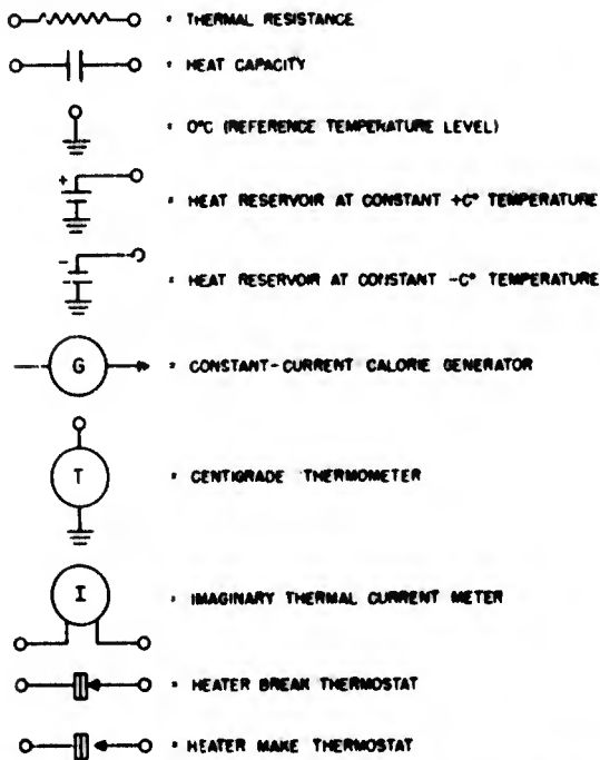
Figure 4-11. Electrical symbols applied to parameters of thermal circuits
