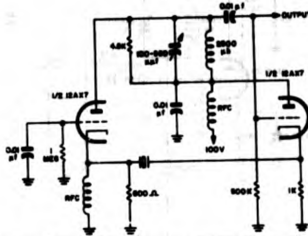
Figure 2-40. Schematic diagram of typical oscillator designed for use with Crystal Unit CR-49/U
