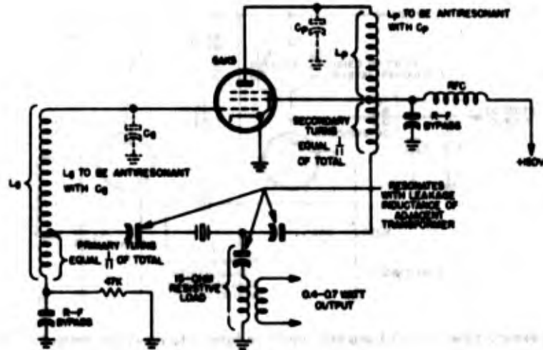
Figure 2-44. Schematic diagram of typical oscillator designed for use with Crystal Unit CR-53/U
