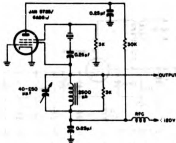
Figure 2-16. Schematic diagram of typical oscillator designed for use with Crystal Unit CR-26/U
