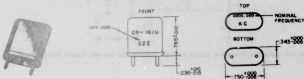
Figure 2-5. Crystal Unit CR-18/U
