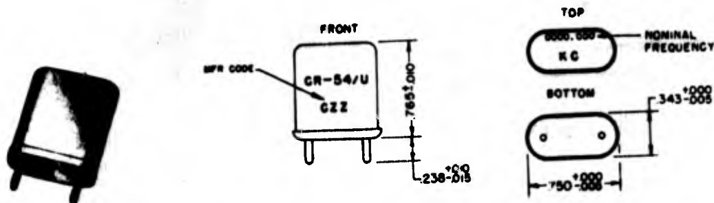
Figure 2-65. Crystal Unit CR-54/U
