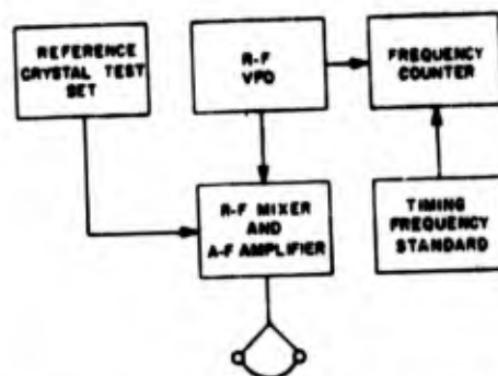
Figure 2-90. System for measuring crystal frequencies aurally with a variable frequency oscillator that is visually monitored by a direct-reading electronic counter
