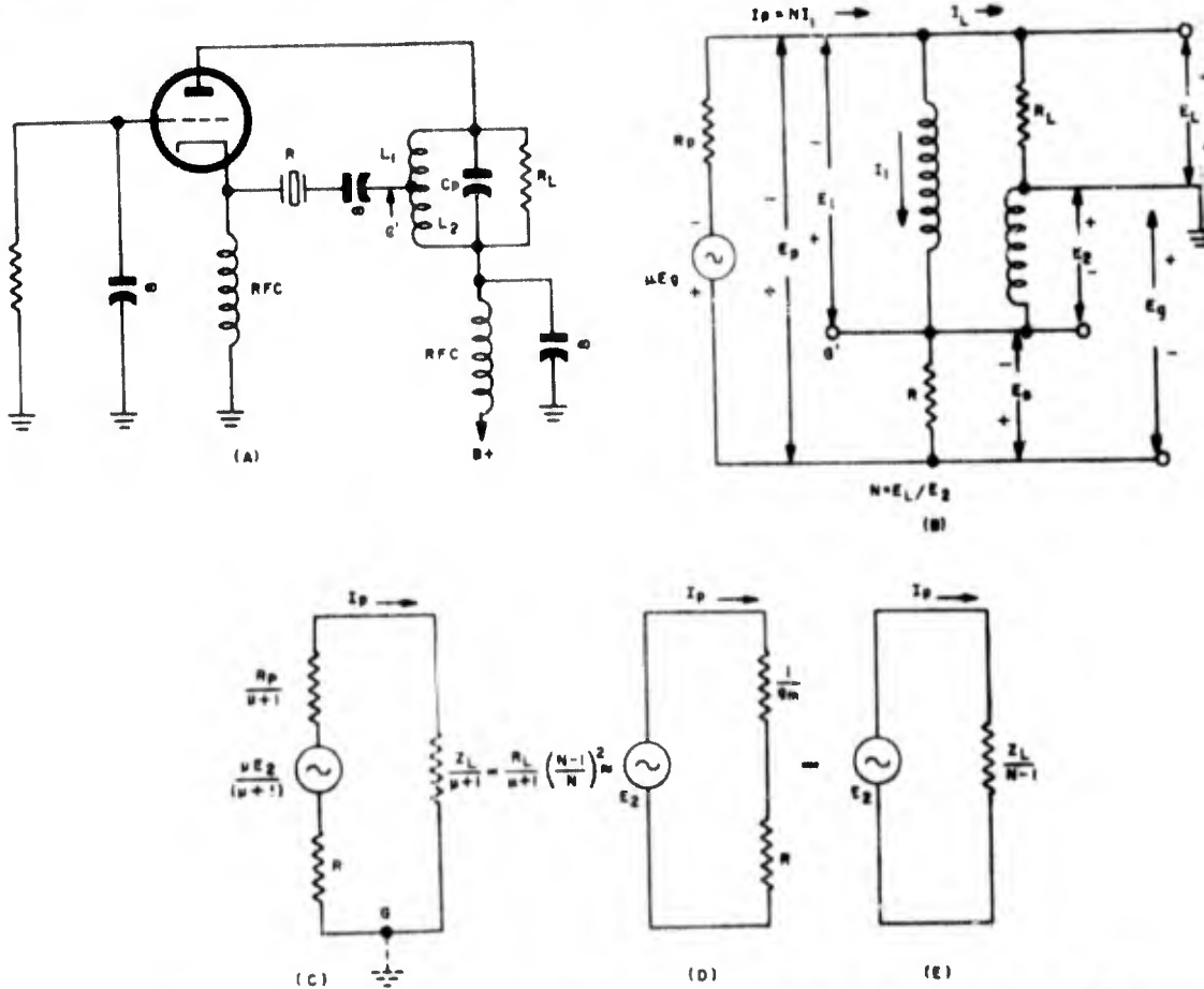
Figure 1-178. Basic grounded-grid oscillator and equivalent circuit progressively simplified
