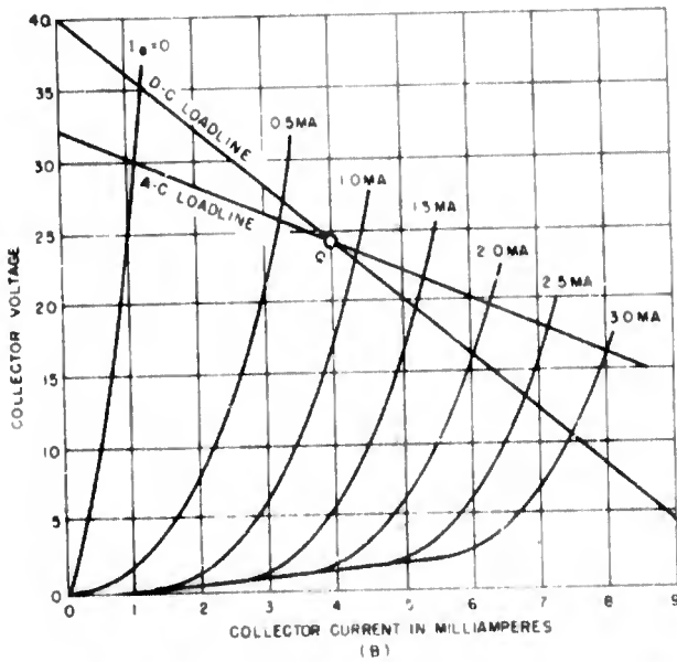
Figure 1-223. (A) Current amplification, \alpha , of point-contact transistor versus emitter current, I_e . (B) Collector characteristics of point-contact transistor. A-C load line indicates approximate operating region during oscillations. (C) Collector current characteristics for different point-contact transistors of type 1729, showing effects of temperature
