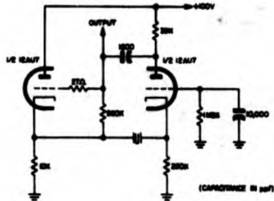
Figure 2-30. Schematic diagram of typical oscillator designed for use with Crystal Unit CB-35/U
