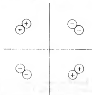
Figure 1-8. Example of distribution of charges having a center of symmetry *
