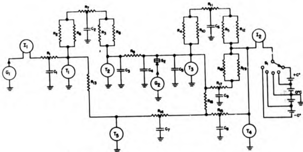
Figure 4-12. Equivalent electrical circuit of crystal oven
