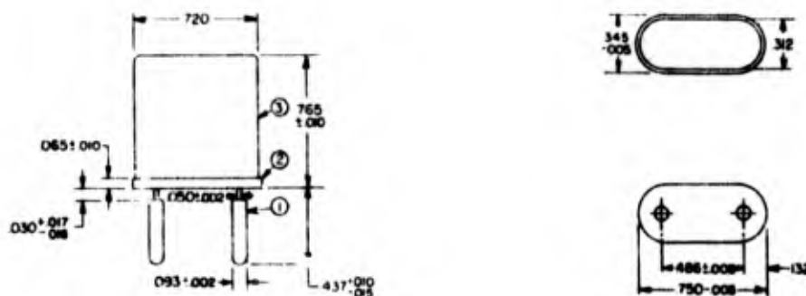
Figure 3-8. Crystal Holder HC-17/U
