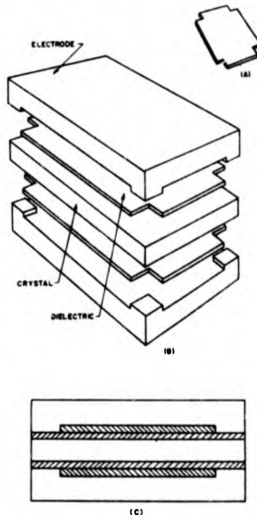
Figure 1-75. Two methods (B and C) by which a corner-clamped, air-gap holder can be converted into a dielectric sandwich. Figure A shows a dielectric sheet cut to the dimensions of the air gap
