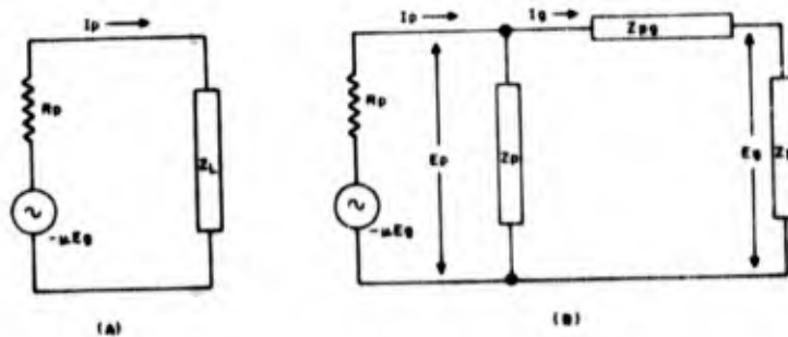
Figure 1-119. (A) Equivalent circuit of vacuum-tube amplifier. (B) Equivalent circuit of crystal oscillators of the Pierce and Miller types
