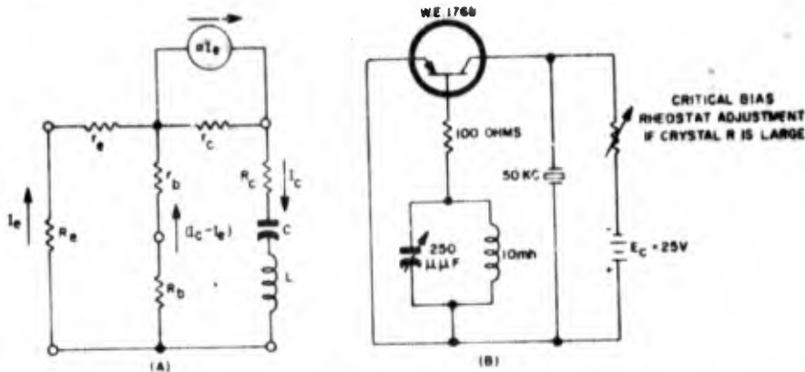
Figure 1-232. (A) Equivalent a-c circuit of tuned-collector negative-resistance oscillator. For crystal control, L , C , and R_c can be interpreted as being the series-arm parameters of a crystal unit; (B) Crystal-controlled tuned-collector negative-resistance oscillator. The parallel tuned tank is inserted in the base circuit in lieu of a resistor in order to obtain negative resistance values in excess of 40,000 ohms
