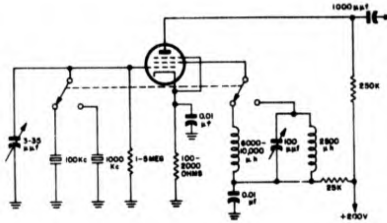
Figure 1-186. Typical design of single-tube general-purpose crystal calibrator circuit
