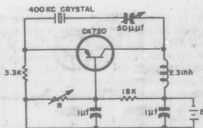
Figure 1-236. Frequency-stabilized circuit for single battery supply
