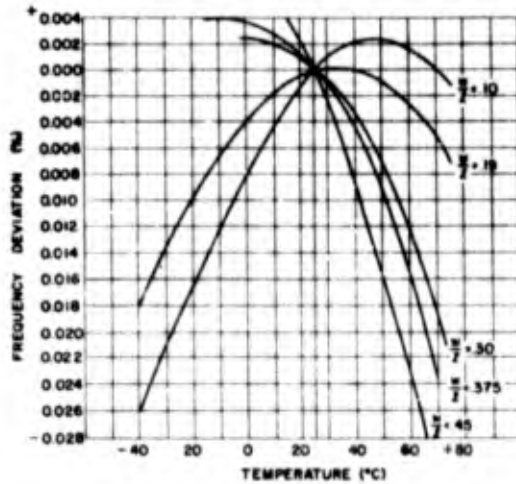
Figure 1-26. Percentage frequency deviation for E elements of various w/l ratios. Initial temperature = 25°C
