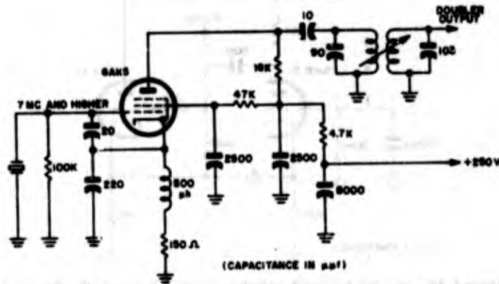
Figure 2-6. Schematic diagram of typical oscillator designed for use with Crystal Unit CR-18/U
