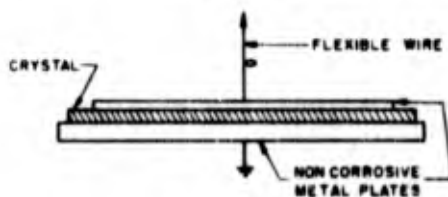
Figure 1-69. Gravity sandwich
