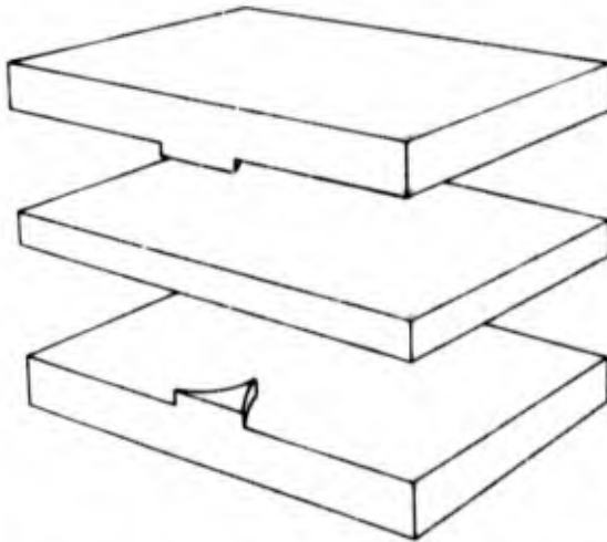
Figure 1-72. Typical nodal-clamped, air-gap method of mounting crystals
