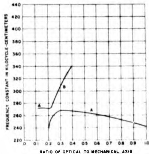
Figure 1-20. Frequency constant for length-extensional mode (curve A) of X-cut crystal where the width and length are parallel to the Z and Y axes, respectively. Curve B is the frequency constant of a face-shear mode coupled to a second flexural mode, whose interference makes the crystal useless for w/l ratios between 0.2 and 0.3, unless the thickness approaches the dimensions of the width *
