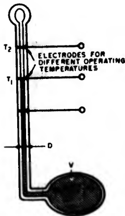
Figure 4-7. Diagram of typical mercury thermostat
