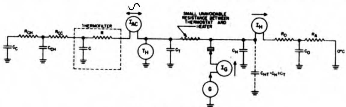
Figure 4-16. Oven thermal A-C circuit
