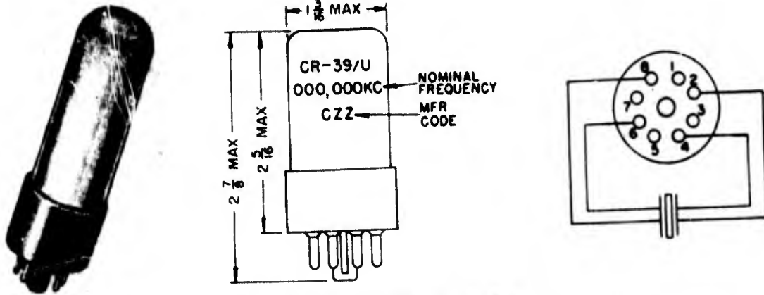
Figure 2-37. Crystal Unit CR-39/U
