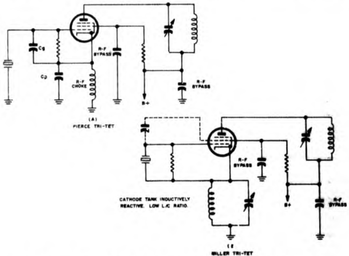
Figure 1-139. Basic tri-tet circuits where excitation voltage is a function of both screen- and plate-circuit r-f currents
