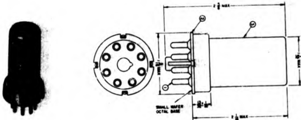
Figure 3-7. Crystal Holder HC-16/U
