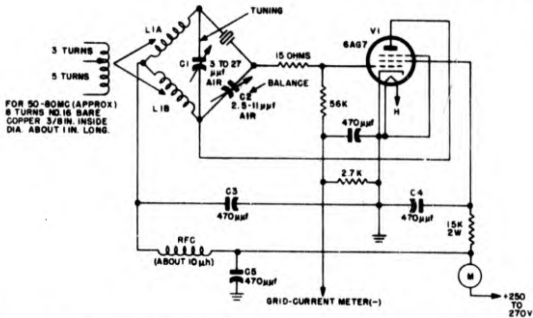
Figure 1-169. A capacitance-bridge oscillator for higher power output which is practical for operation in the 50-80-mc frequency range. Resistors not otherwise specified are 1/2 w. All fixed capacitors have mica dielectrics
