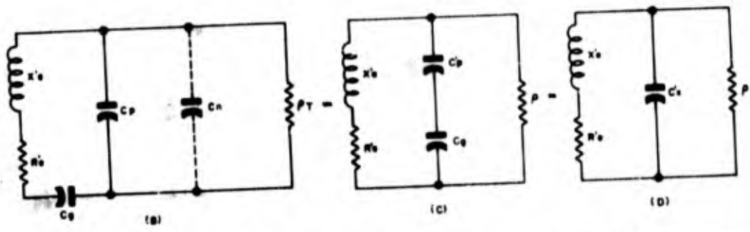
Figure 1-121. Generalized Pierce oscillator. X_c' and R_c' are the effective impedance parameters of the crystal unit based upon the assumption that C_{pr} is a part of C_p . C_n is an equivalent negative capacitance having a positive resistance equal to that of L_T . I_p is the r-f plate current of the vacuum tube.
