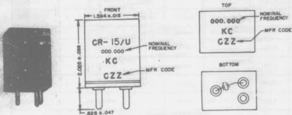
Figure 2-1. Crystal Unit CR-15/U
