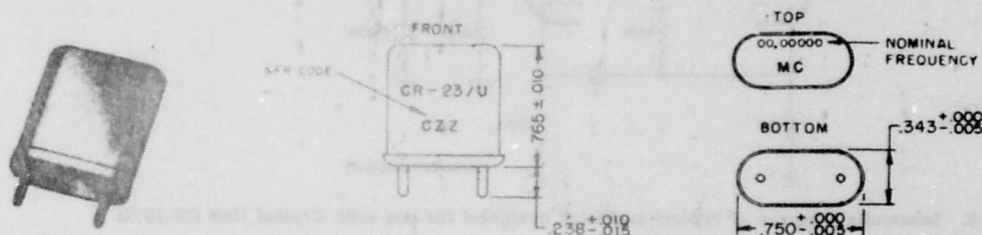
Figure 2-9. Crystal Unit CR-23/U
