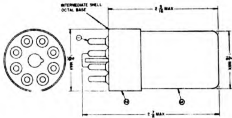
Figure 3-6. Crystal Holder HC-15/U
