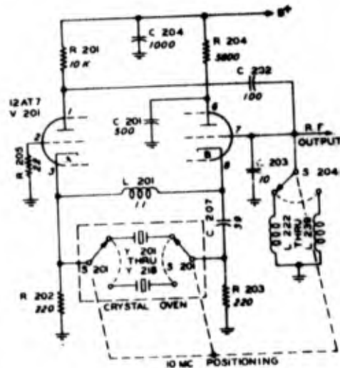
Figure 1-205. Oscillator unit of 1st injection system in Radio Receiver R-278/GR. Schematic diagram
