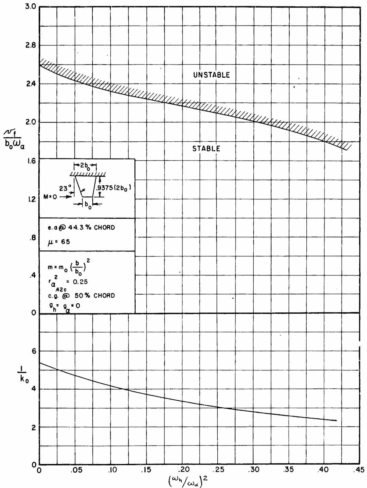
FIGURE 3.7 THEORETICAL RESULTS FOR BARE STRAIGHT-WING PLANFORM BASED ON INCOMPRESSIBLE THEORY
