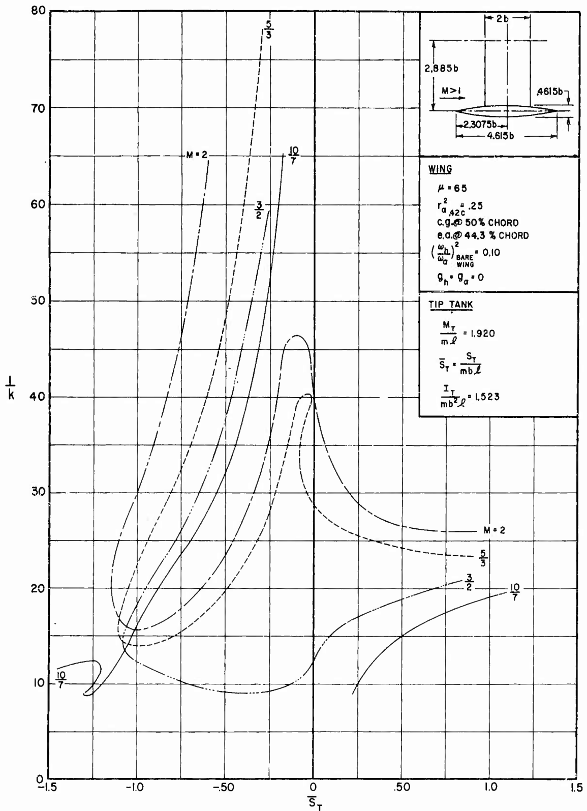
FIGURE C.7(b) REDUCED FREQUENCY VERSUS TIP-TANK STATIC-UNBALANCE PARAMETER FOR STRAIGHT-WING PLANFORM, FREE-TO-ROLL
