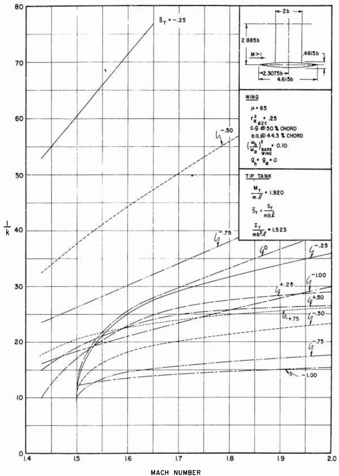
FIGURE 3.15 (Continued) THEORETICAL RESULTS FOR STRAIGHT WING WITH TIP TANK, FREE TO ROLL
