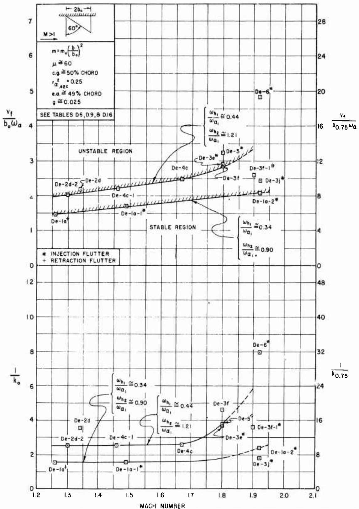
FIGURE 3.10 EXPERIMENTAL FLUTTER STABILITY BOUNDARIES FOR BARE DELTA-WING PLANFORM
