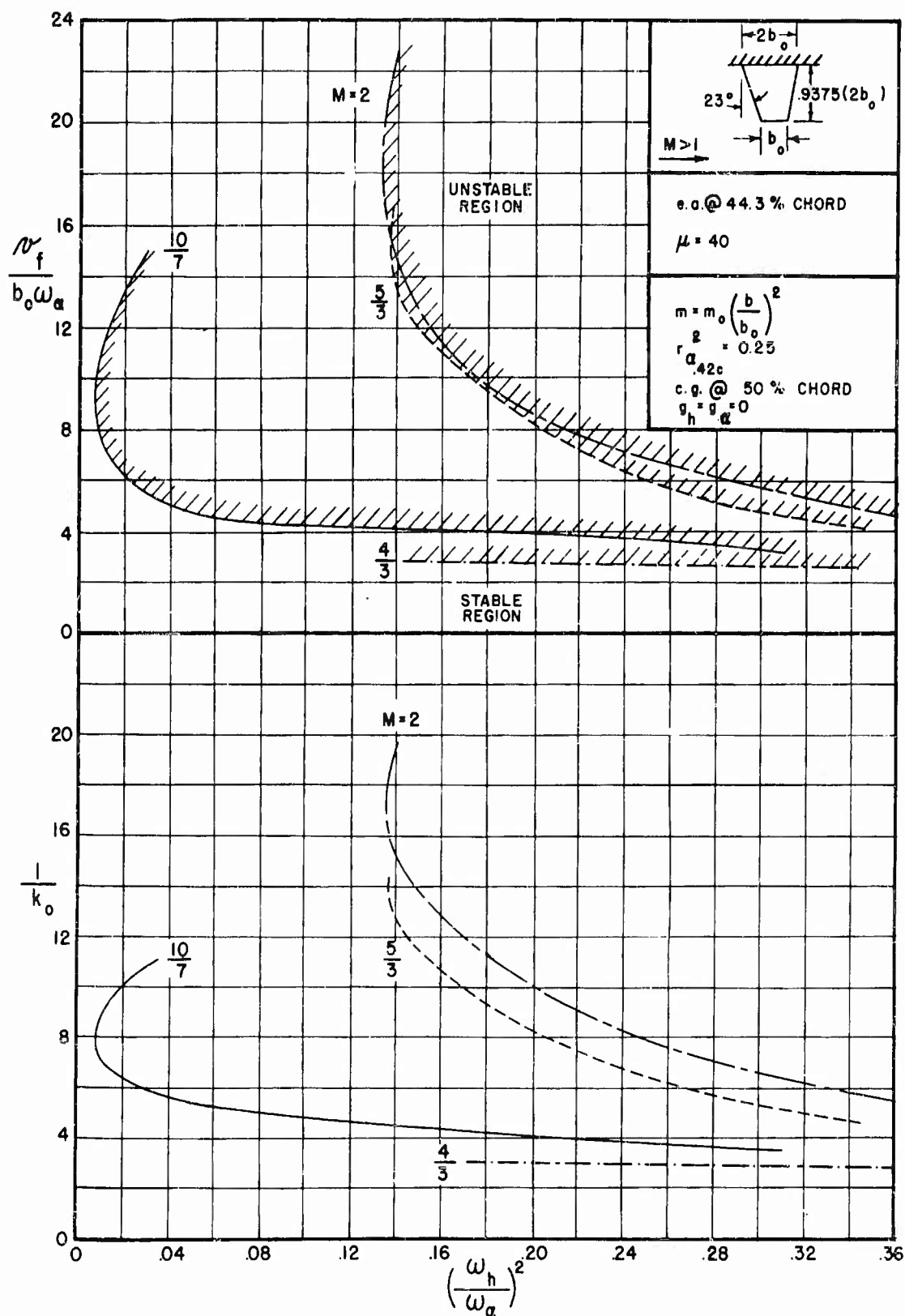
FIGURE C.1(f) FLUTTER COEFFICIENT AND REDUCED FREQUENCY VERSUS FREQUENCY RATIO FOR BARE STRAIGHT-WING PLANFORM, e.a. AT 44.3% CHORD, \mu = 40
