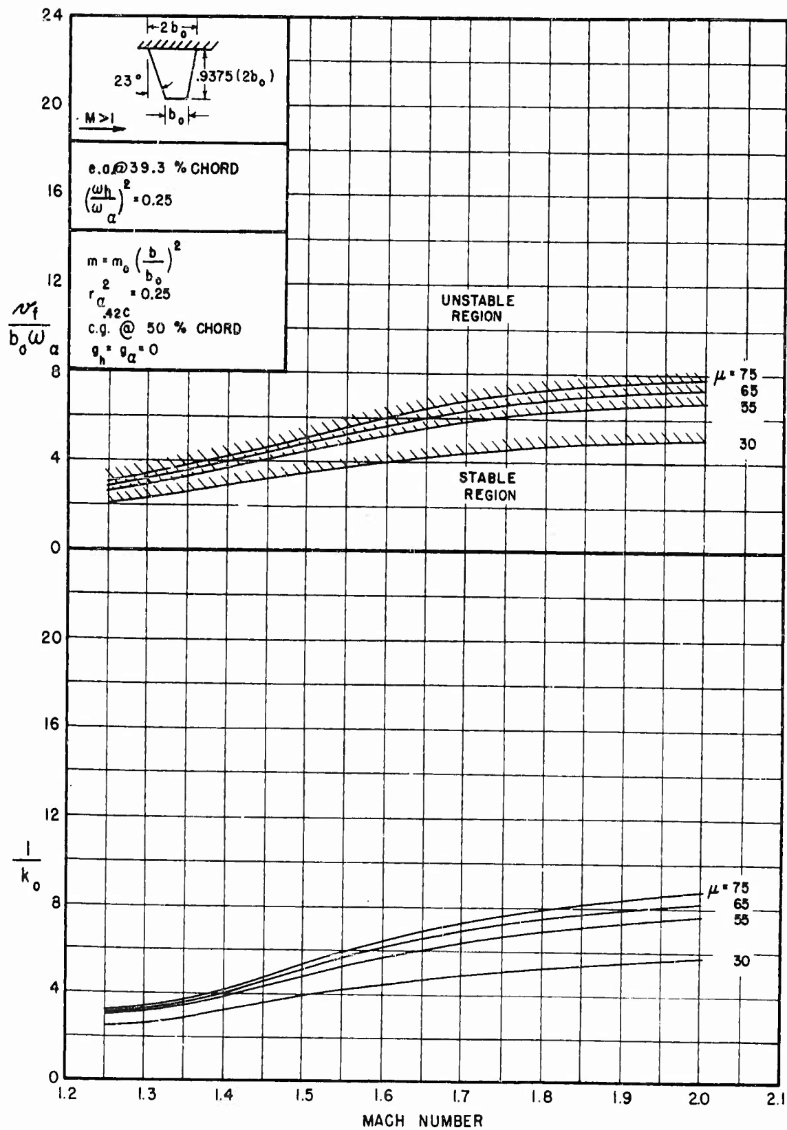
FIGURE 3.1(c) THEORETICAL RESULTS FOR BARE STRAIGHT-WING PLAN-FORM, e.a. AT 39.3% CHORD, (\frac{\omega_h}{\omega_\alpha})^2 = 0.25
