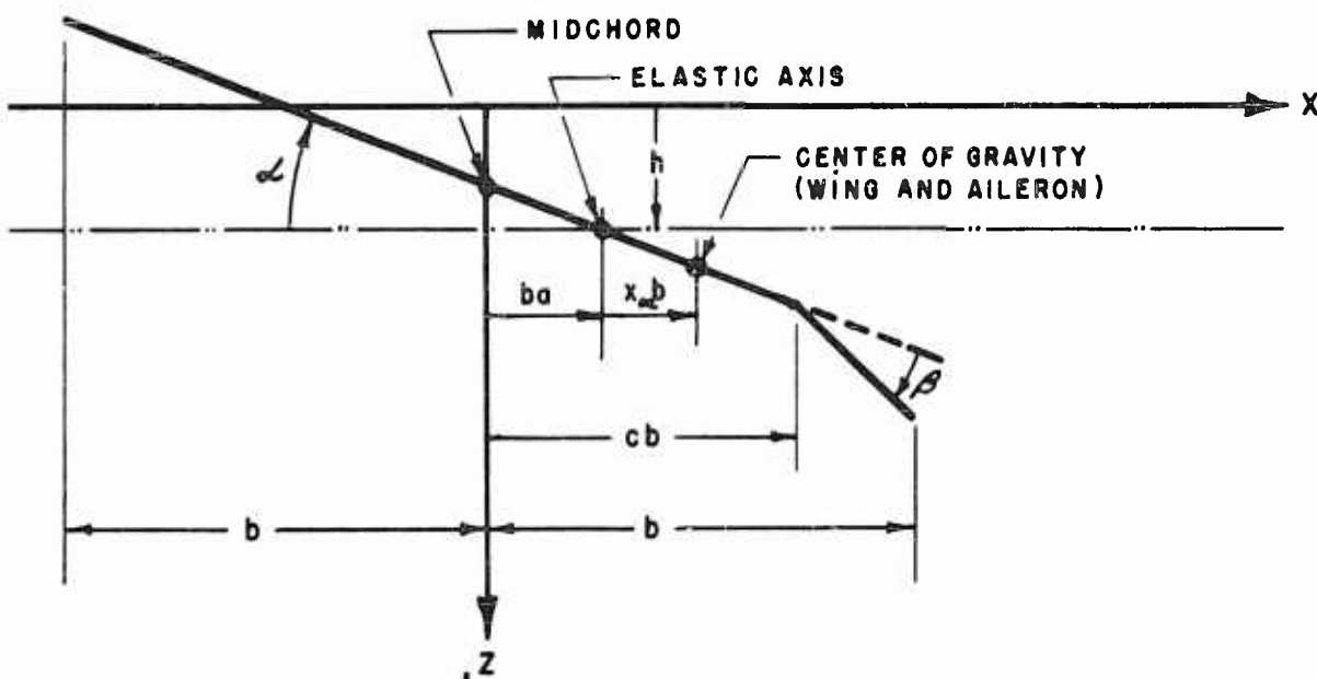
(b) Streamwise Section
