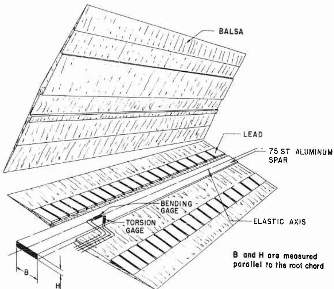
FIGURE D.1 A TYPICAL SUPERSONIC FLUTTER MODEL
