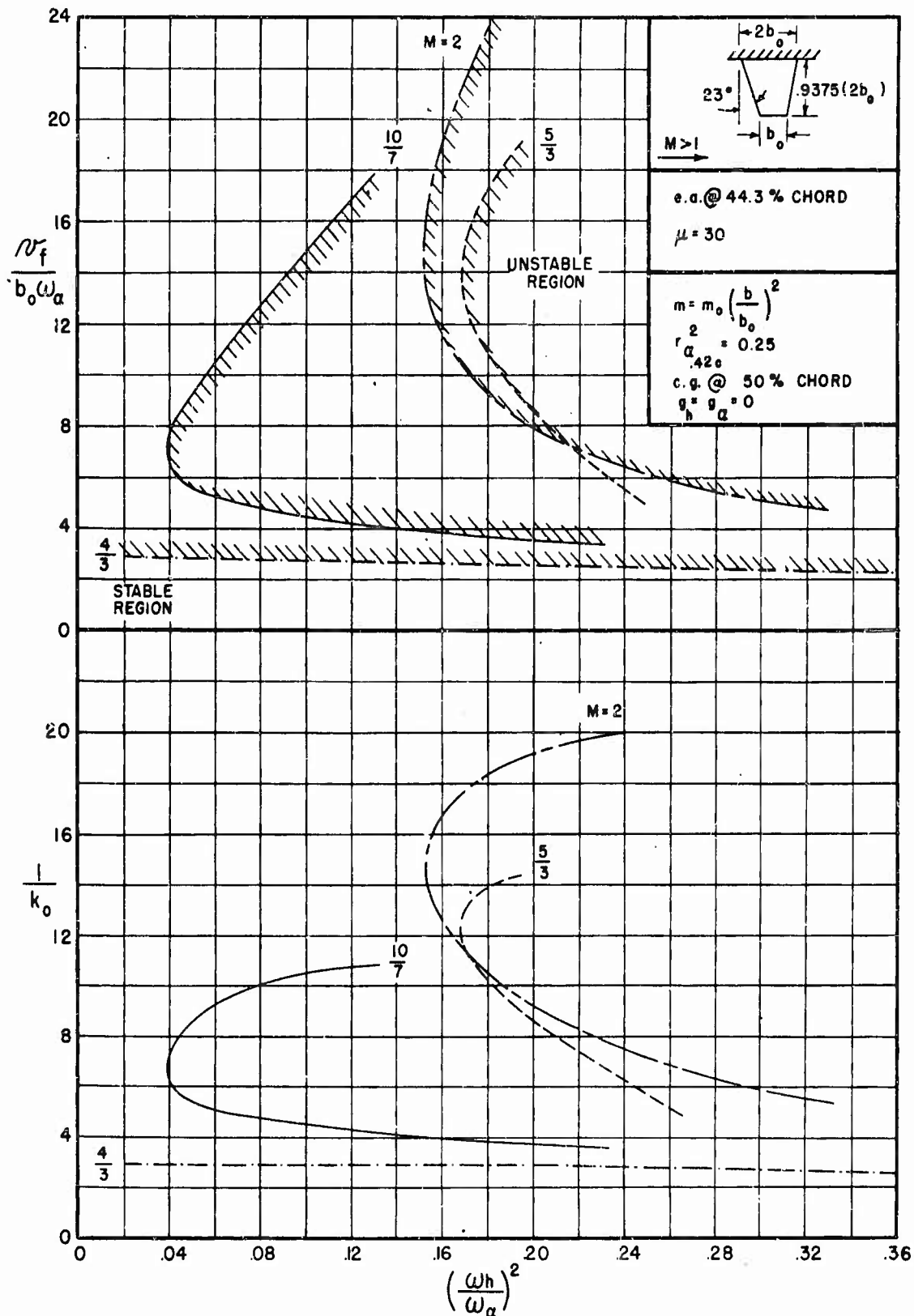
FIGURE C.1(e) FLUTTER COEFFICIENT AND REDUCED FREQUENCY VERSUS FREQUENCY RATIO FOR BARE STRAIGHT-WING PLANFORM, e.a. AT 44.3% CHORD, \mu = 30
