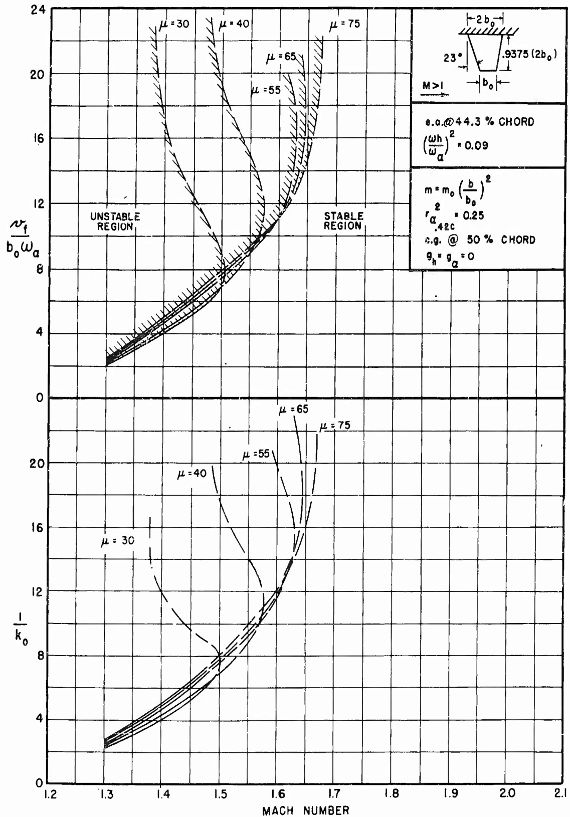
FIGURE 3.1(d) THEORETICAL RESULTS FOR BARE STRAIGHT-WING PLAN-FORM, e.a. AT 44.3% CHORD, (\frac{\omega_h}{\omega_a})^2 = 0.09
