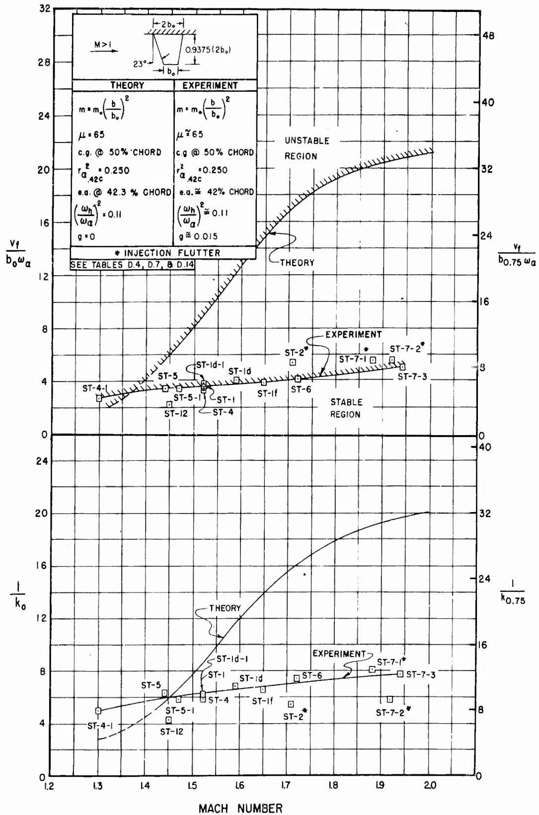
FIGURE 3.4 THEORETICAL AND EXPERIMENTAL FLUTTER STABILITY BOUNDARIES FOR BARE STRAIGHT-WING PLANFORM
