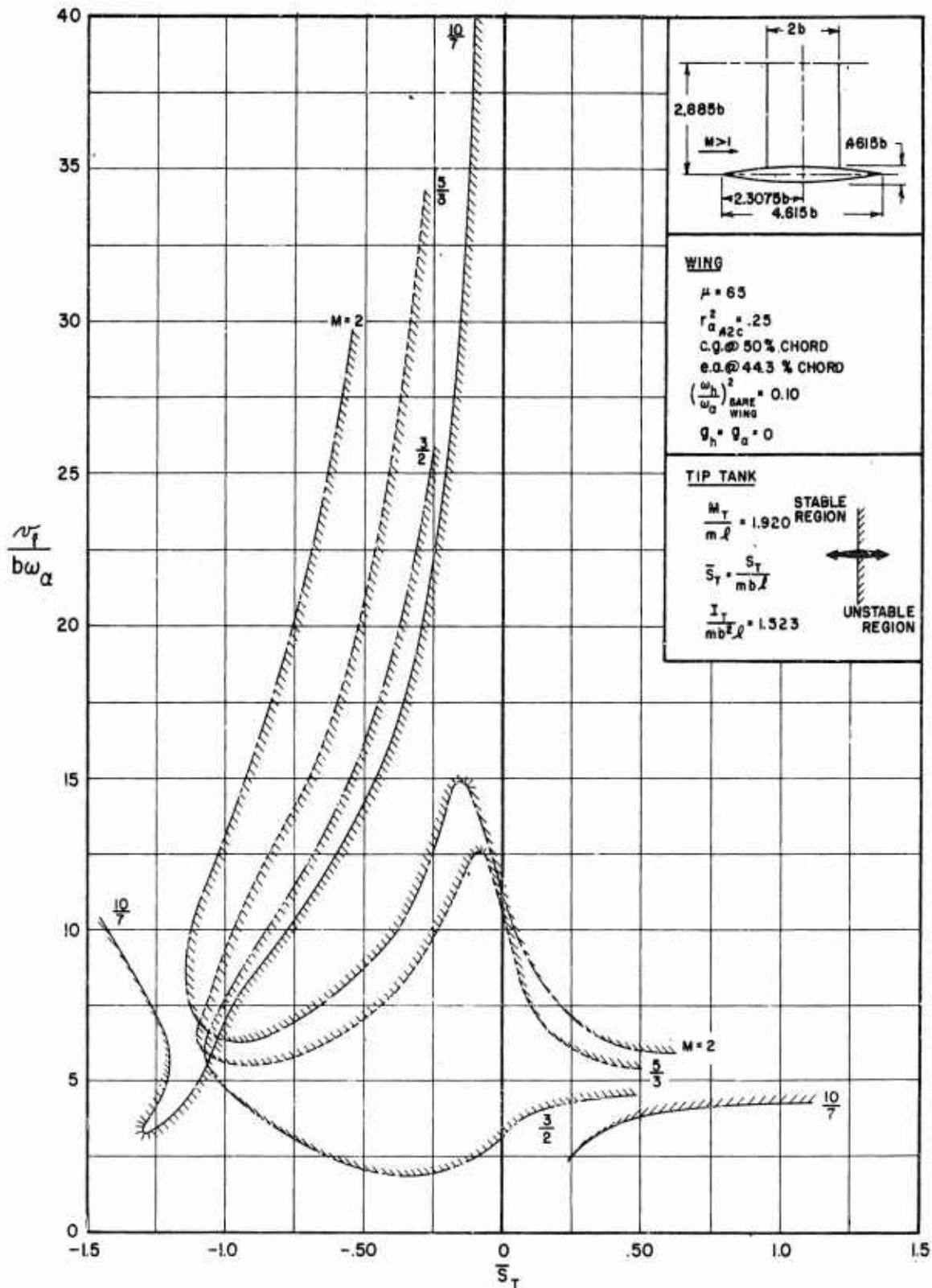
FIGURE C.7(a) FLUTTER COEFFICIENT VERSUS TIP-TANK STATIC-UNBALANCE PARAMETER FOR STRAIGHT-WING PLANFORM, FREE-TO-ROLL
