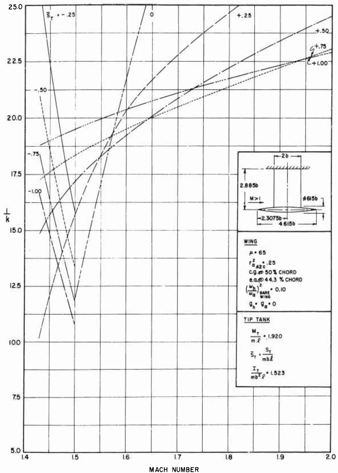
FIGURE 3.13 (Continued) THEORETICAL RESULTS FOR STRAIGHT WING WITH TIP TANK, NO STRUCTURAL DAMPING
