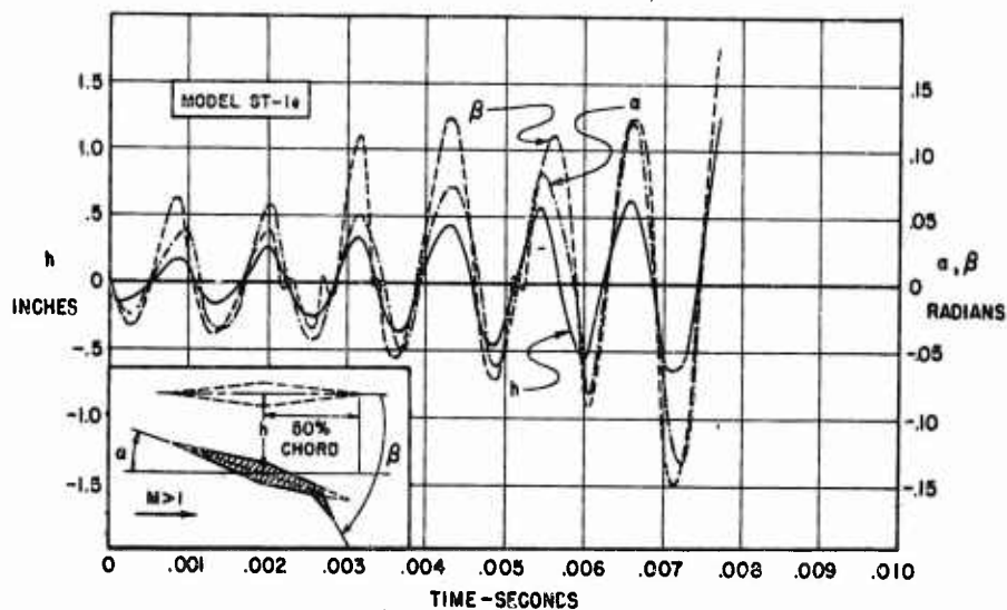
(a) Straight Wing with Free Aileron, Cantilever
