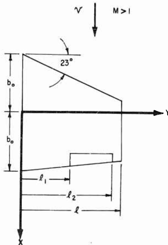
(a) Plan View of Wing
