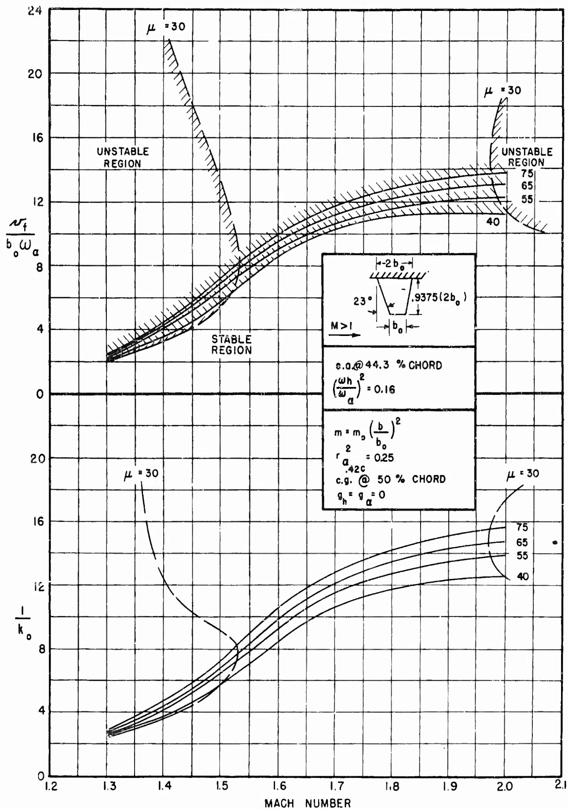
FIGURE 3.1(e) THEORETICAL RESULTS FOR BARE STRAIGHT-WING PLAN-FORM, e.a. AT 44.3% CHORD, (\frac{\omega_h}{\omega_a})^2 = 0.16
