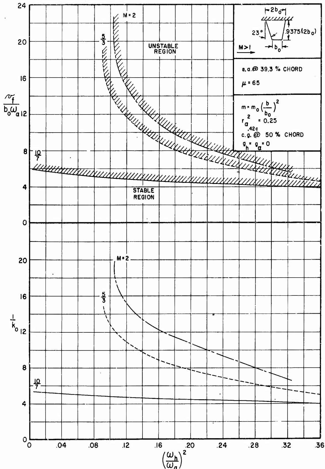
FIGURE C.1(c) FLUTTER COEFFICIENT AND REDUCED FREQUENCY VERSUS FREQUENCY RATIO FOR BARE STRAIGHT-WING PLANFORM, e.a. AT 39.3% CHORD, \mu = 65
