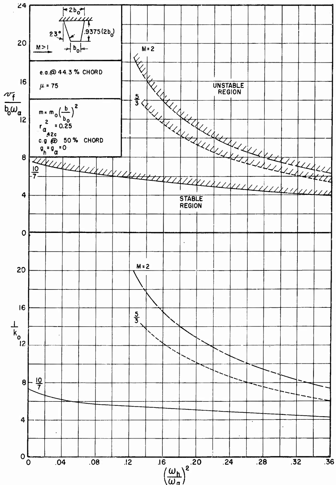
FIGURE C.1(d) FLUTTER COEFFICIENT AND REDUCED FREQUENCY VERSUS FREQUENCY RATIO FOR BARE STRAIGHT-WING PLANFORM, e.a. AT 39.3% CHORD, \mu = 75
