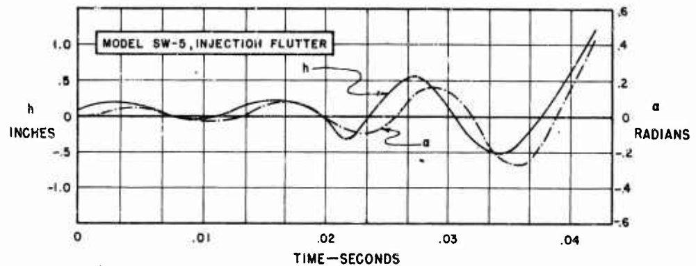
(e) Bare Swept Wing, Cantilever (Injection Flutter)
