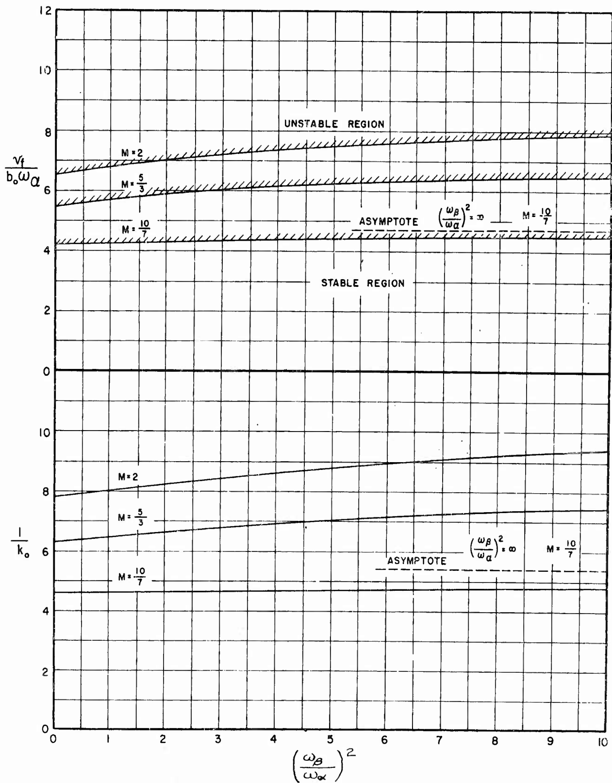
FIGURE C.2 FLUTTER COEFFICIENT AND REDUCED FREQUENCY VERSUS FREQUENCY RATIO FOR STRAIGHT WING WITH AILERON
