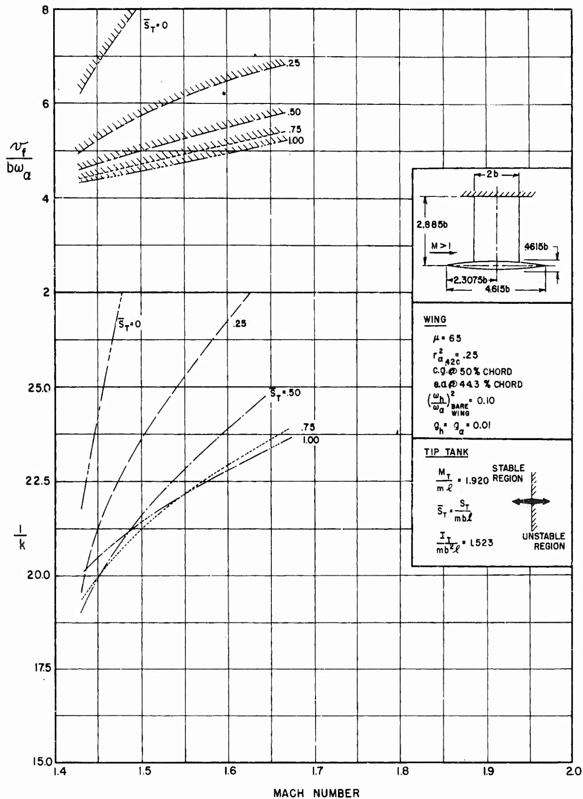
FIGURE 3.14 THEORETICAL RESULTS FOR CANTILEVER STRAIGHT WING WITH TIP TANK, STRUCTURAL DAMPING INCLUDED
