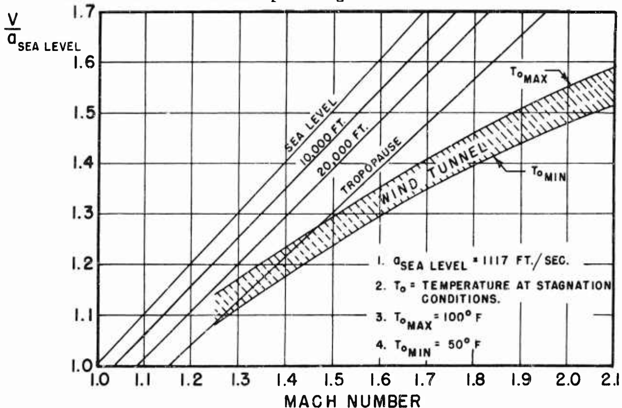
FIGURE 3.2 VELOCITY VERSUS MACH NUMBER FOR EXTREME RANGES OF ATMOSPHERIC AND WIND TUNNEL CONDITIONS
