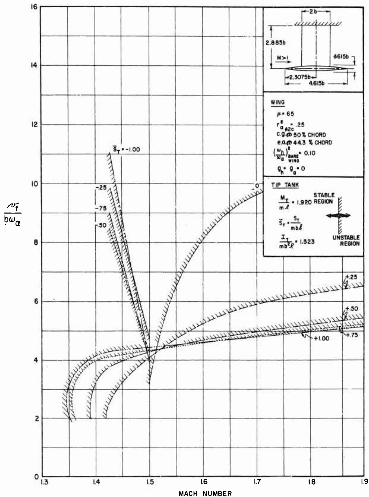
FIGURE 3.13 THEORETICAL RESULTS FOR STRAIGHT WING WITH TIP TANK, NO STRUCTURAL DAMPING
