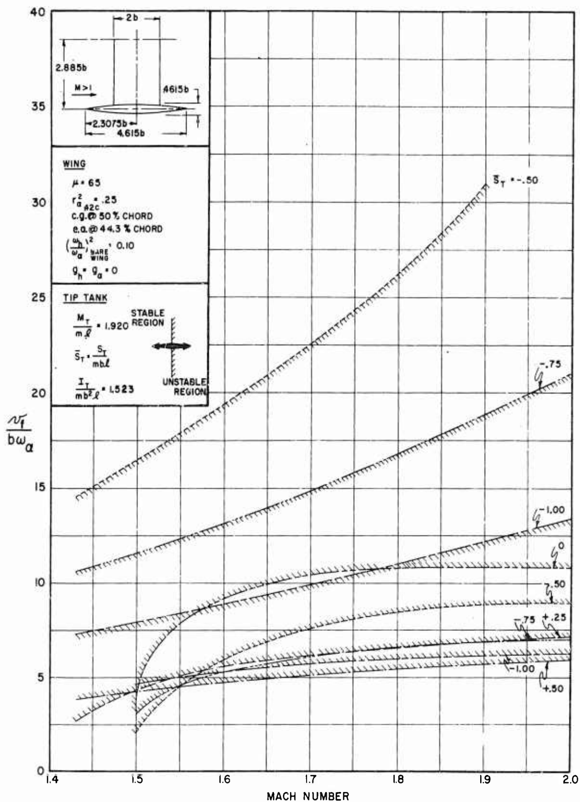
FIGURE 3.15 THEORETICAL RESULTS FOR STRAIGHT WING WITH TIP TANK, FREE TO ROLL
