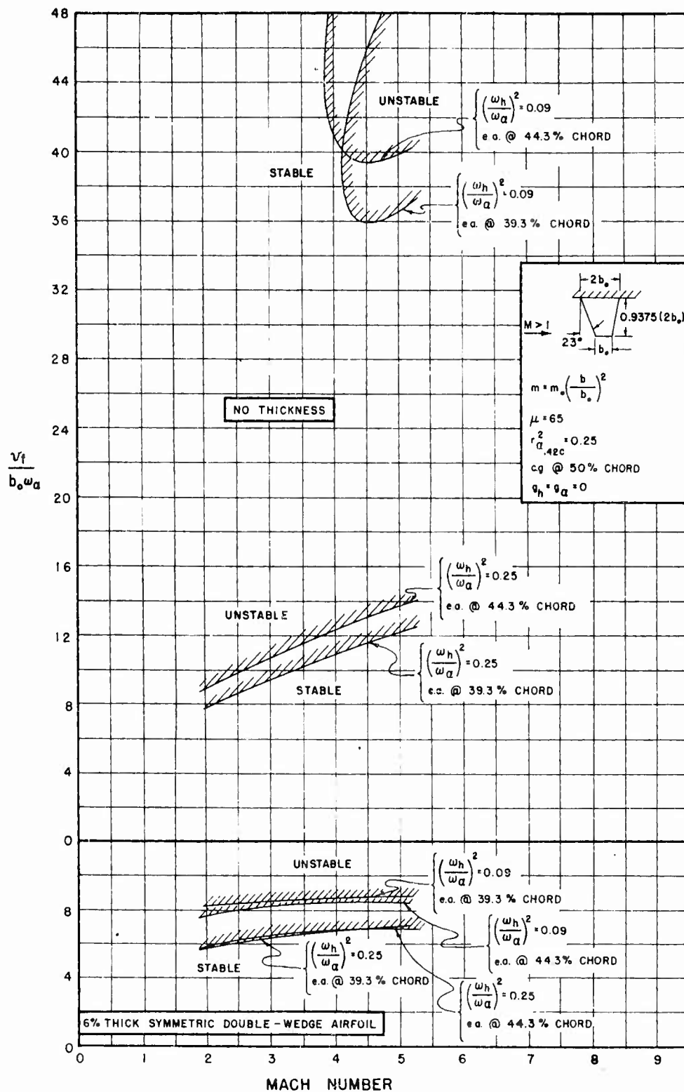
FIGURE 3.6 THEORETICAL RESULTS FOR BARE STRAIGHT-WING PLANFORM BASED ON PISTON THEORY
