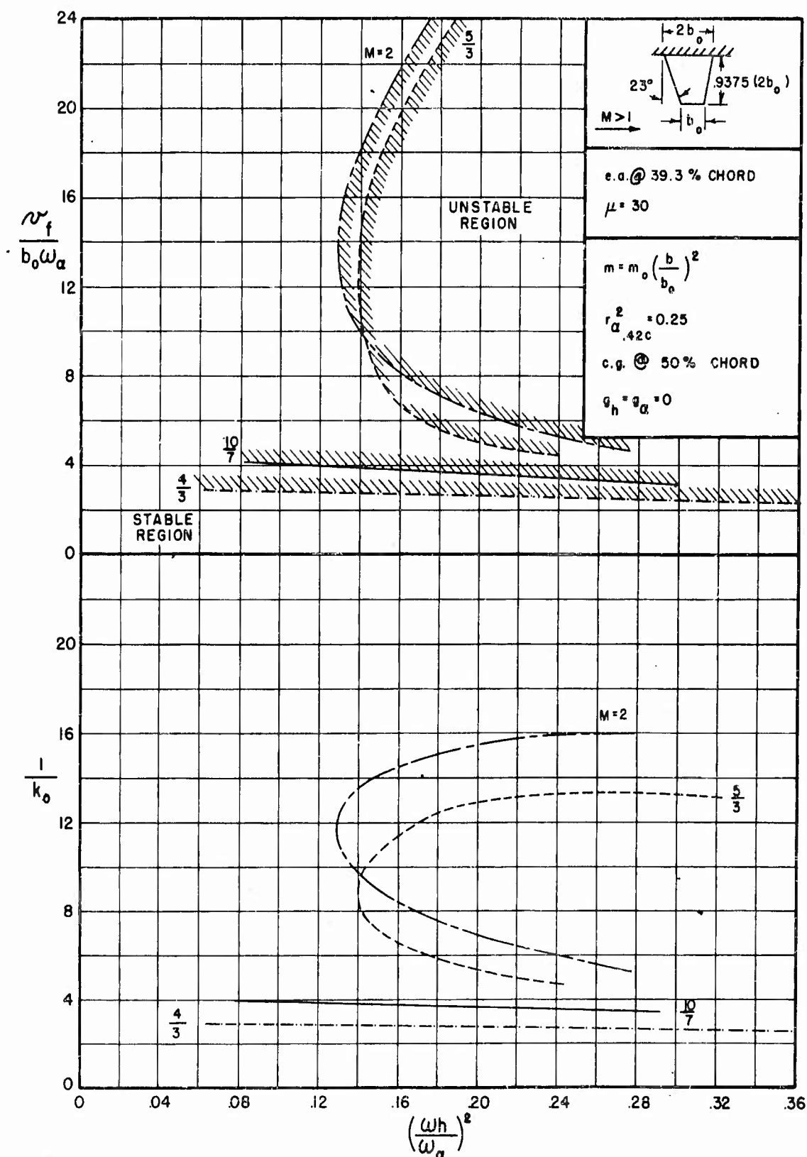
FIGURE C.1(a) FLUTTER COEFFICIENT AND REDUCED FREQUENCY VERSUS FREQUENCY RATIO FOR BARE STRAIGHT-WING PLANFORM, e.a. AT 39.3% CHORD, \mu = 30
