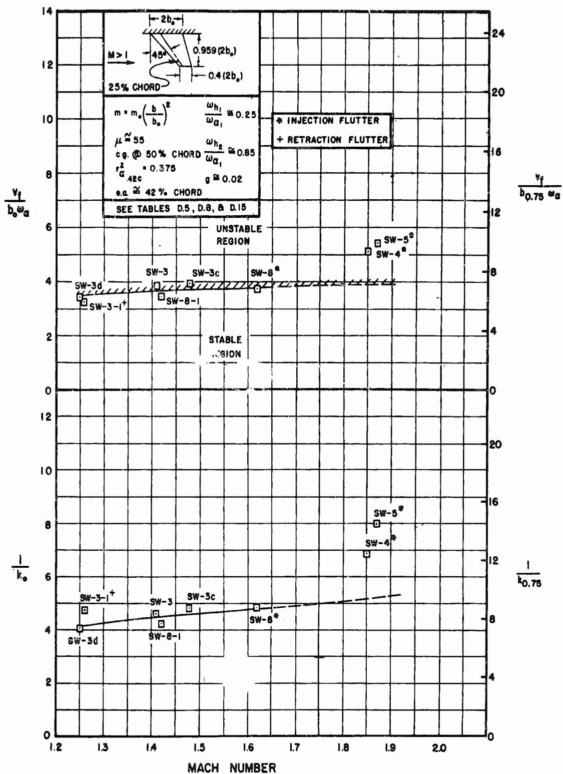
FIGURE 3.8 EXPERIMENTAL FLUTTER STABILITY BOUNDARY FOR BARE SWEPT-WING PLANFORM
