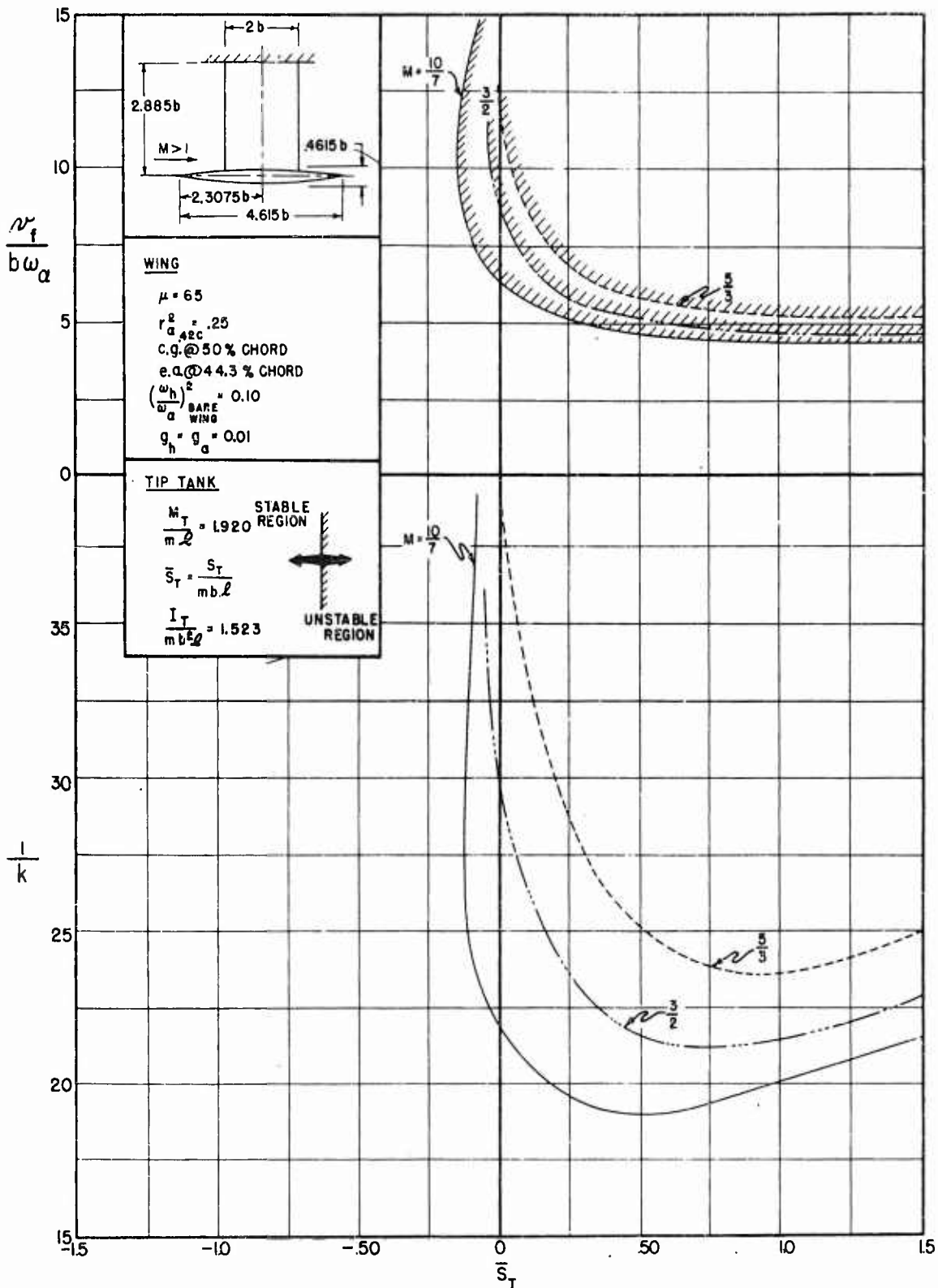
FIGURE C.5 FLUTTER COEFFICIENT AND REDUCED FREQUENCY VERSUS TIP TANK STATIC-UNBALANCE PARAMETER FOR STRAIGHT-WING PLANFORM, STRUCTURAL DAMPING INCLUDED
