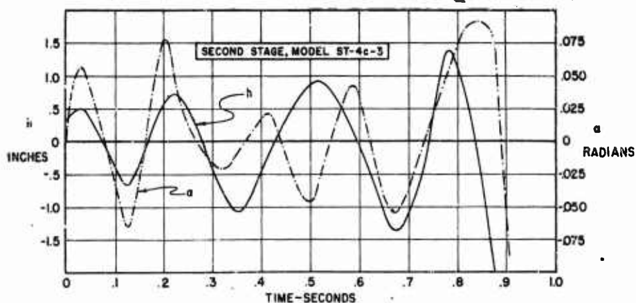
(c) Straight Wing with Tip Tank, Free-to-Roll (Second Stage)
