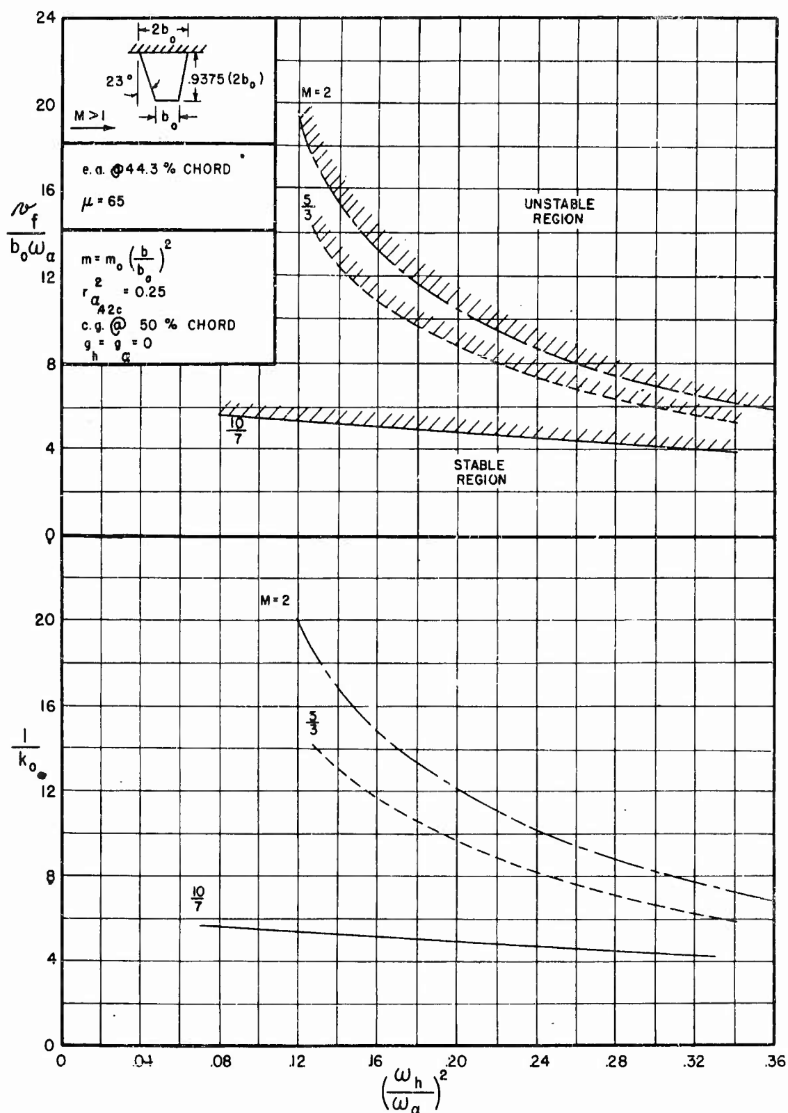
FIGURE C.1(h) FLUTTER COEFFICIENT AND REDUCED FREQUENCY VERSUS FREQUENCY RATIO FOR BARE STRAIGHT-WING PLANFORM, e.a. AT 44.3% CHORD, \mu = 65
