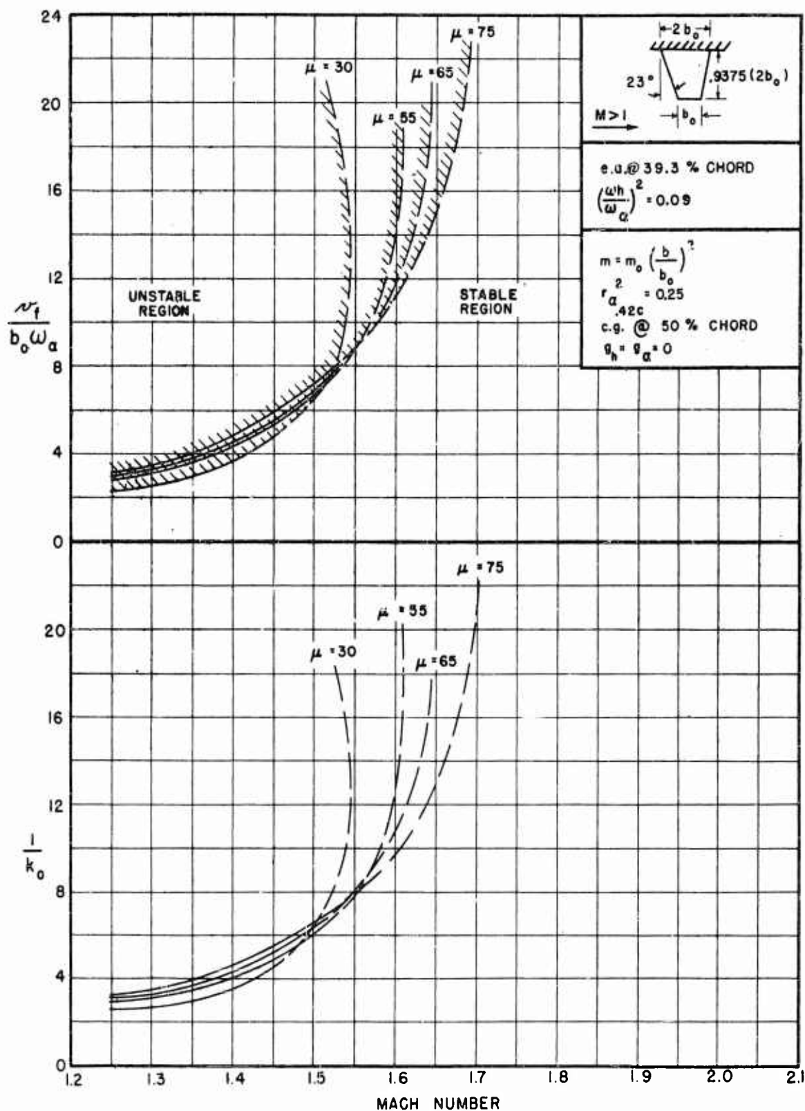
FIGURE 3.1(a) THEORETICAL RESULTS FOR BARE STRAIGHT-WING PLAN-FORM, e.a. AT 39.3% CHORD, \left(\frac{\omega_h}{\omega_a}\right)^2 = 0.09
