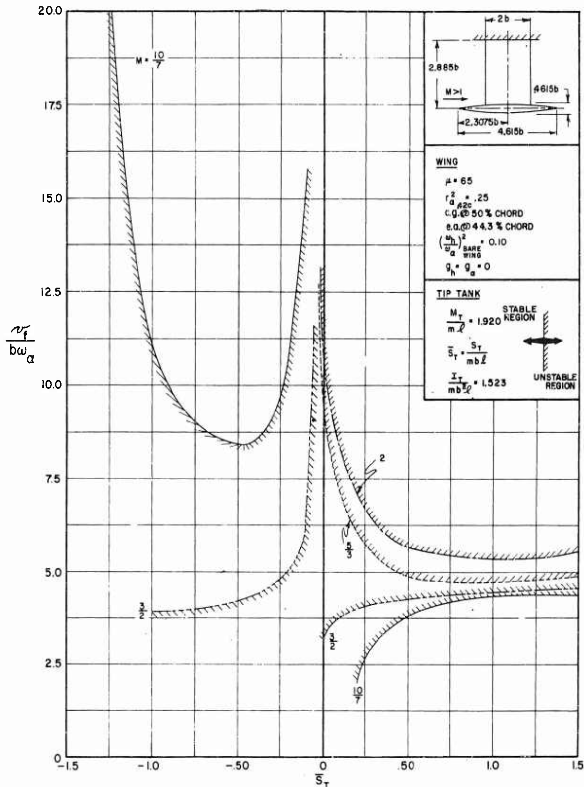
FIGURE C.4(a) FLUTTER COEFFICIENT VERSUS TIP-TANK STATIC-UNBALANCE PARAMETER FOR STRAIGHT-WING PLANFORM, NO STRUCTURAL DAMPING
