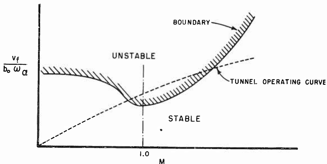
FIGURE 1.2 HYPOTHETICAL FLUTTER BOUNDARY
