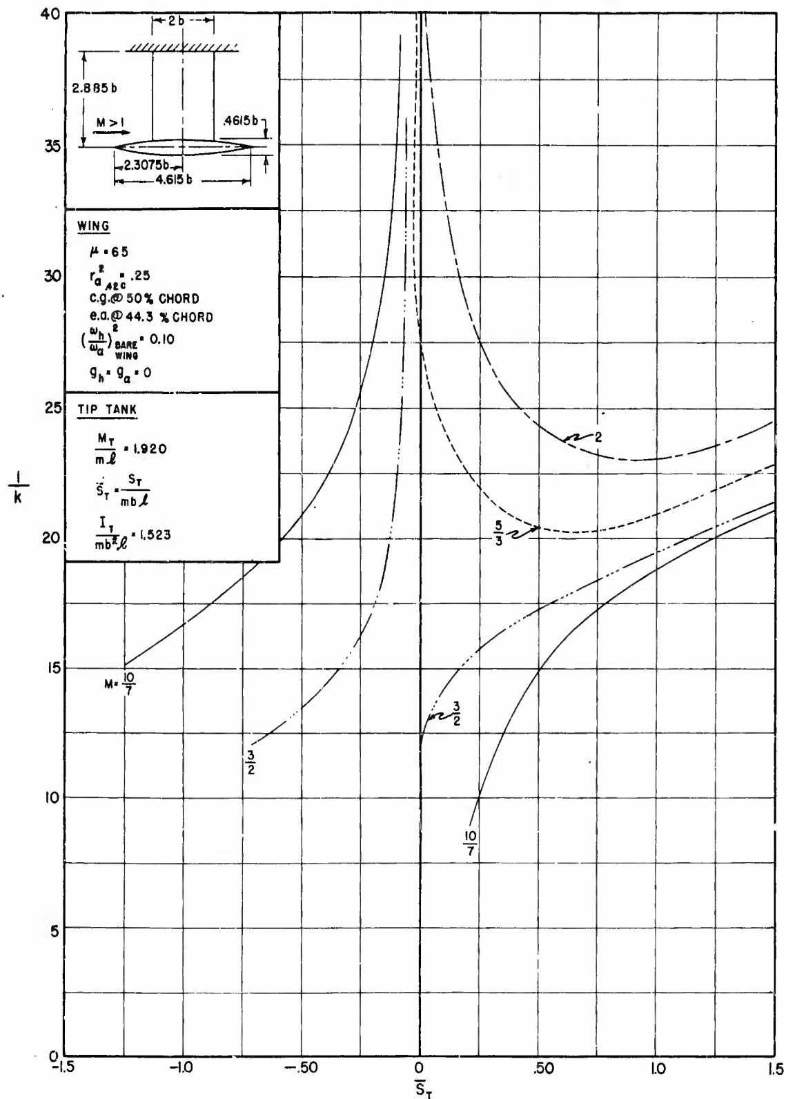
FIGURE C.4(b) REDUCED FREQUENCY VERSUS TIP-TANK STATIC-UNBALANCE PARAMETER FOR STRAIGHT-WING PLANFORM, NO STRUCTURAL DAMPING
