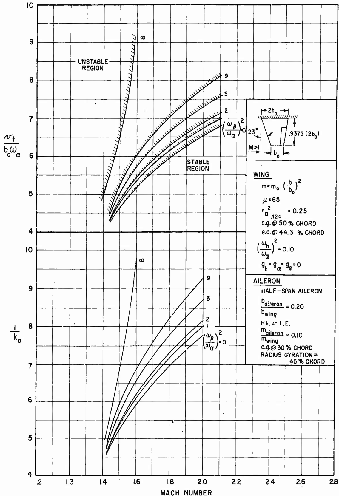
FIGURE 3.12 THEORETICAL RESULTS FOR STRAIGHT WING WITH AILERON
