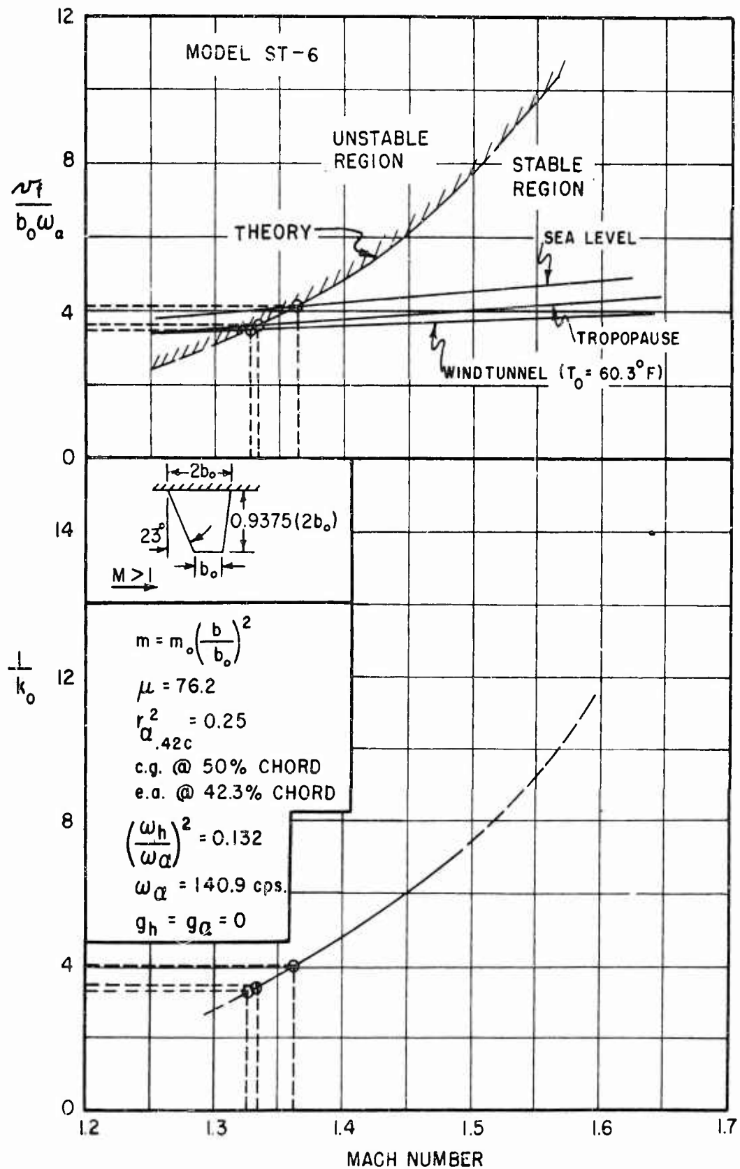
FIGURE 3.3 EXAMPLE USE OF THEORETICAL CURVES
