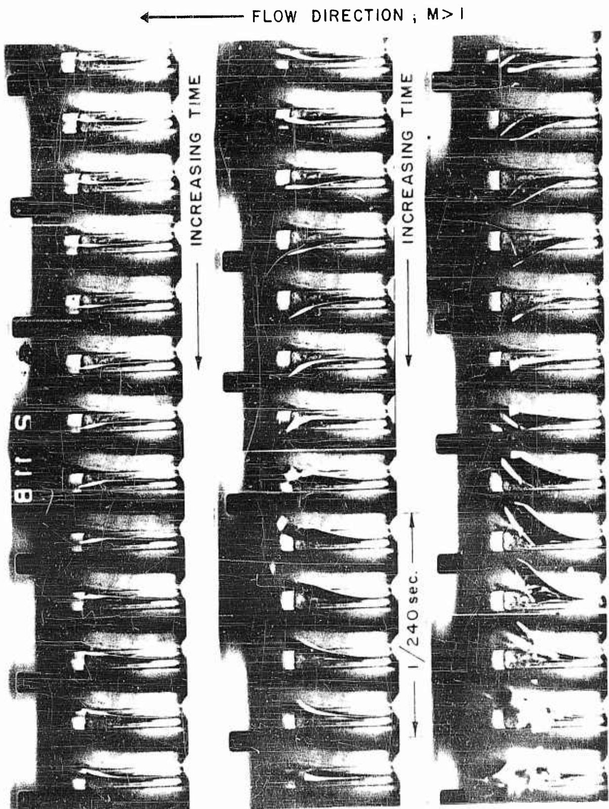
(e) Bare Swept Wing, Cantilever (Model SW-5, Injection Flutter) FIGURE D.3 (Continued) SOME HIGH-SPEED MOVIES AT SUPERSONIC FLUTTER
