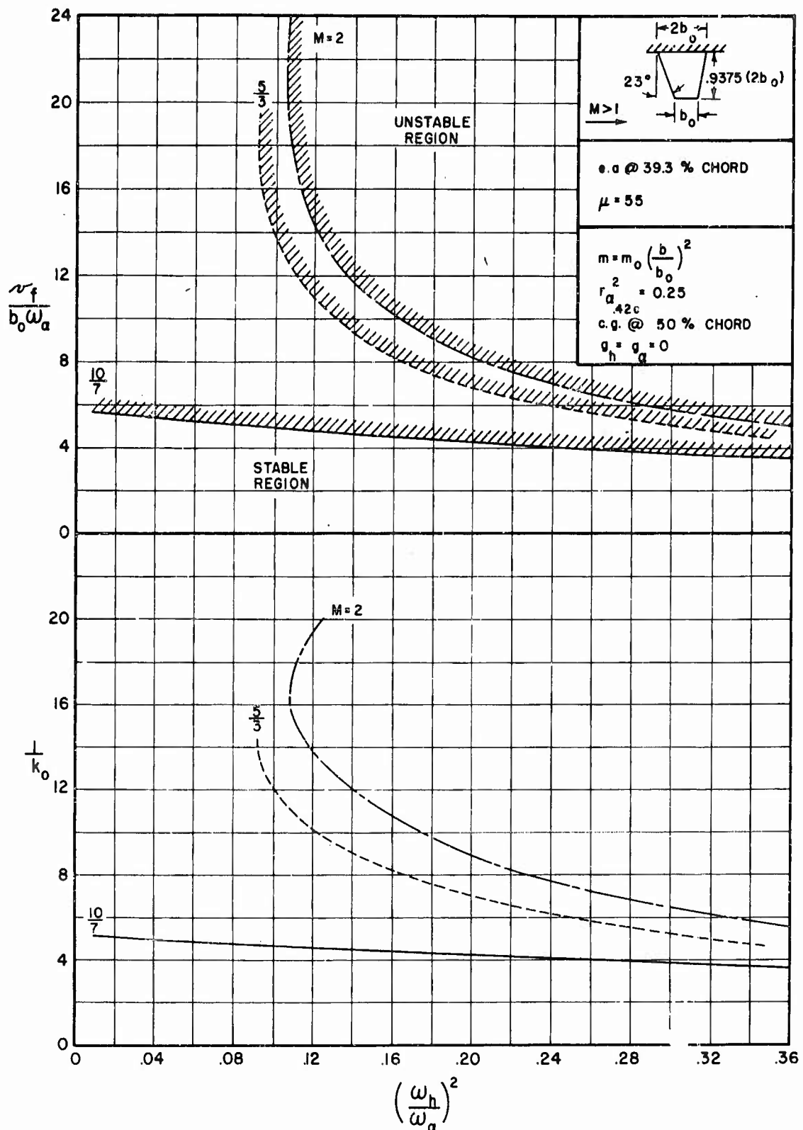
FIGURE C.1(b) FLUTTER COEFFICIENT AND REDUCED FREQUENCY VERSUS FREQUENCY RATIO FOR BARE STRAIGHT-WING PLANFORM, e.a. AT 39.3% CHORD, \mu = 55
