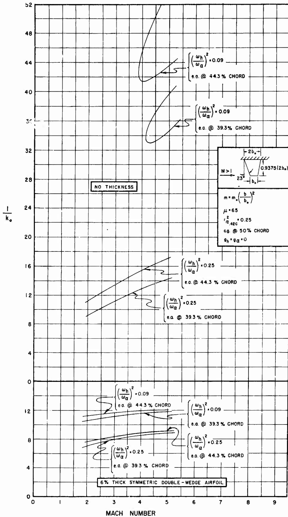
FIGURE 3.6 (Continued) THEORETICAL RESULTS FOR BARE STRAIGHT-WING PLANFORM BASED ON PISTON THEORY
