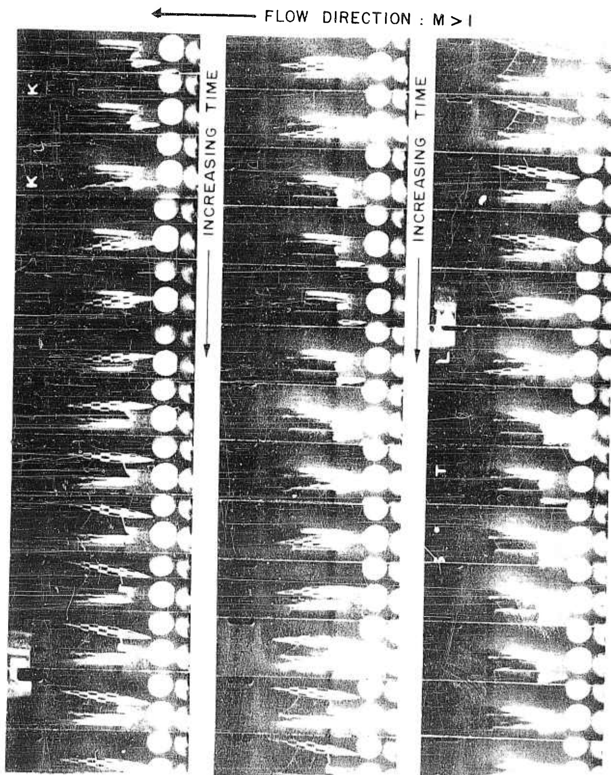
(c) Straight wing with Tip Tank, Free-to-Roll (Second Stage, Model ST-4c-3)
