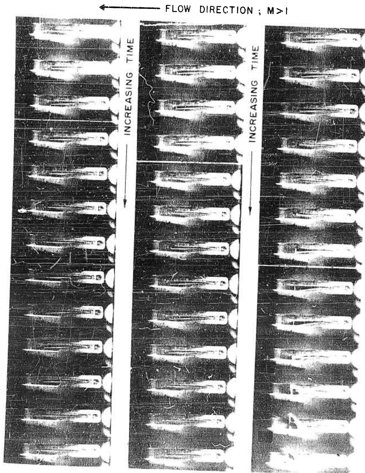
(g) Bare Delta Wing, Cantilever (Model De-4c) FIGURE D.3 (Continued) SOME HIGH-SPEED MOVIES AT SUPERSONIC FLUTTER
