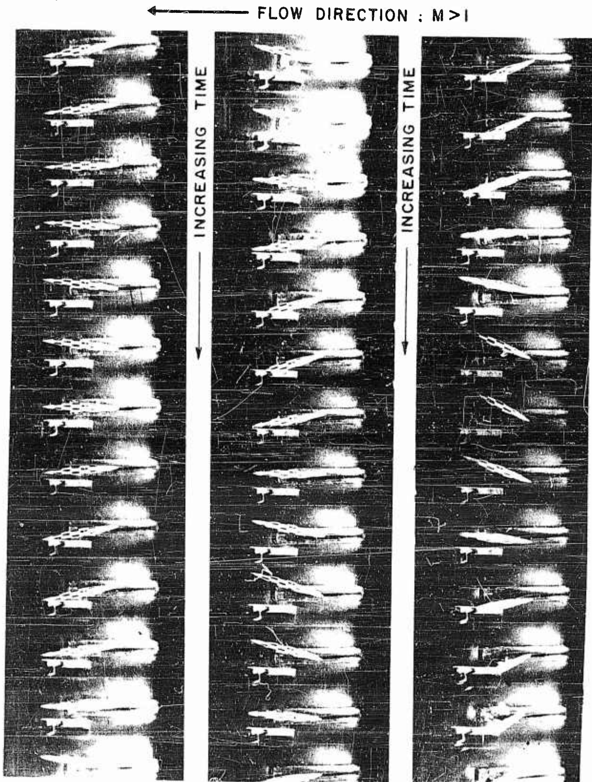
(f) Swept Wing with Tip Tank, Cantilever (Model SW-6)
