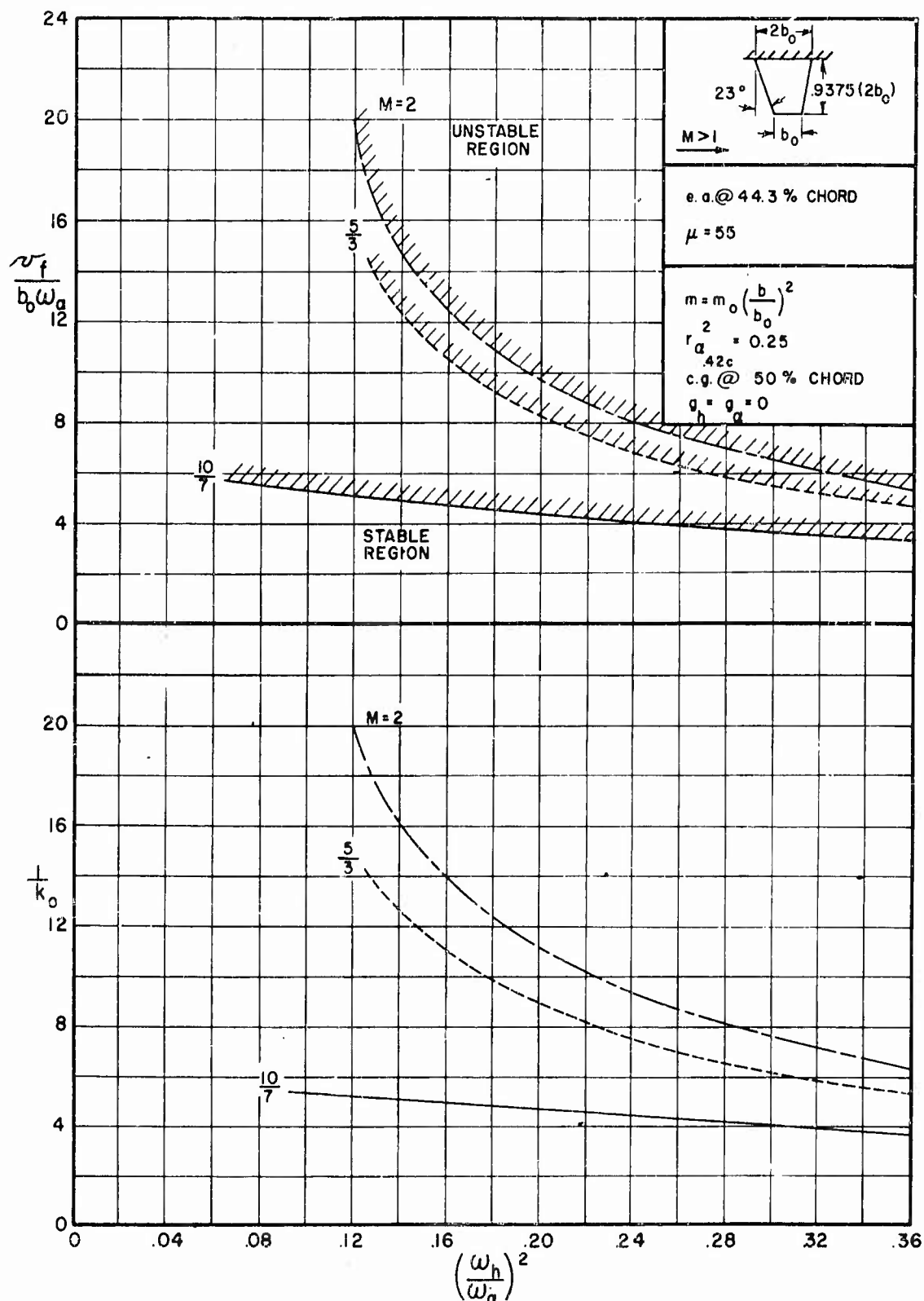
FIGURE C.1(g) FLUTTER COEFFICIENT AND REDUCED FREQUENCY VERSUS FREQUENCY RATIO FOR BARE STRAIGHT-WING PLANFORM, e.a. AT 44.3% CHORD, \mu = 55
