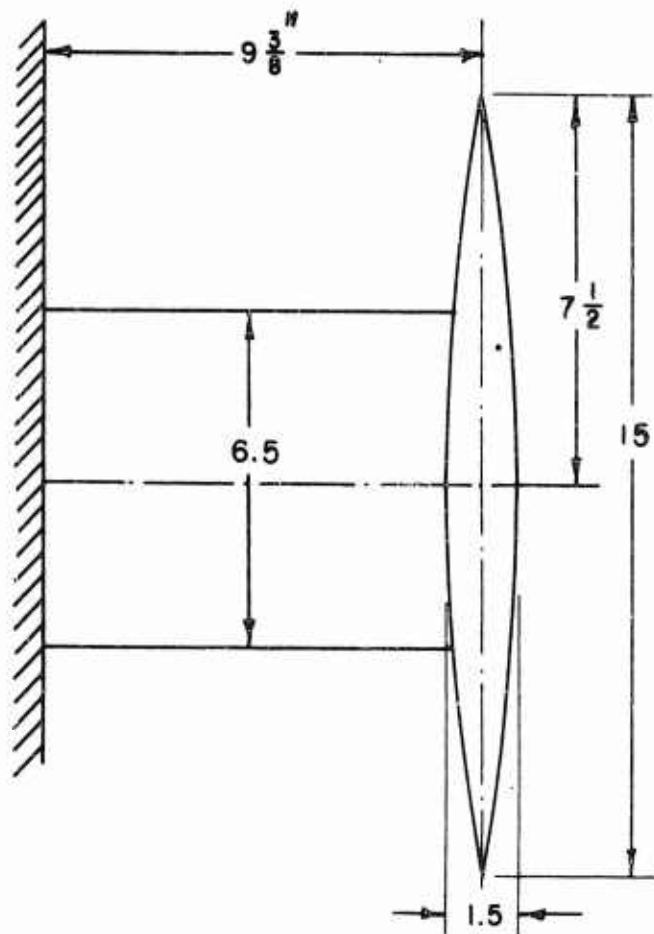
FIGURE C.3 TIP-TANK MODEL FOR CALCULATIONS
