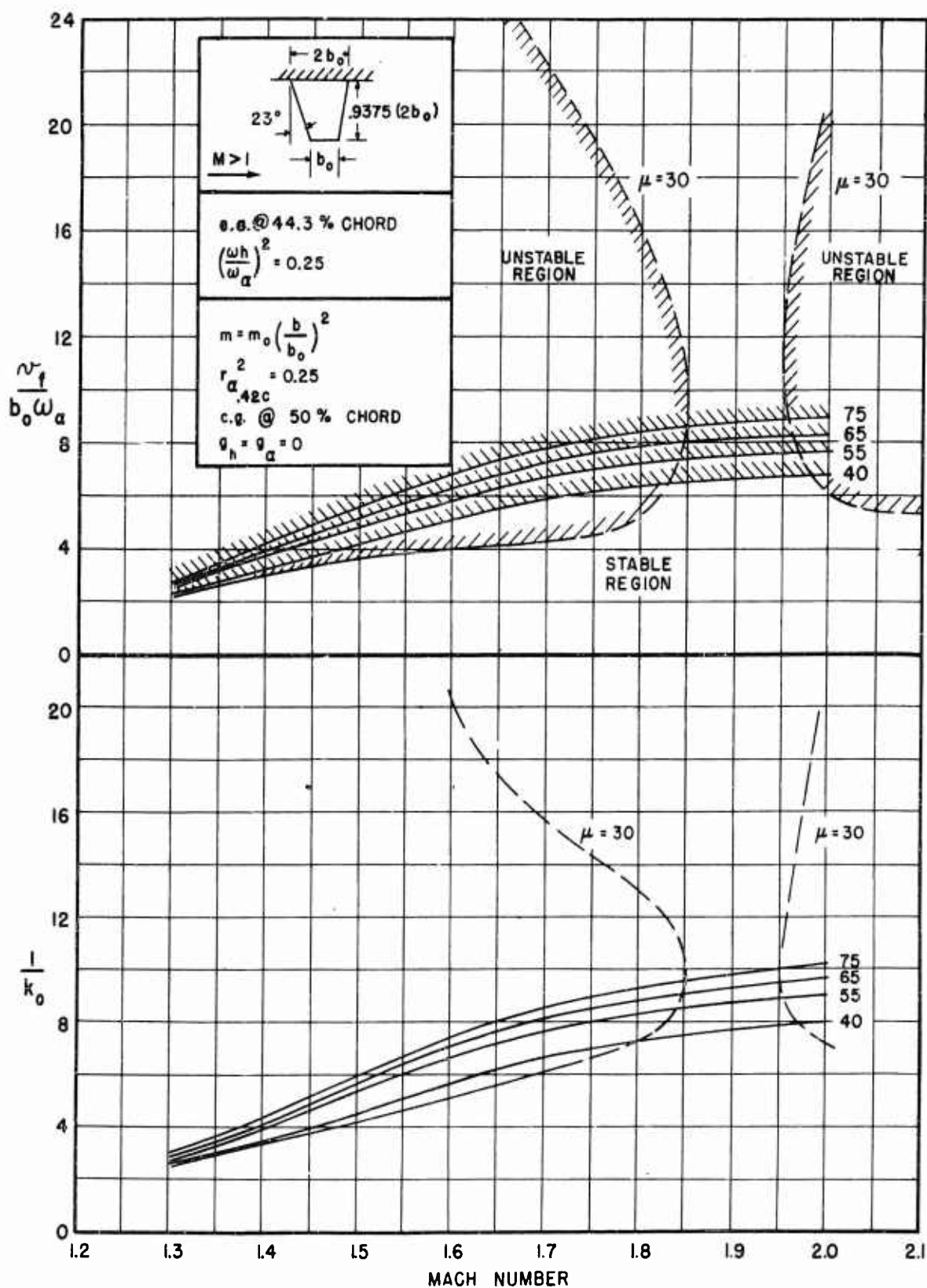
FIGURE 3.1(f) THEORETICAL RESULTS FOR BARE STRAIGHT-WING PLAN-FORM, e.a. AT 44.3% CHORD, (\frac{\omega_h}{\omega_a})^2 = 0.25
