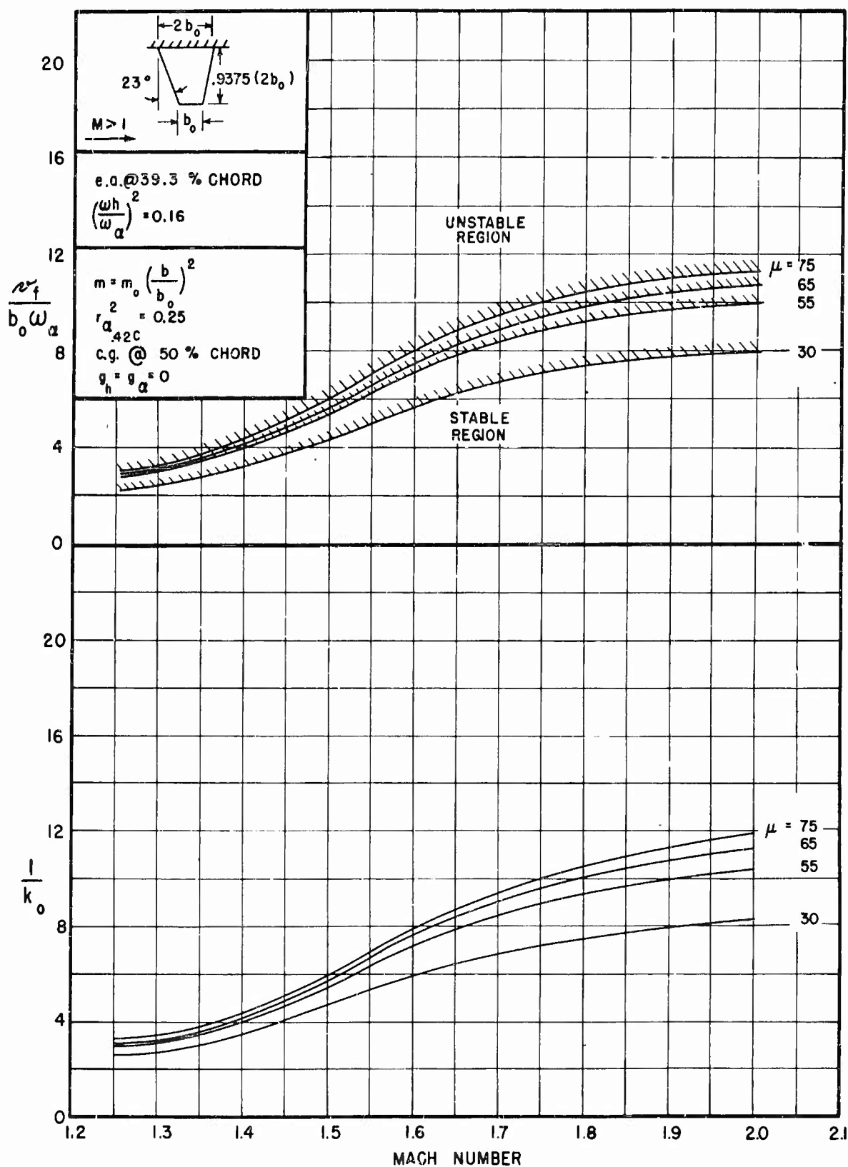
FIGURE 3.1(b) THEORETICAL RESULTS FOR BARE STRAIGHT-WING PLAN-FORM, e.a. AT 39.3% CHORD, (\frac{\omega_h}{\omega_a})^2 = 0.16
