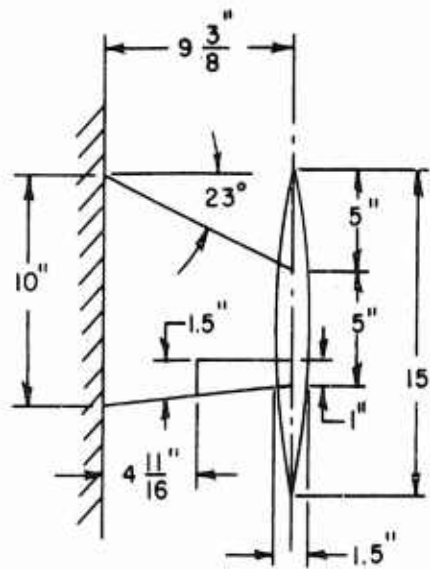
STRAIGHT WING
