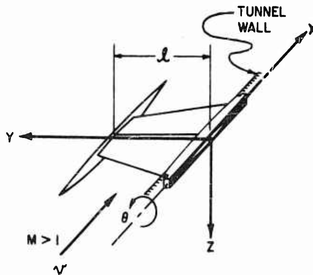
FIGURE A.2 AXIS SYSTEM FOR WING WITH TIP TANK
