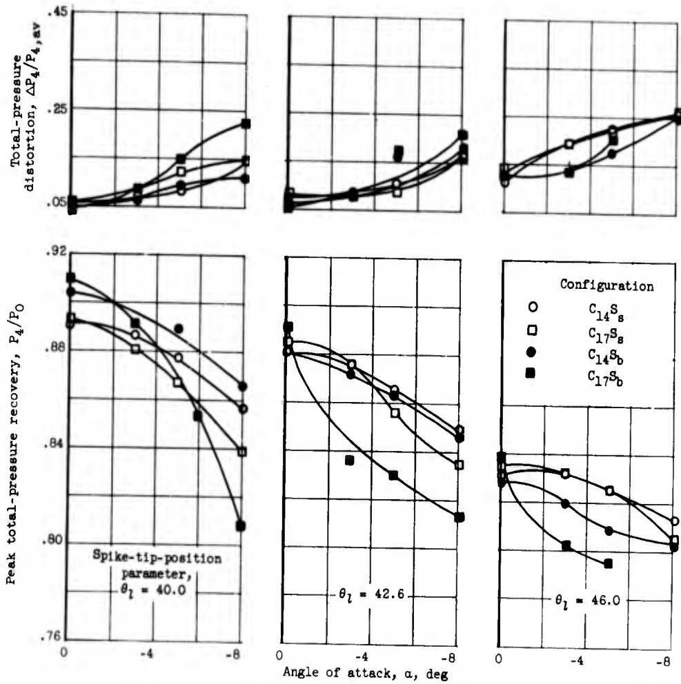
(a) Free-stream Mach number, 2.0.
