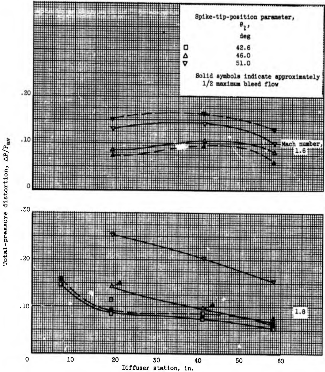
(b) Reduced Mach number; angle of attack, \alpha' .
