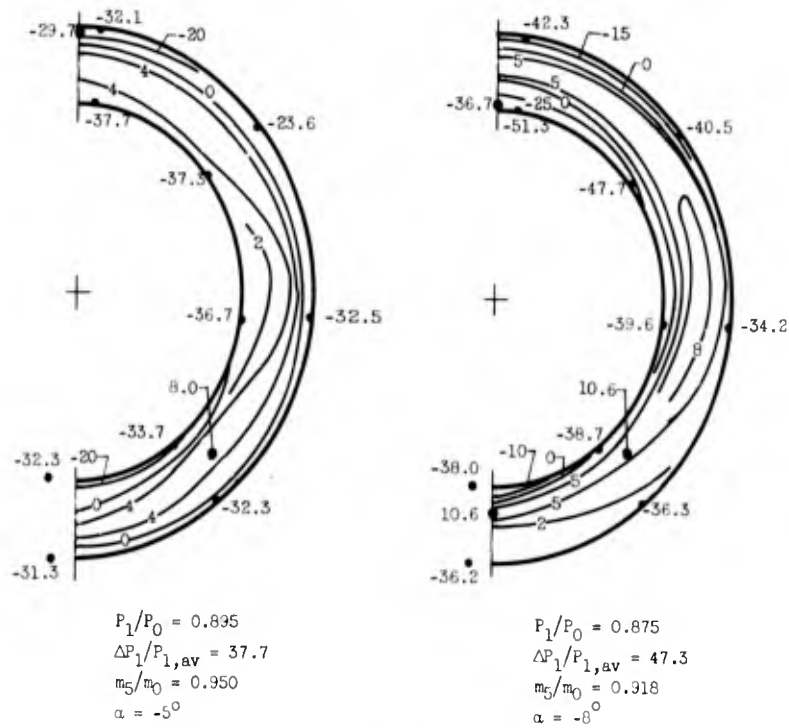
(a) Inlet C_{14}S_8 . Spike-tip-position parameter, 42.6^\circ .
