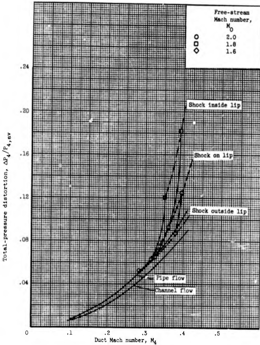
(a) Inlet C_{17S_8} ; angle of attack, 0^\circ .
