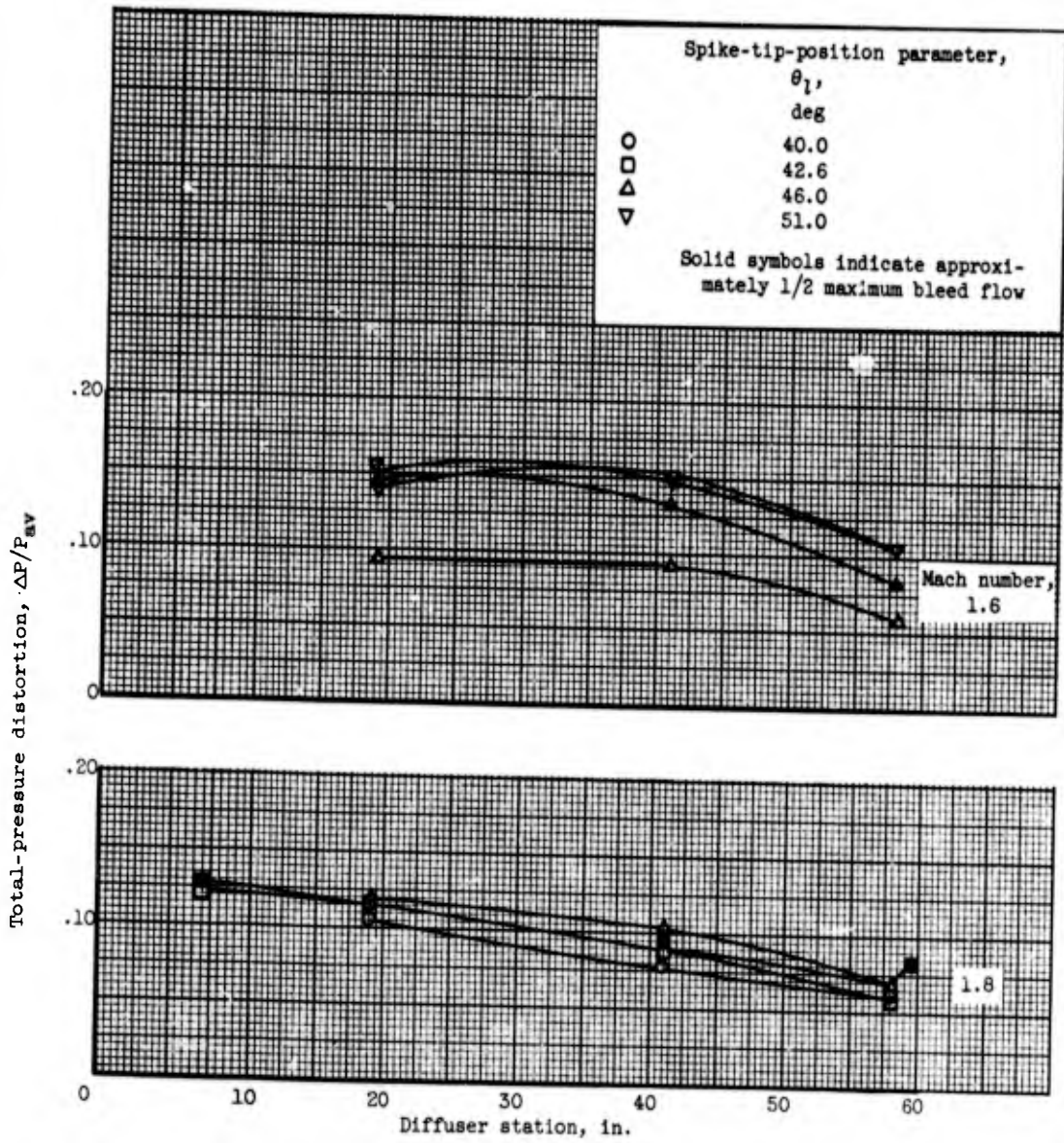
(b) Reduced Mach number; angle of attack, 0^\circ .
