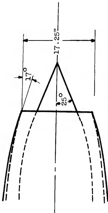
(a) Inlet C_{17S} .
