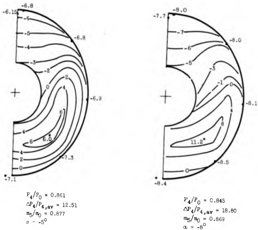
(c) Inlet C_{14}S_b with maximum bleed flow.
