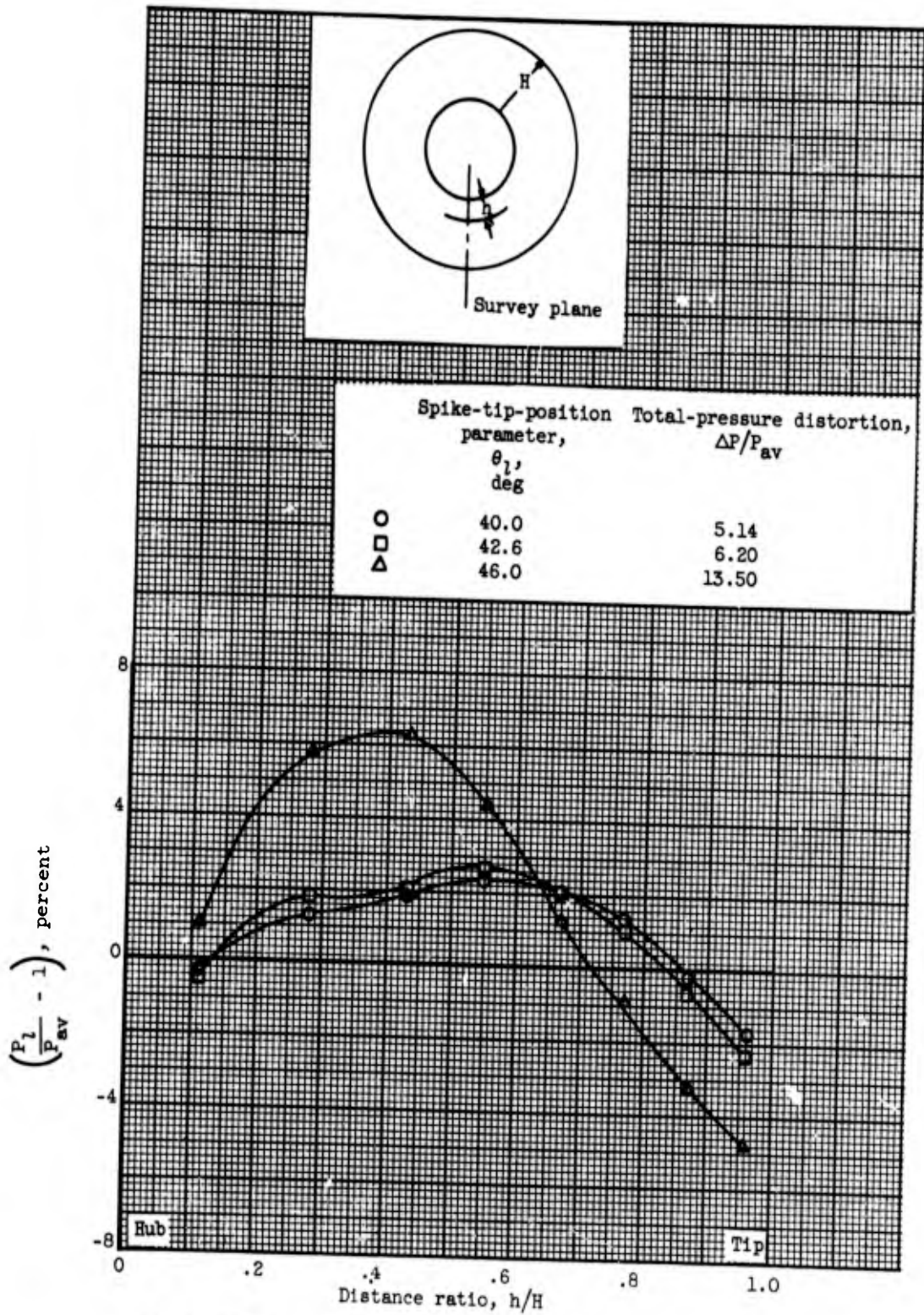
(b) Inlet C_{17}S_8 ; station 58. Free-stream Mach number, 2.0; angle of attack, 0^\circ .
