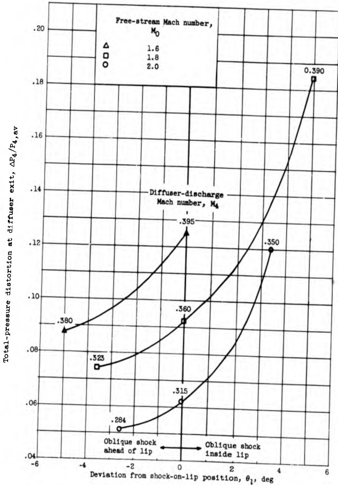
Figure 21. - Effect of oblique-shock location on distortion at diffuser exit. Inlet C_{17}S_8 ; angle of attack, 0^\circ .
