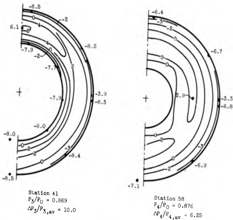
Figure 15. - Total-pressure contour development.
