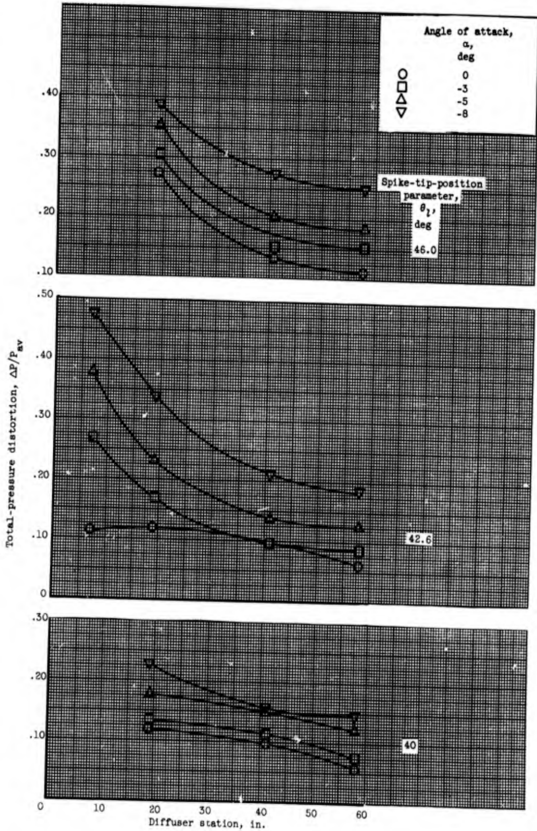
(a) Mach number, 2.0.
