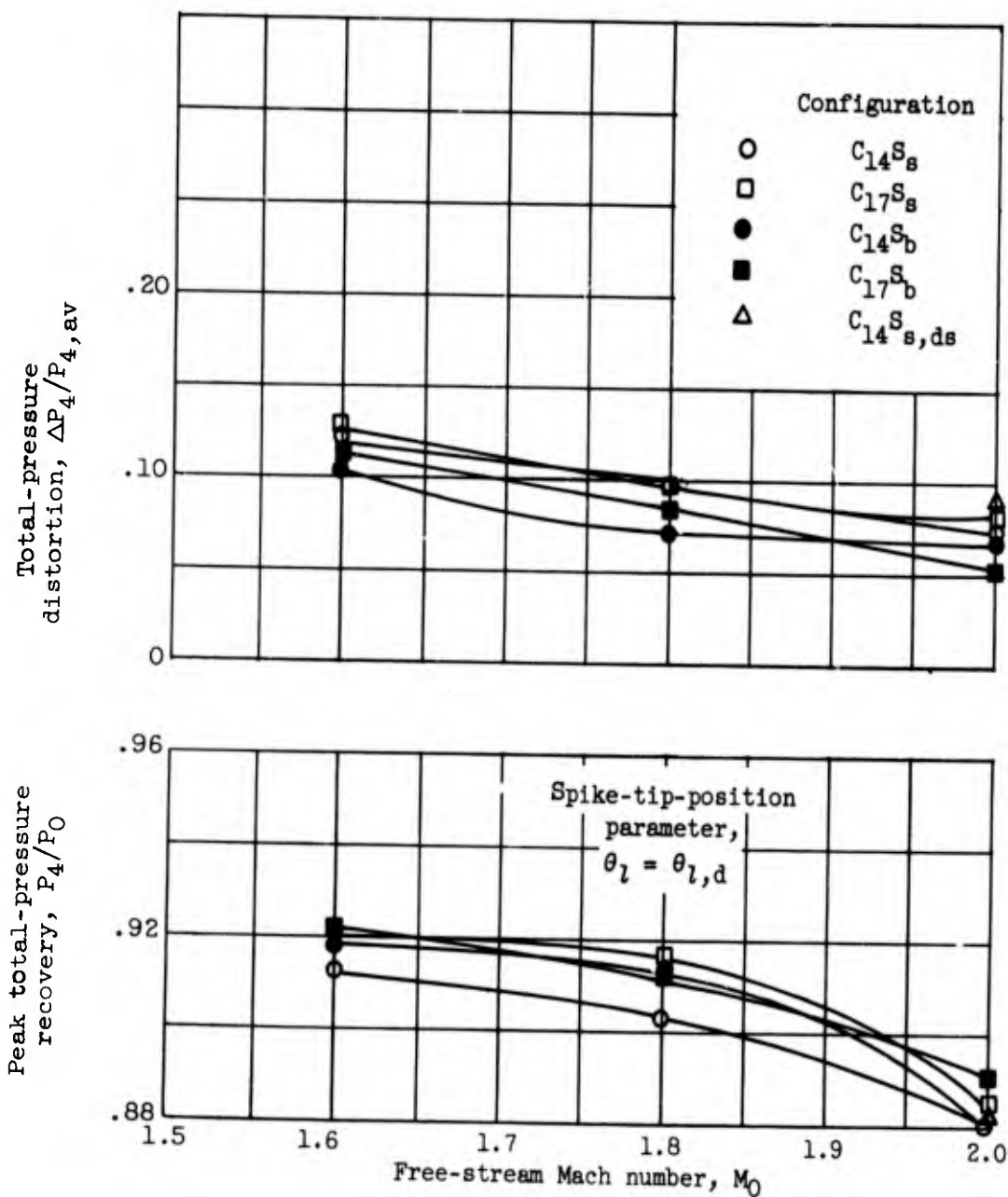
(b) Angle of attack, 0^\circ .
