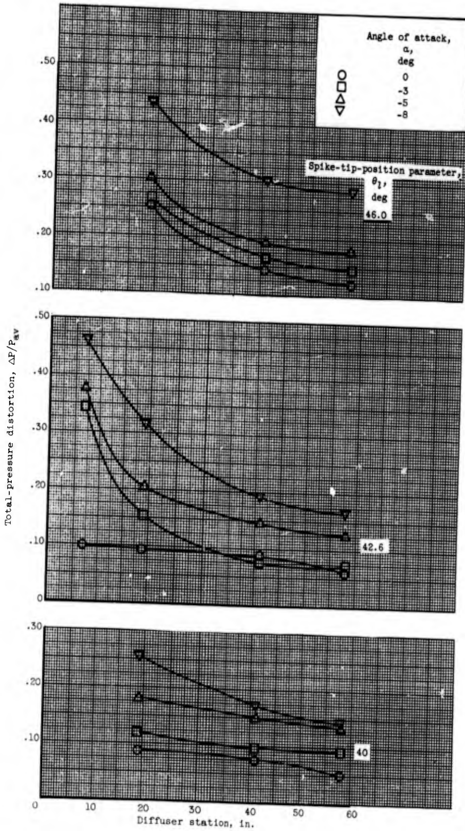
(a) Mach number, 2.0.
