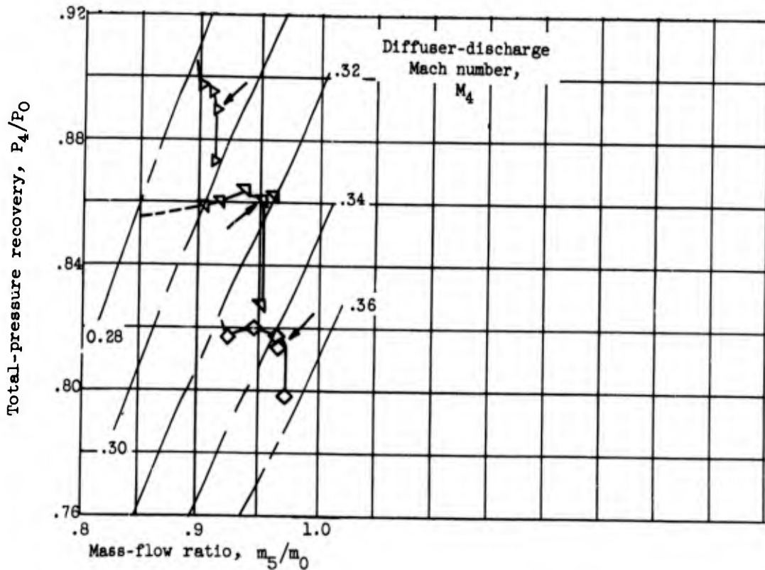
Figure 9. - Concluded. Performance of double-shock inlet C_{14}S_{s,ds} .
