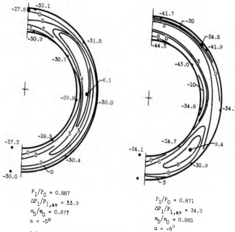
(c) Inlet C_{14}S_b . Spike-tip-position parameter, 42.6^\circ .
