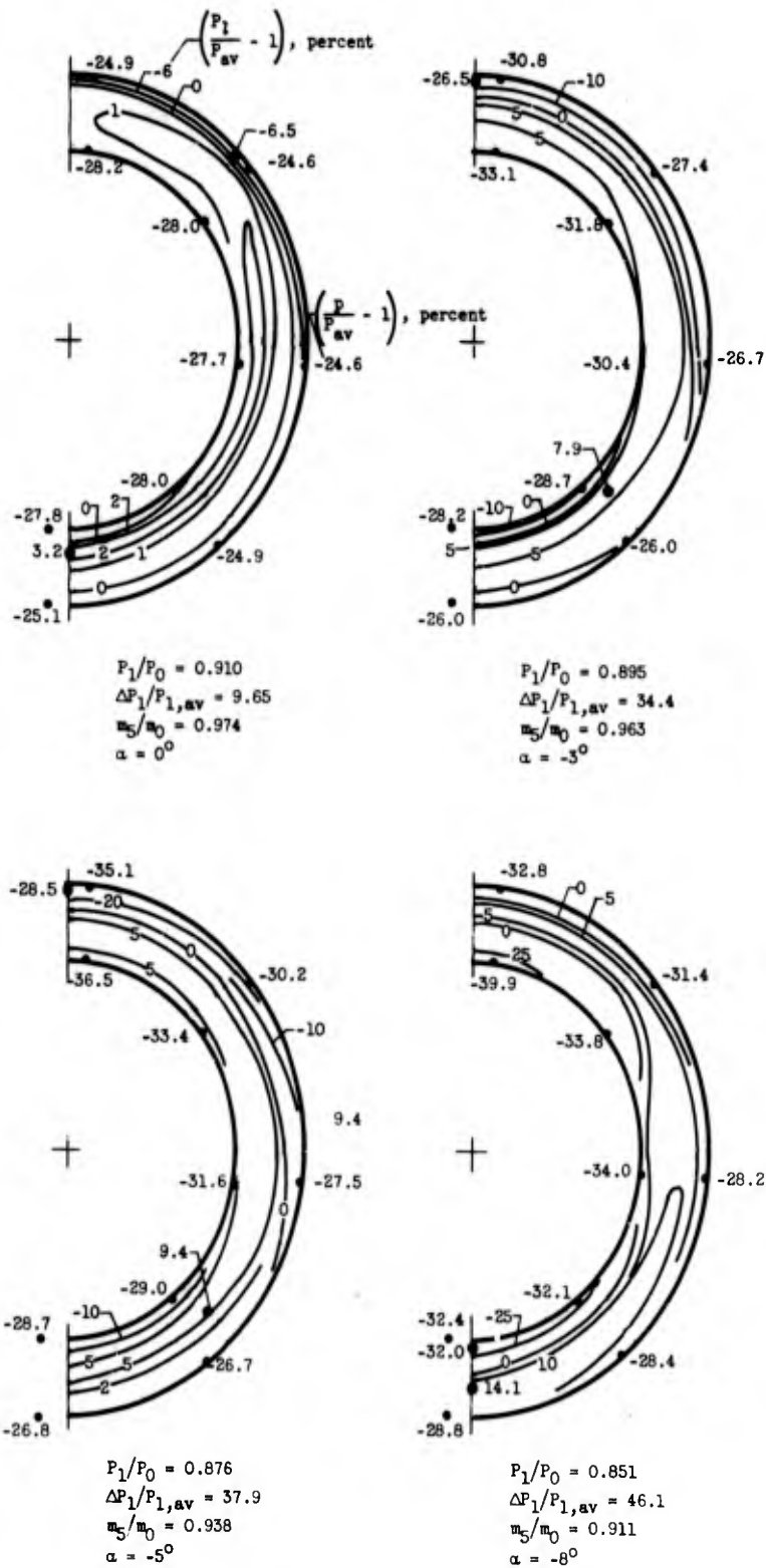
(b) Inlet C_{17S_8} . Spike-tip-position parameter, 42.6^\circ .
