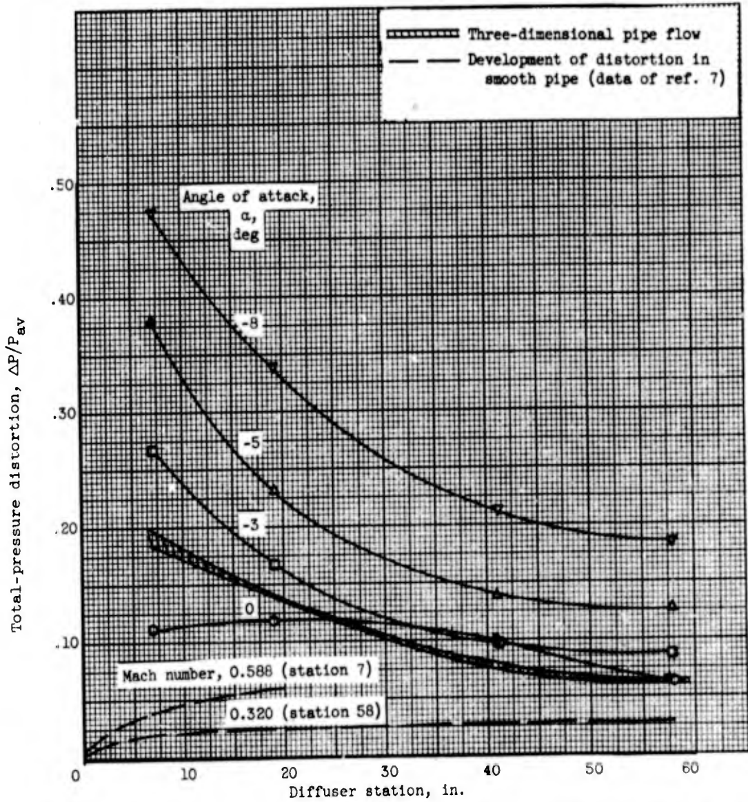
(b) Inlet C_{14}S_8 . Free-stream Mach number, 2.0; spike-tip-position parameter, 42.6.
