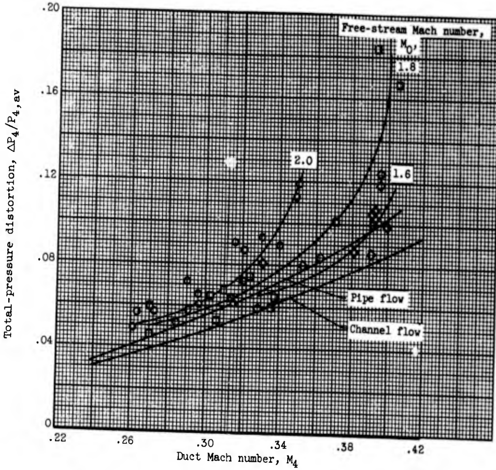
(b) Summary for all configurations.
