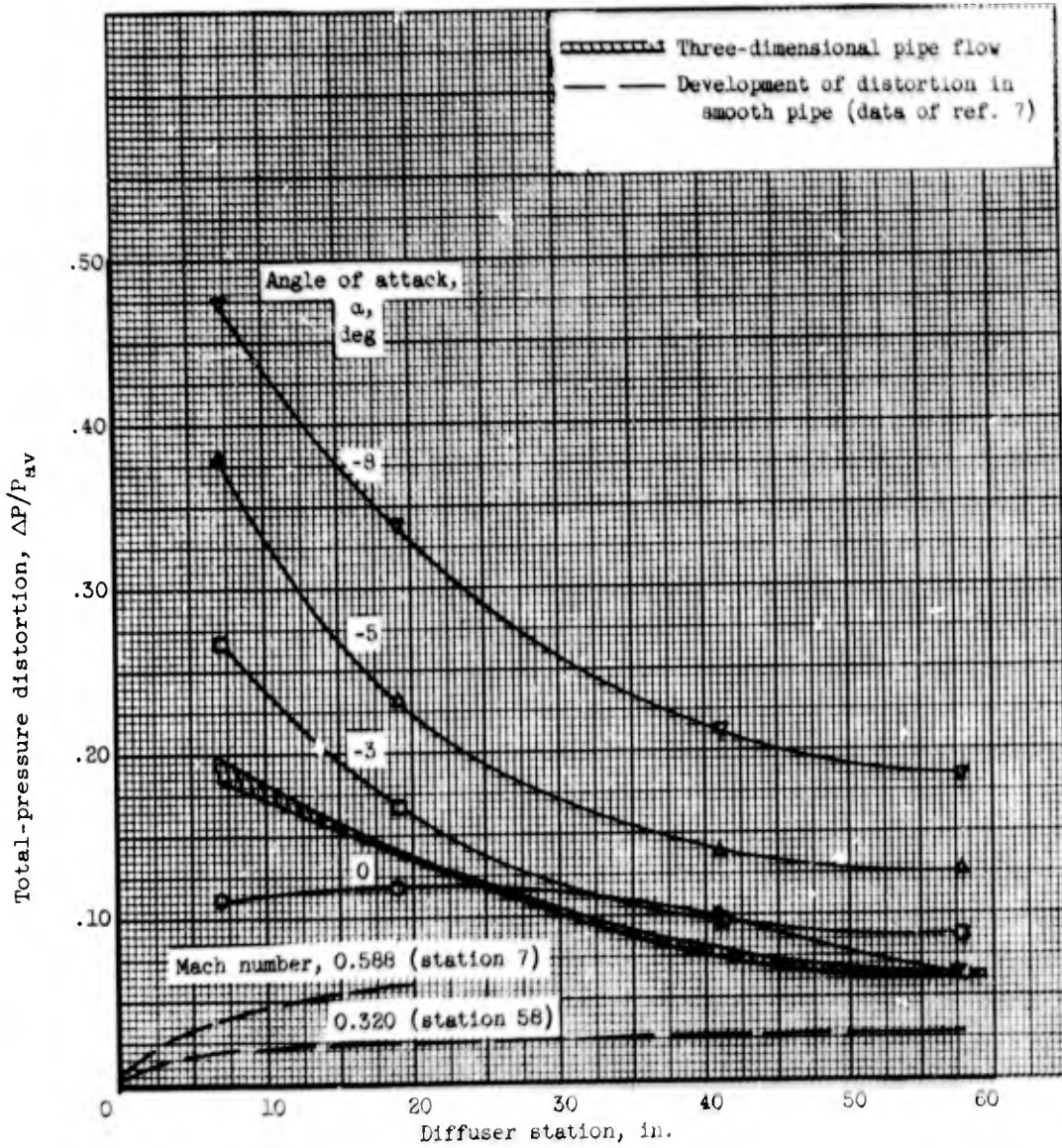
(b) Inlet C_{14}S_8 . Free-stream Mach number, 2.0; spike-tip-position parameter, 42.6.
