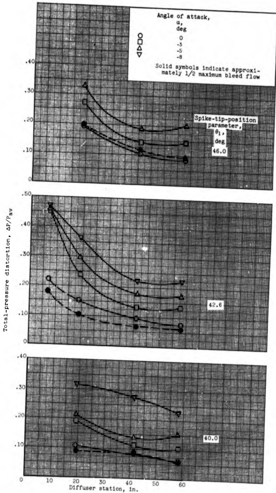
(a) Mach number, 2.0.
