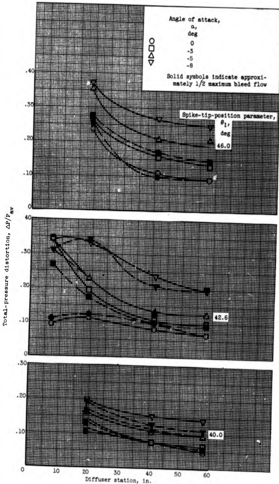
(a) Mach number, 2.0.
