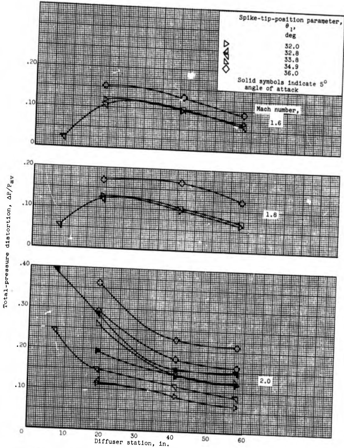
Figure 20. - Distortion in diffuser duct of inlet C_{14}S_{8,ds} for critical inlet operation.
