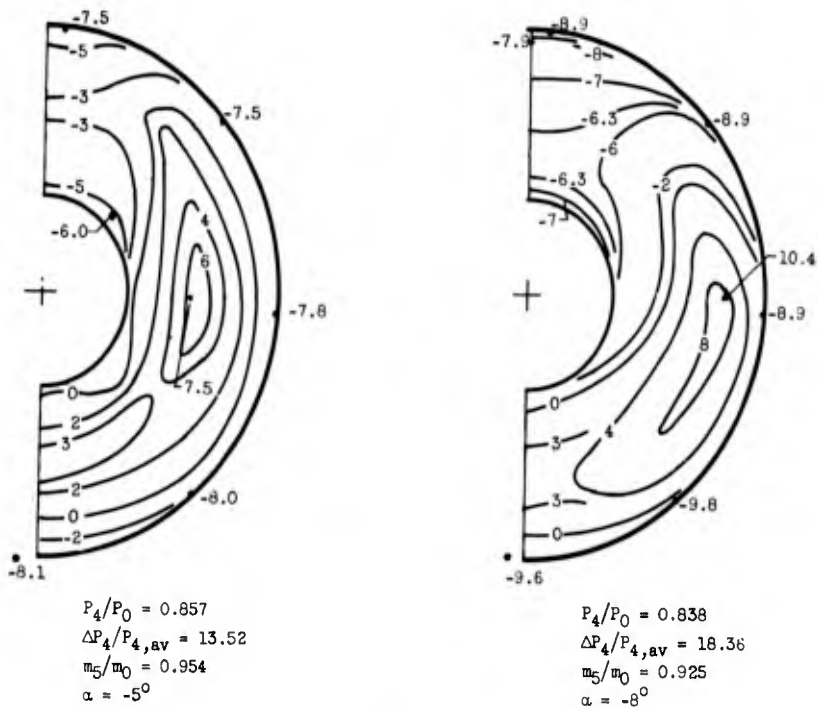
(a) Inlet C_{14}S_8 .
