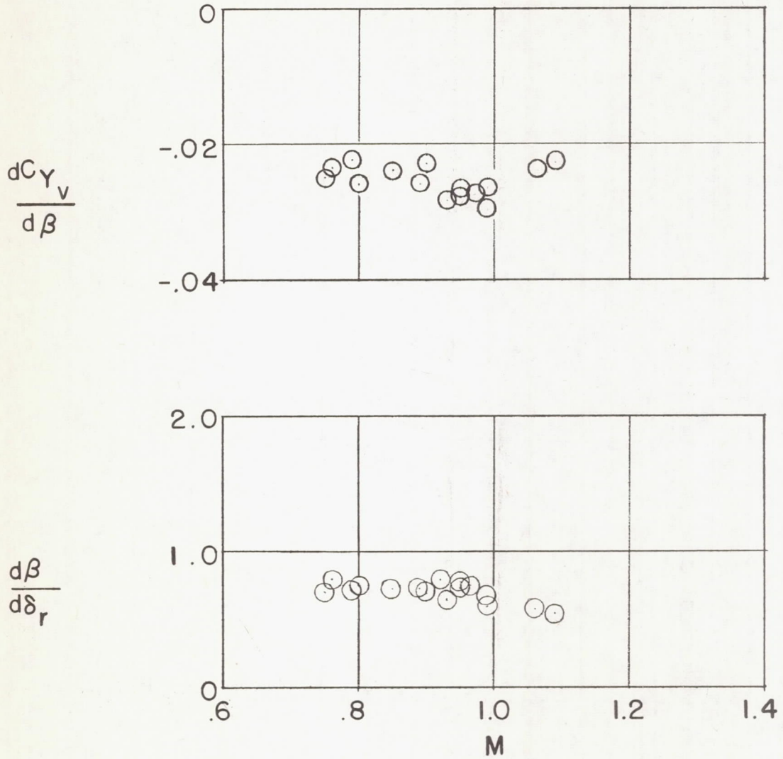
Figure 16.- Variation with Mach number of the vertical-tail side-force coefficient per unit sideslip angle and the sideslip angle for a unit rudder deflection in steady sideslips.
