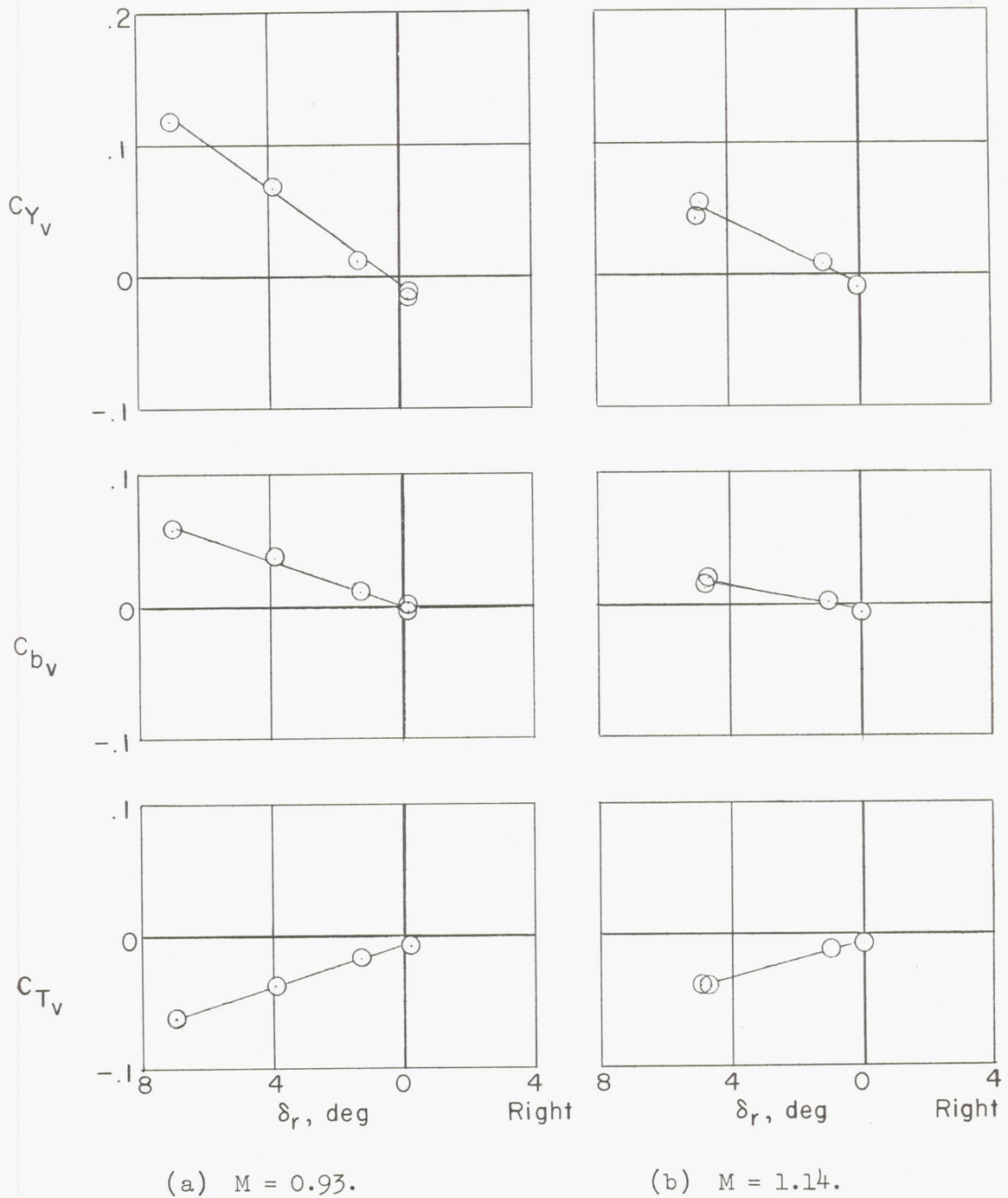
Figure 6.- Variation of vertical-tail side-force, bending-moment, and torque coefficients with rudder position (sideslip angle constant) during rudder-pulse maneuvers at M = 0.93 and 1.14 at 30,000 feet.
