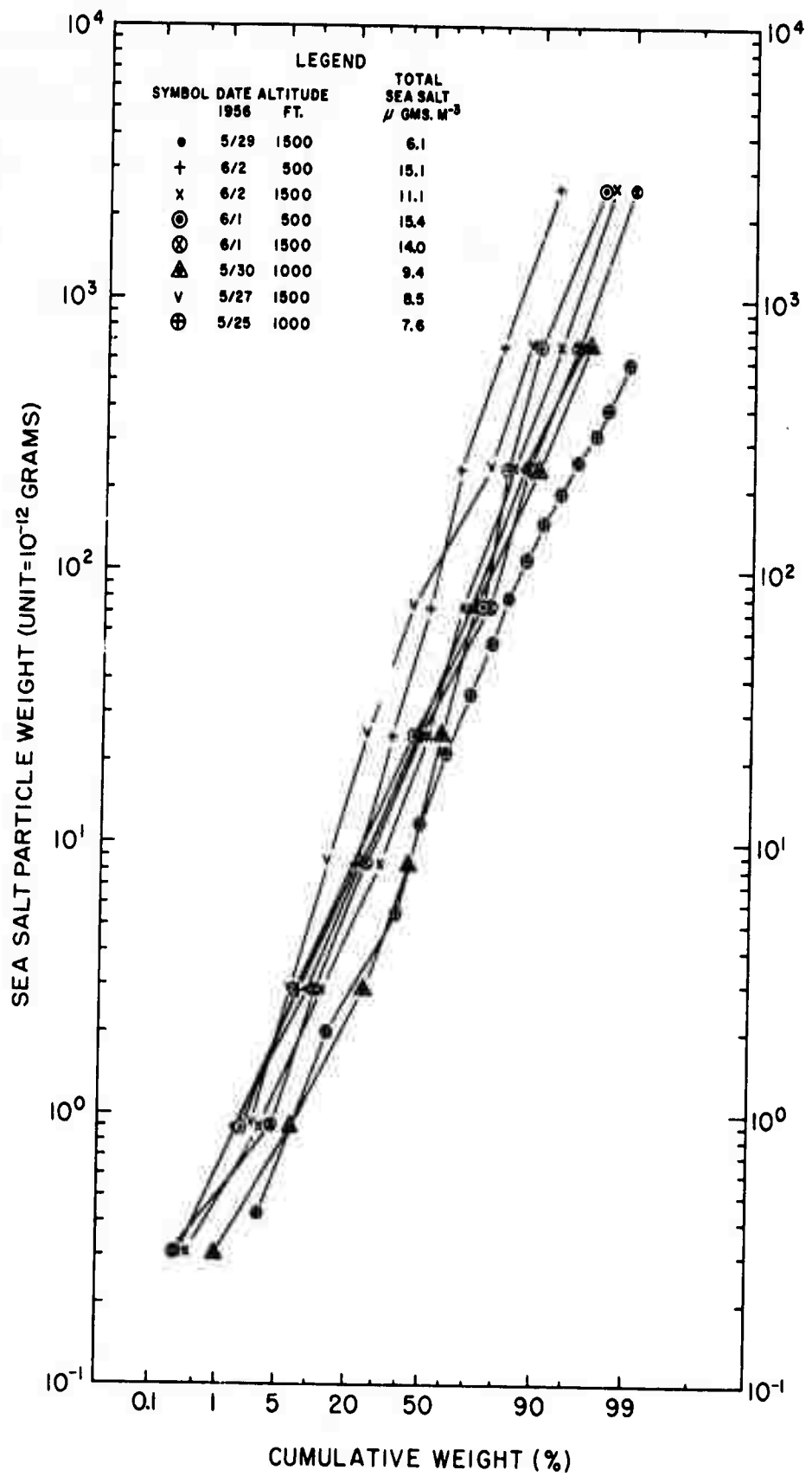
Fig. 9 Cumulative percent weight distribution curves, representing atmospheric salt-particle samples taken at the altitudes where, due to more complete sampling, the widest range of particle size was obtained. The sampling location was over the sea in the Virgin Islands region.
