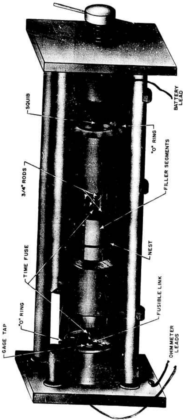
FIG.14 PRESSURE BOMB FOR CONSTANT VOLUME TESTS
