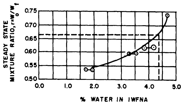
Figure 10. Limit of Steady State Operation at -33^{\circ}\text{F} with Gas Generator HGP-81
