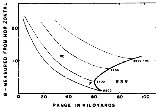
Figure 9 - Graph of angle of emergence from a shallow source as a function of range to illustrate the focussing peak and the RSR region
