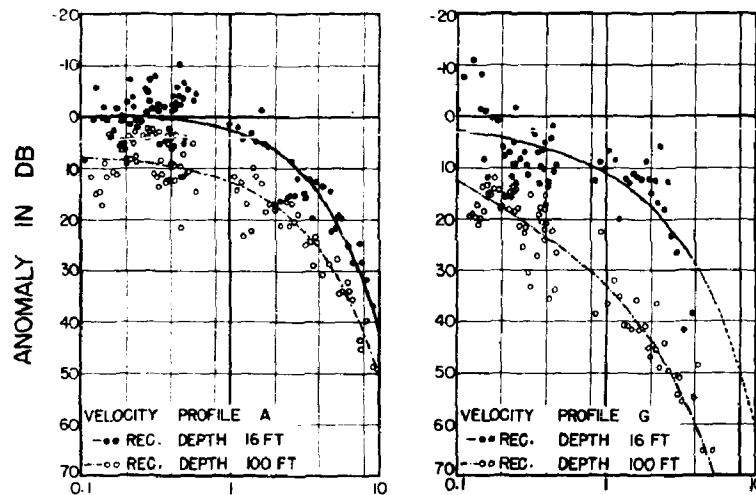
Figure 20 - Anomaly vs range for 22.5-kc sound in and near a brashy ice pack with source depth of 15 feet
