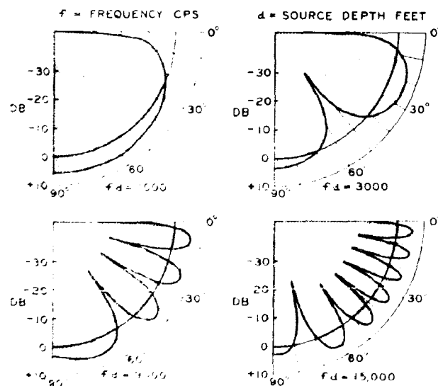
Figure 13. Directivity of doublet formed by near-surface source and its surface image
