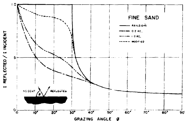
Figure 3 - Ratio of reflected to incident energies vs grazing angle for fine sand for Rayleigh's equation with and without attenuation in the sand estimated to be typical for the Bering Sea. The modified curve is for attenuation extrapolated as the first power of the frequency.
