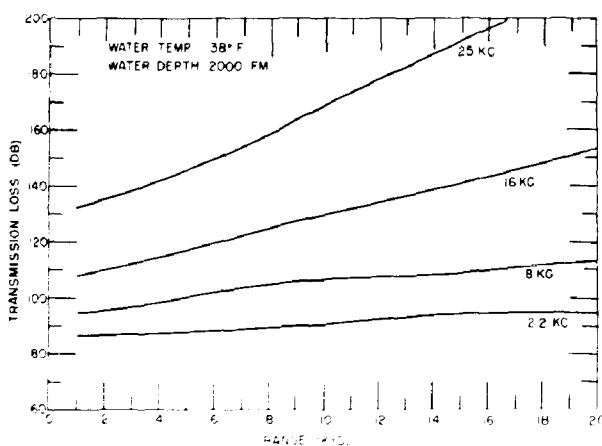
Figure 11 - Transmission loss vs range for bottom-reflected transmission
