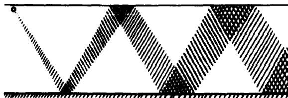
Figure 1 - Steep-angled sound beam resulting in first and second bottom-reflected signals
