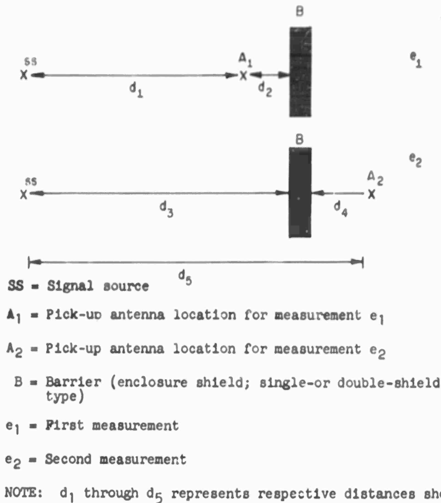
FIGURE 7 - "Attenuation" Test
