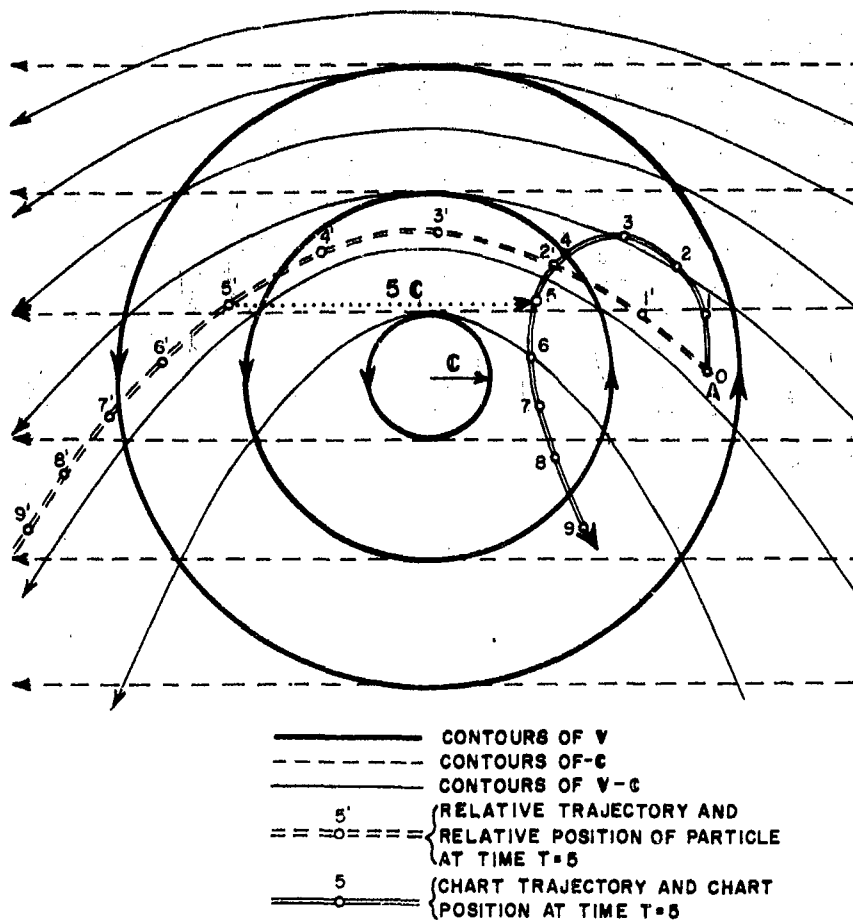
Figure 5. Trajectory by the Relative Trajectory Method. A circular vortex of uniform speed moves to the right with constant speed \vec{c} . The relative trajectory and the chart trajectory, starting from a point A, are indicated.
