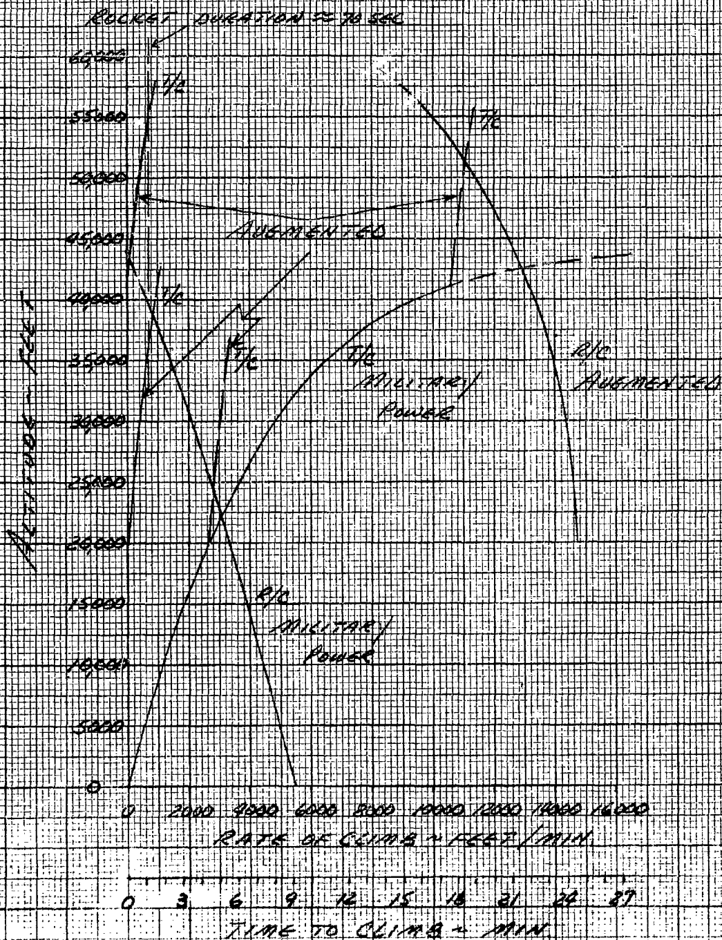
FIGURE No 3 COMBINED CLIMB PERFORMANCE F-86E USAF NO 31-2773 J-97-66-13 ENGINE YLR 63-A1-3 ROCKET ENGINE 15,984 LBS AT ENGINE START INLET SCREENS IN PLACE
