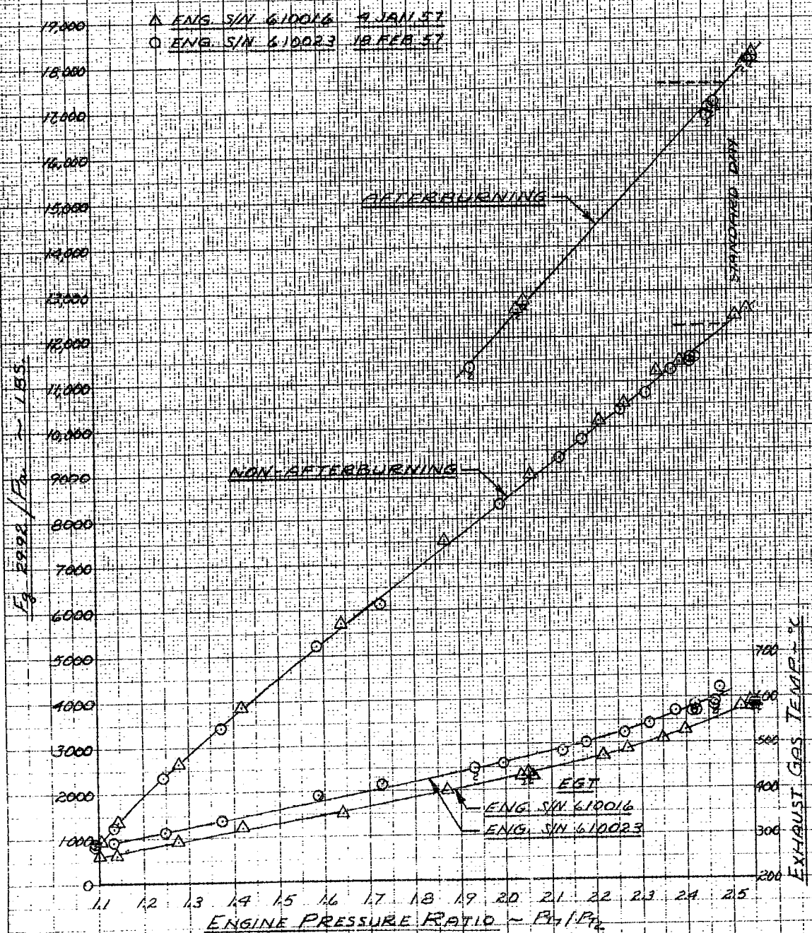
FIG. NO. 26 STATIC THRUST CALIBRATION F-105B USAF NO. 54-100 YJ-75 A-3 ENGINE
