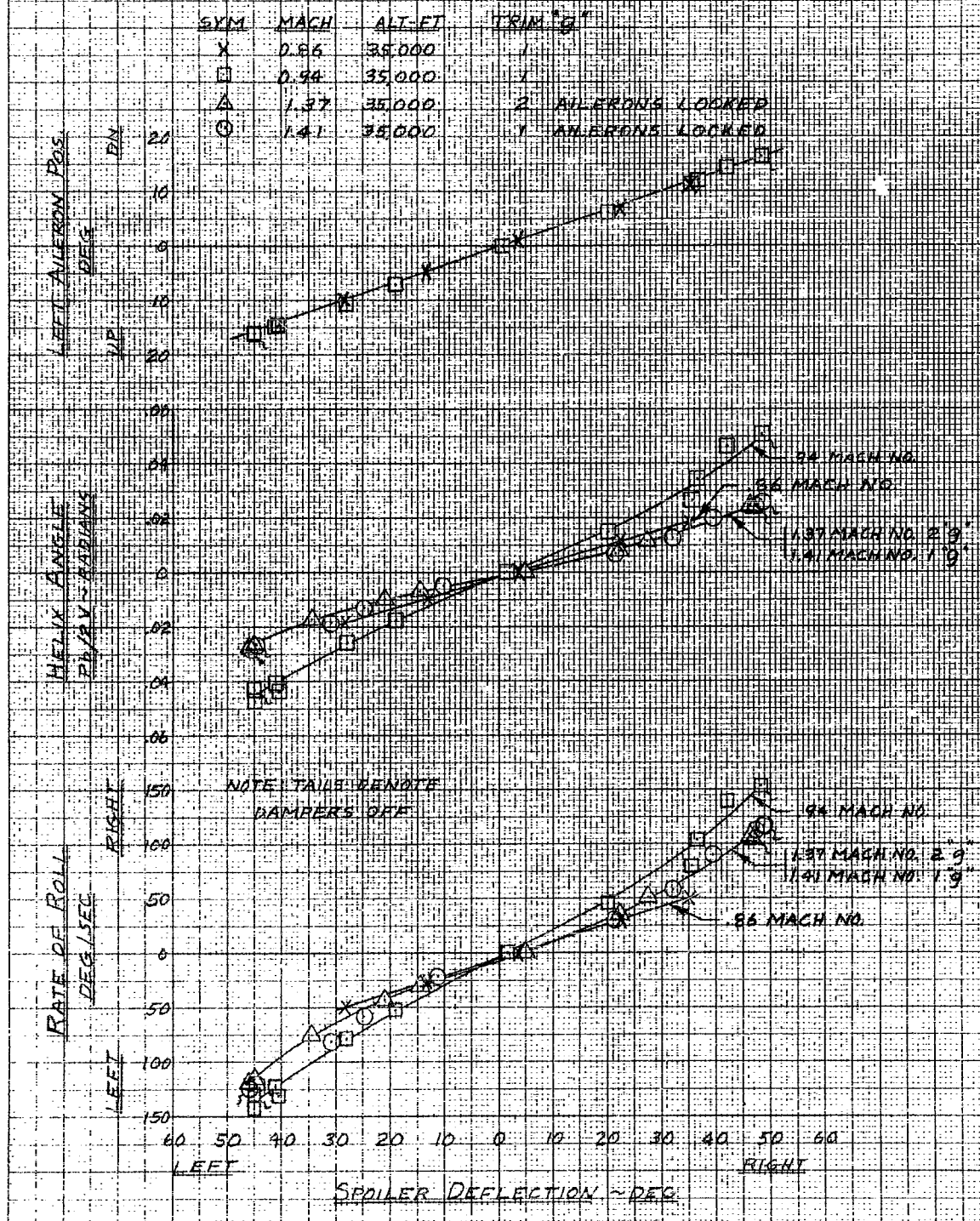
FIG. No. 66 ROLL SUMMARY F-105B L99AF NO 54-100
