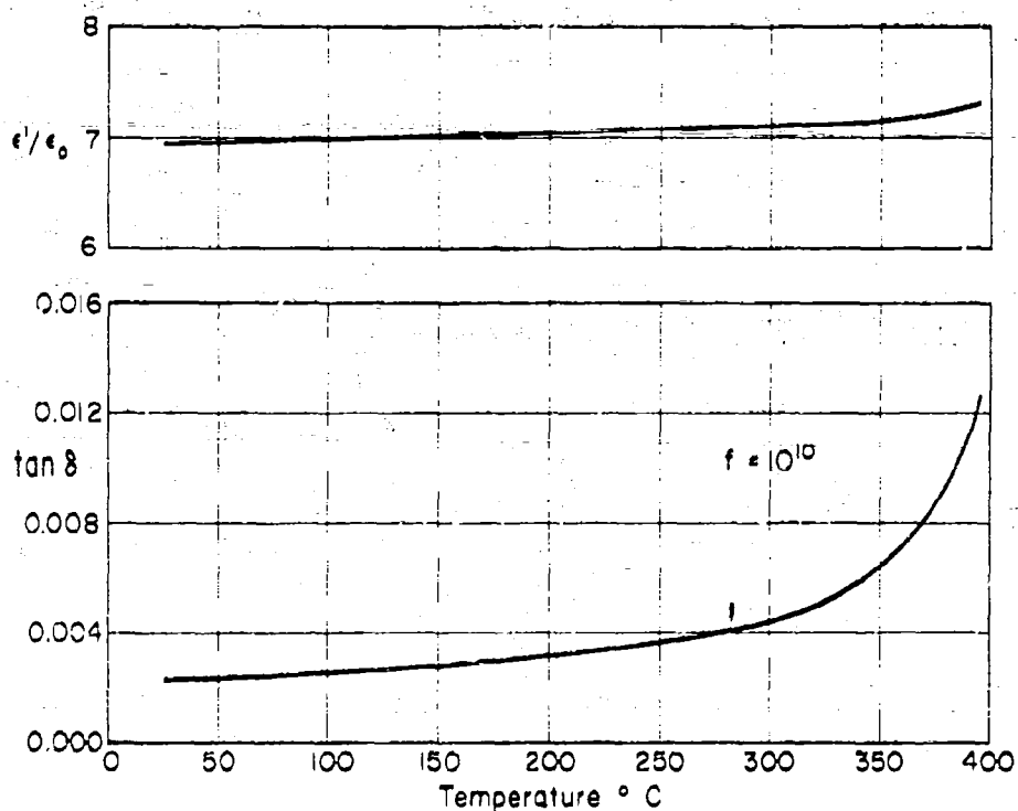
Fig. 18. Dielectric constant and loss tangent vs. temperature for synthetic mica bonded with glass (Supramica 500, Mycalex Corp.) at 10,000 Mc.
