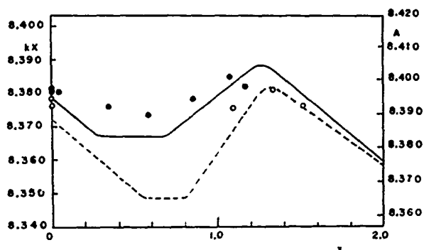
Figure 1—Lattice parameter of the \text{FeFe}_{(2-x)}\text{Cr}_x\text{O}_4 solid solution system measured at room temperature. Full curve, synthetic stoichiometric solutions quenched from 1180 C, 1100 C, 950 C; dashed curve, synthetic oxygen-rich solutions quenched from 950 C. From scale analysis: full circles, coexisting with wüstite phases; open circles, without wüstite.
