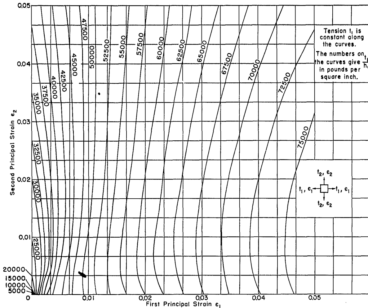
Figure 7 - Tension Due to Biaxial Strain
