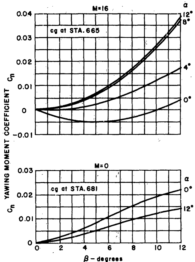
Figure 19. Estimated Yawing Moment Characteristics
