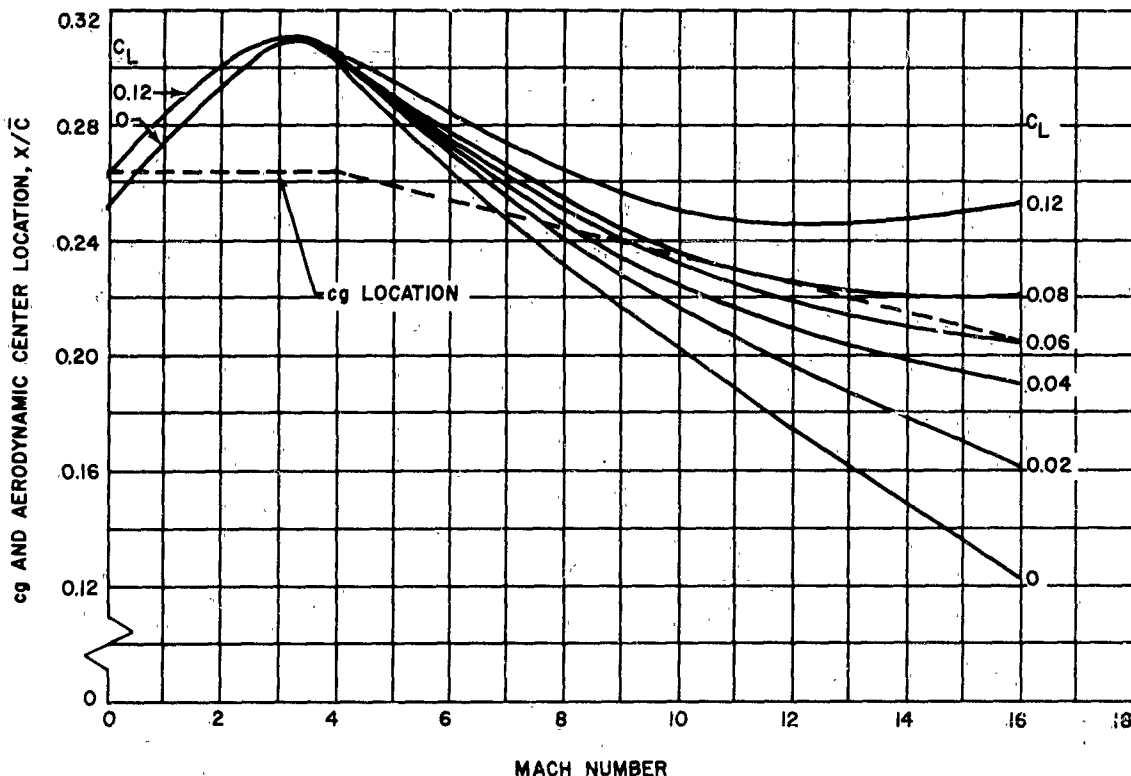
Figure 18. Estimated Center of Gravity and Aerodynamic Center Locations
