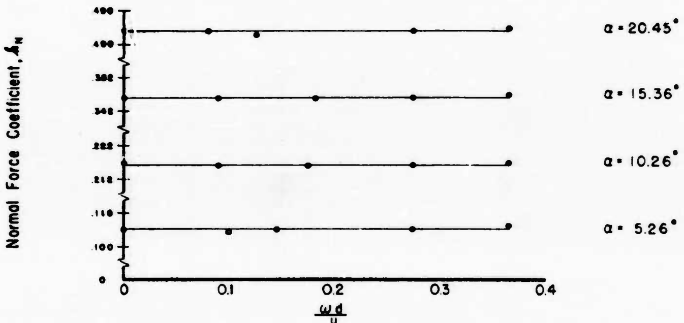
PITCH DATA VARIATION WITH SPIN FOR 30 MM BULLET M_0 = 2.47 Re = .76 \times 10^6 FIG.19
