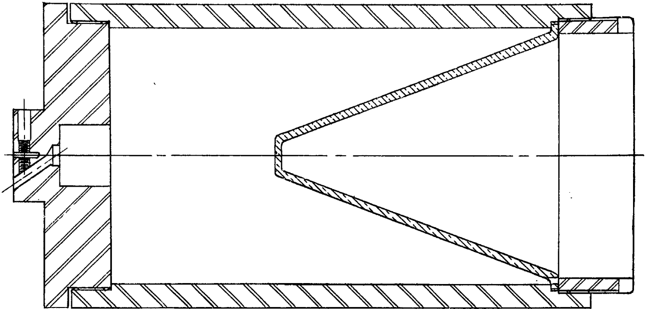
Fig. 22. Penetration Test Assembly. DRC-23-1185-1 With Cone DRB-25-1253-1.
