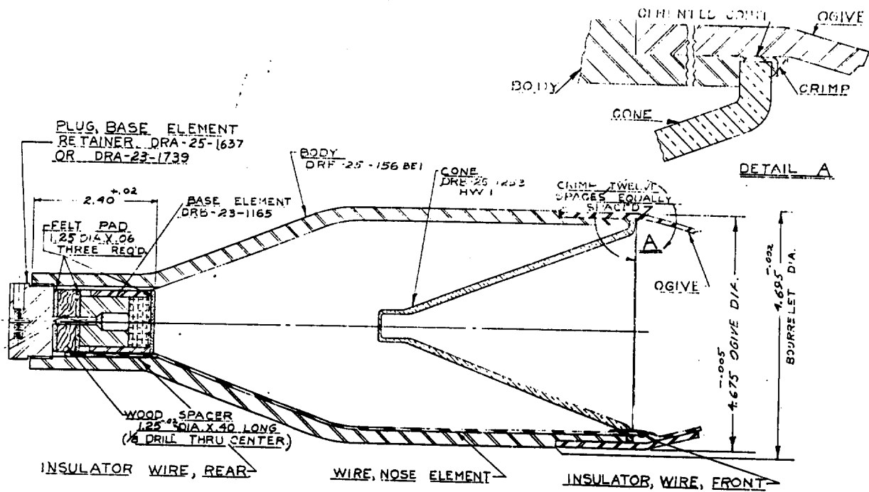
Fig. 26. 120 mm. Test Assembly, T336E21. Firestone Drawing No. DRD-25-619-1.
