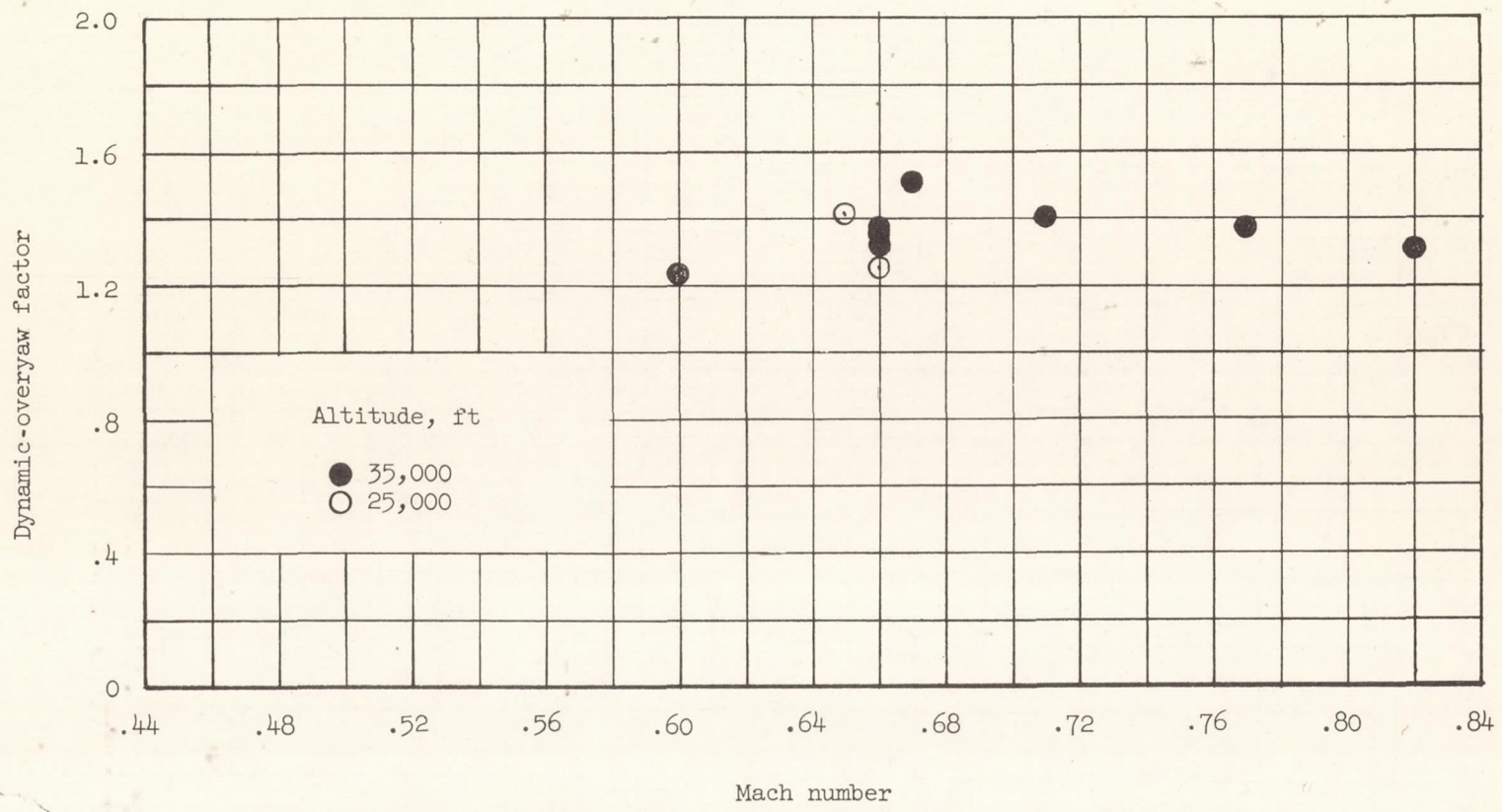
Figure 24.- Dynamic-overyaw factor.
