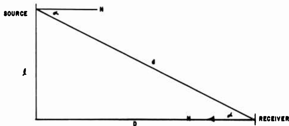
Fig. 3.3—Flux geometry.
