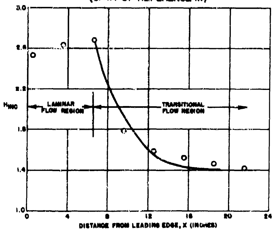
FIG.9 COMPARISON BETWEEN CALCULATED AND EXPERIMENTAL VALUES OF H_{INC} FOR COMPRESSIBLE ZERO PRESSURE GRADIENT FLOW (DATA OF REFERENCE m)
