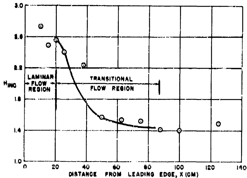
FIG.7 COMPARISON BETWEEN CALCULATED AND EXPERIMENTAL VALUES OF H_{INC} FOR INCOMPRESSIBLE FLAT PLATE FLOW (DATA OF REFERENCE 1)
