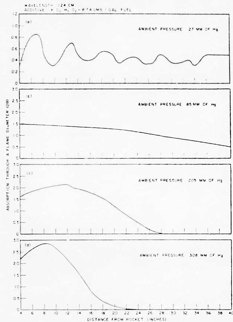
Fig. A-3 - Absorption through a flame diameter versus distance from rocket motor for several ambient pressures
