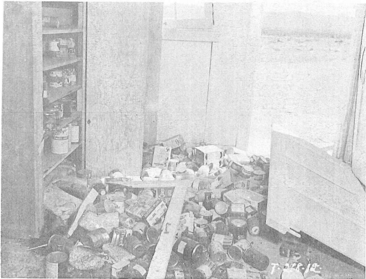
Fig. 4.16—Kitchen cabinets of white frame house at 5500 ft from Ground Zero after the shot.
