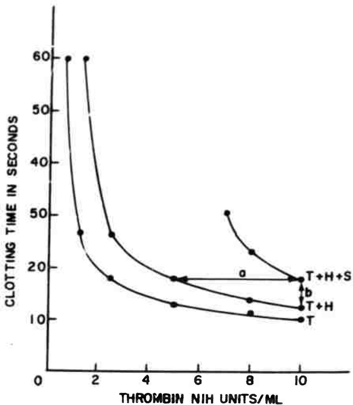
Fig. 7. Effect of bovine serum (cofactor source) on the thrombin-heparin-clotting time. Upper curve (T + H + S) obtained with 0.5 NIH units of heparin and 0.025 ml serum per ml reaction mixture. Middle curve (T + H) obtained with 0.5 NIH units of heparin. Lower curve is standard thrombin assay as described. The displacement of (T + H + S) from (T + H) is used for calculation of effect of serum, and does not vary with thrombin concentration in direction of the horizontal axis within range of limits of reasonable precise clotting time measurements.
