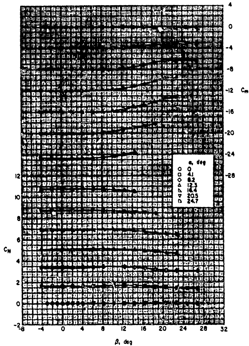
(b) Large delta wing, P_{1W_1A_2} .
