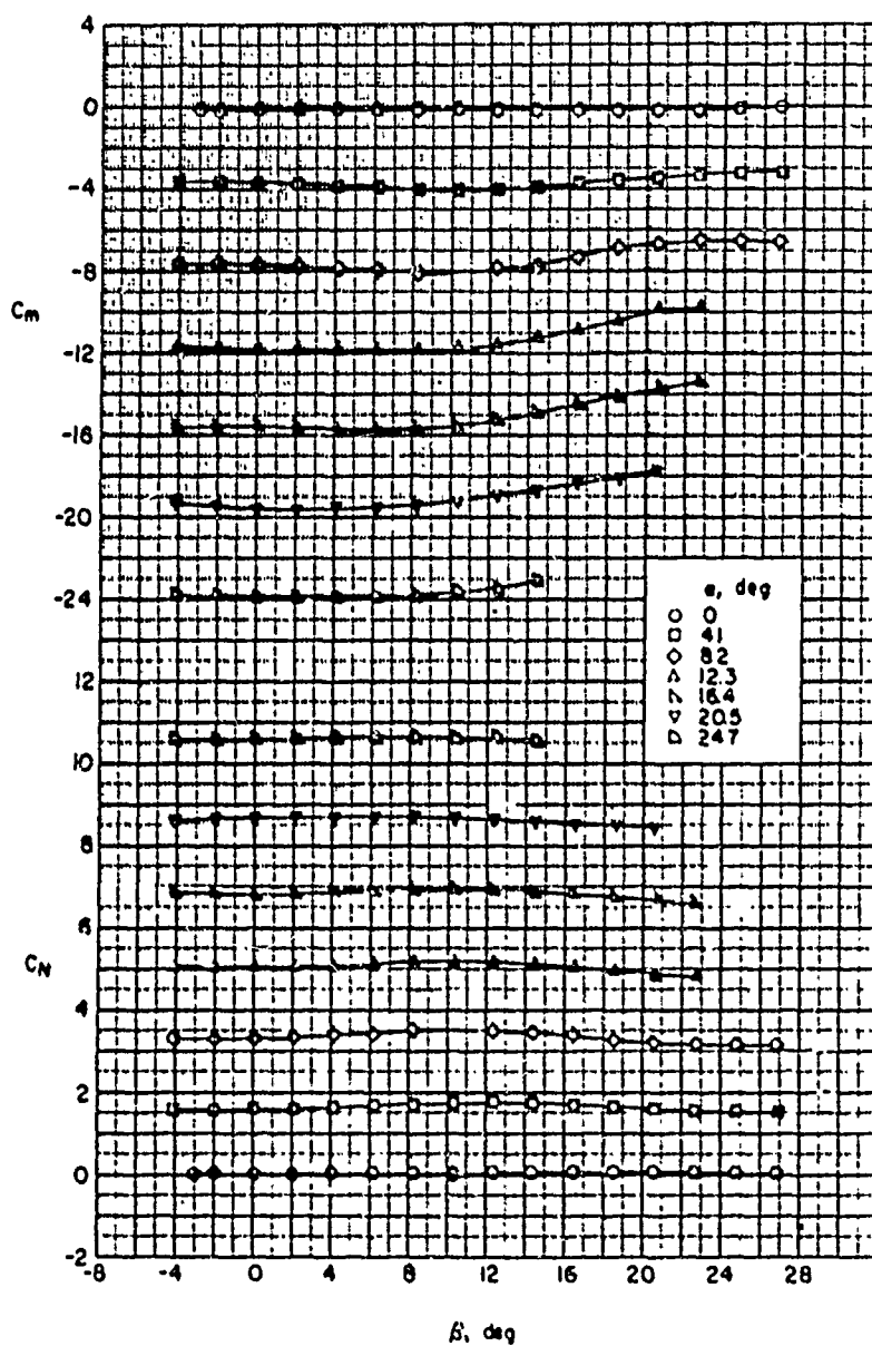
(c) Large delta wing, F1W1A1.
