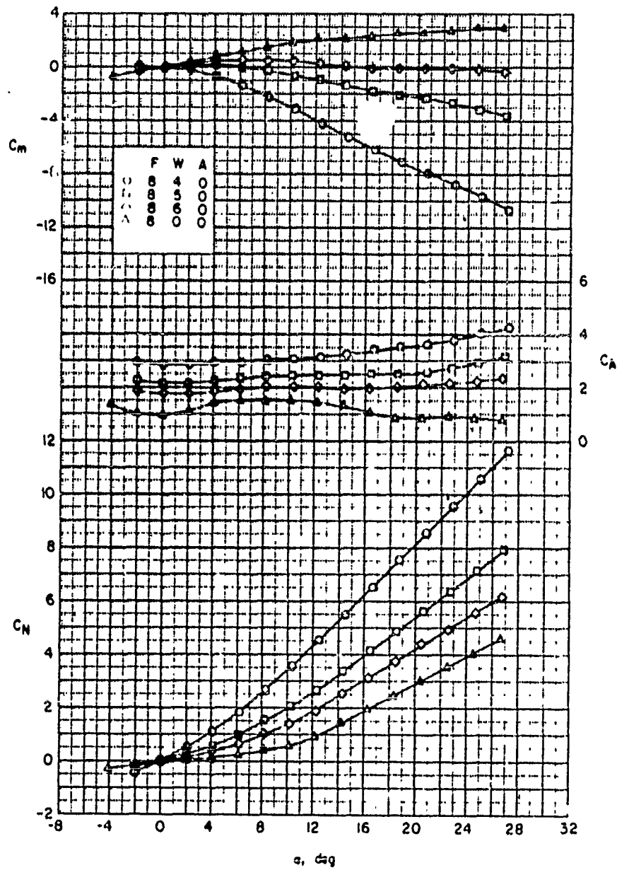
Figure 13.- Effect of rectangular wings on aerodynamic characteristics in pitch. No afterbody; l/l = 10 .
