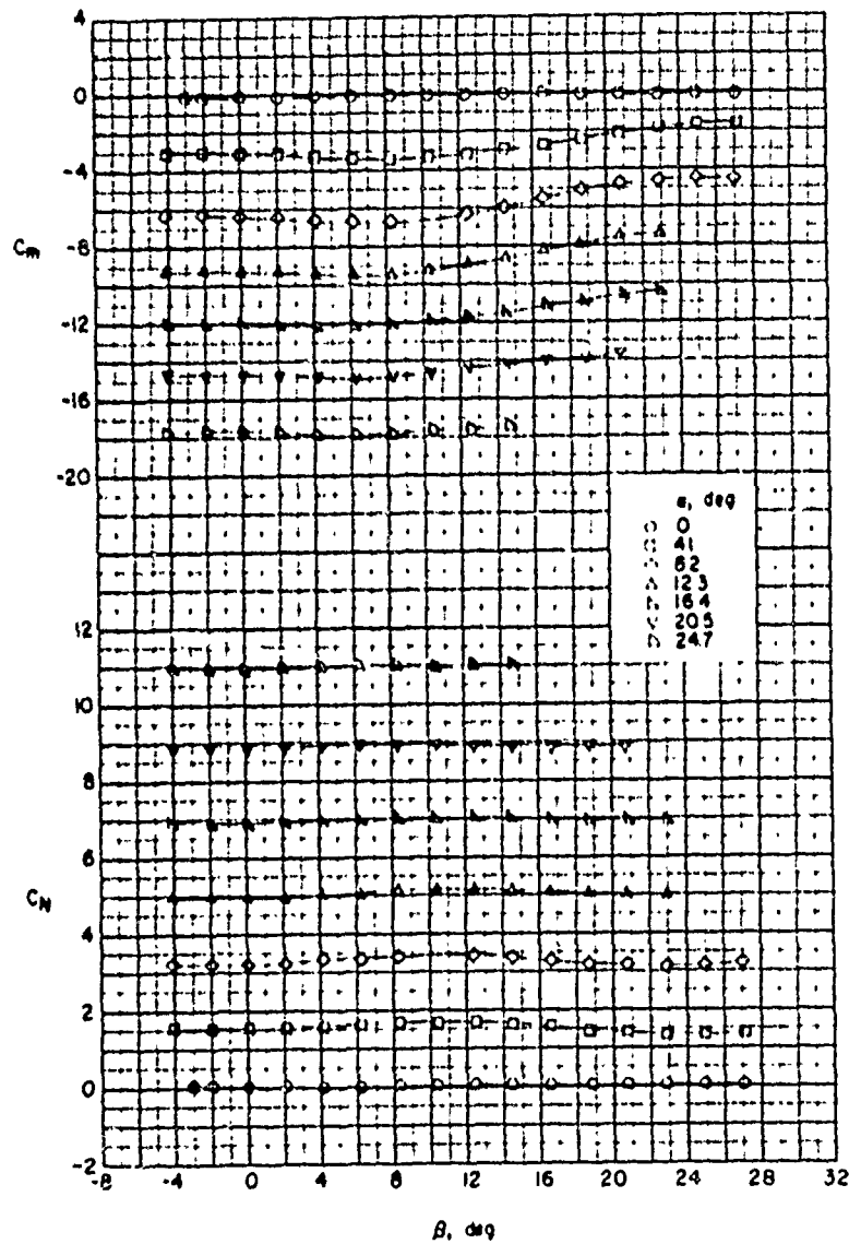
(e) Large delta wing, F_0W_1A_1 .
