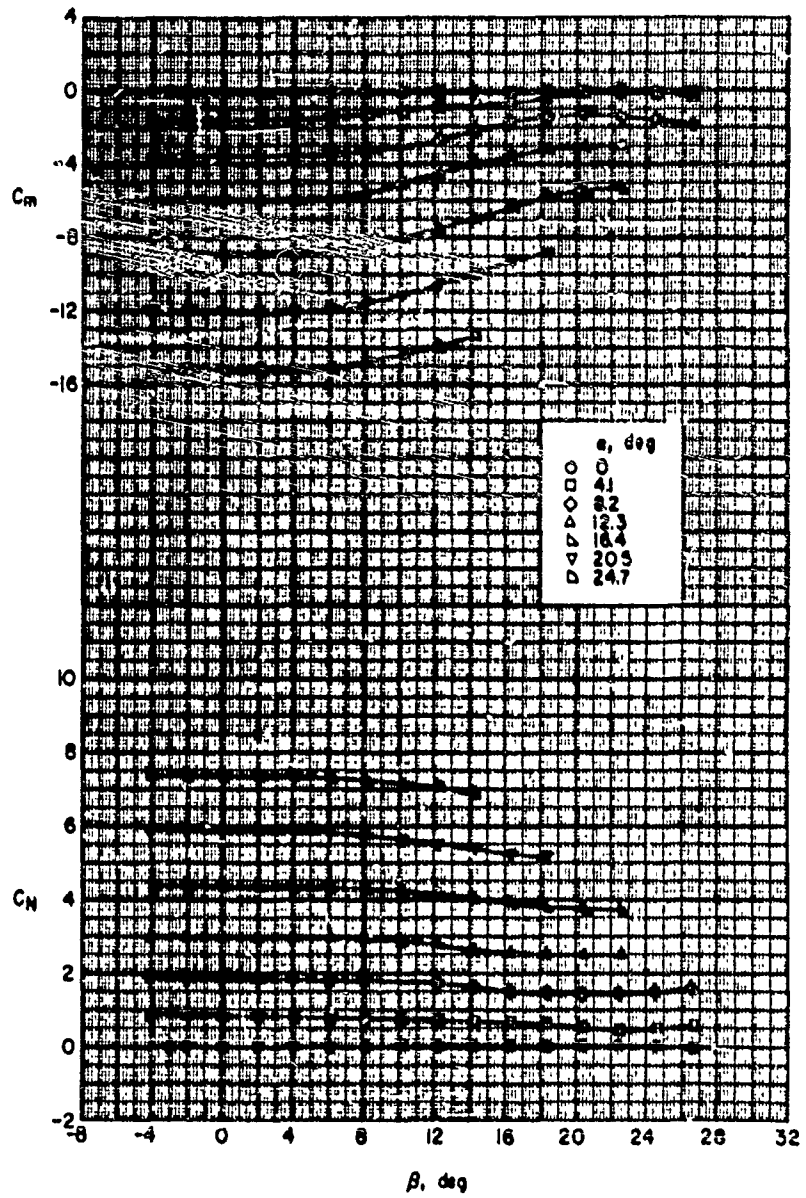
(c) Medium delta wing, F_1W_2A_2 .
