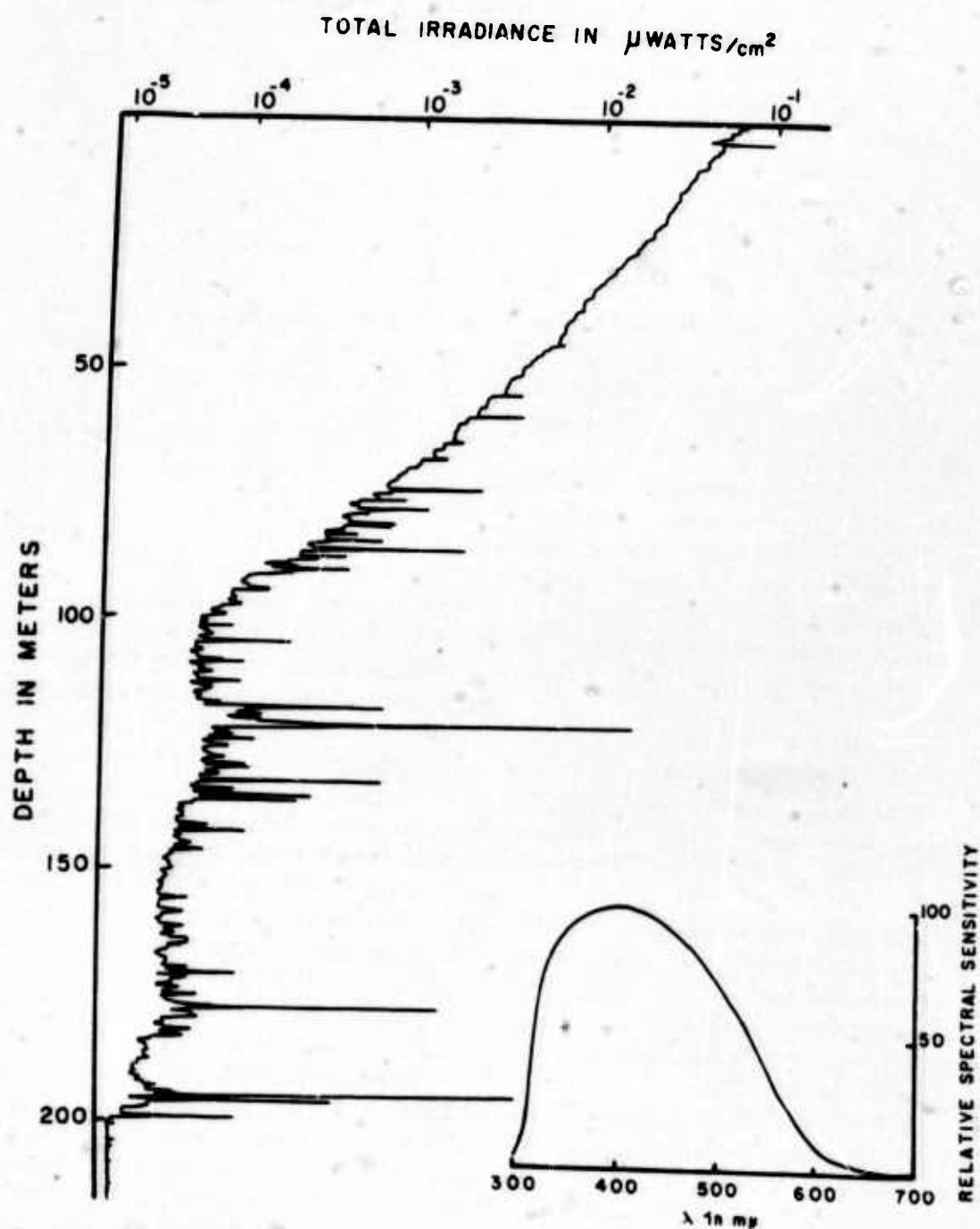
FIG. 1. Tracing of total irradiance recorded on Leeds and Northrup Speedomax recorder by bathyphotometer without color filters. Spectral sensitivity of the 931-A photomultiplier tube is shown in inset. This is from manufacturer's specifications and is an average curve. The record was made at 2400 hours, June 9, southwest of Oahu.
