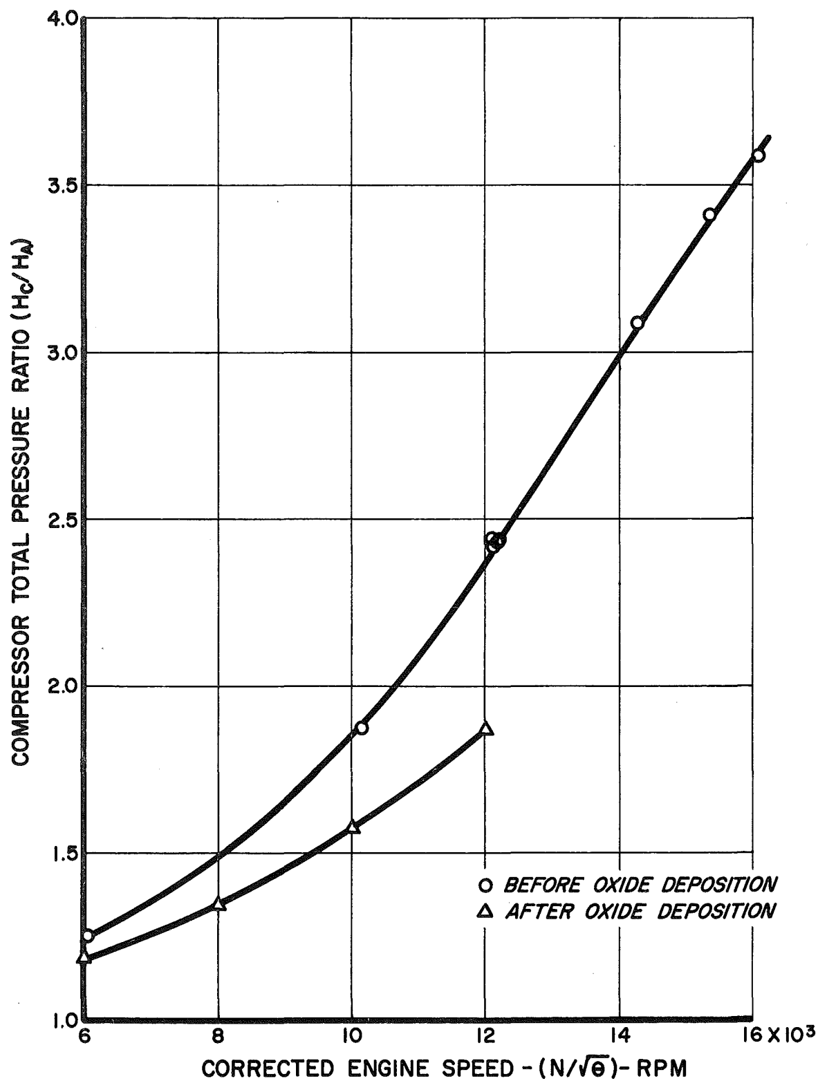
Fig. 7. Effect of B_2O_3 Deposition in Compressor Flow Passages on Axial Flow Compressor Pressure Ratio at Various Rotational Speeds
