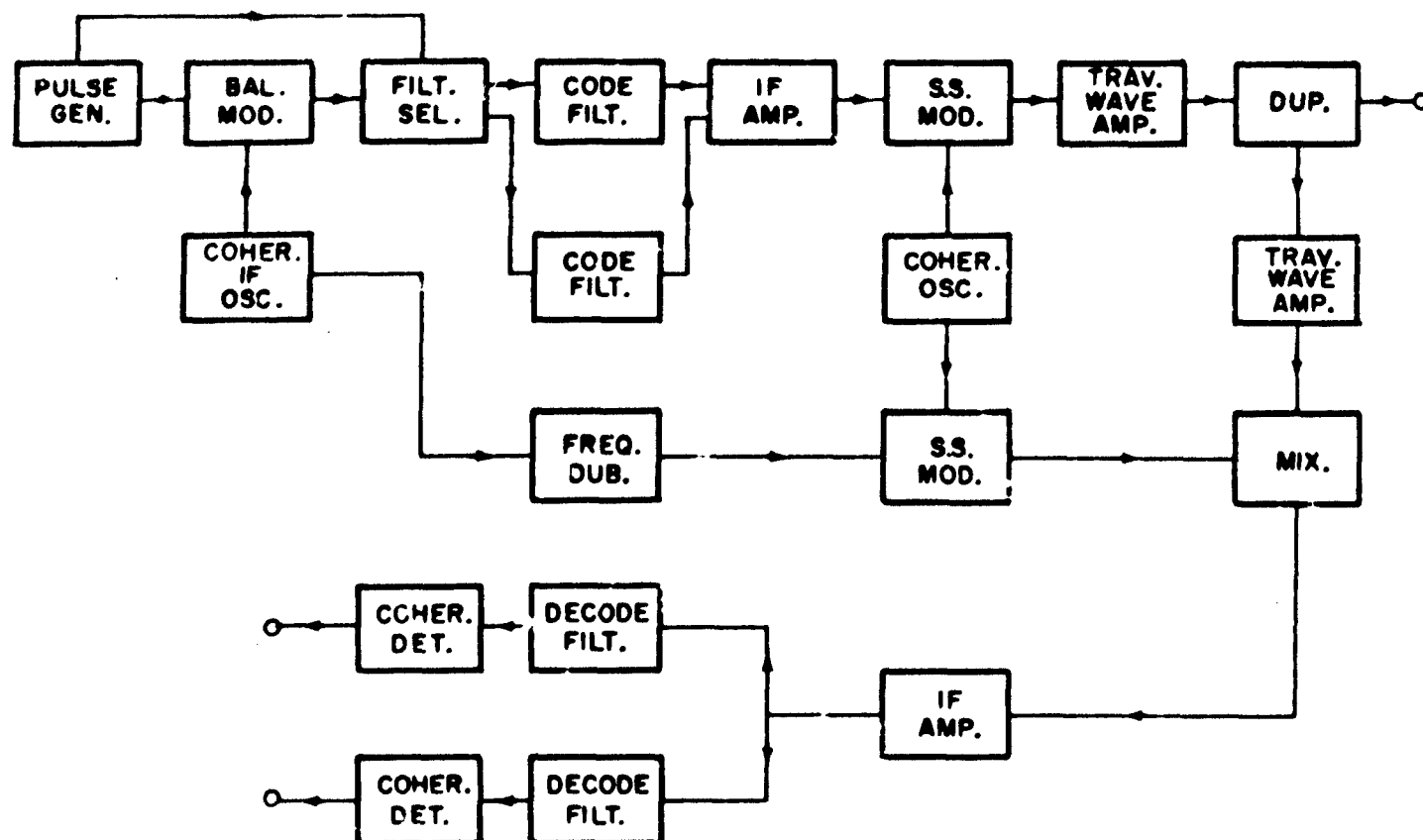
Figure 57. Chirp System
