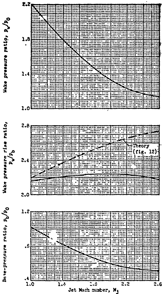
(a) Constant jet pressure ratio, 15.
