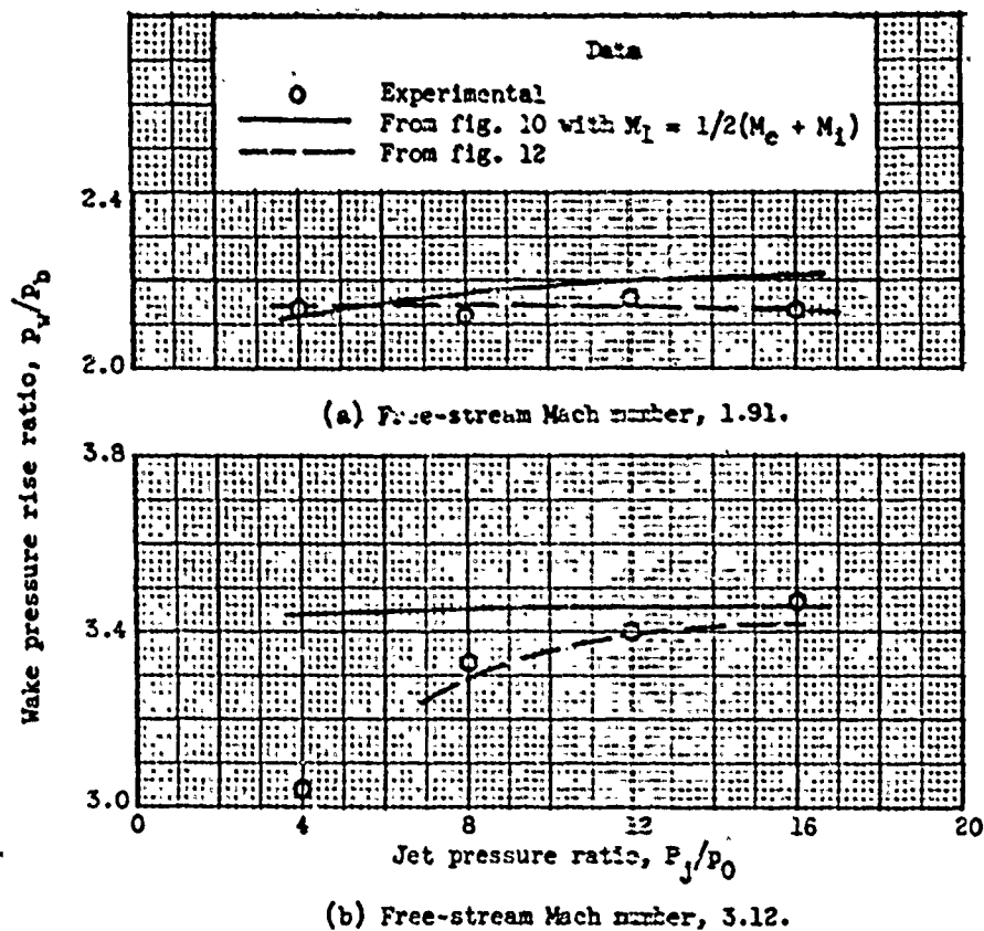
Figure 45. - Wake pressure rise ratio approximated by method of reference 4. Base-to-jet diameter ratio, 2.00; boattail angle, 5.63^\circ ; jet Mach number, 1.0.
