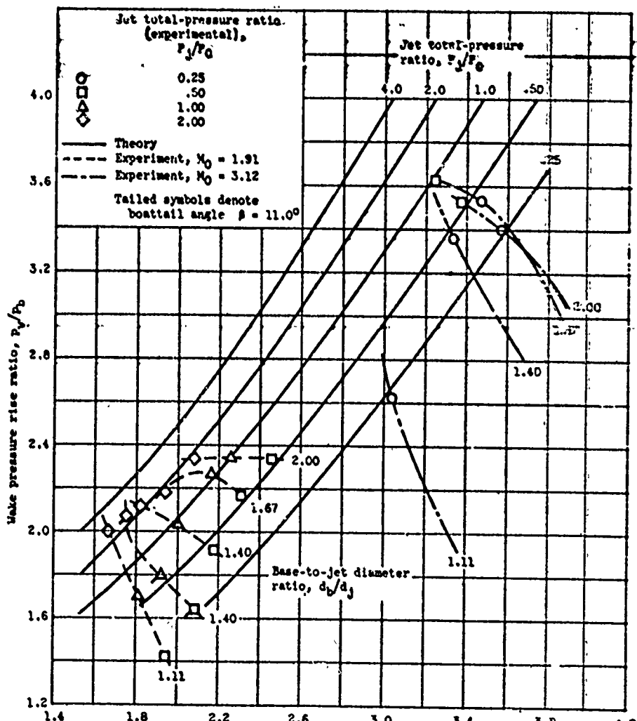
Figure 43. - Summary of wake pressure rise ratio data. Boattail angle, 11.0^\circ ; nozzle angle, 0^\circ .
