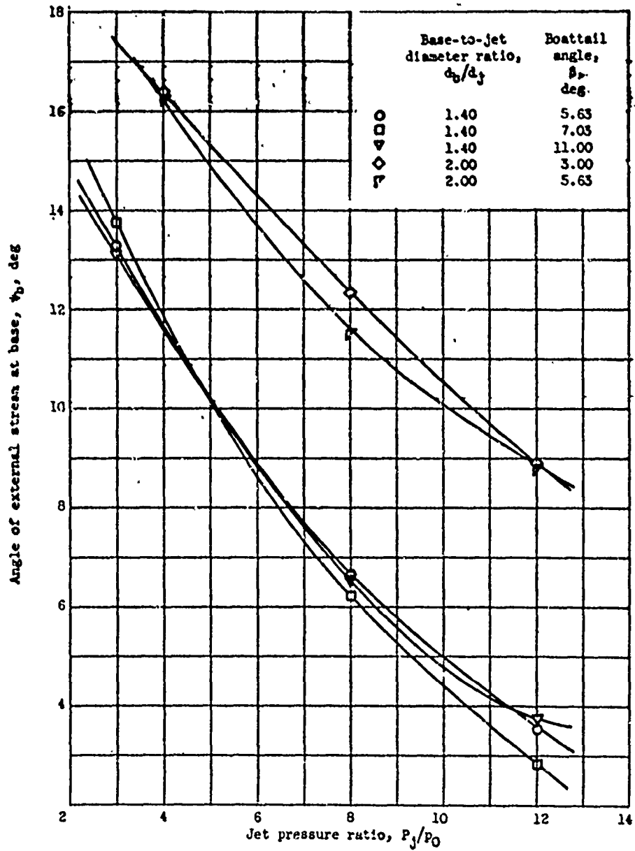
(a) Free-stream Mach number, 1.91.
