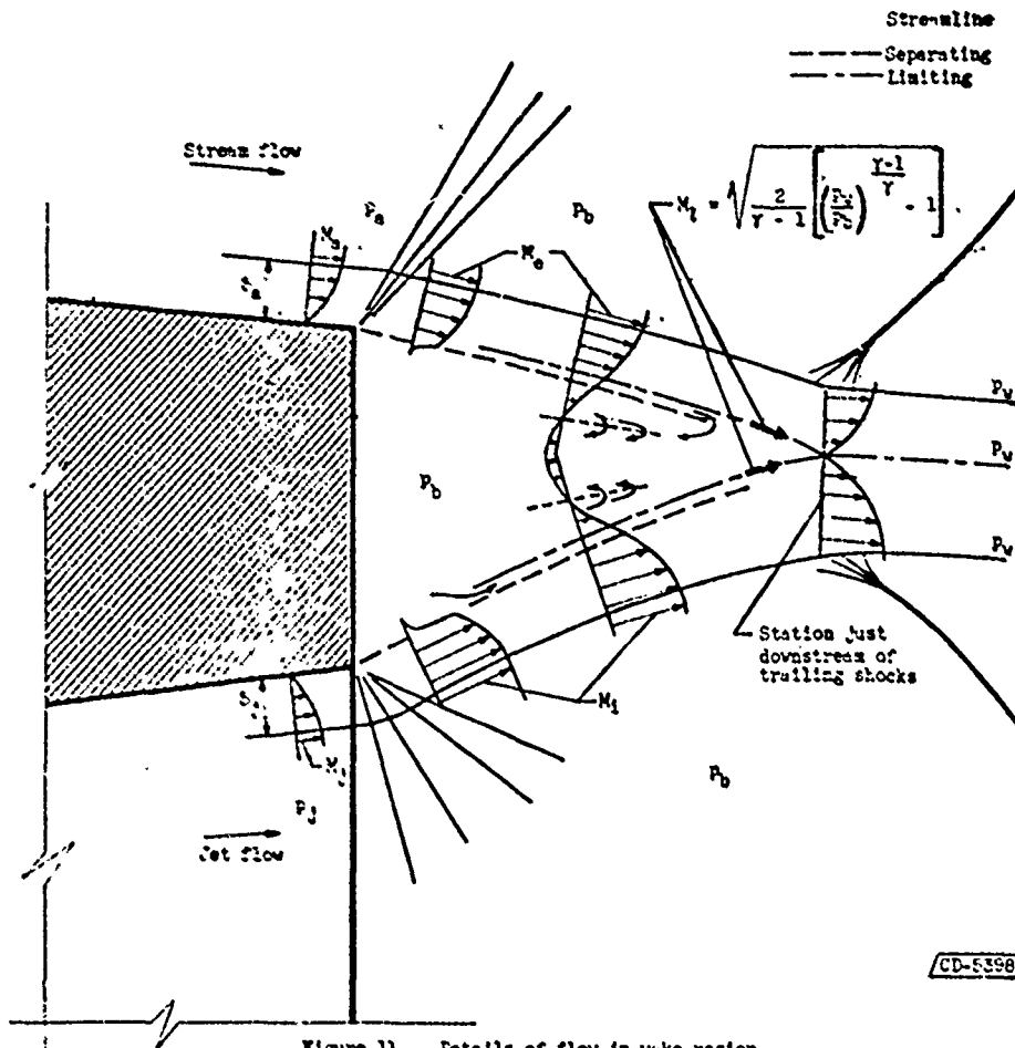
Figure 11. - Details of flow in wake region.
