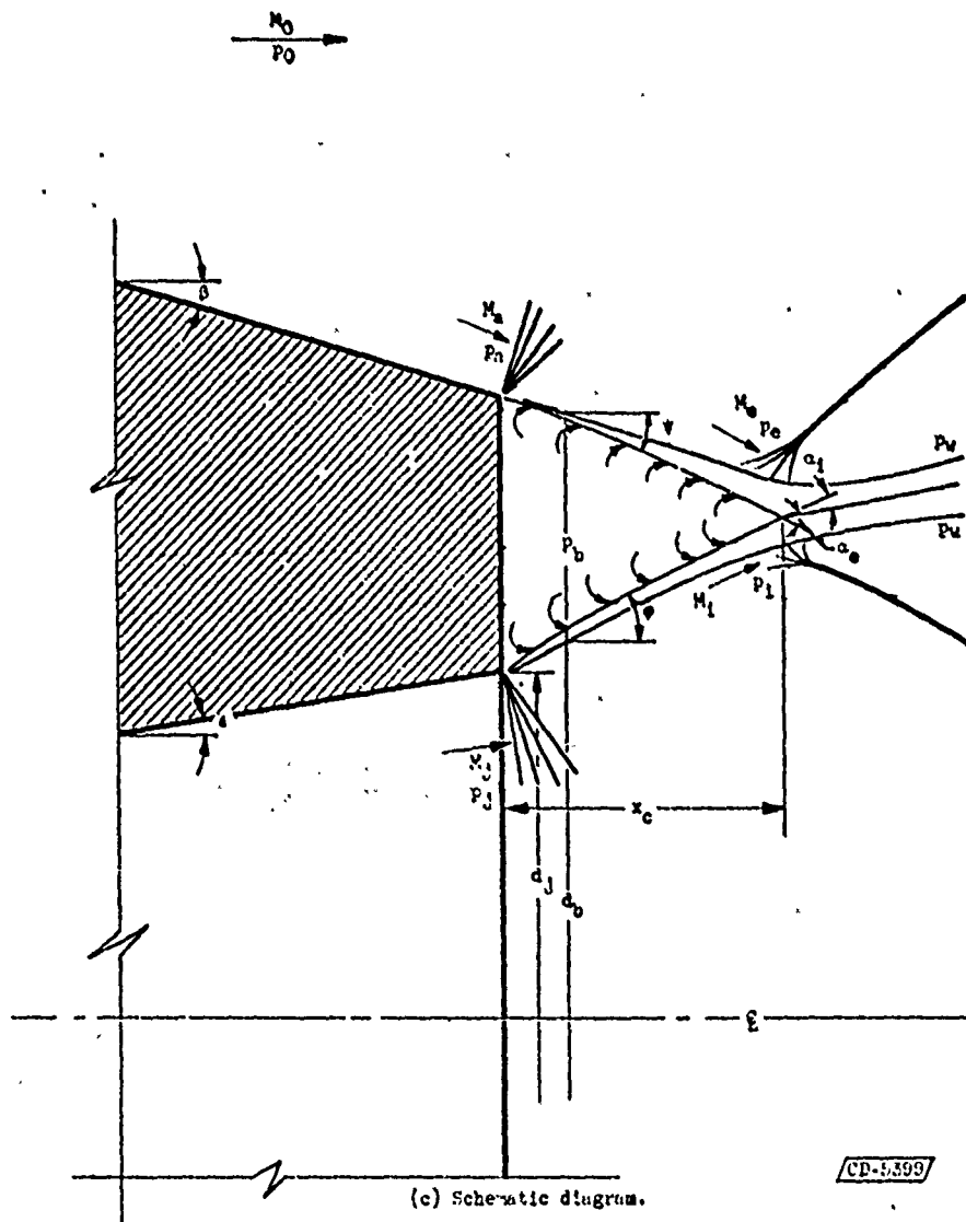
Figure 9. - Concluded. Flow geometry.
