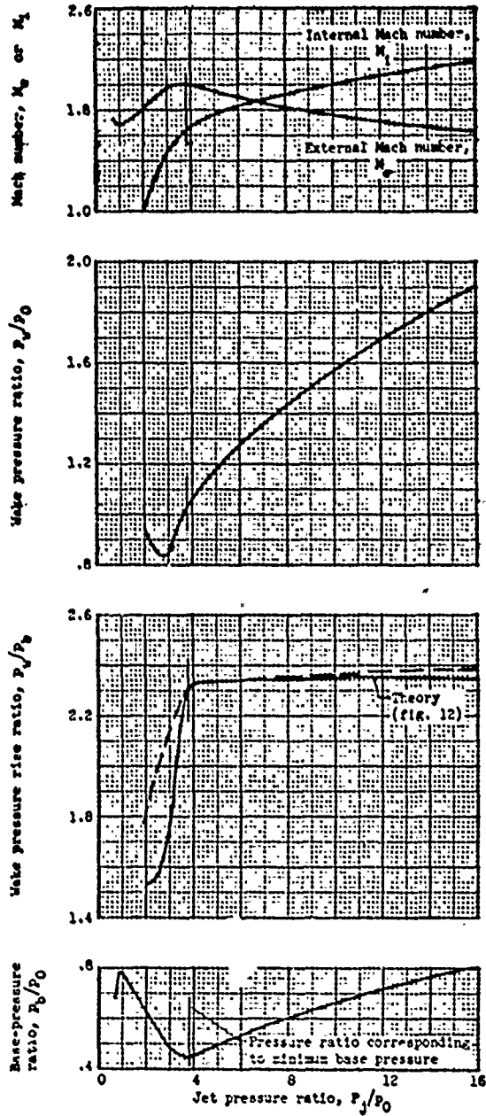
Figure 17. - Variation of base-pressure components with jet pressure ratio. Base-to-jet diameter ratio, 2.00; boattail angle, 5.63^\circ ; Jet Mach number, 1.00; free-stream Mach number, 1.91.
