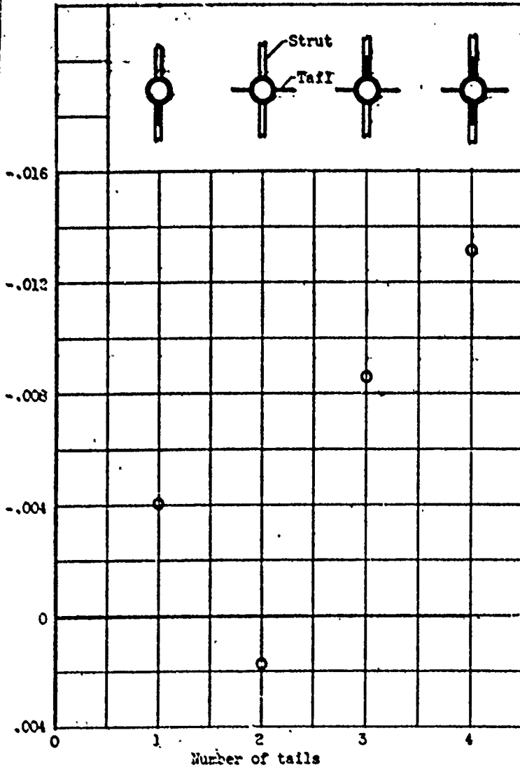
(b) Effect of number of tail surfaces. Distance from base, 0; no jet flow.
