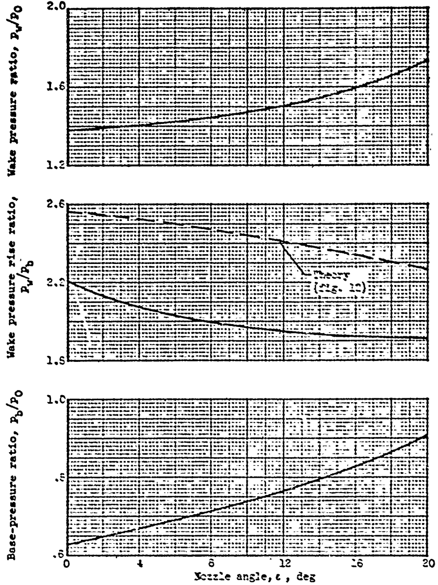
Figure 28. - Variation of base-pressure components with nozzle angle. Base-to-jet diameter ratio, 1.40; boattail angle, 5.5^\circ ; jet Mach number, 2.19; free-stream Mach number, 1.91; jet pressure ratio, 15.
