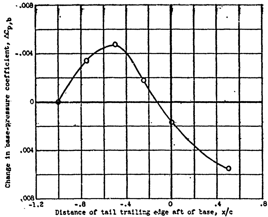
(c) Effect of axial position of plane tail. Boattail angle, 5.63^\circ ; no jet flow.
