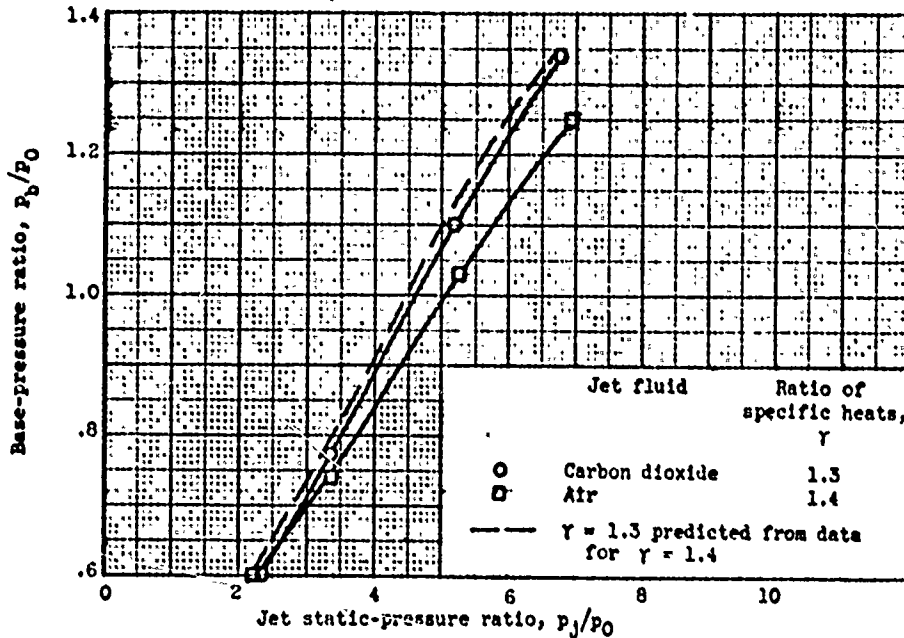
Figure 38. - Effect of ratio of specific heats on base pressure. Base-to-jet diameter ratio, 1.40; boattail angle, 5.63°; free-stream Mach number, 1.91.
