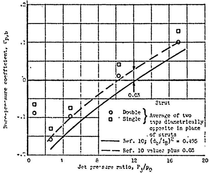
(b) Base pressure; ratio of base area to body area, 0.276.
