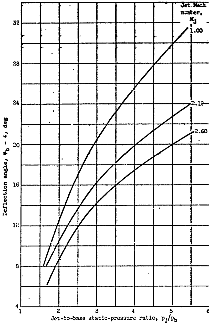
Figure 34. - Variation of deflection angle at base with jet to base static-pressure ratio for several values of jet Mach number. Ratio of specific heats, 1.4.
