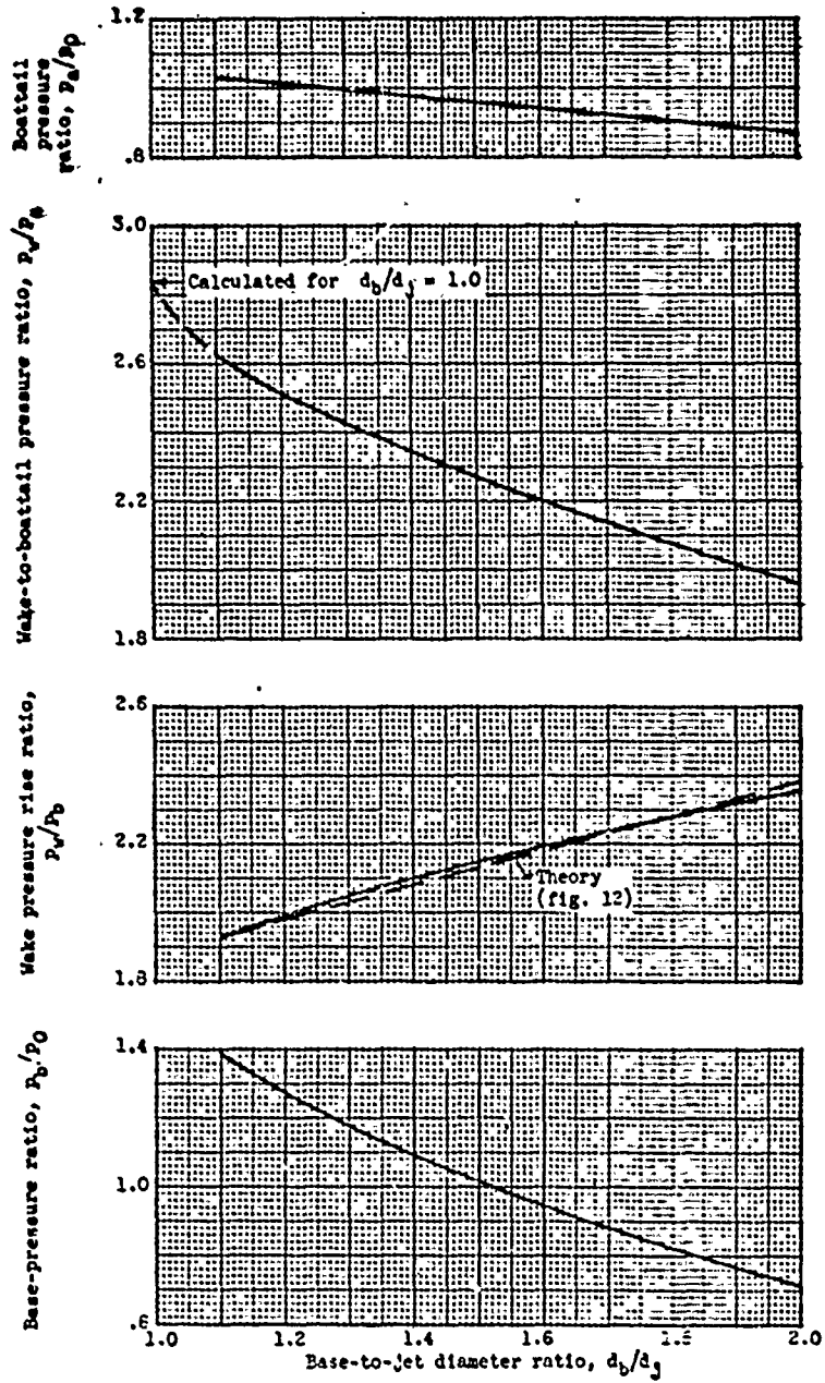
Figure 20. - Variation of base-pressure components with base-to-jet diameter ratio. Boattail angle, 5.63^\circ ; jet Mach number, 1.00; free-stream Mach number, 1.91; jet pressure ratio, 12.
