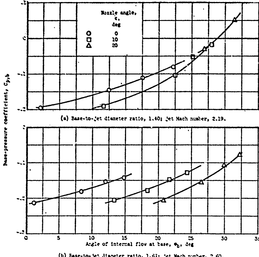
Figure 29. - Nozzle angle correlation. Free-stream Mach number, 1.97; boattail angle, 5.63°.
