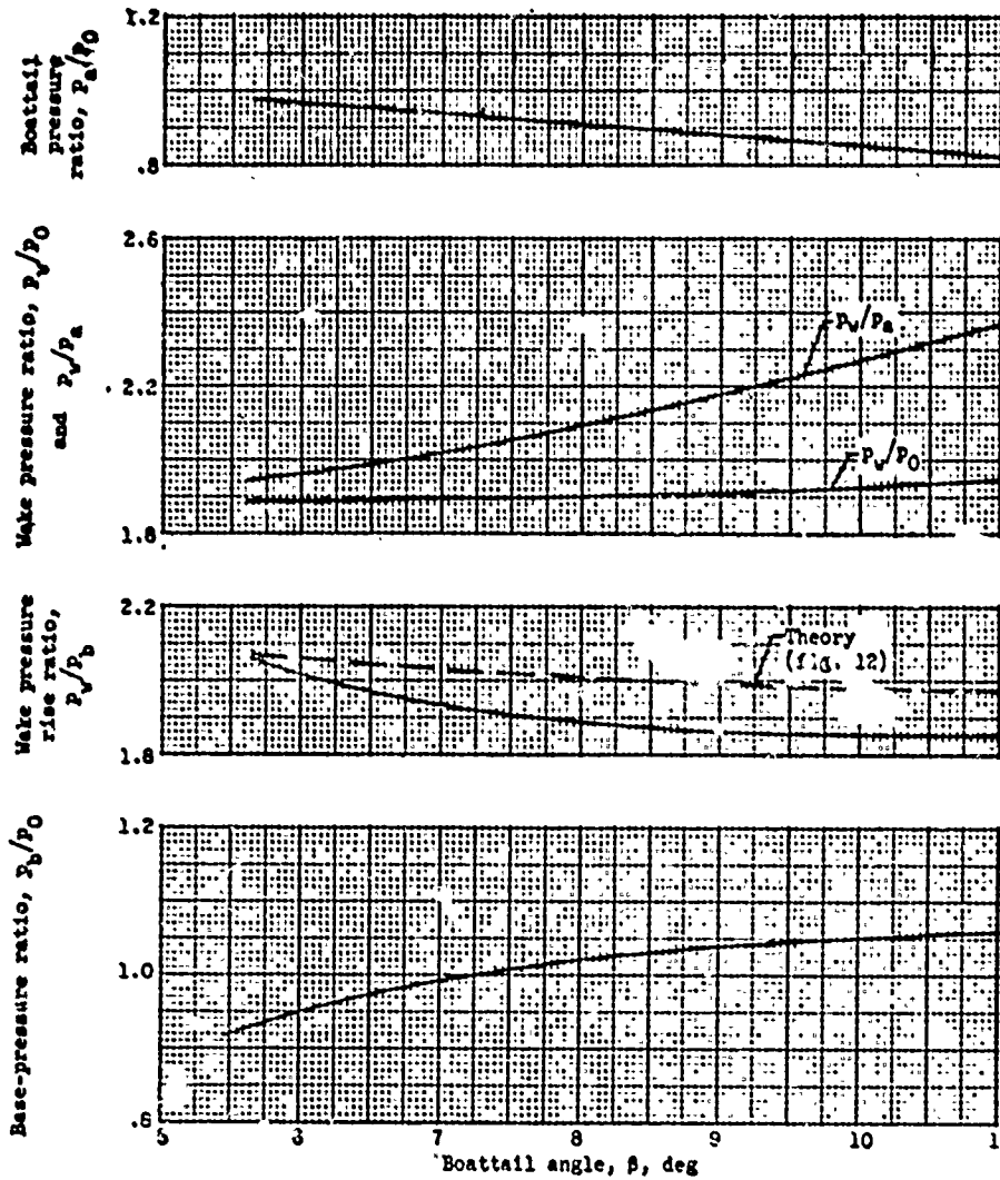
Figure 25. - Variation of component pressure ratios with boattail angle. Base-to-jet diameter ratio, 1.40; jet Mach number, 1.00; free-stream Mach number, 1.91; jet pressure ratio, 8.
