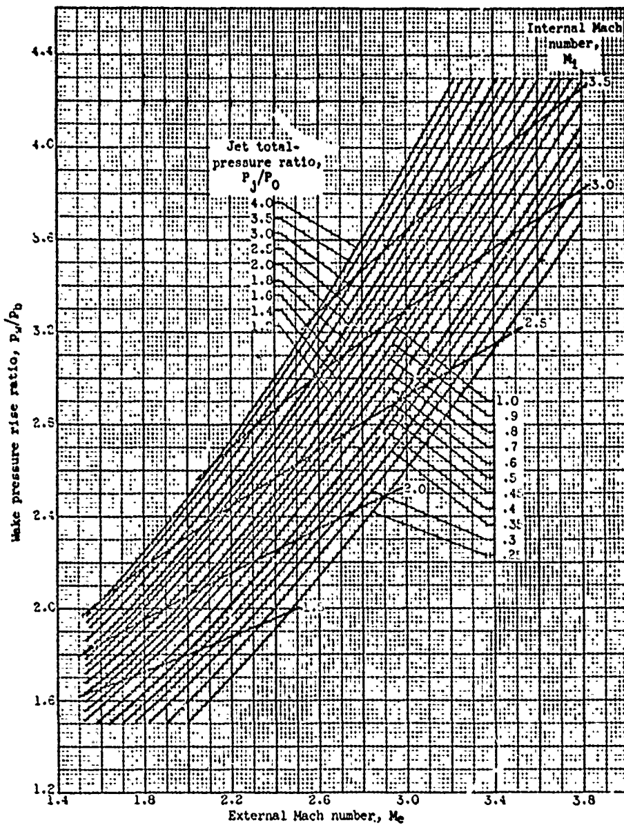
Figure 12. - Theoretical wake pressure rise ratio. T_e = T_1 ; X_e = X_1 ; two-dimensional flow.
