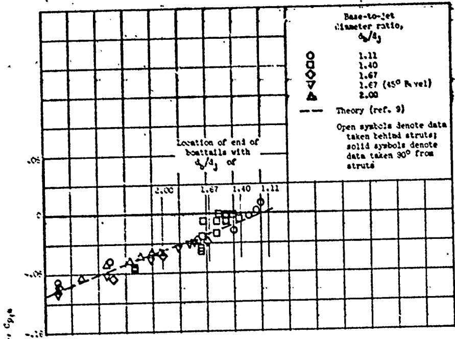
(a) Free-stream Mach number, 1.91. Instrumentation behind model support strut.
