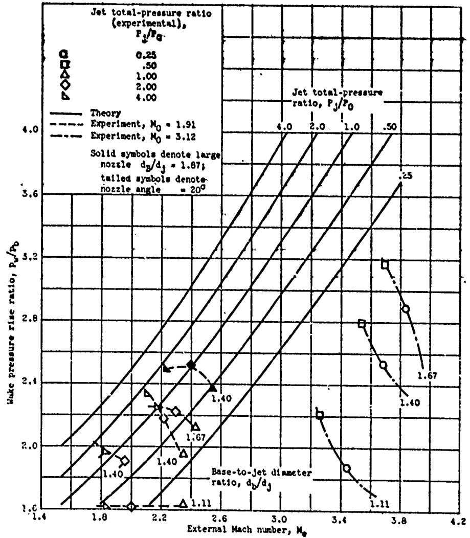
(b) Convergent-divergent nozzle; jet Mach number, 2.16; body-to-jet diameter ratio, 2.67 (except as noted).
