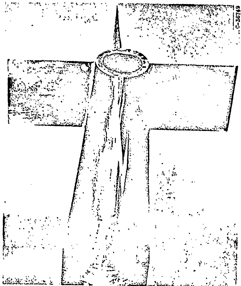
(b) Three-quarter view of cruciform tail on 5.63° boat tail. Figure 4. - Concluded. Tail interference model.
