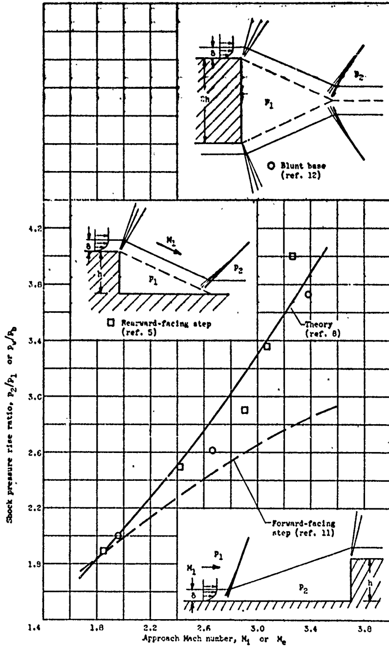
Figure 10. - Summary of pressure rise data. Turbulent mixing; h/\delta > 4 .
