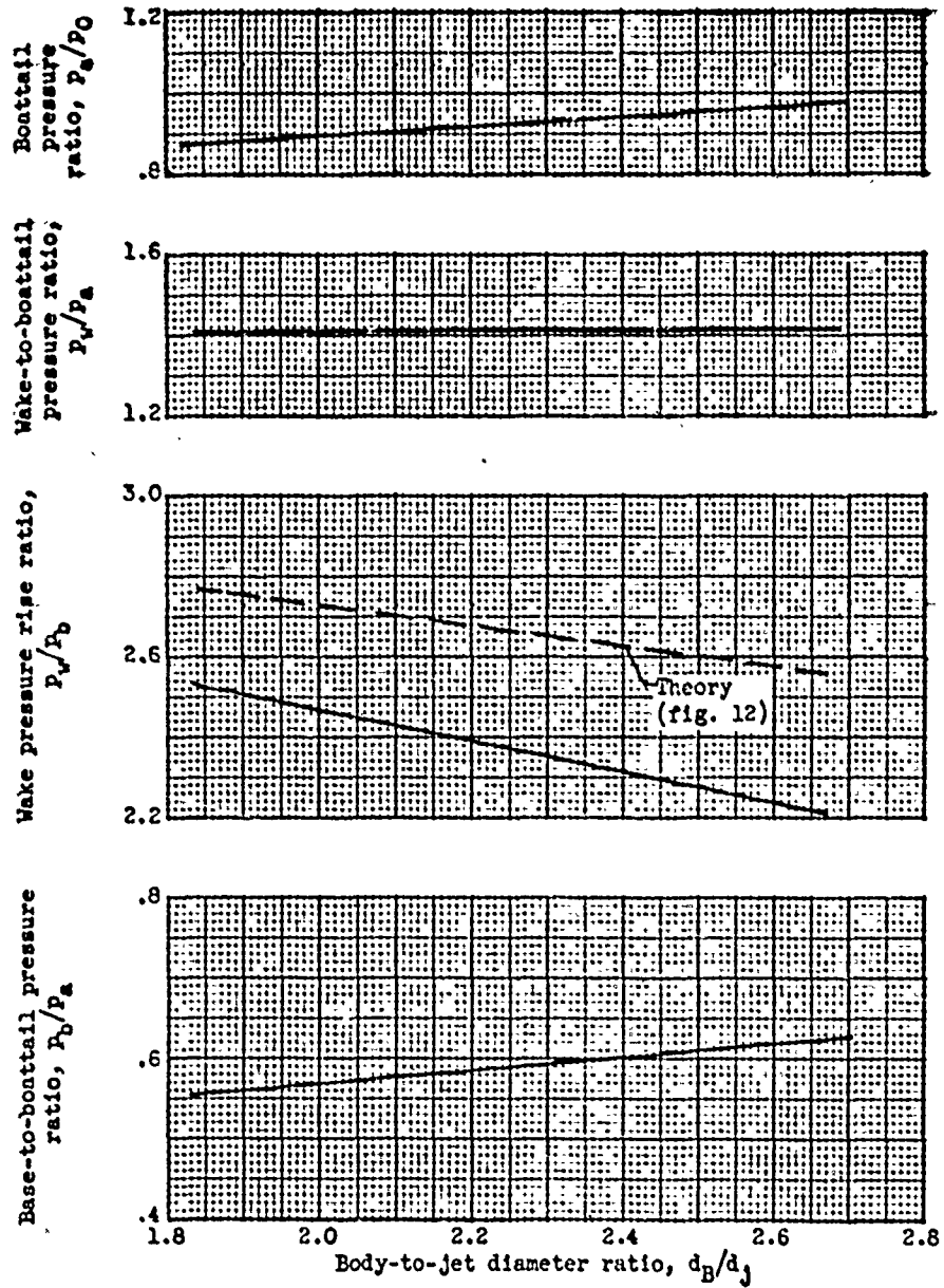
Figure 22. - Variation of base-pressure components with body-to-jet diameter ratio. Base-to-jet diameter ratio, 1.40; boattail angle, 5.63^\circ ; nozzle angle, 0^\circ ; jet Mach number, 2.19; free-stream Mach number, 1.91; jet pressure ratio, 15.
