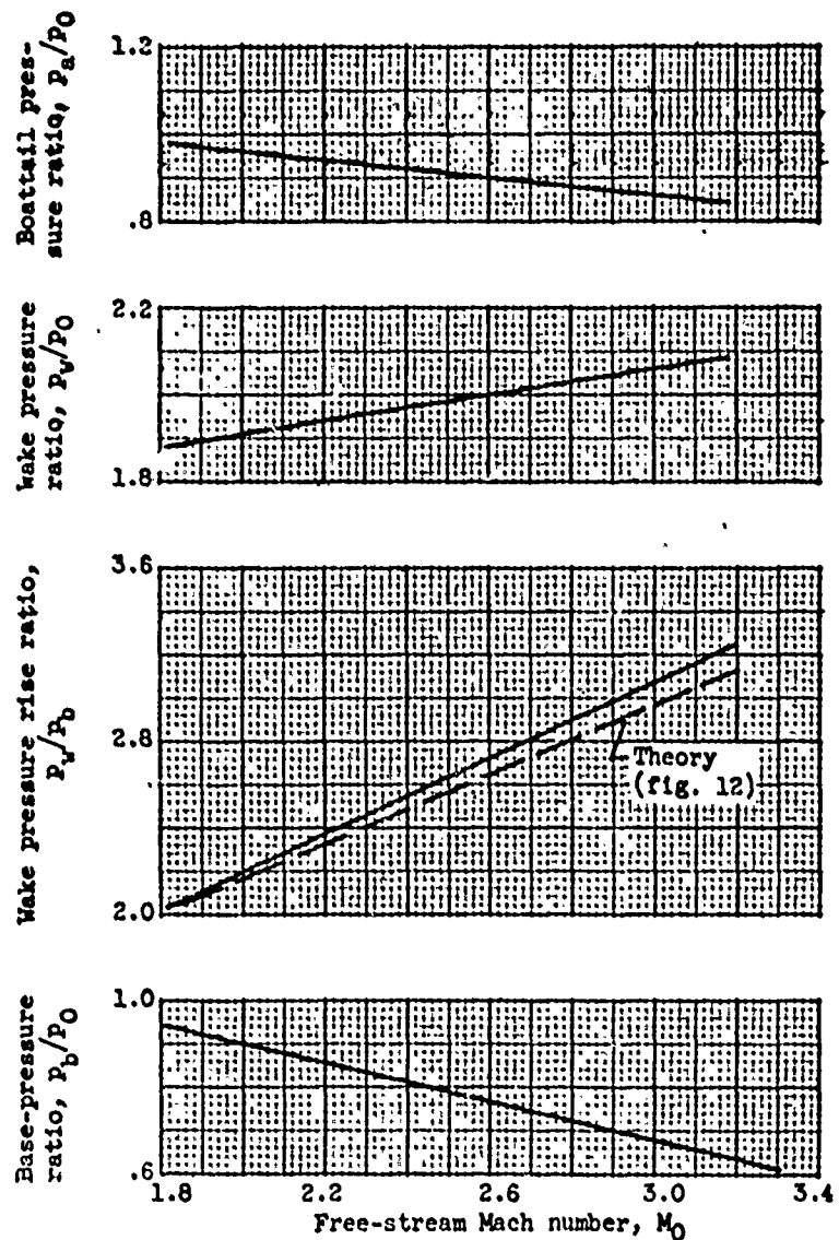
Figure 37. - Variation of component pressures with free-stream Mach number. Base-to-jet diameter ratio, 1.40; boattail angle, 5.63^\circ ; jet Mach number, 1.0; jet pressure ratio, 8.
