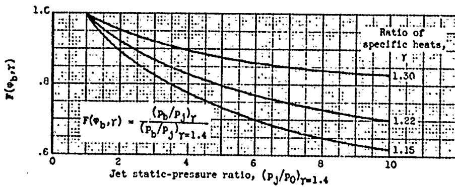
Figure 39. - Gamma correction function. Jet Mach number, 1.0; nozzle angle, 0°.
