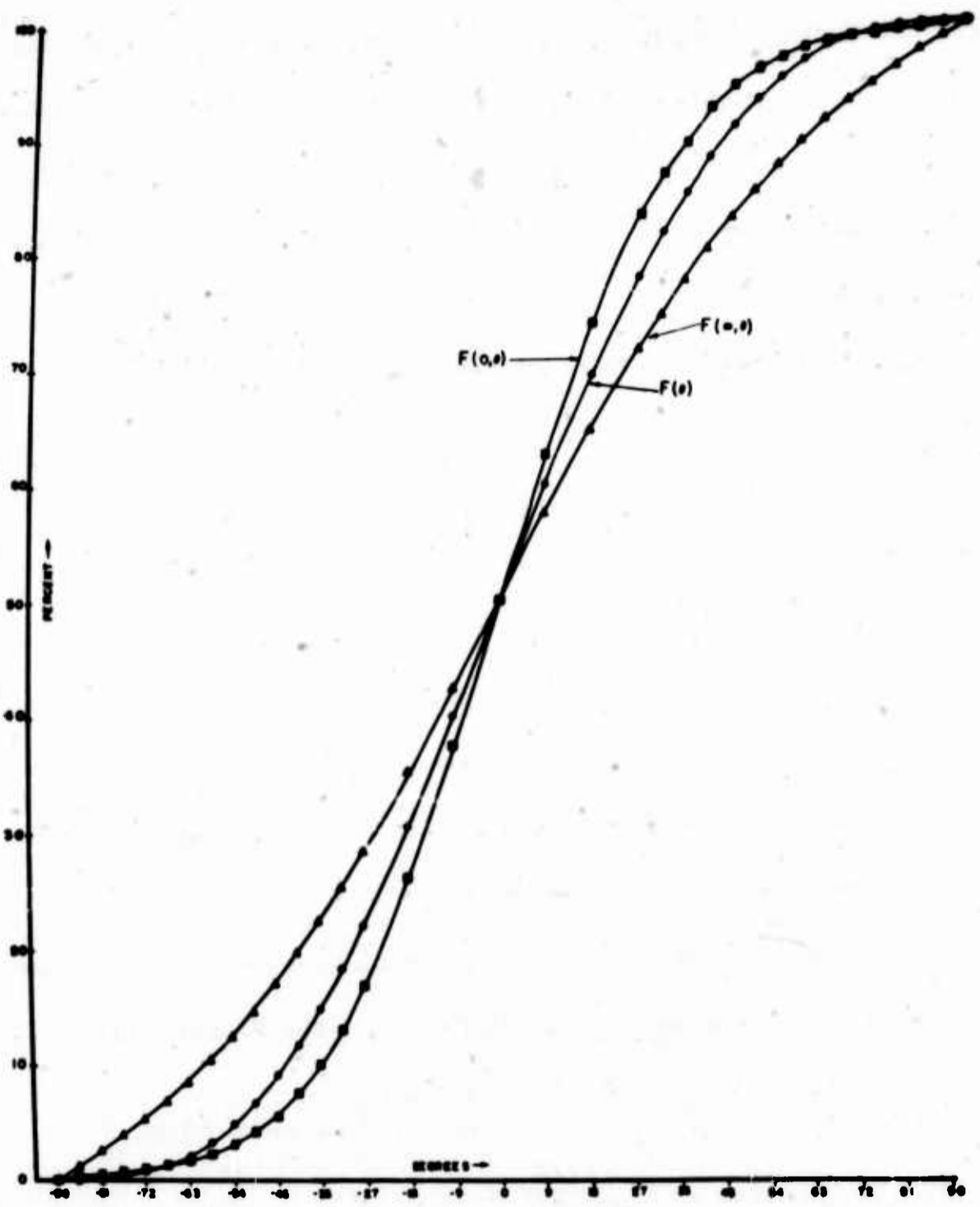
Fig. 11.32 ANGULAR SPREADING FACTOR FOR F(0, \theta) , F(\pi/2) and F(\pi, \theta)
