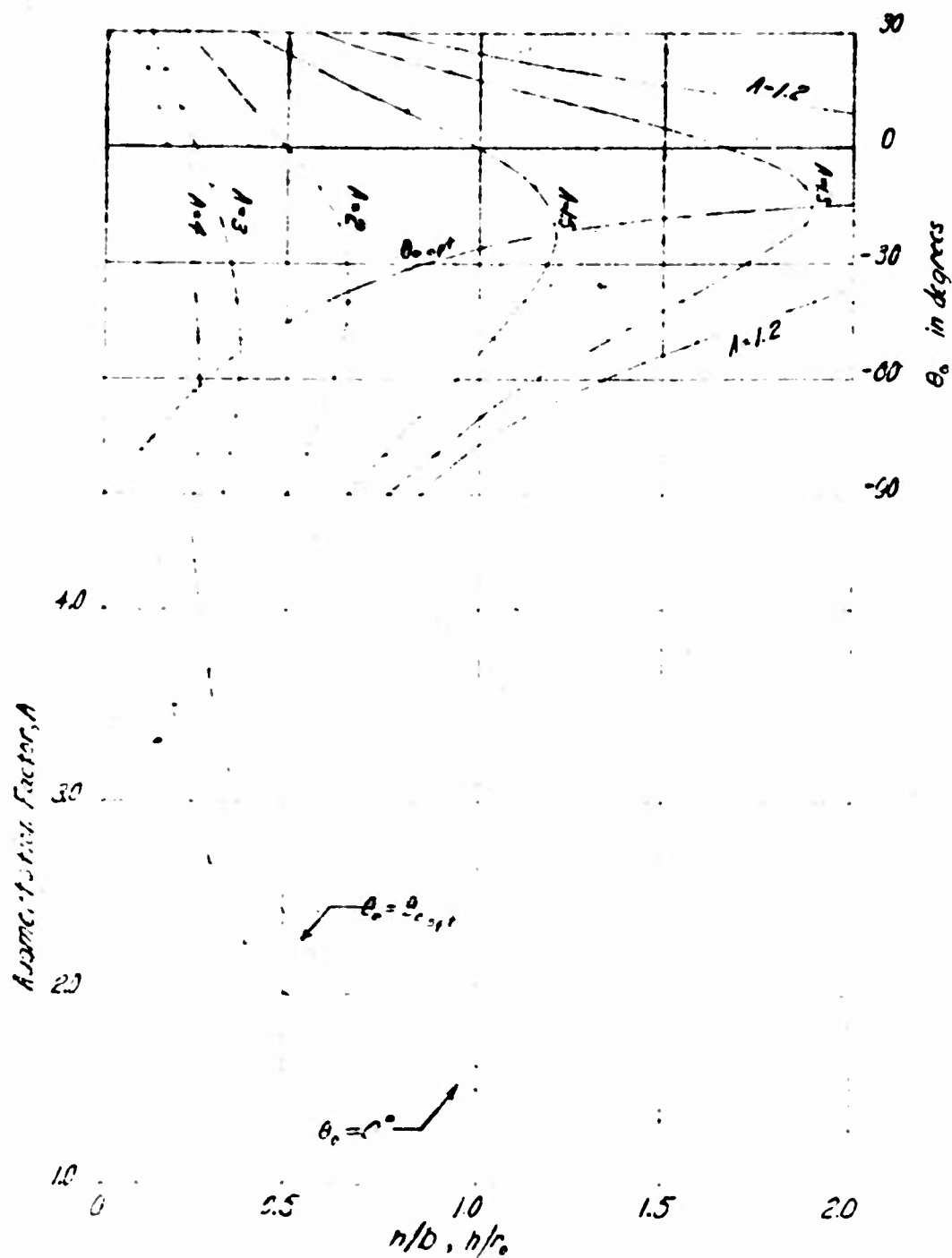
Figure 1- Augmentation Factor According to Equation (1)
