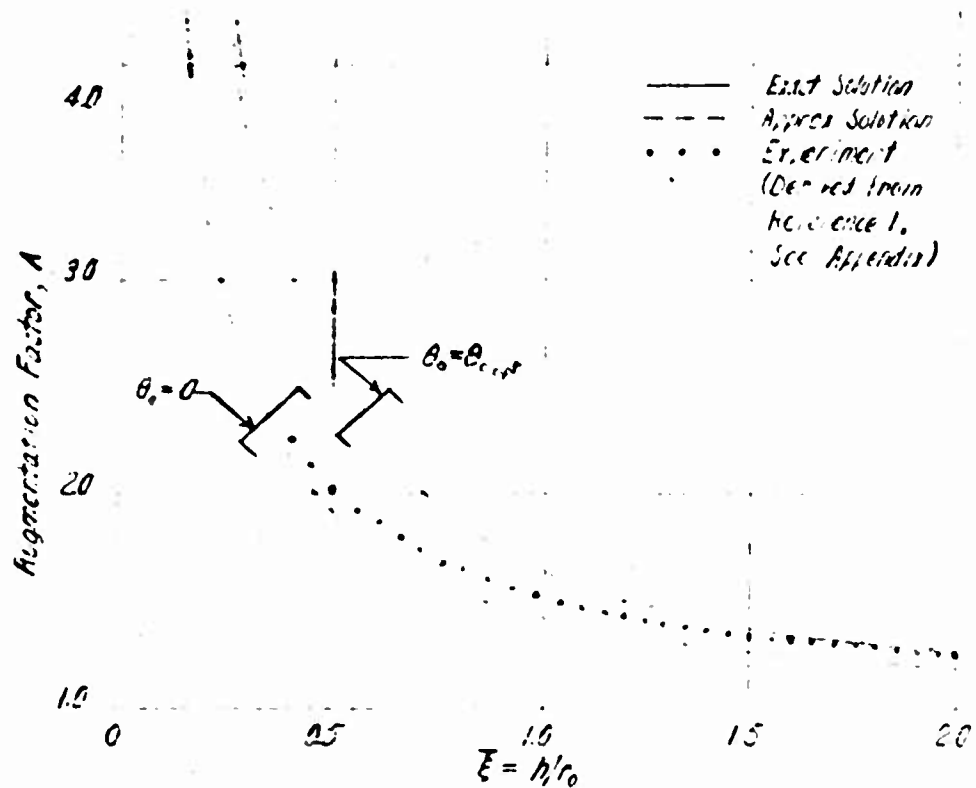
Figure 4 - Augmentation Factor for an Fully-Symmetric Annular Nozzle
