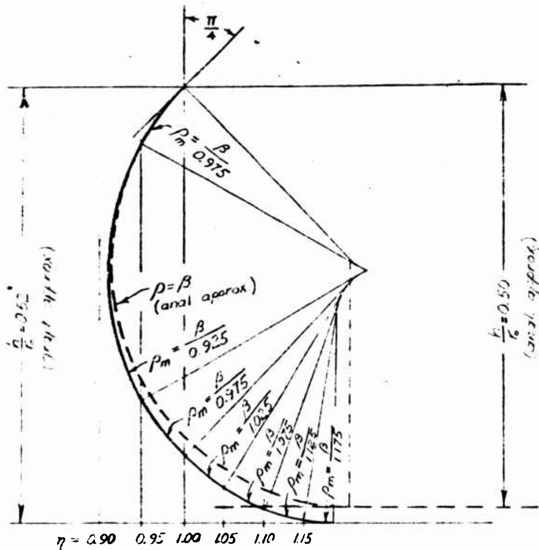
Figure 2—Illustrative Example of the Graphical Approximation of the Set of Points for an Assumed Horizontal Wave Ground-Effect Augmentation
