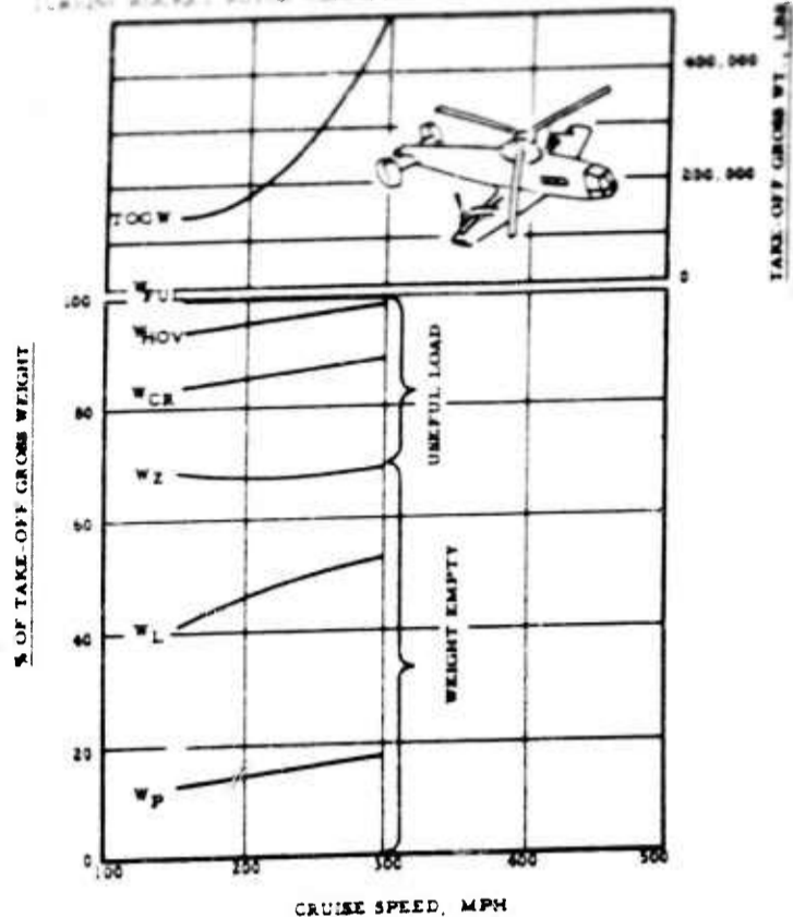
CURRENT MILITARY SHIPBOARD HELICOPTER WITH TURBOPROPS
