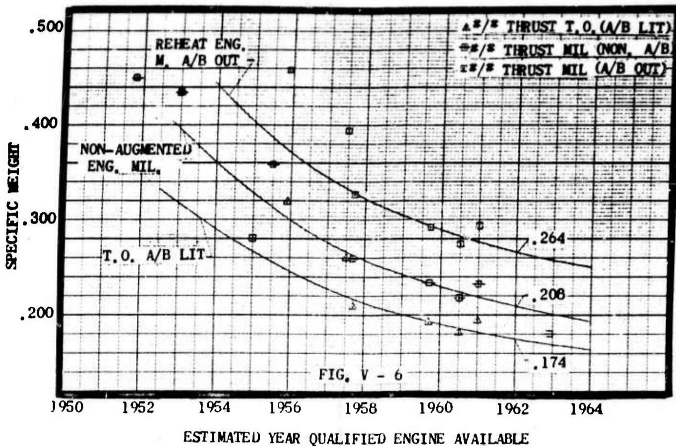
Figure V-6 presents specific weight trend curves for non-augmented and afterburner equipped turbojet engines. The specific weights of typical turbojet engines as indicated by an asterisk (*) in Figure V-2 have been plotted against the year in which these engines are scheduled to complete their qualification testing.
