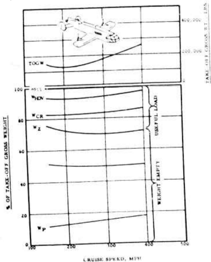
TURBINE ROCKET ROTOR-PROPELLER DRIVEN RETRACTOPLANE
