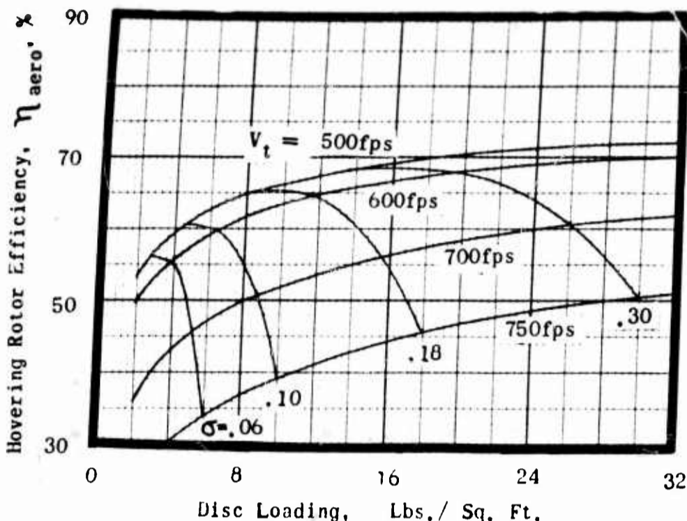
Fig. VI-3b Hovering Rotor Efficiency vs. Disc Loading NACA 0015 Airfoil (Overlapped Rotors) \bar{C}_L = .6 6000' Altitude, Ambient Temp, = 95 F
