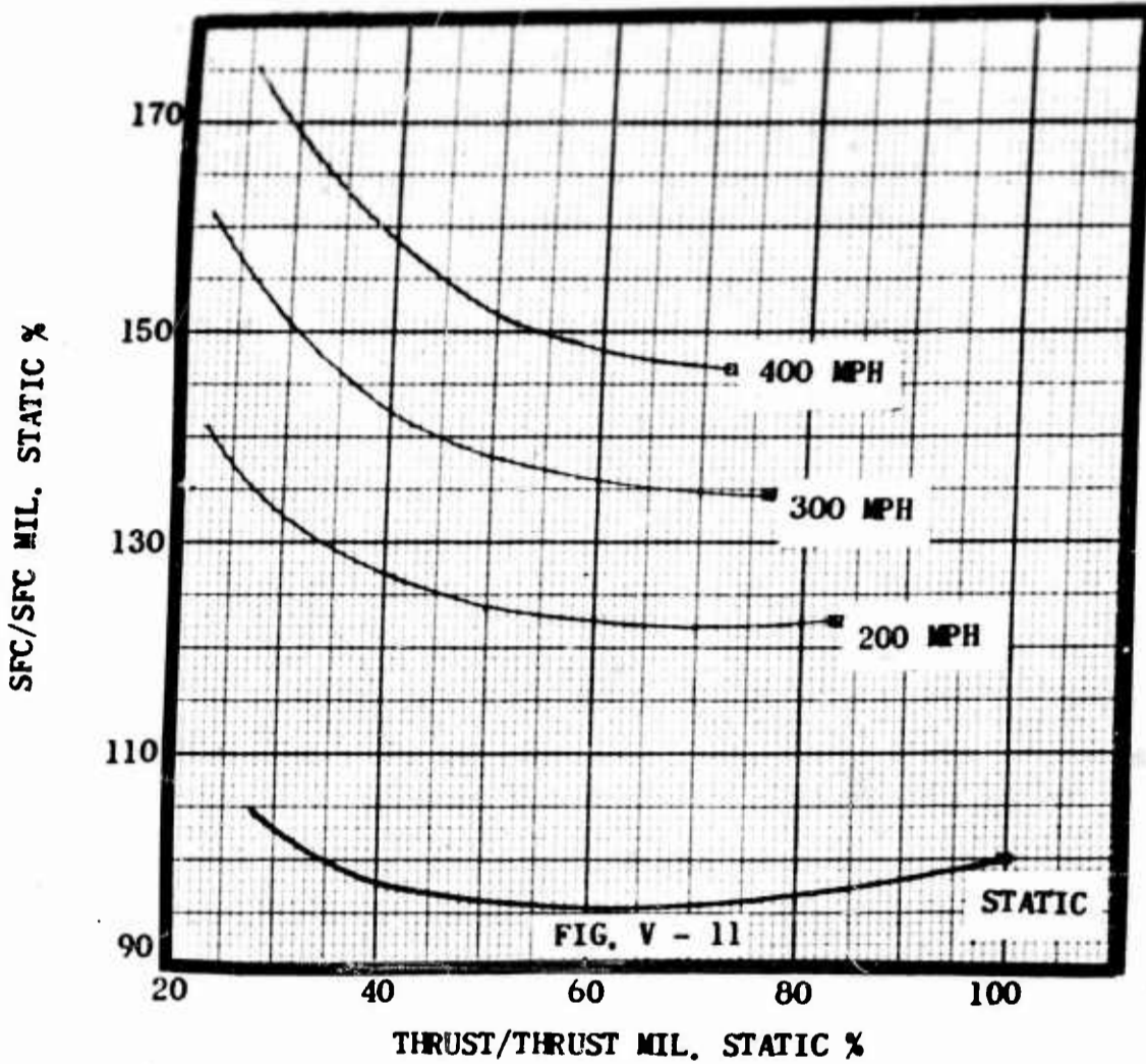
Figure V-11 represents the ratio of part load specific fuel consumption at the noted flight speeds to static military thrust specific fuel consumption as a function of the ratio of part load thrust at these flight speeds to static military thrust for a typical ducted fan engine.
