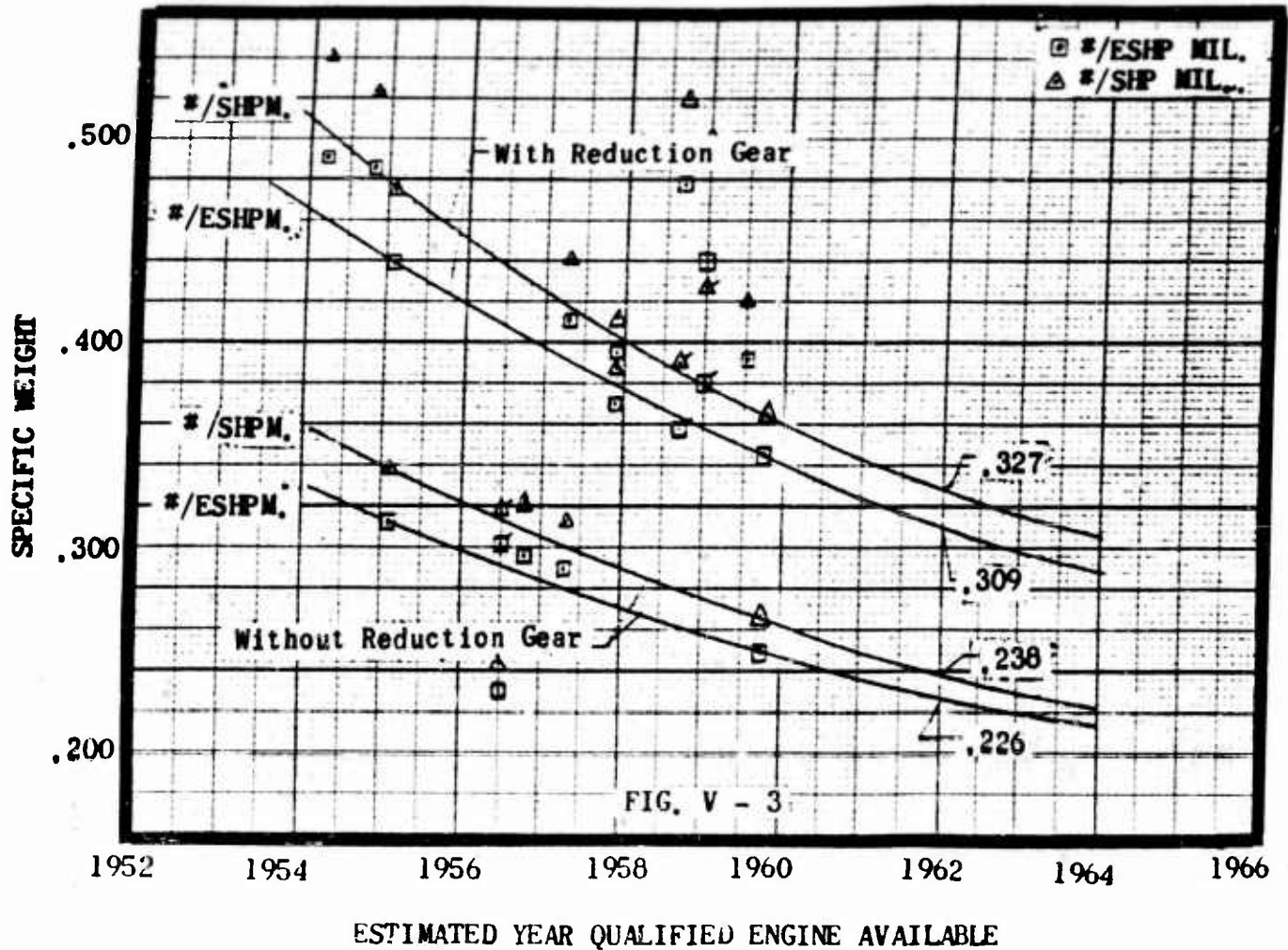
FIG. V - 3 ESTIMATED YEAR QUALIFIED ENGINE AVAILABLE Figure V-3 presents specific weight trend curves for shaft turbine engines with reduction gearing to provide a shaft speed of approximately 1,000 RPM and for direct drive turbines with shaft speeds of approximately 10,500 RPM. The specific weights of typical shaft turbine engines as indicated by an asterisk (*) in Figure V-2 have been plotted against the year in which these engines are scheduled to complete their qualification testing.
