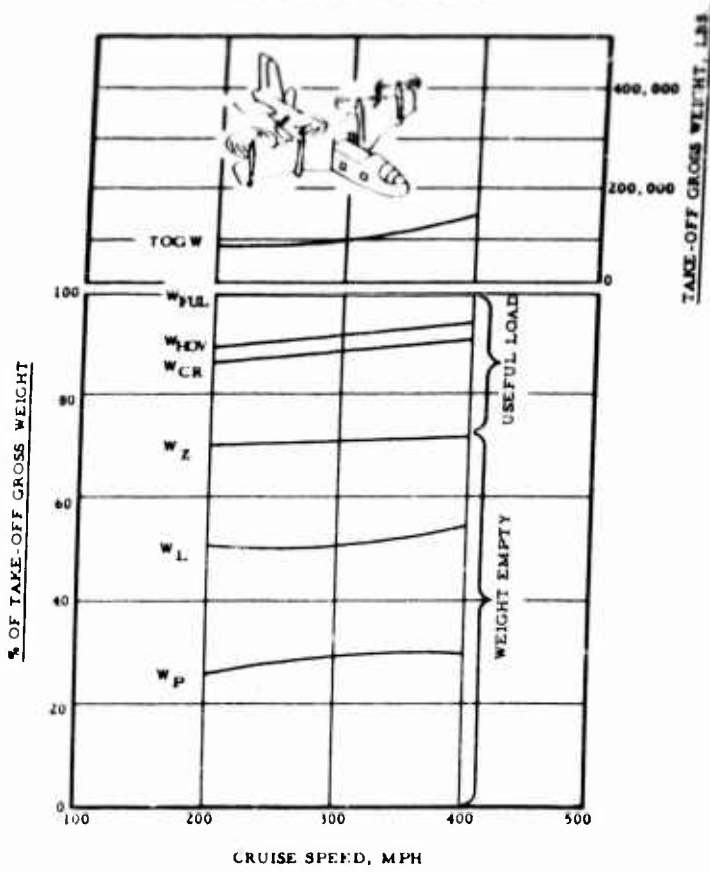
TILTING WING-PROPELLER
