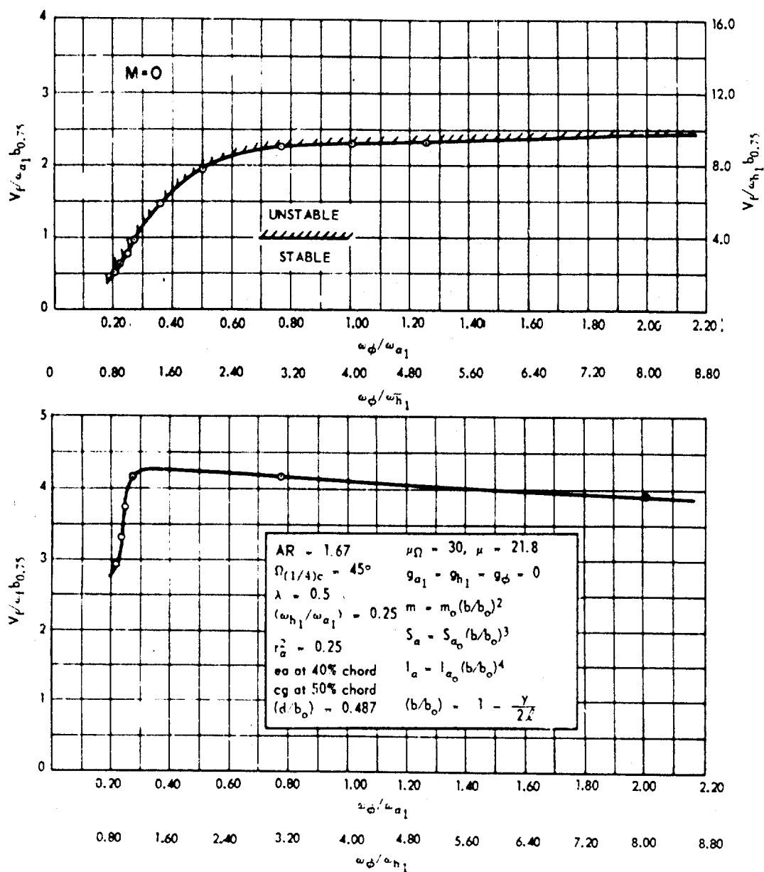
Fig. 2. Flutter parameters V_f / \omega_{a1} b_{0.75} and V_f / \omega_{h1} b_{0.75} versus (\omega_\phi / \omega_{a1}) and (\omega_\phi / \omega_{h1}) from three-degree-of-freedom incompressible calculation.
