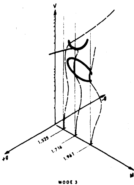
Fig. 11. Sketches of V versus g versus Mach number curves from four-degree-of-freedom calculations.
