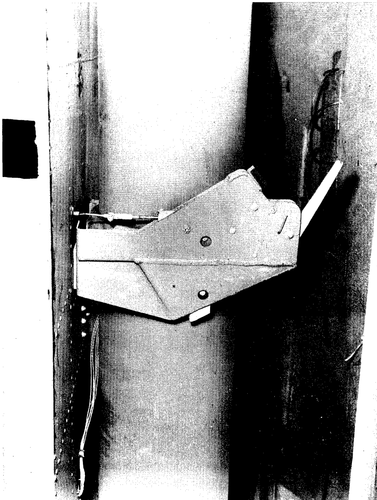
FIGURE 14. CATAPULT TRIGGER ASSEMBLY INSTALLATION ON CARRIAGE.
