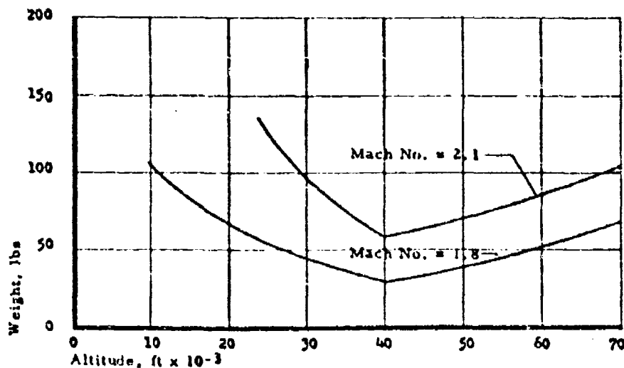
FIGURE 42 TOTAL EQUIVALENT WEIGHT VERSUS ALTITUDE FOR A FREON-11 VAPOR CYCLE COOLING SYSTEM ( T_{E0} = 275^\circ\text{F} )
