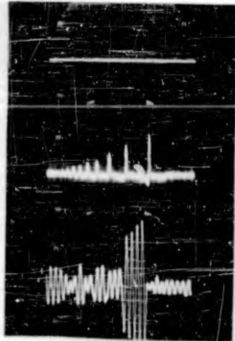
5" Drop - Q = 40 Upper Trace: Input Accel; 24g Max. Lower Trace: Response Acceleration
