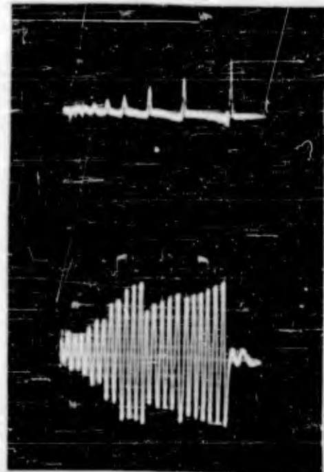
10" Drop - Q = 40 Upper Trace: Input Accel; 28g Max. Lower Trace: Response Acceleration
