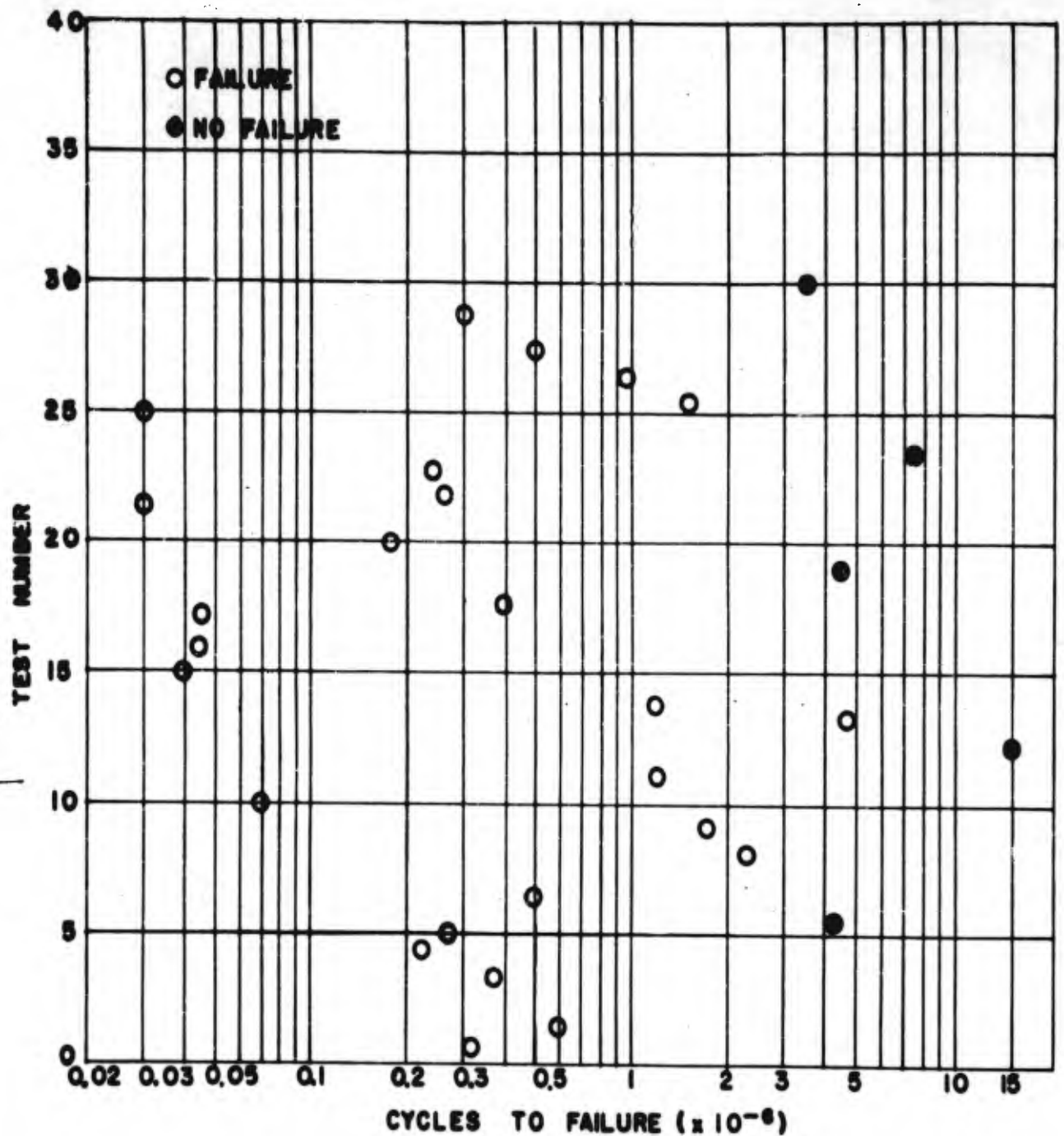
FIGURE 13. NUMBER OF CYCLES TO FAILURE IN VIBRATION TESTS CONDUCTED BY THE CALIDYNE CO.
