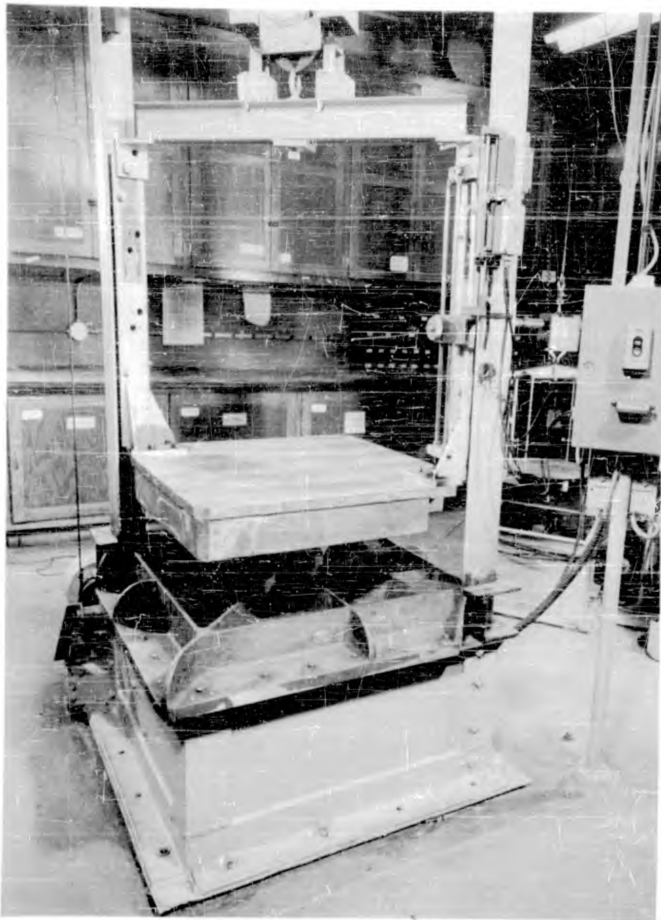
FIGURE 65. 150/400VD SHOCK TESTING MACHINE MODIFIED FOR REPEATED DROP TESTING.
