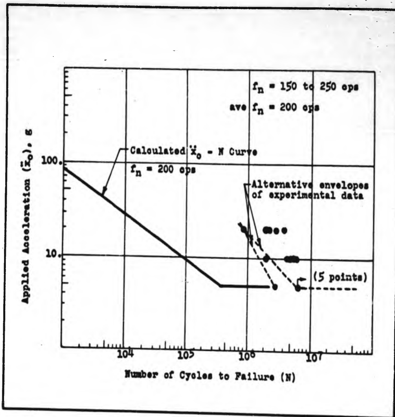
FIGURE 21. RESONANT FATIGUE TESTS OF 6J5 WGT TUBES(ARMOUR)
