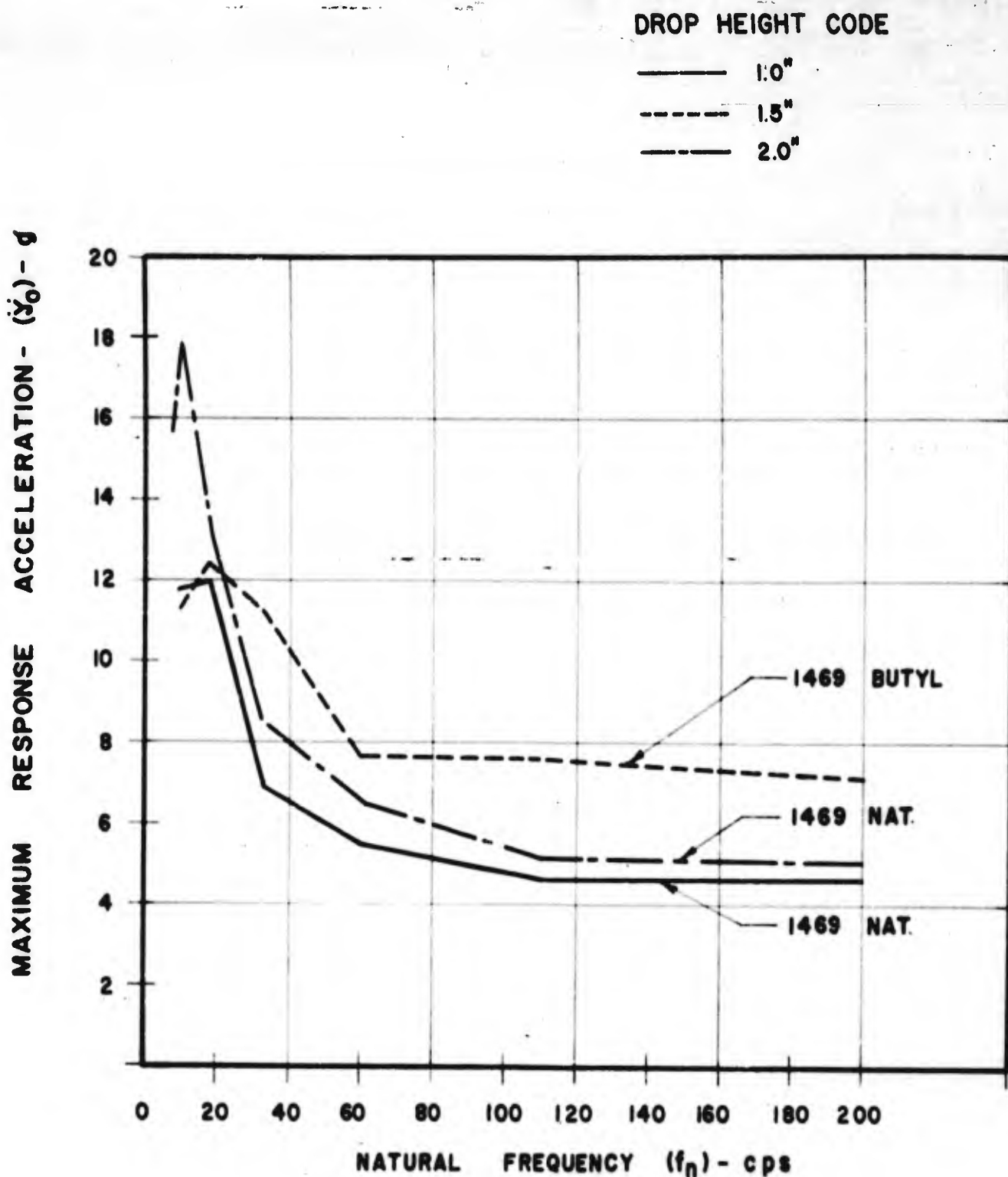
FIGURE 96. COMPARISON OF RESPONSE SPECTRA OBTAINED WITH NATURAL & BUTYL RUBBER PADS OF SAME CONFIGURATION - 150/400 MACHINE - NO TABLE LOAD - Q = 20
