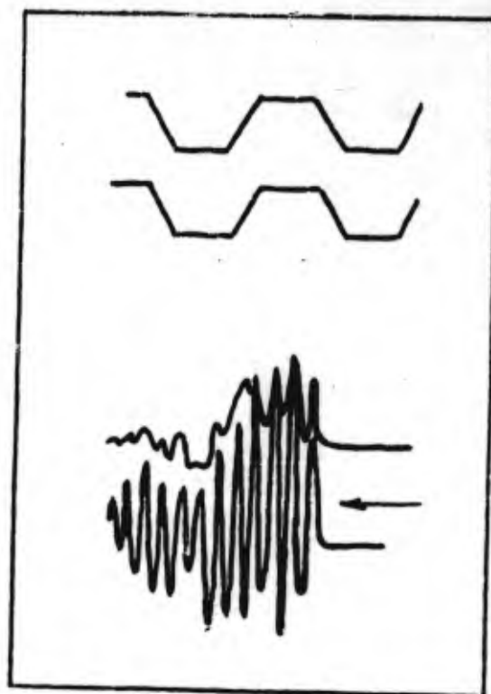
(B) 13 Inch Free Fall Time
