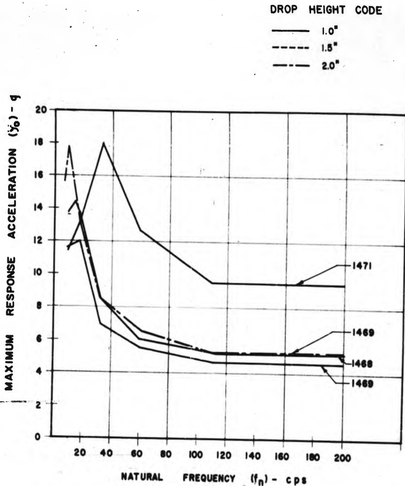
FIGURE 94. RESPONSE SPECTRA- 150/400 MACHINE FOR VARIOUS NATURAL RUBBER PAD CONFIGURATIONS AND DROP HEIGHTS. Q = 20 . NO TABLE LOAD.
