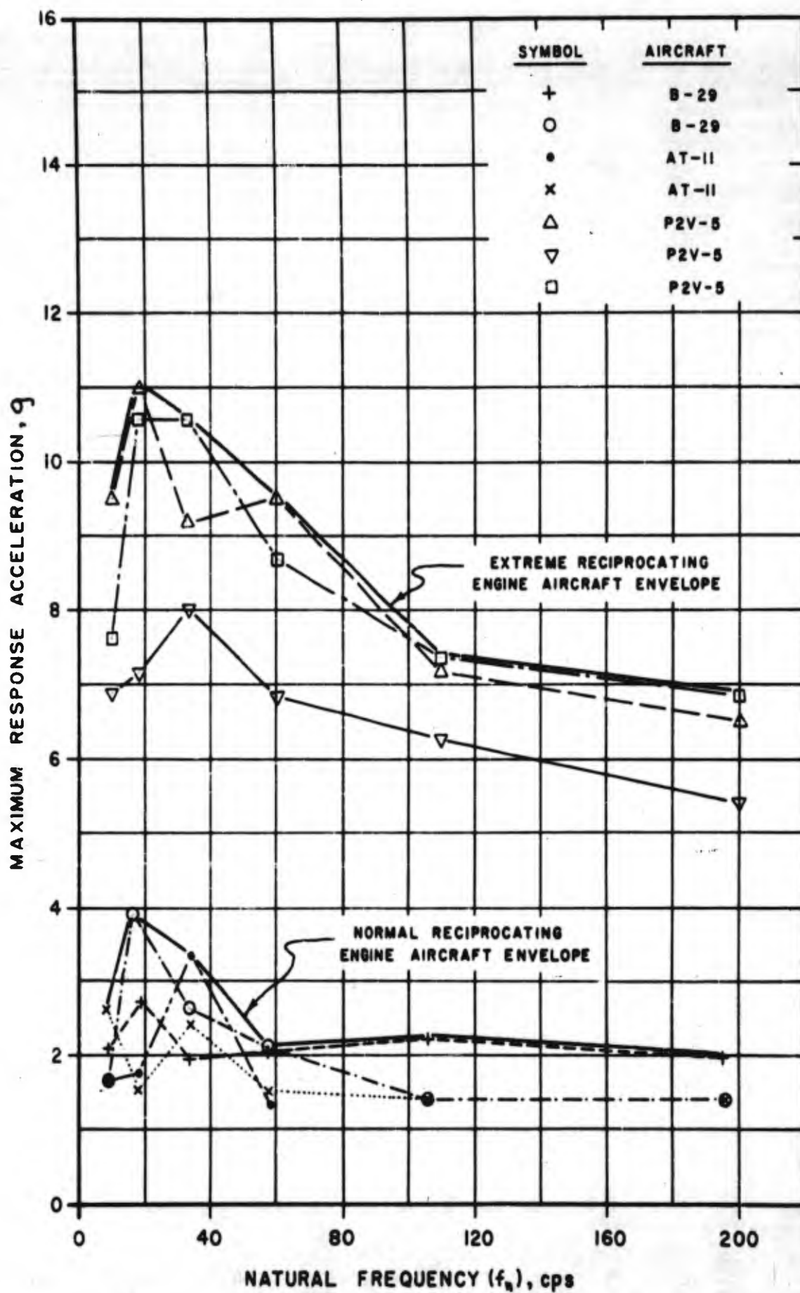
FIGURE 54. SHOCK SPECTRA FOR INDIVIDUAL LANDING RECORDS OF RECIPROCATING ENGINE AIRCRAFT, Q=20
