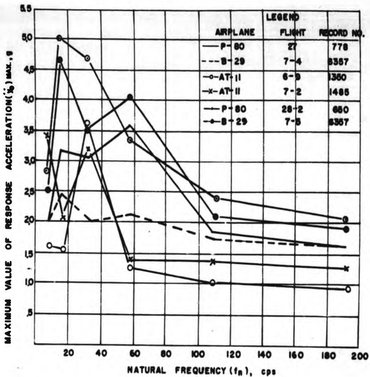
FIGURE 52. SHOCK SPECTRA FOR INDIVIDUAL LANDING RECORDS, Q = 50 .
