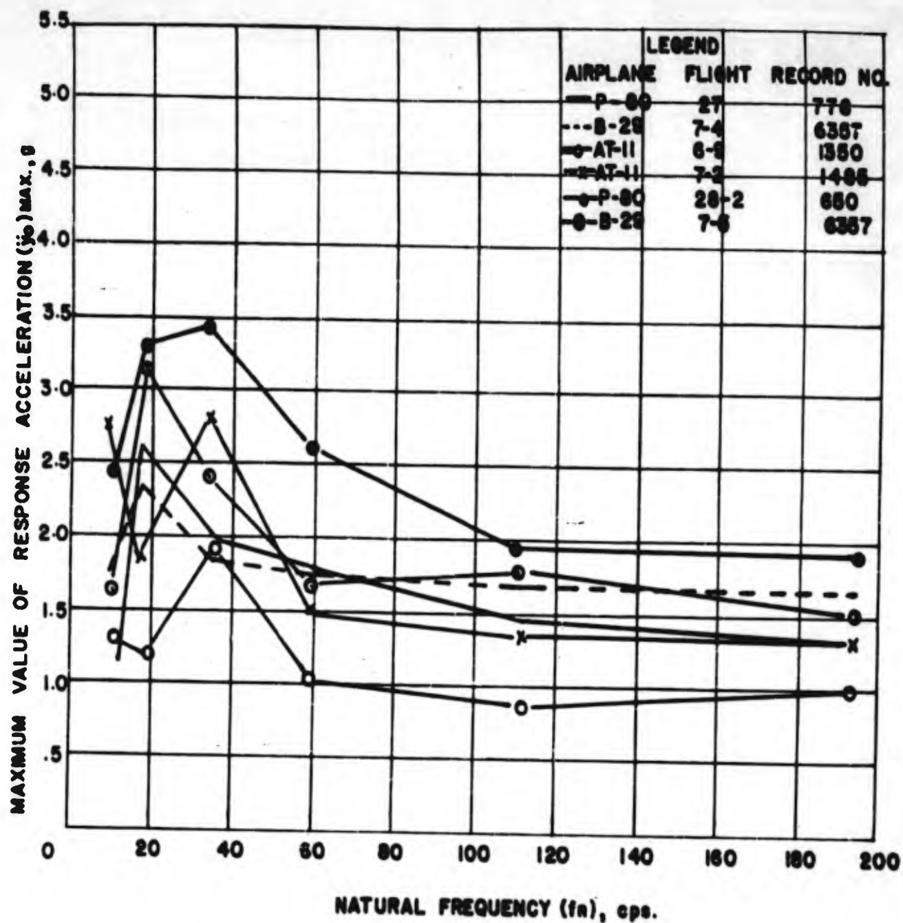
FIGURE 50. SHOCK SPECTRA FOR INDIVIDUAL LANDING RECORDS, \theta = 10 .
