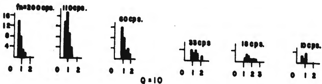
FIGURE 85. BLOCK DIAGRAMS OF RESPONSE ACCELERATION AS A FUNCTION OF NUMBER OF OCCURRENCES FOR SYSTEMS HAVING Q=10, 20, \text{ and } 50 , SUBJECTED TO P-80 LANDING SHOCK.
