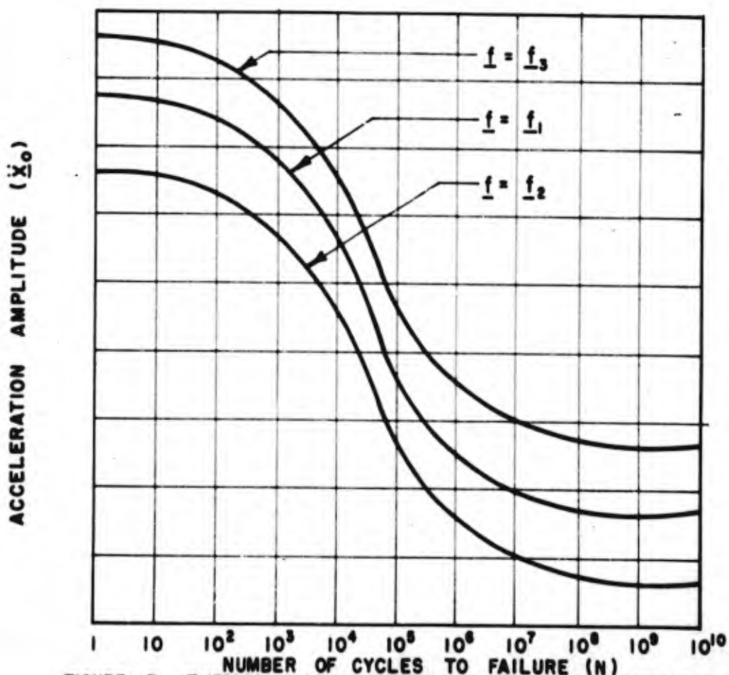
FIGURE 9. TYPICAL CURVE SHOWING ENDURANCE PROPERTIES OF SYSTEM ILLUSTRATED IN FIGURE 6 FOR A GIVEN NATURAL FREQUENCY AND KNOWN RELATION BETWEEN y_0 AND \underline{g} .
