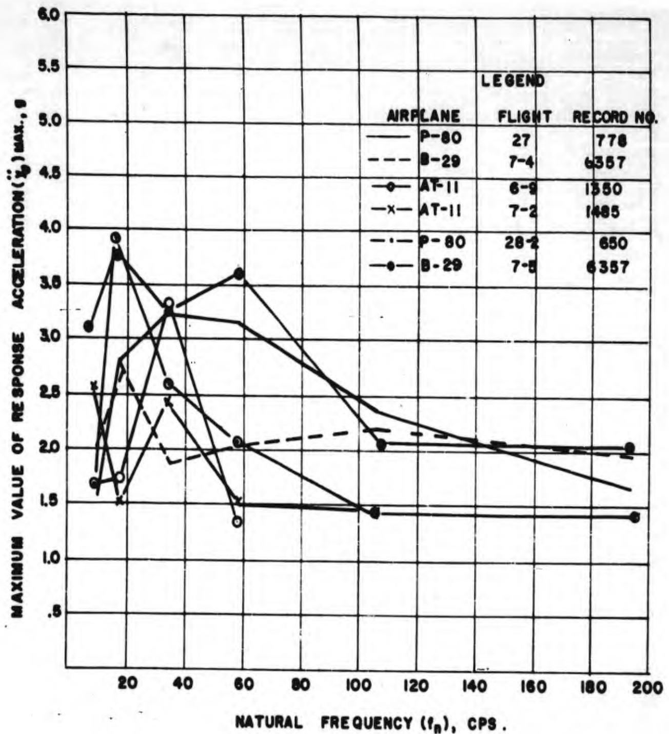
FIGURE 51. SHOCK SPECTRA FOR INDIVIDUAL LANDING RECORDS, \theta = 20^\circ .
