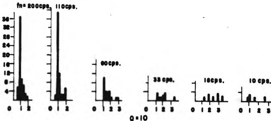
FIGURE 89. BLOCK DIAGRAMS OF RESPONSE ACCELERATION AS A FUNCTION OF NUMBER OF OCCURRENCES FOR SYSTEMS HAVING Q = 10, 20, \text{ \& } 50 , SUBJECTED TO P-80 LANDING SHOCK.
