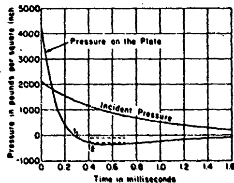
Figure 10 - Pressure on a Plate, in the Absence of Cavitation, plotted on a Time Base
