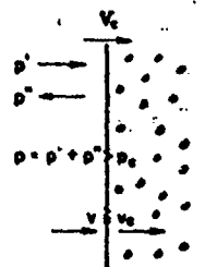
Figure 5 - A Plane Forced Closing-Front advancing toward the Right
