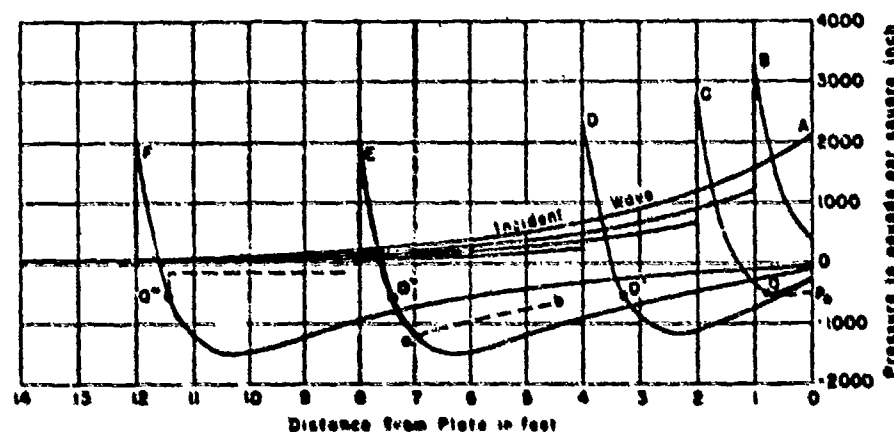
Figure 11 - Distributions of Pressure behind a Plate at Successive Instants of Time, in the Absence of Cavitation
