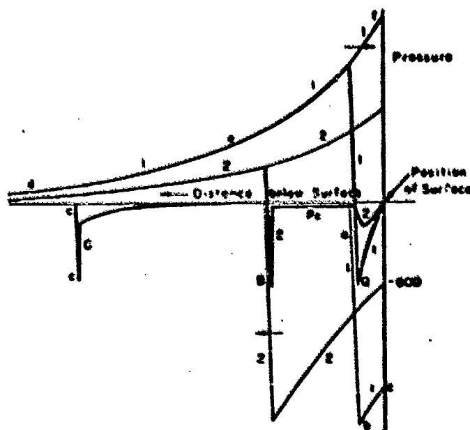
Figure 14 - Diagram illustrating the Distribution of Pressure below the Surface of the Sea, as explained in the Text
