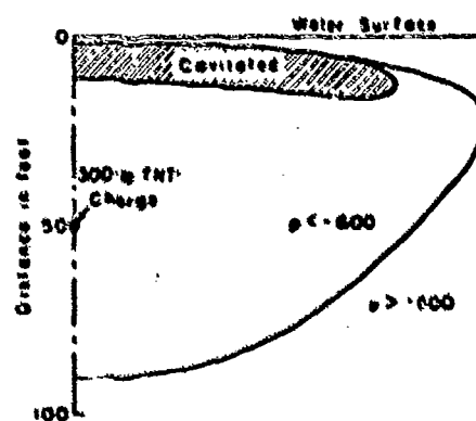
Figure 13 - Diagram of Region of Reduced Pressure following Reflection of a Pressure Wave from the Surface
