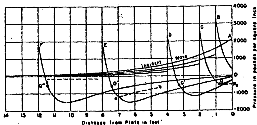
Figure 11 - Distributions of Pressure behind a Plate at Successive Instants of Time, in the Absence of Cavitation
