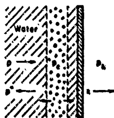
Figure 9 - Diagram illustrating the Case in which Bulk Cavitation occurs in the Water
