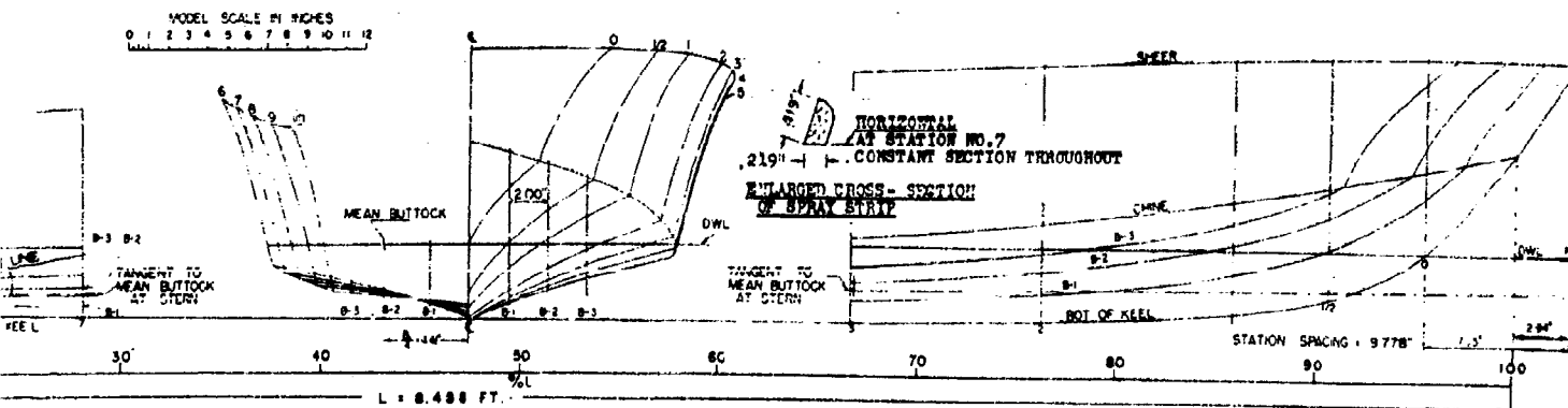
Figure 5 - Design Data Sheet for Model 3722
