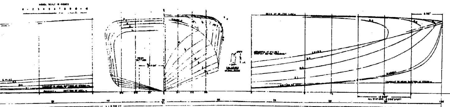
Figure 2 - Design Data Sheet for Model 3592-1
