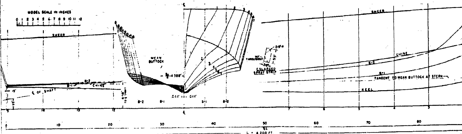
Figure 4 - Design Data Sheet for Model
