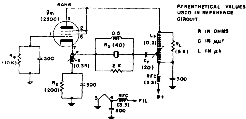
FIG. 31 — GROUNDING GRID OSCILLATOR AT 105 mcs.
