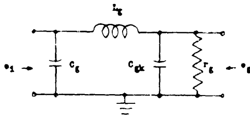
Fig. 30 - Equivalent Circuit of the Pi Network
