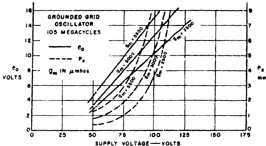
FIG. 32 — CIRCUIT PERFORMANCE WITH CHANGES IN g_m .
