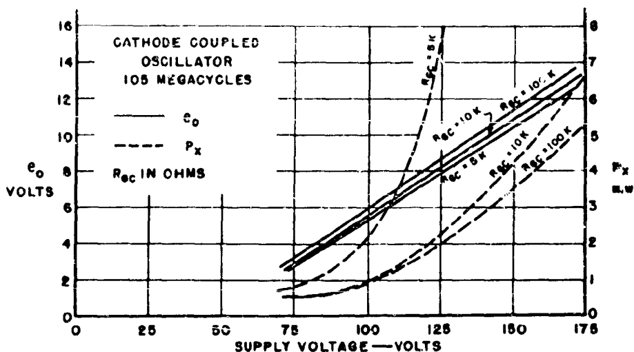
FIG. 45—CIRCUIT PERFORMANCE WITH CHANGES IN R_{gc} .
