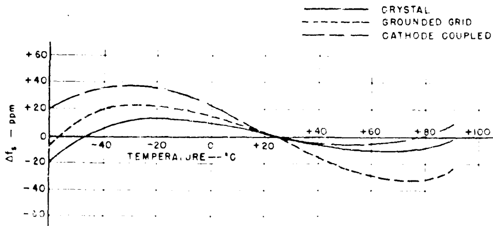
FIG. 23b — FREQUENCY TEMPERATURE CHARACTERISTICS
